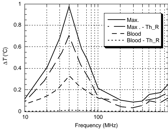
FIGURE 10.27 Maximum temperature increases ( \Delta T ) in the body and blood of a subject wearing shoes, as a function of frequency, with or without thermoregulation ( Th\_R ) for a P_{inc} equal to the limits set by ICNIRP [101].
