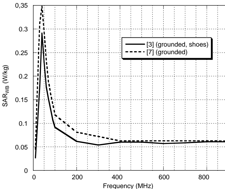
FIGURE 10.20 SAR as averaged over the whole body as a function of the frequency.
