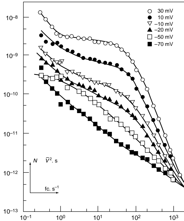
FIGURE 5.15 Voltage noise spectra of a frog node of Ranvier at different levels of membrane potential. (From Sichenga, E. and Verveen, A.A., in Proceedings of the 1st European Biophysics Congress , Vol. 5, Verlag Wiener Medizinischen Akademik, Vienna, Austria, 219, 1971. With permission.)
