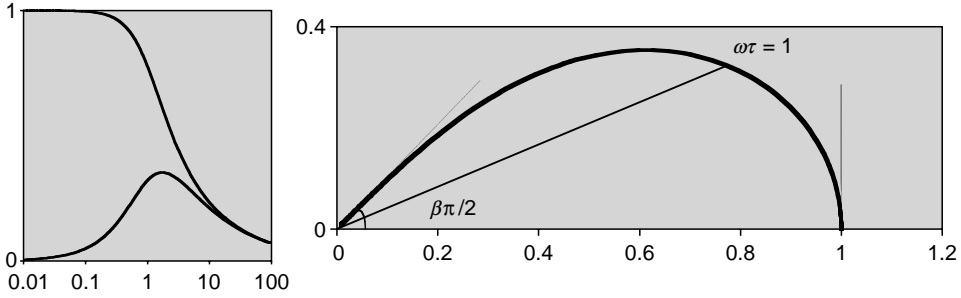
FIGURE 3.6 Left: Frequency dependence of normalized permittivity (\epsilon' - \epsilon_\infty)/(\epsilon_s - \epsilon_\infty) and loss factor \epsilon''/(\epsilon_s - \epsilon_\infty) for a Cole–Davidson model with \beta = 0.5 . Right: Plot of normalized loss factor against permittivity showing the characteristic Cole–Davidson skewed arc where the maximum in \epsilon'' does not correspond with \omega\tau = 1 ; this point is found at the interception of the bisector of the high-frequency limiting angle with the data plot.
