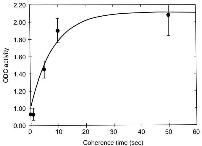
FIGURE 5.7 Plot of the enhancement of ODC activity (exposed/control) as a function of the coherence time, \tau_{\text{coh}} , of the applied field. The solid line is the best fit to the mathematical function given by Equation 5.44, where \tau_{\text{cell}} is found to be 8.2 sec. The experimental points shown represent a minimum of six different exposures. (© Academic Press; From Litovitz, T.A., Krause, D., and Mullins, J.M., Biochem. Biophys. Res. Commun. , 178, 3, 862, 1991. With permission.)
