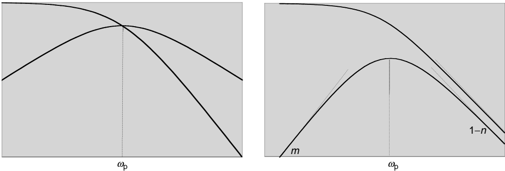
FIGURE 3.10 Log–log plot of the normalized permittivity and loss factor against frequency for a Debye-type behavior (left) and a non-Debye response (right).
