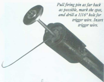
M203 firing pin removed from breech, showing hole for trigger wire.
