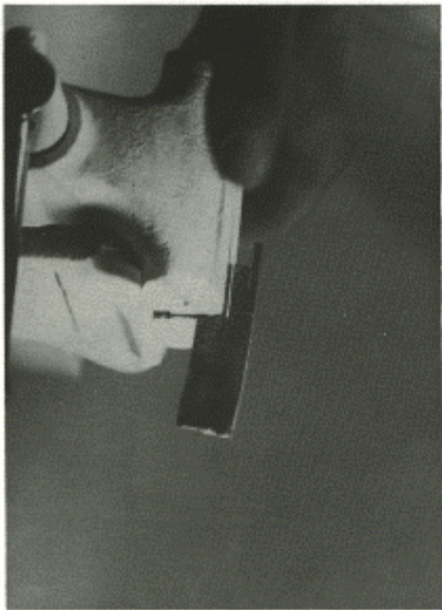
With the stem and body width cuts completed, the auto sear blank is cut to length (arrow).
