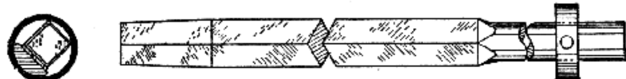
Shotgun boring bit, also sometimes used on rifle barrels. End view shows how wood packing strip and shims are used.
