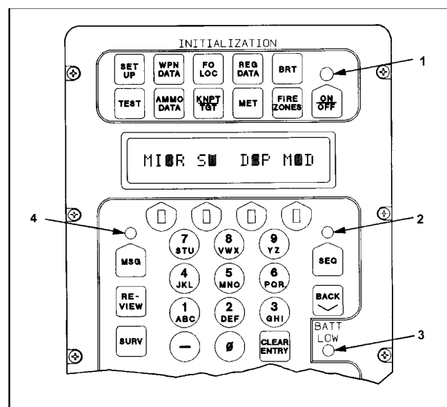
Figure 6-8. LED Indicators.
