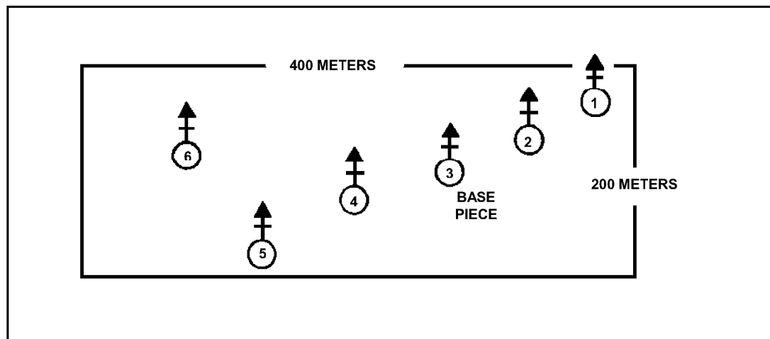
Figure E-6. Dimension parameters for six-mortar platoon.
