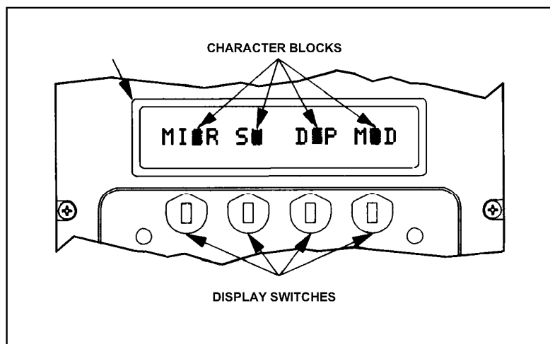
Figure 6-7. Display switches.
