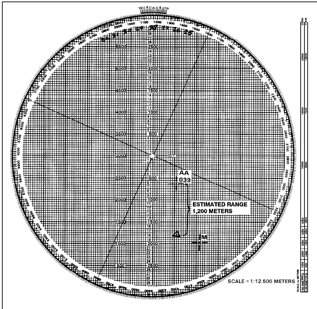
Figure 12-25. Estimate of range from reference point of FO's location.
