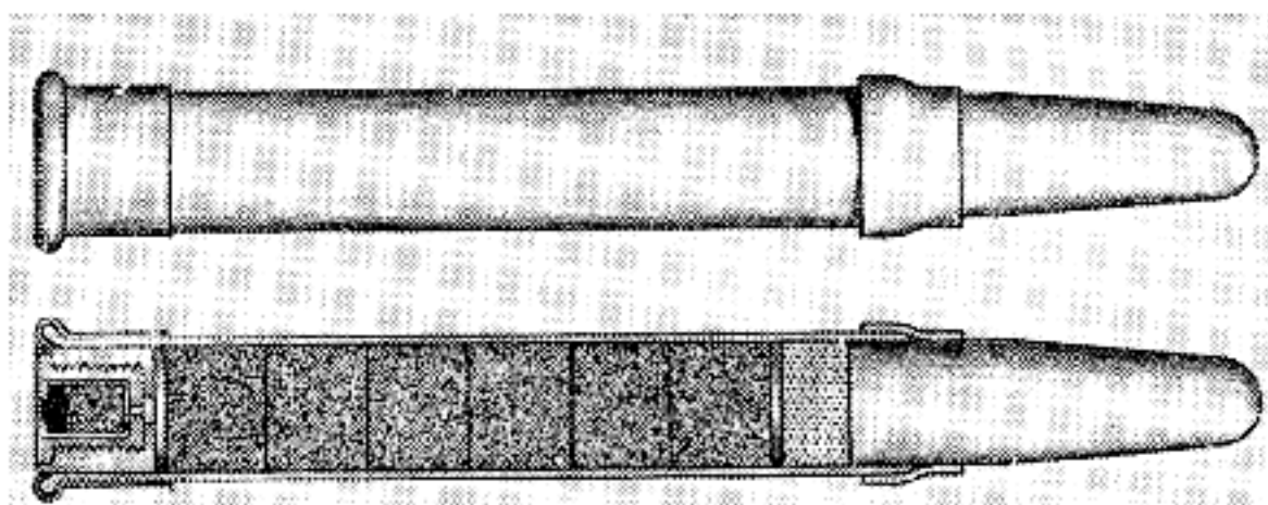
The Chassepot Rifle Cartridge that Was Used in the Mitrailleuse.
