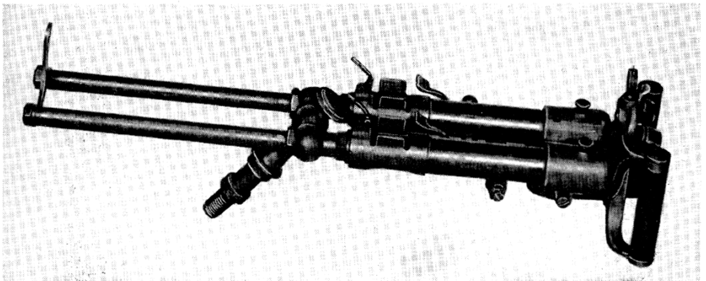
Villar-Perosa Aircraft Machine Gun, 9 mm.
