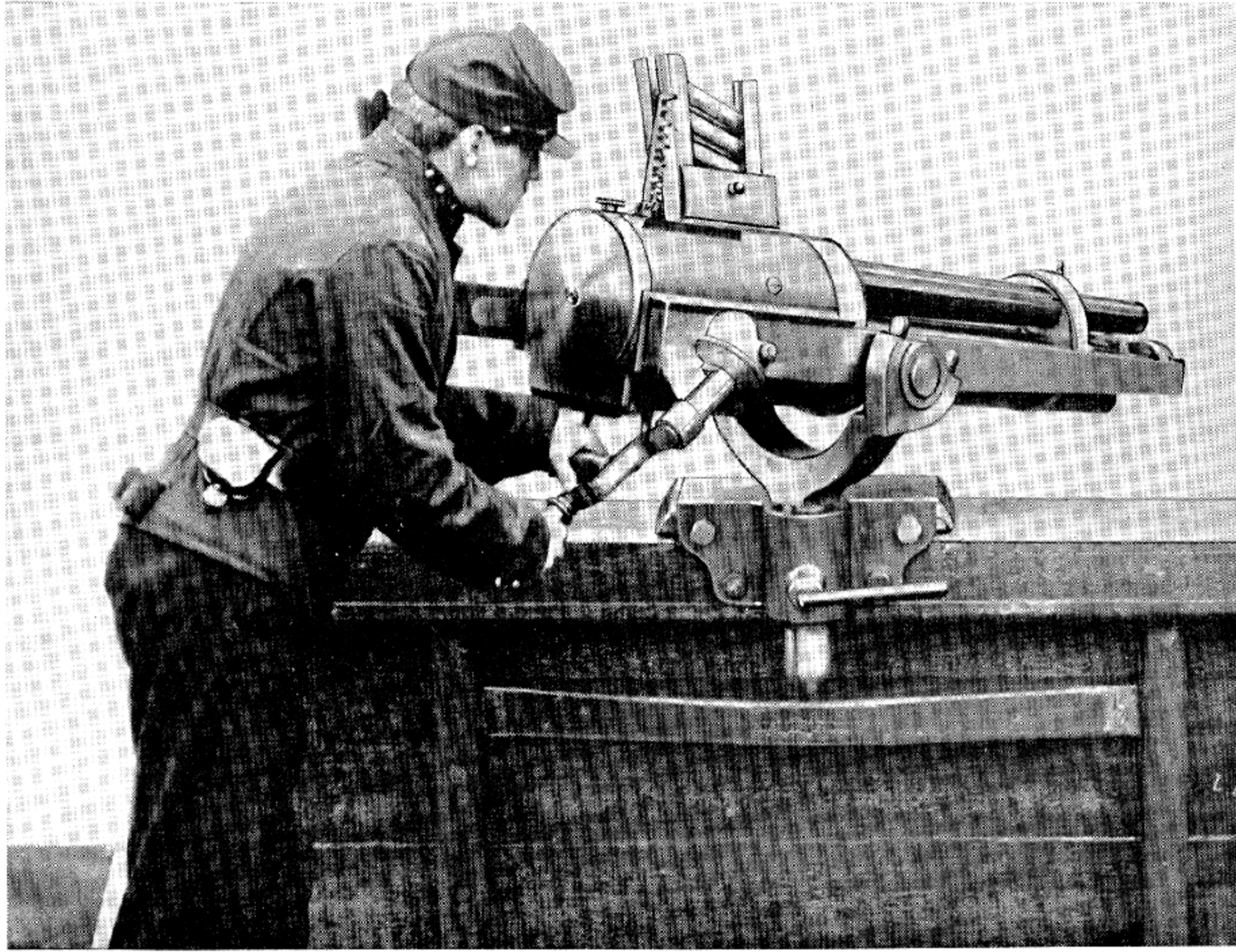
Hotchkiss 37 mm Revolving Cannon Mounted on Ship's Gunwale.
