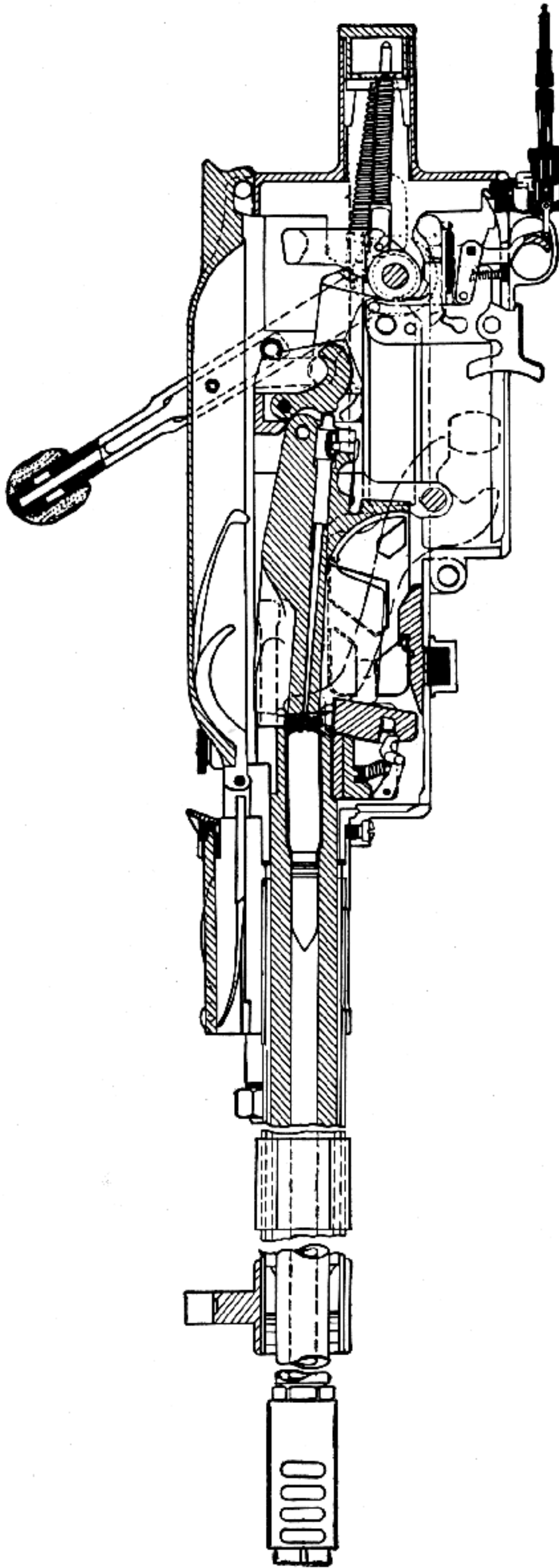
Section Drawing of the Madsen 23-mm Automatic Aircraft Cannon.
