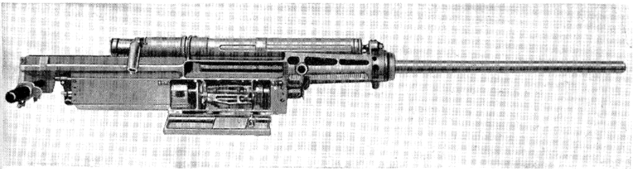
Szakats 20-mm Automatic Aircraft Cannon, Model SZC.
