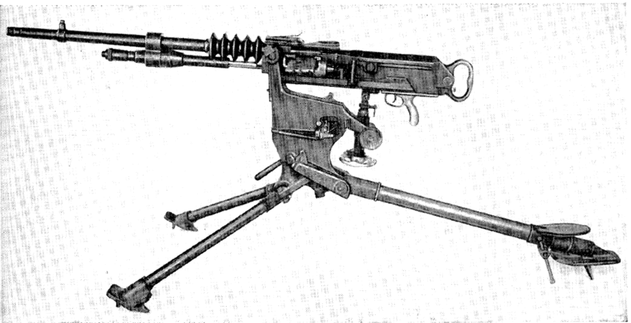
Hotchkiss Machine Gun, Model 1914, 8 mm.
