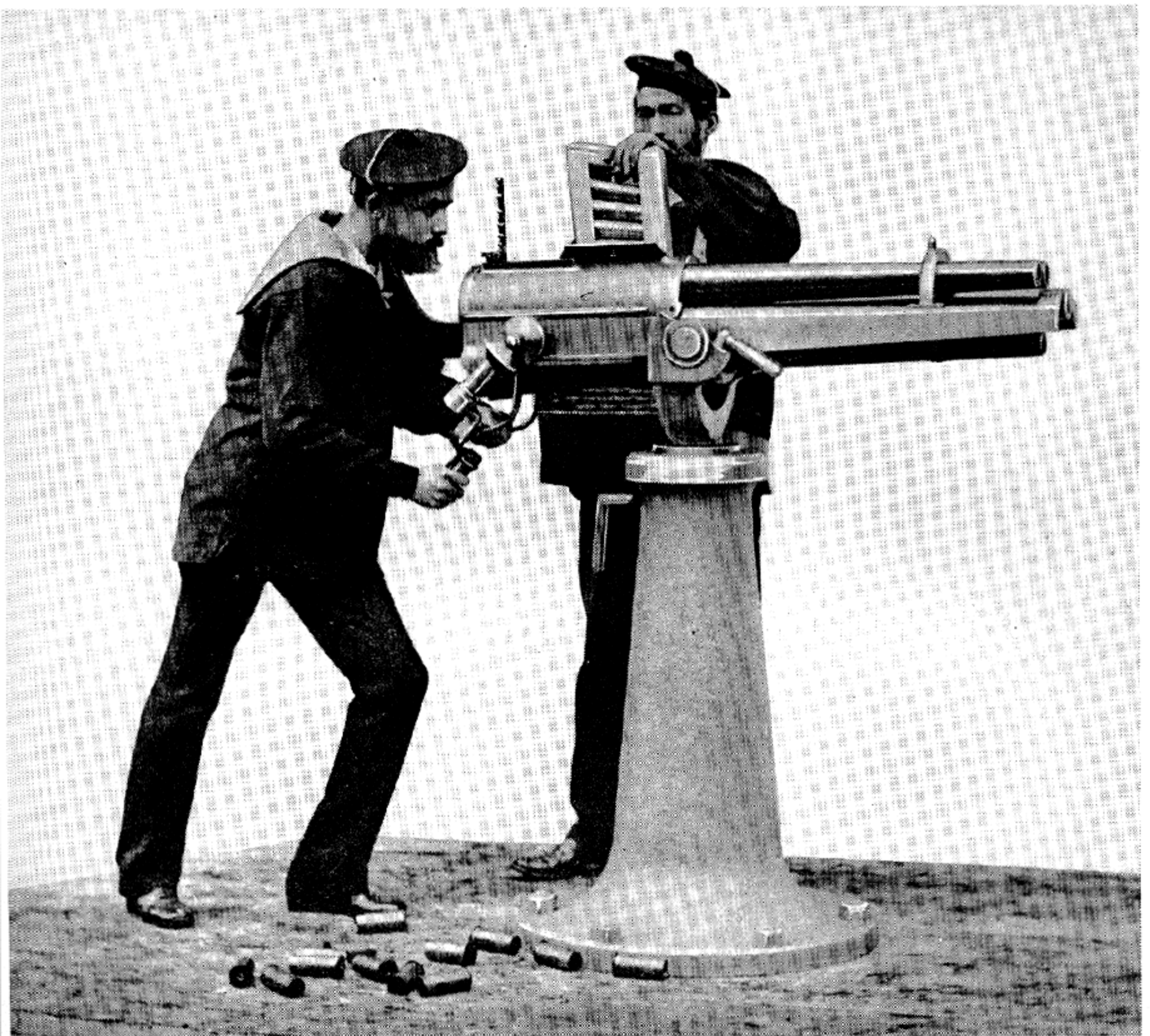
Hotchkiss 37-mm Revolving Cannon on Naval Deck Mount.
