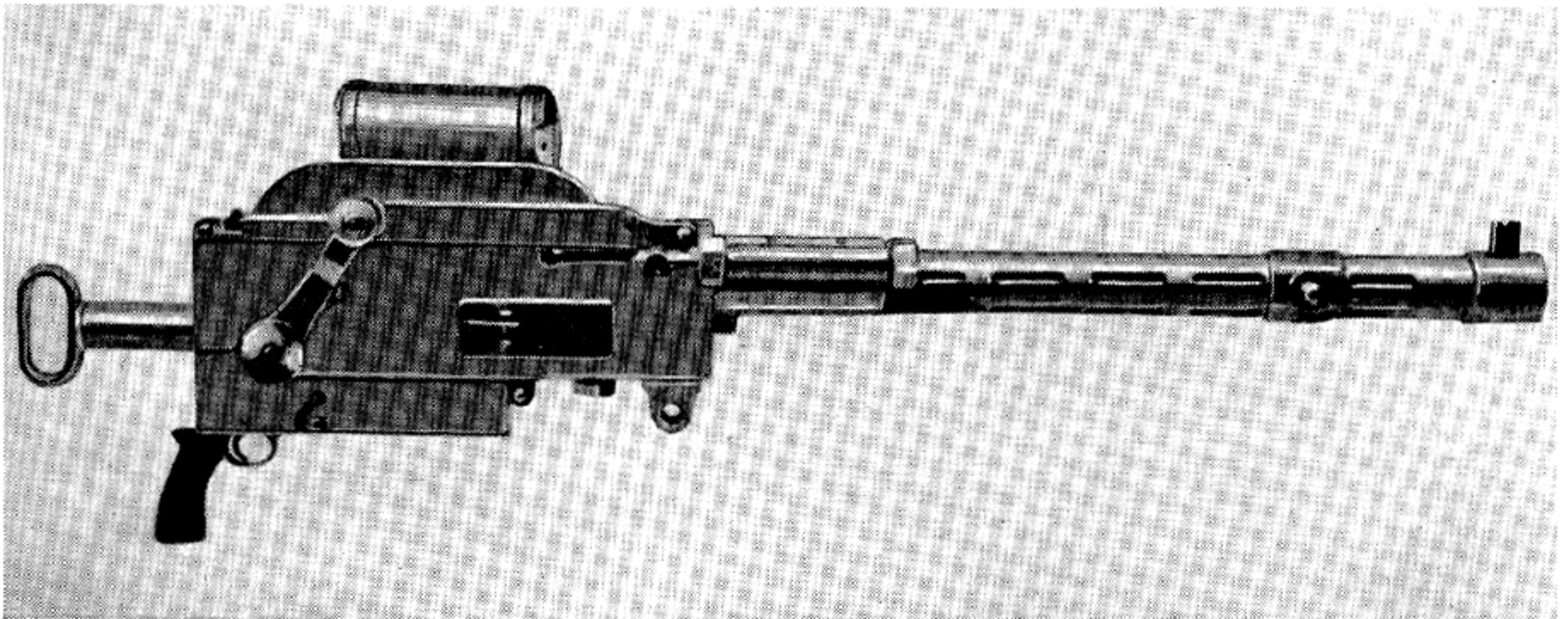
Madsen 20-mm Automatic Aircraft Cannon, Model 1926 (Prototype).
