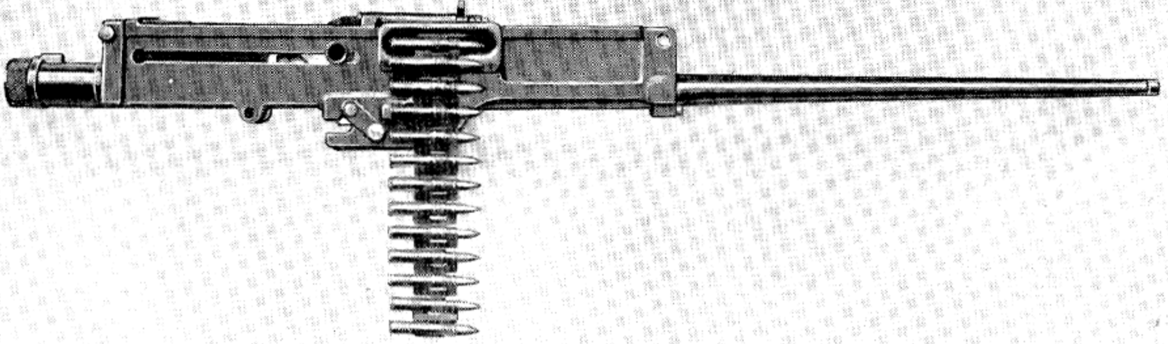
Fiat Aircraft Machine Gun, Model 1928 A, 7.7 mm
