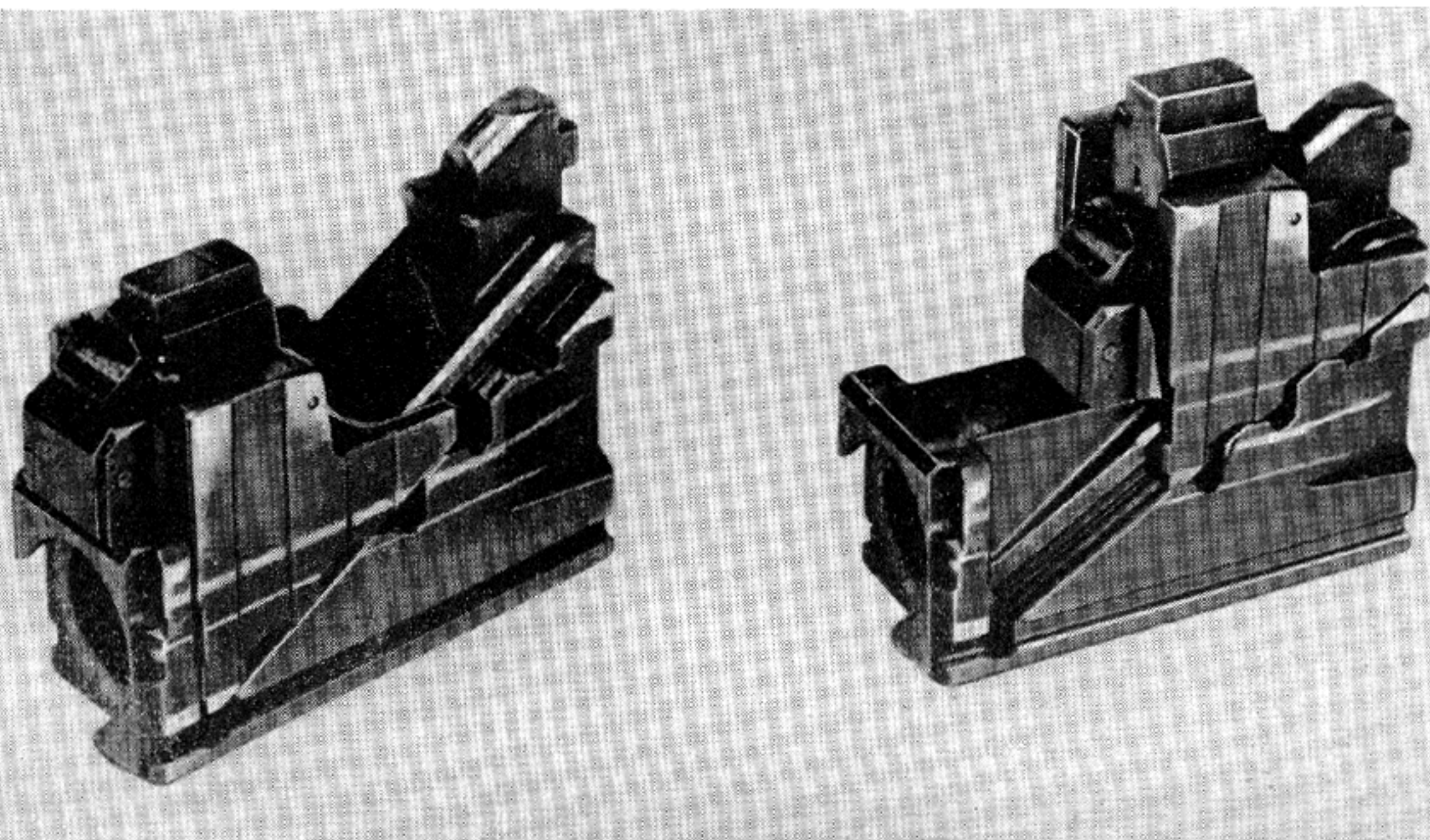
Bolt Assembly of the Breda 20-mm Automatic Cannon. Left: Bolt in Traveling Position. Right: Bolt Locked in Battery Position.
