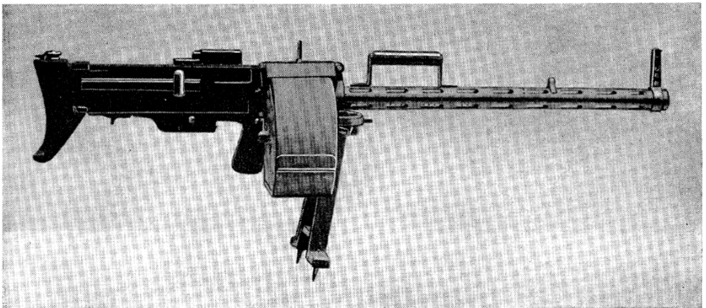
Bergmann Machine Gun, Model 1915, N. A., 7.92 mm.
