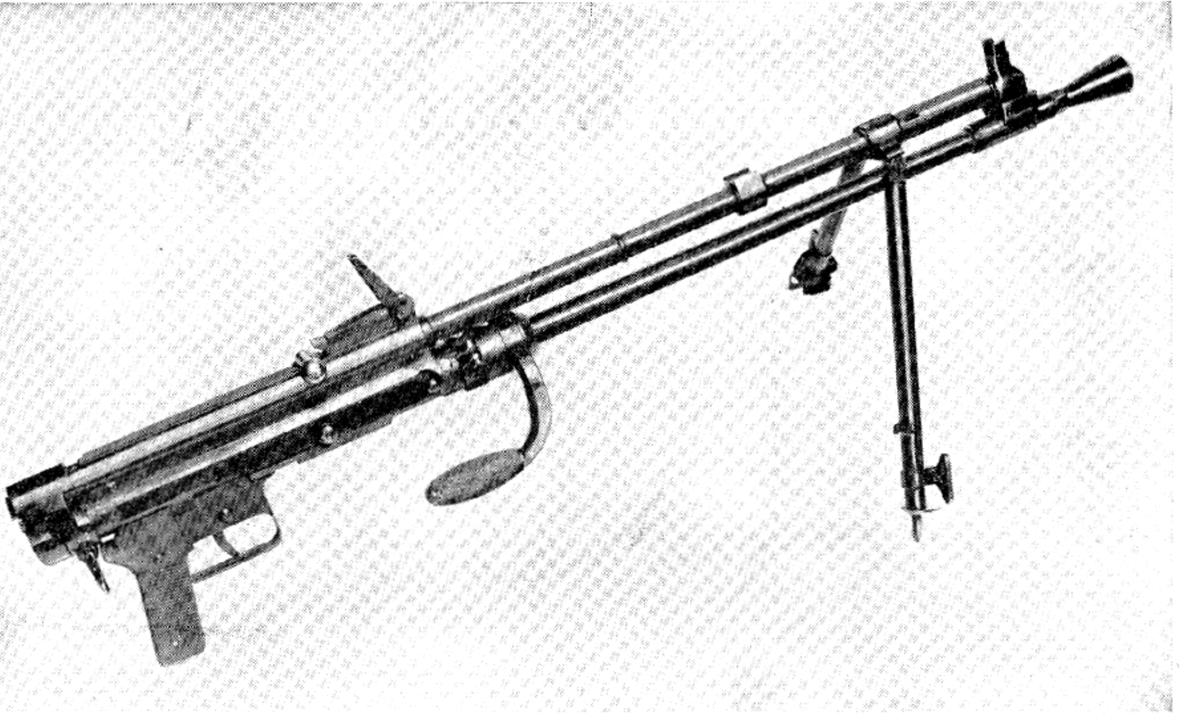
Knorr-Bremse Machine Gun, Model 35/36, 7.92 mm.
