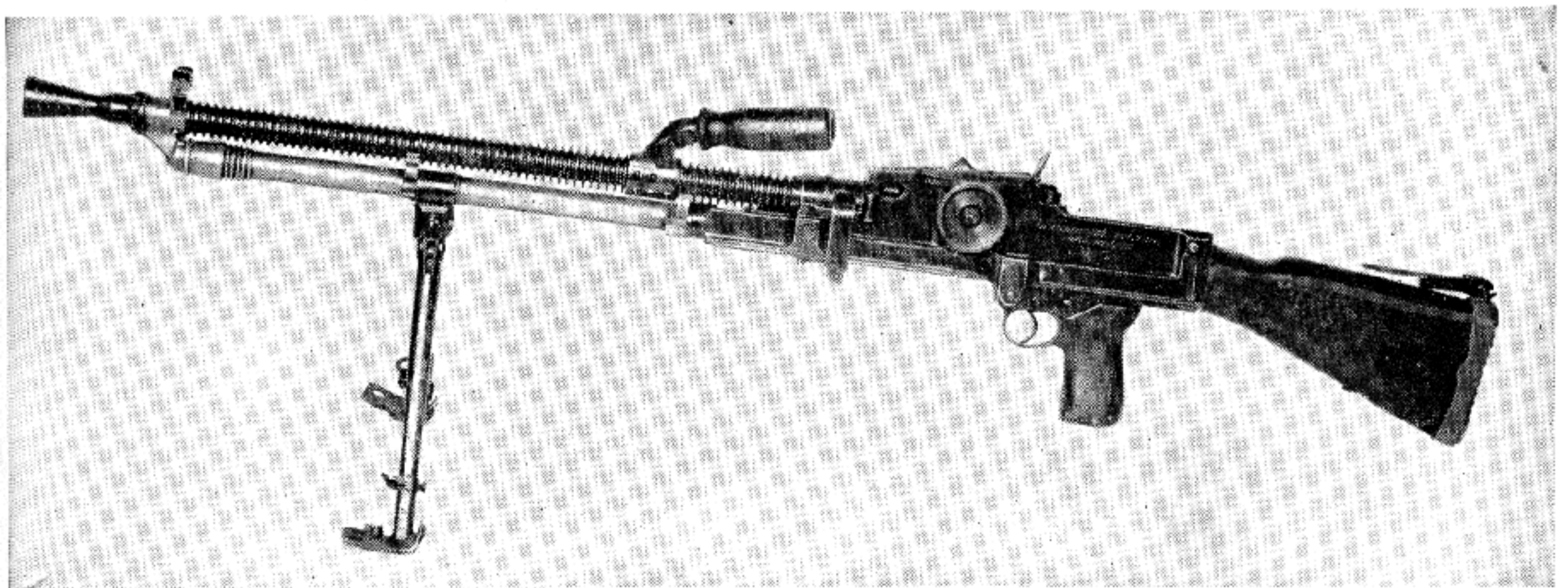
ZB Machine Gun, Model 1925, 7.92 mm.
