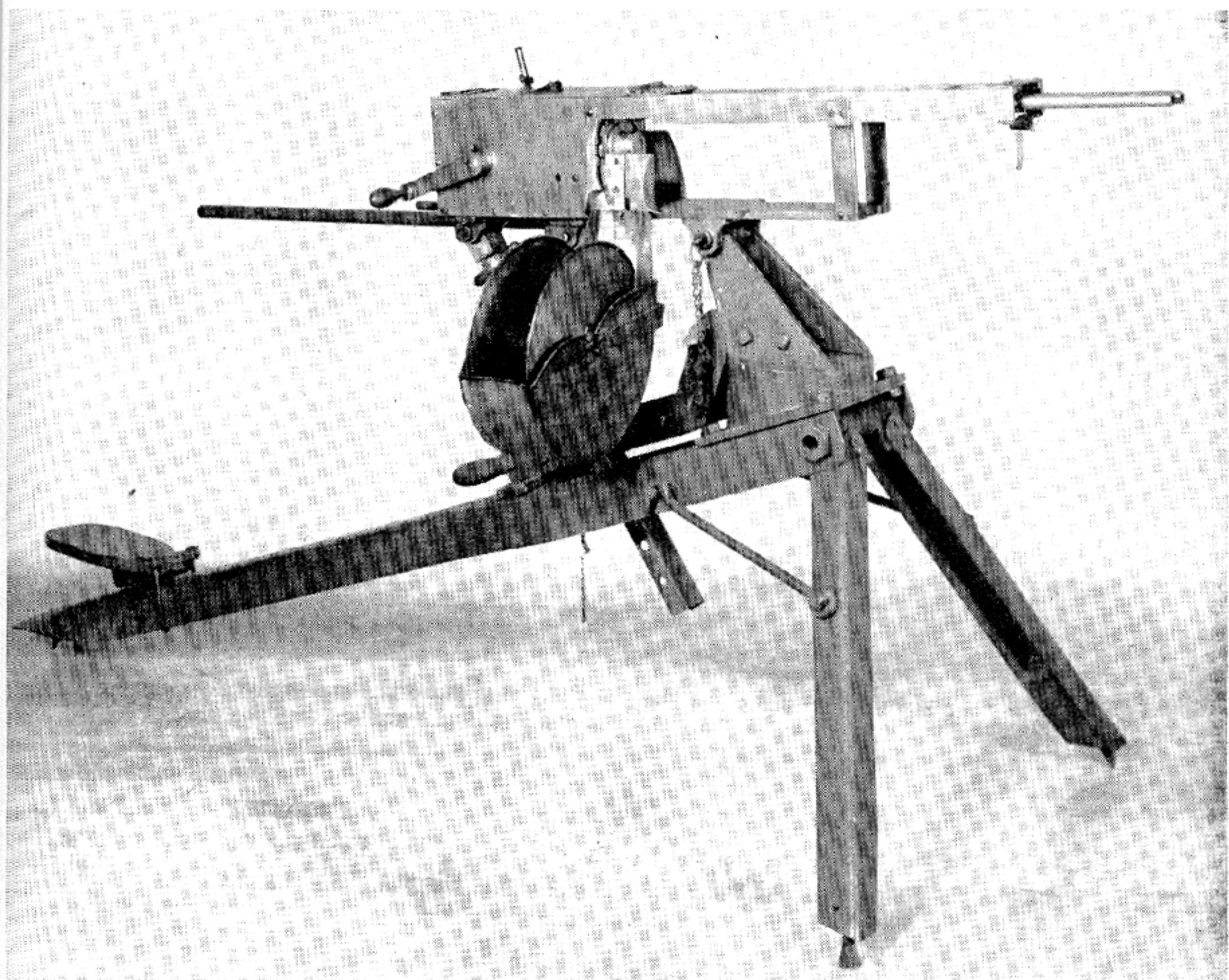
Robertson Double-Barrel Machine Gun, Cal. .30.
