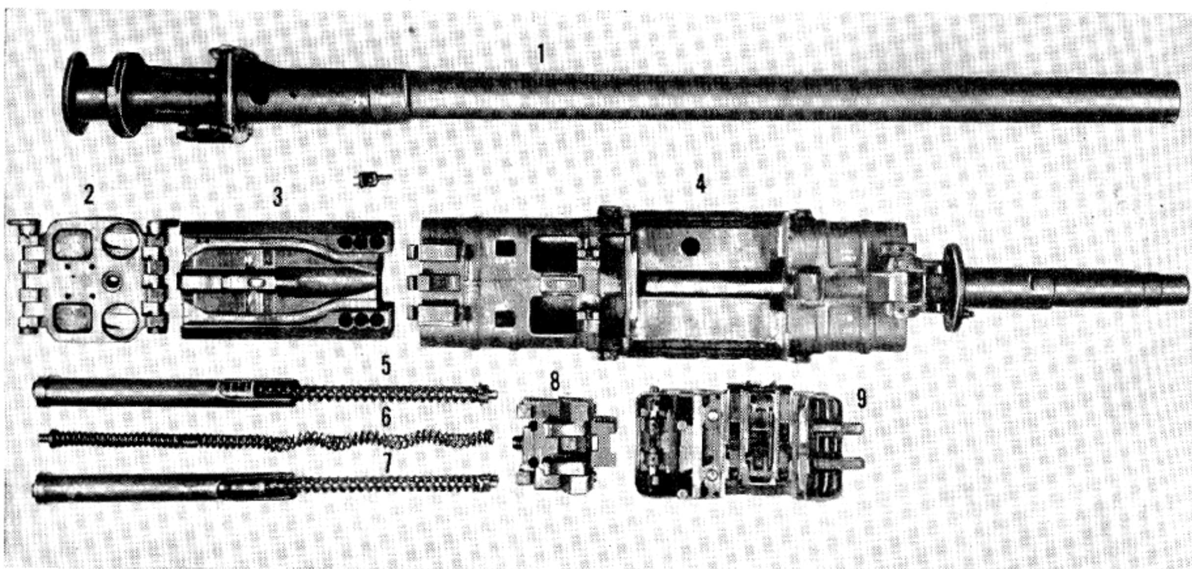
Rheinmetall 30-mm Automatic Aircraft Cannon, MK-108, Disassembled. (1) Blast Tube. (2) Back Plate Assembly. (3) Bolt Assembly. (4) Receiver and Barrel Assembly. (5 and 7) Driving Spring Assembly. (6) Charger Spring Assembly. (8) Sear Plate Assembly. (9) Feed Cover Plate Assembly.
