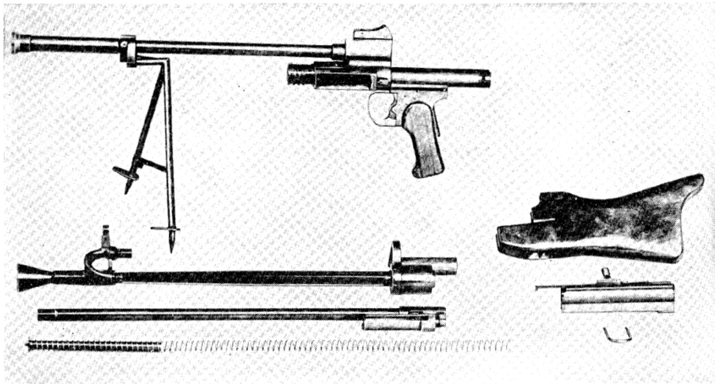
Components of the Knorr-Bremse Machine Gun, Model 1933.
