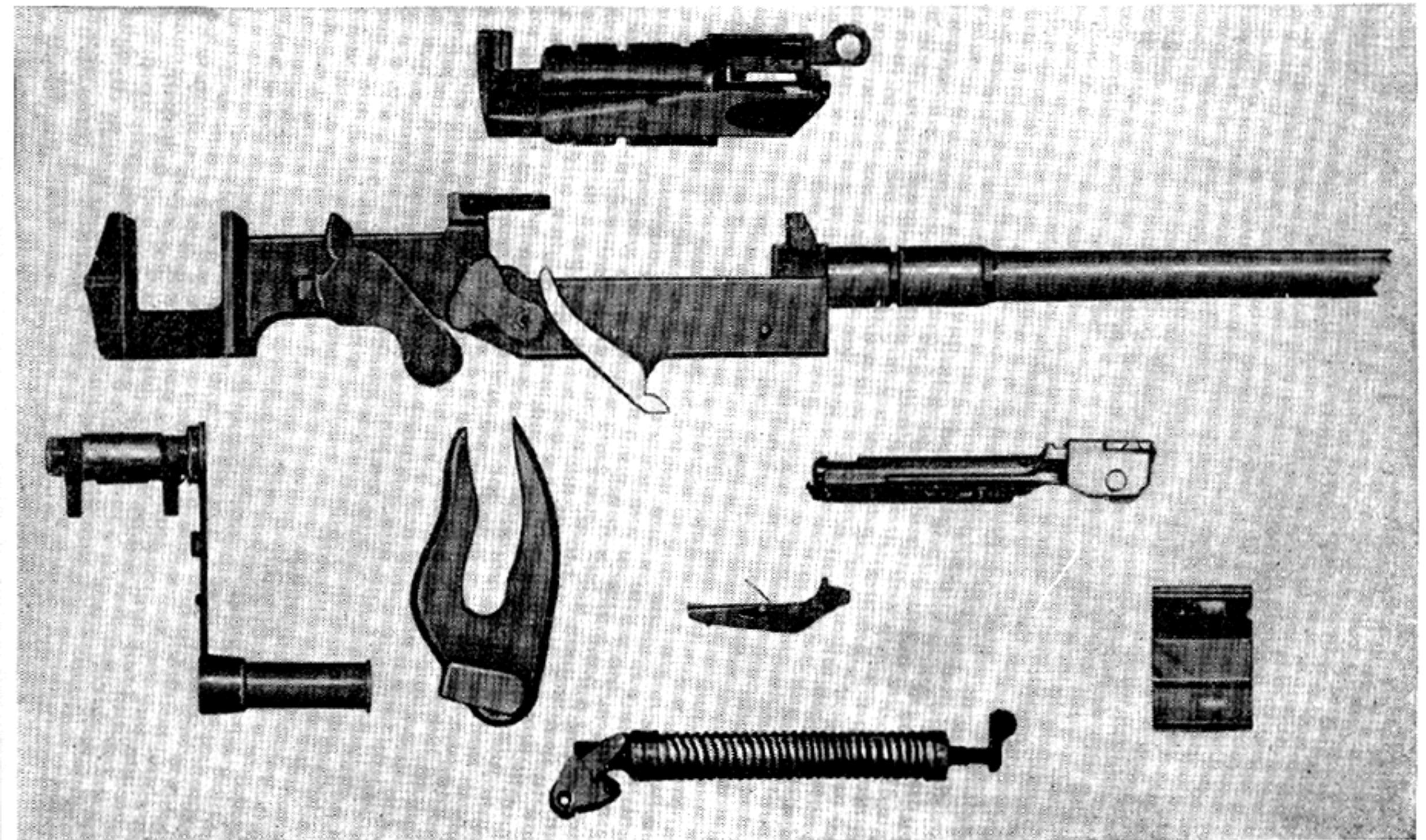
Components of the Nordenfelt Machine Gun.
