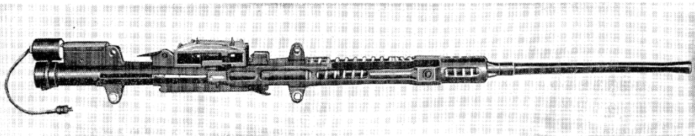
Oerlikon 20-mm Automatic Aircraft Cannon, Model 99 (Fixed). This Belt-Fed Weapon Was Manufactured in Japan and Used by Its Naval Air Force.
