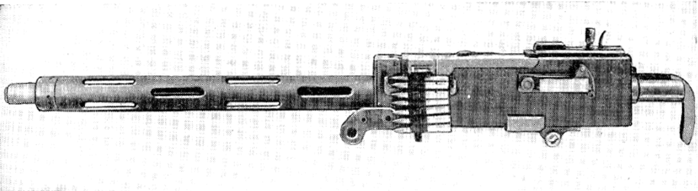
Browning Aircraft Machine Gun, Model 1918, M1, Cal. .30.
