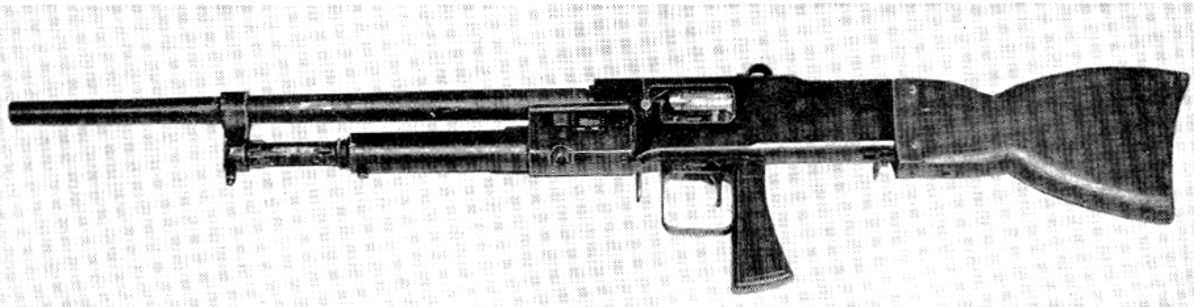
Darne Machine Gun, Model 1929, 7.5 mm.
