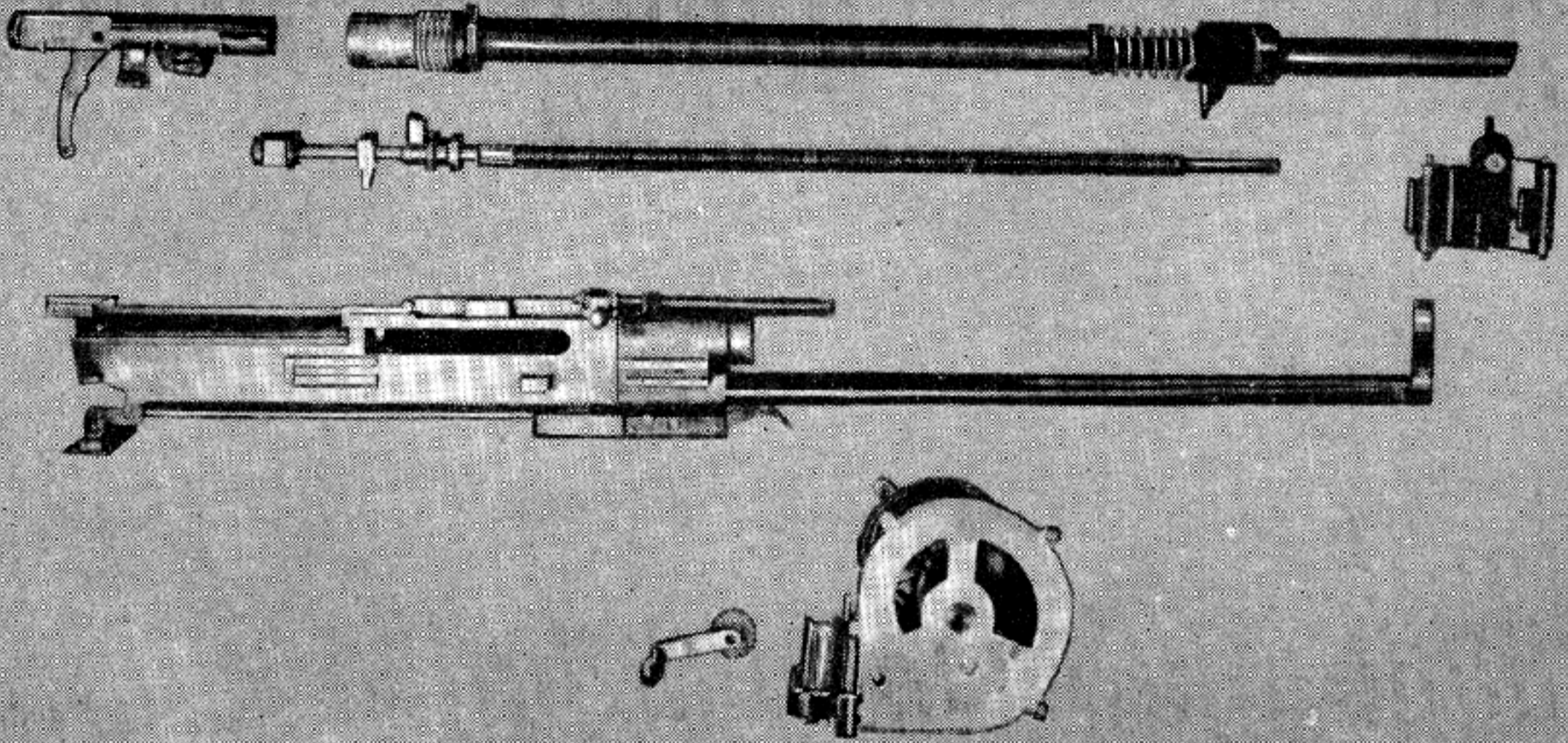
Lübbe 20-mm Automatic Aircraft Cannon Disassembled.
