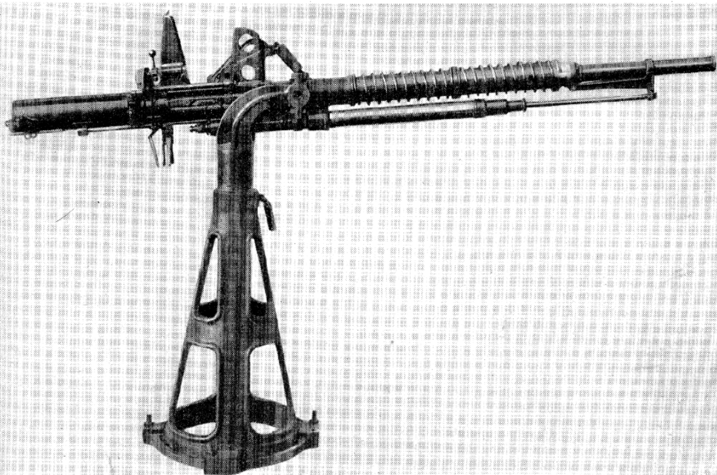
C. O. W. 37-mm Automatic Aircraft Cannon Mk III.
