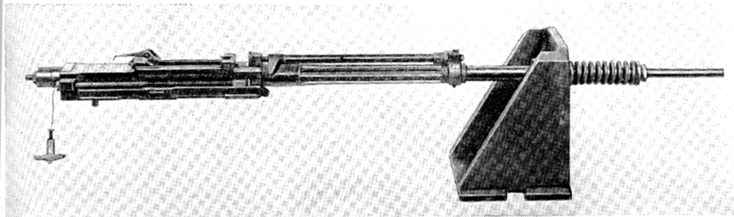
Hispano-Suiza 20/60 Automatic Aircraft Cannon. Experimental Model Manufactured by the British M.A.R. Company.
