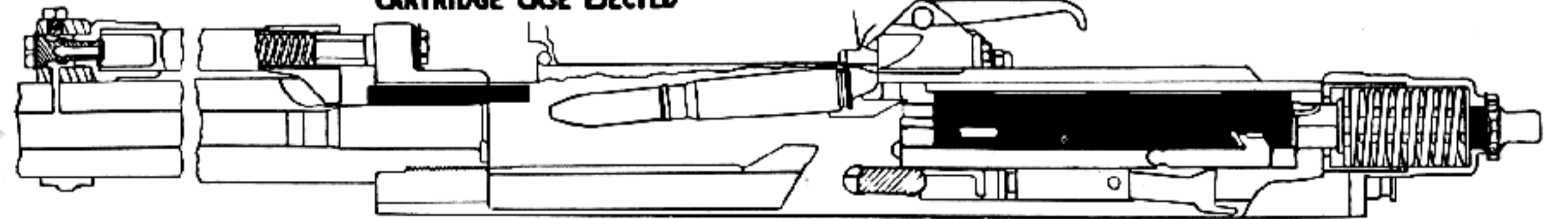
BREECH BLOCK FULLY RECOILED, BUFFER SPRING COMPRESSED
