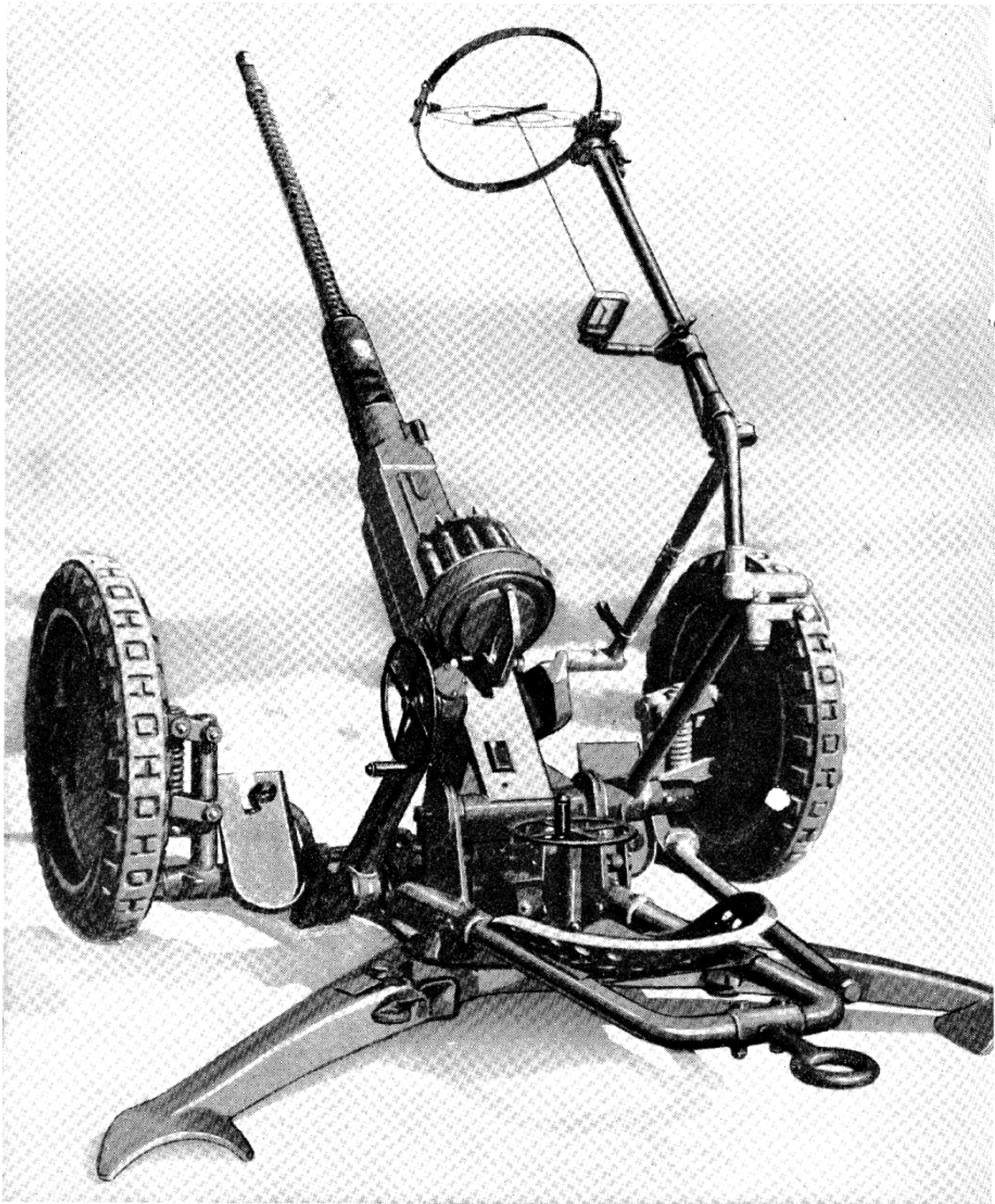
Bofors 20-mm Automatic Cannon, Model L/70, on a Field Carriage.
