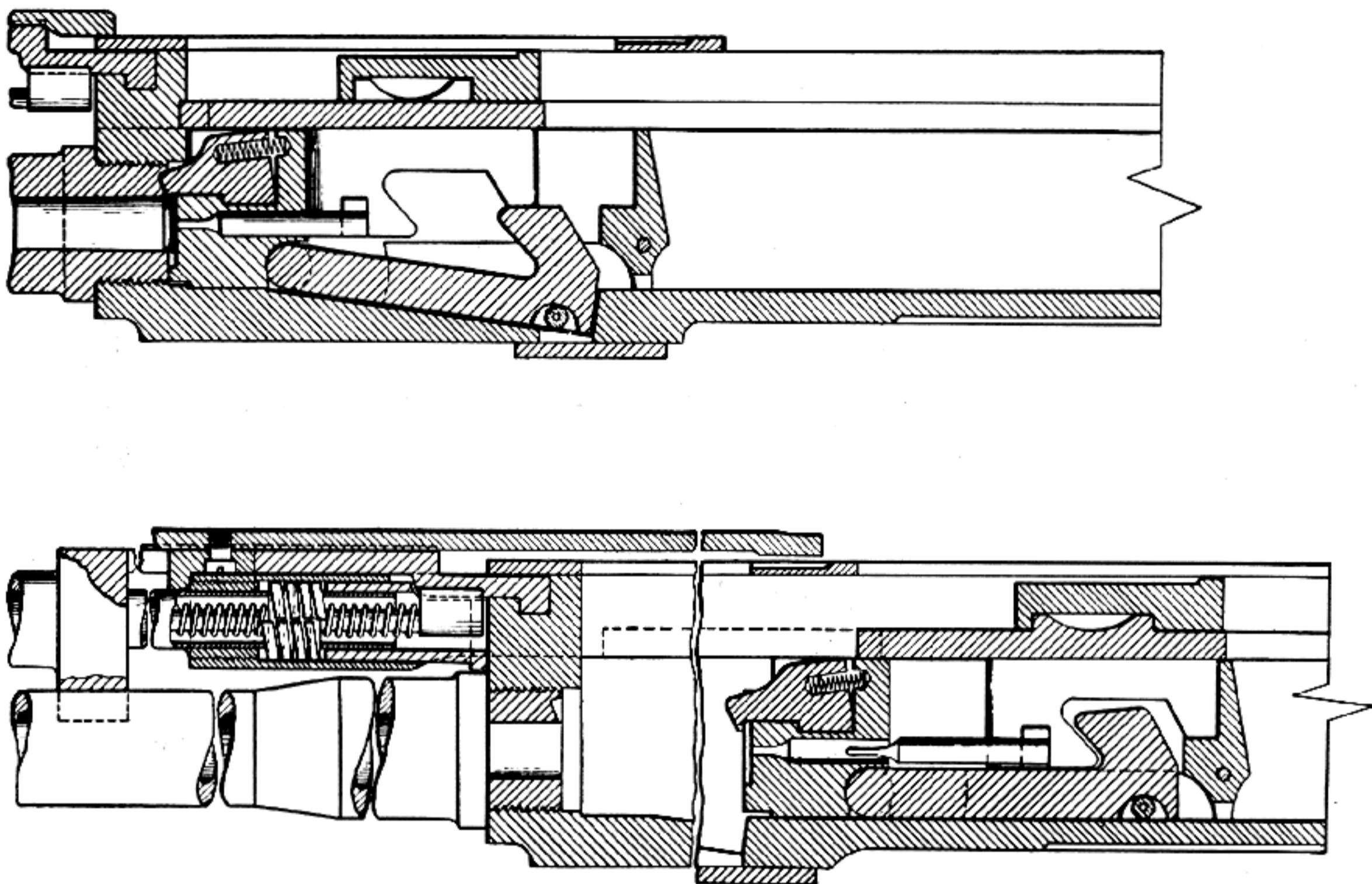
The Method of Locking Patented by Carl Swabilus.
