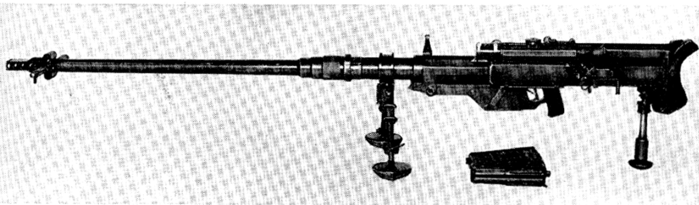
Rheinmetall (Solothurn) 20-mm Semi-Automatic Antitank Cannon, Model S18-1000.
