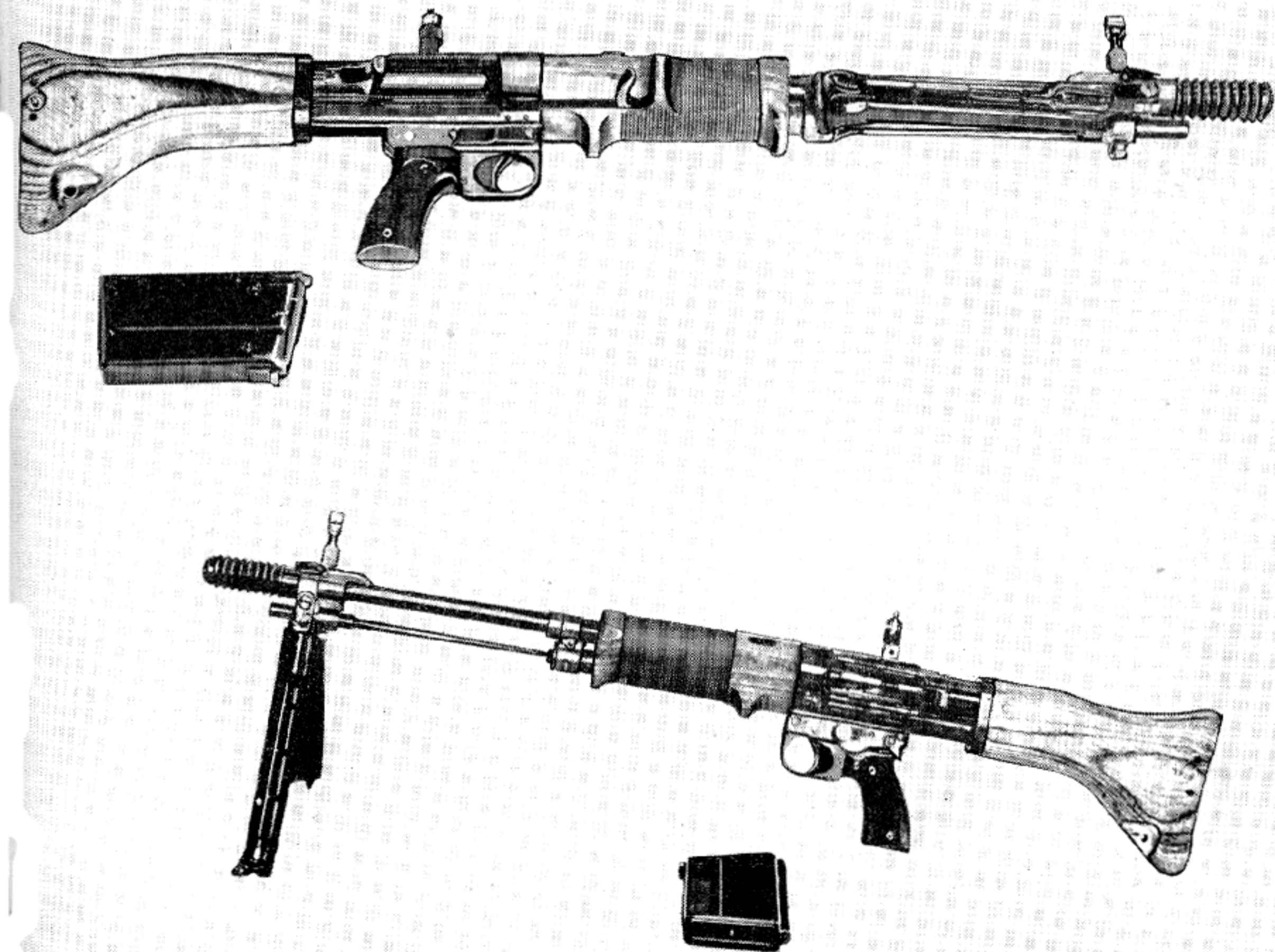
Machine Gun, Model FG-42, 7.92 mm.
