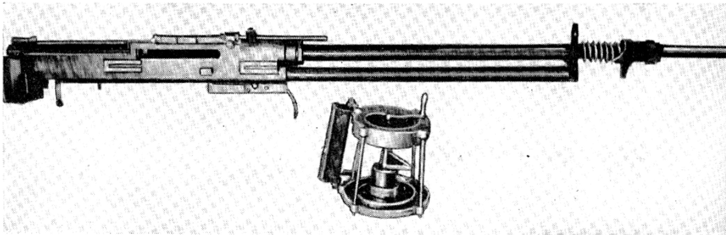
Lübbe 20-mm Automatic Aircraft Cannon and Feeder.
