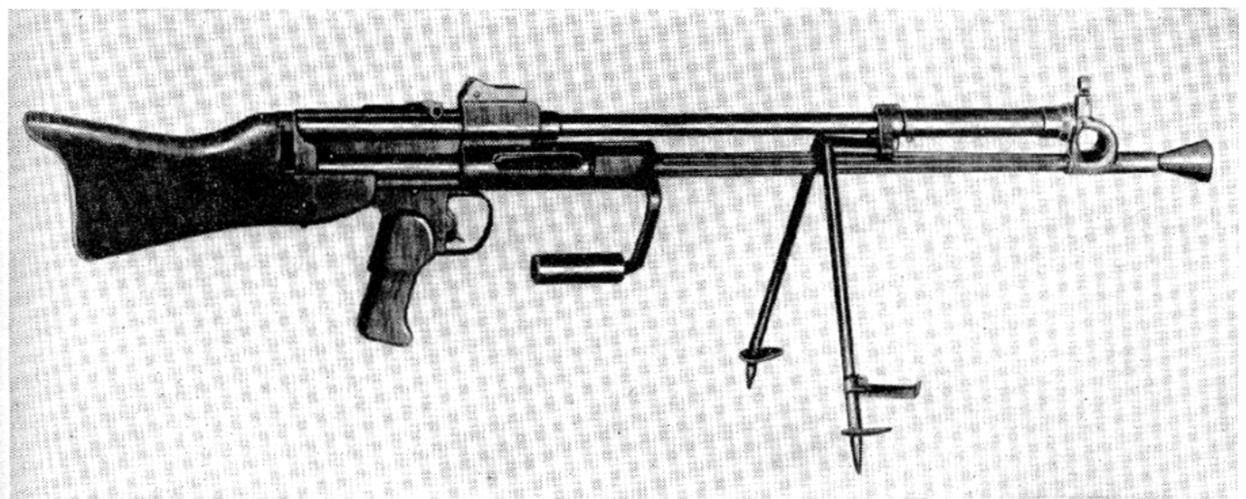
Knorr-Bremse Machine Gun, Model 1933, 7.92 mm.
