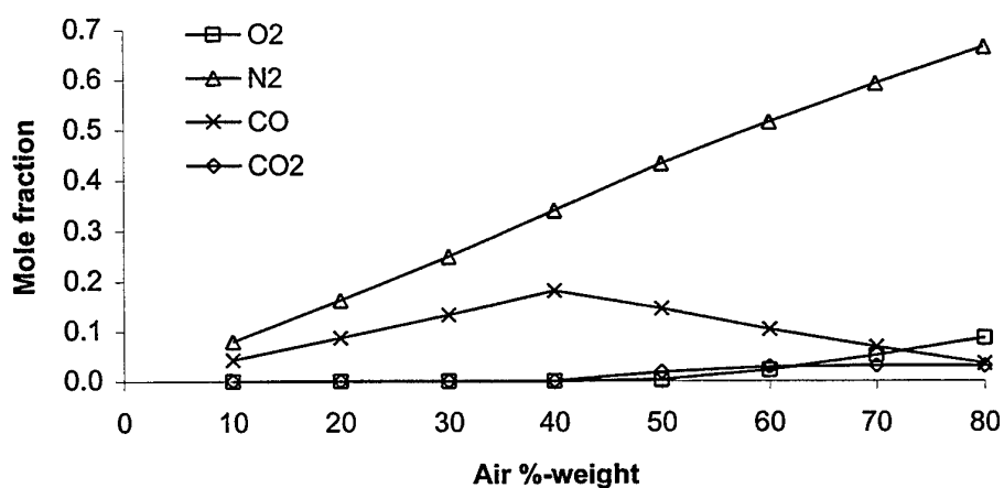
Figure 12: CO, O 2 , CO 2 and N 2 profiles of MTV-air combustion.
