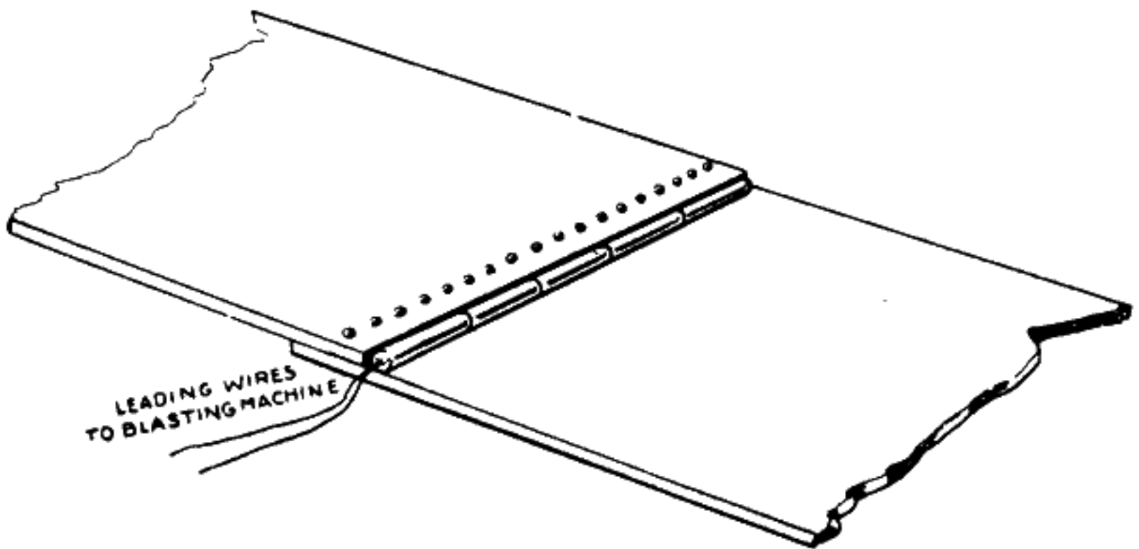
Fig. 105.—By stringing cartridges along the seams and covering with mud the plates can be easily sheared. Sometimes the cartridges can be split lengthwise into halves or quarters for light plates.
