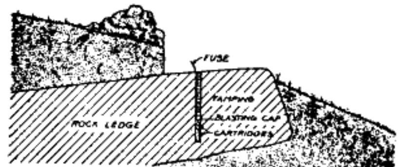
Fig. 116.—Correct method of loading the out-crop of a rock ledge.
