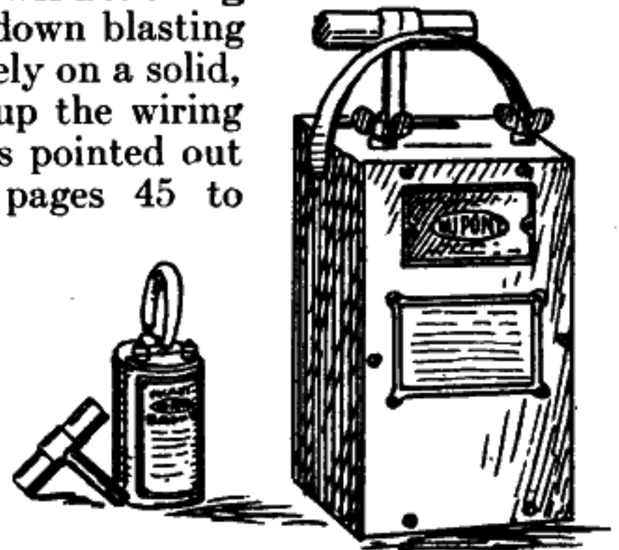
Fig. 61.—Showing the two types of Blasting Machines.
