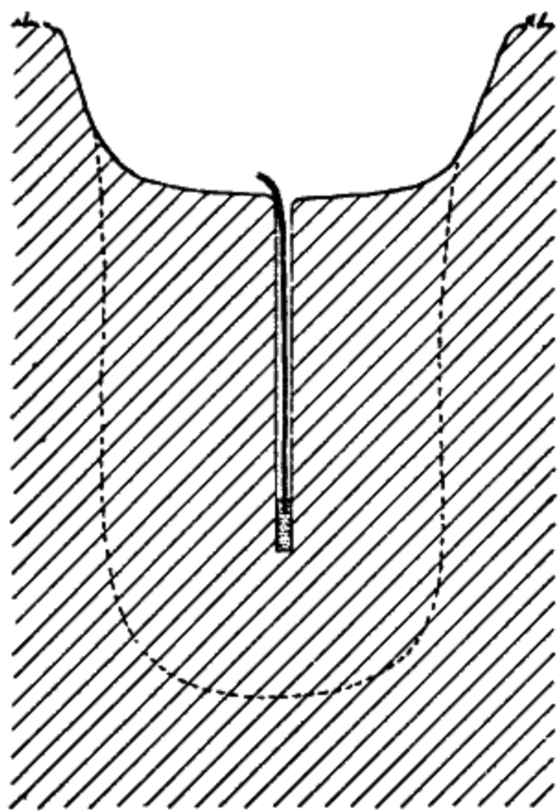
Fig. 99.—Method of loading to blast a shallow pole or post hole. The object is to loosen the soil so that it can be easily shoveled.
