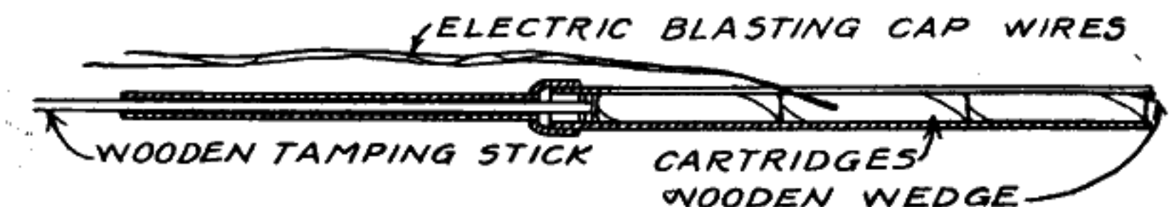
Fig. 163.—Showing section of a loading tube for loading holes under water
