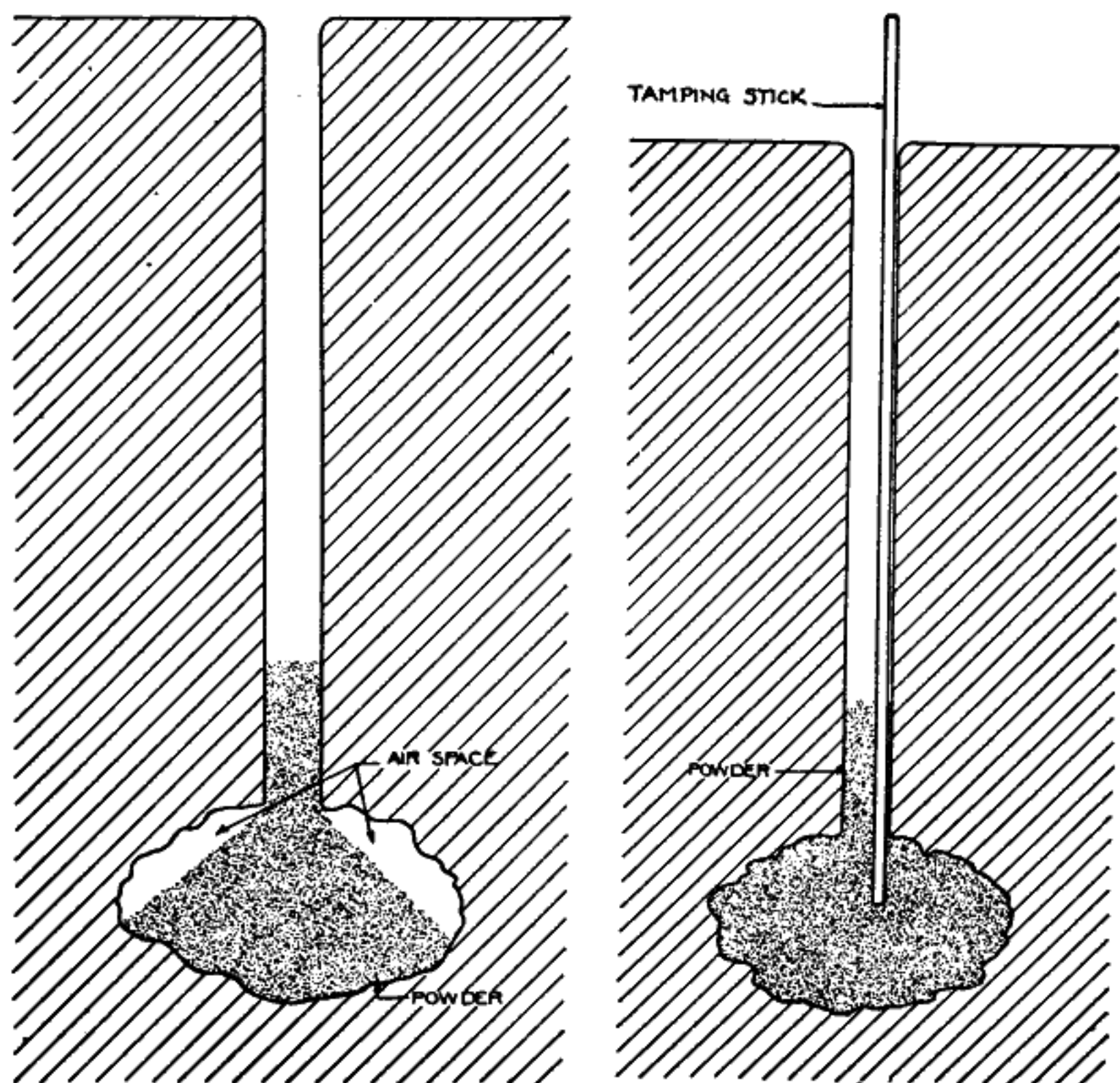
Vertical bore hole chambered and showing powder filled to top of chamber and not spread out, leaving an air pocket.
