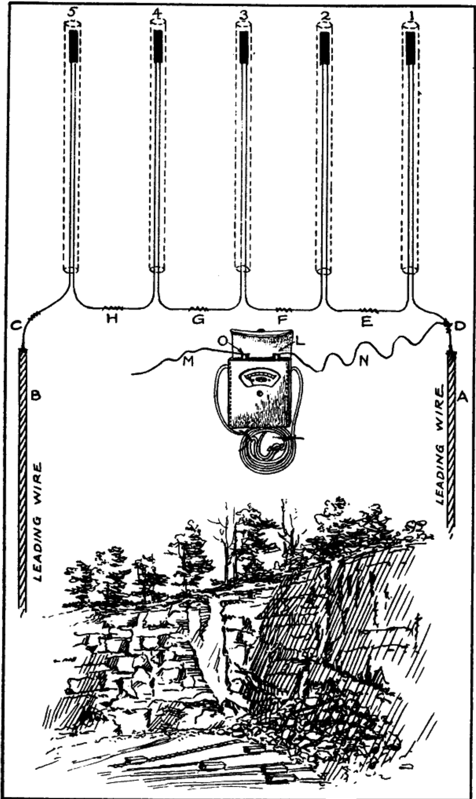
Fig. 59.—Diagram showing method of locating a break with a du Pont Galvanometer.
