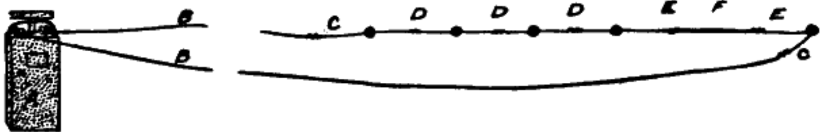
Fig. 47.—Series connections. A. Blasting machine. B. The two strands of single leading wire. C. Connections between leading wire and electric blasting cap wires. D. Connections between electric blasting cap wires. E. Connections between electric blasting cap wires and a short piece of connecting wire F, used to connect electric blasting cap wires that are too short to reach from hole to hole. This may be left out when long electric blasting cap wires are used, or it may be used between all holes in some cases.
