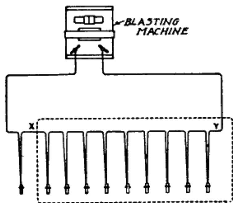
Fig. 64.—Testing a Blasting Machine without a Rheostat.
