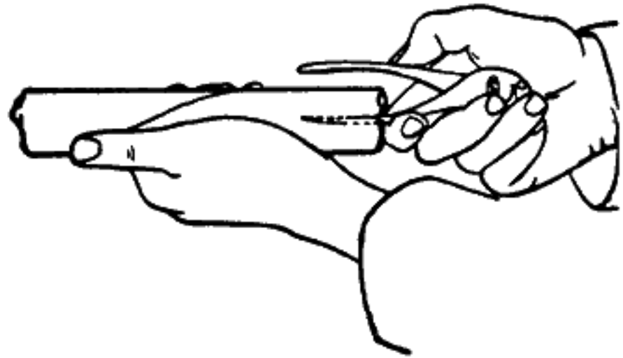
Fig. 34.—Punch hole with handle of cap crimper.
