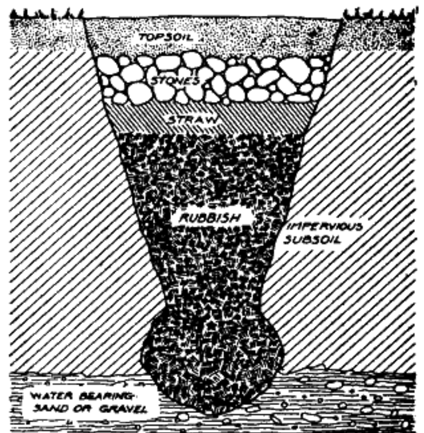
Fig. 151.—Diagram of deep drainage hole, showing the use of trash to prevent the hole becoming clogged with fine clay.
