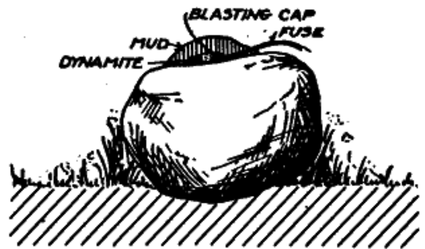
Fig. 120.—Correctly placed mud-cap. The mud covering should be several inches thick.
