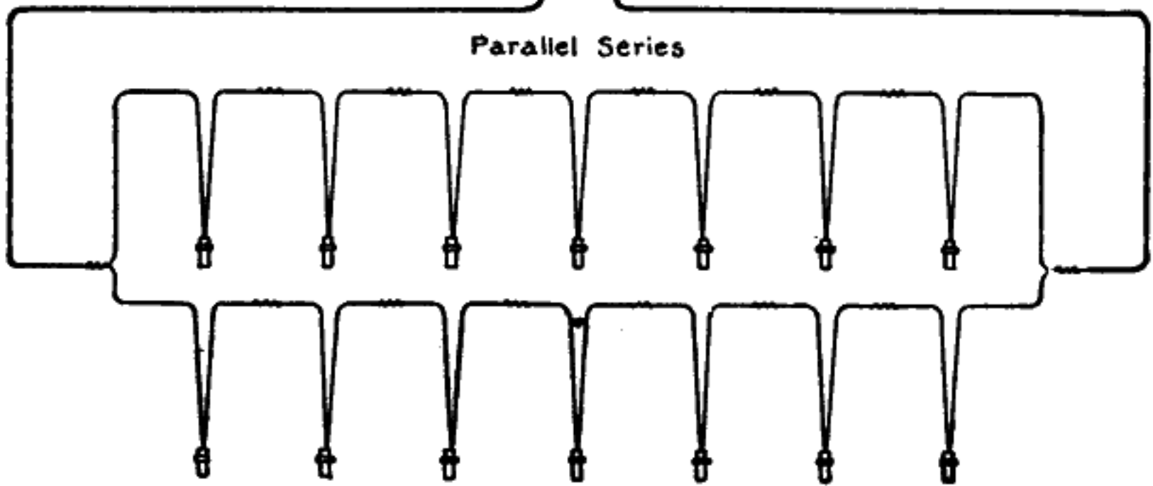
Fig. 57.—Another view of parallel series connections.
