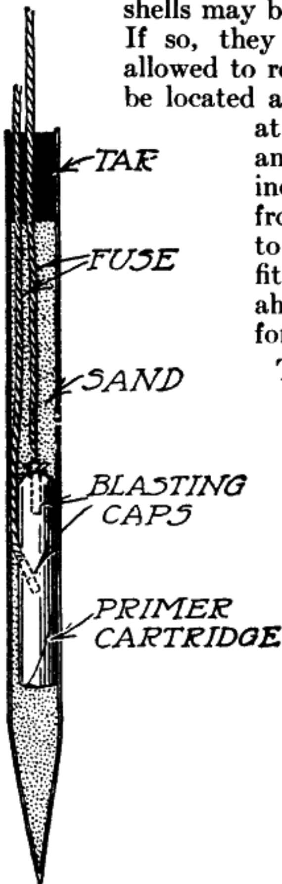
Fig. 140.—“Jack Squib” for exploding nitroglycerin container.
