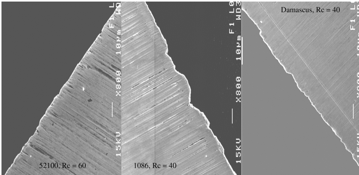
Figure 46 Face views of 3 non stainless steels. As-ground on 1000 grit TruHone wheels at 2\beta = 30 degrees. useful for the TruHone machine, 2\beta = 30 degrees. The face profiles of three blades sharpened at this angle are presented in Fig. 46. It is seen that the variation of edge roughness with hardness is similar to that shown in Fig. 45.
