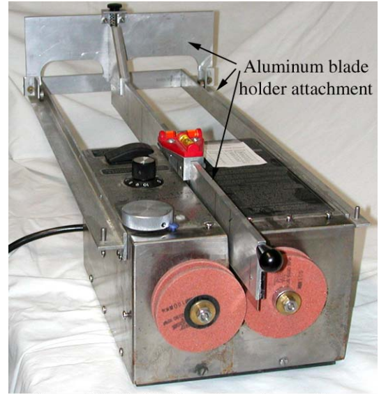
Figure A10 The TruHone sharpening machine with special attachment for grinding thin blades.
