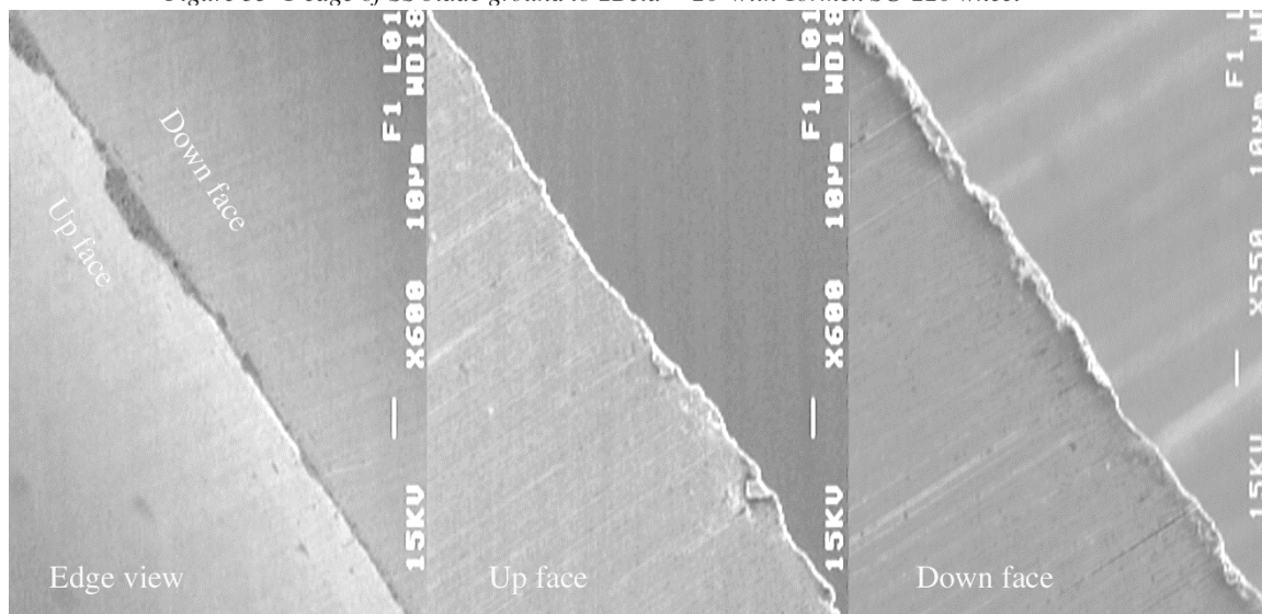
Figure 36 T edge of SS blade ground to 2\beta = 20^\circ with Tormek waterstone wheel.
