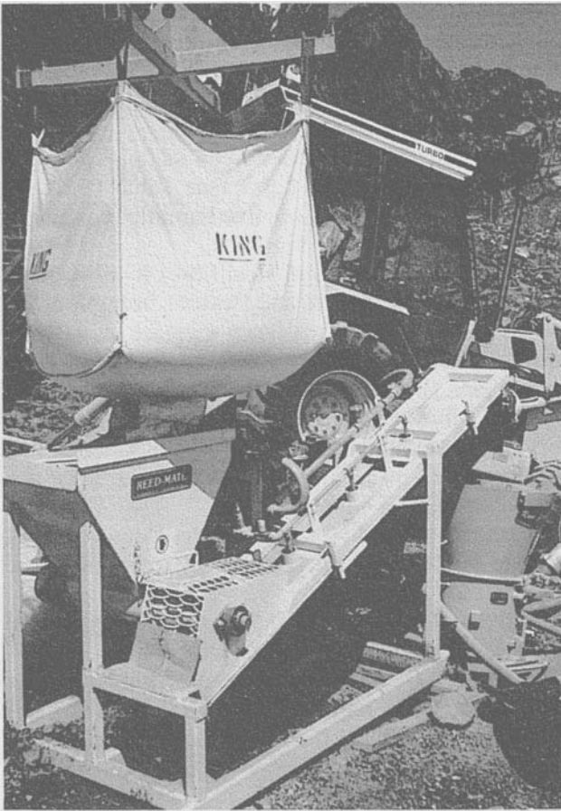
Figure 15.3: Bagged pre-mixed dry shotcrete components being delivered into a hopper feeding a screw conveyor, fitted with a pre-dampener, which discharges into the hopper of a shotcrete machine.
