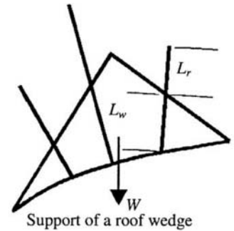
rockbolt capacity
