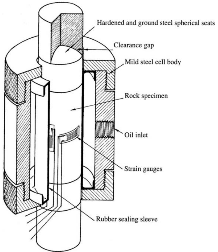
Figure 8.1: Simple triaxial cell used for testing rock cores in field laboratories. The rubber sealing sleeve is designed to retain the oil so that the cell does not need to be drained between tests. Cells are available to accommodate a variety of standard core sizes.
