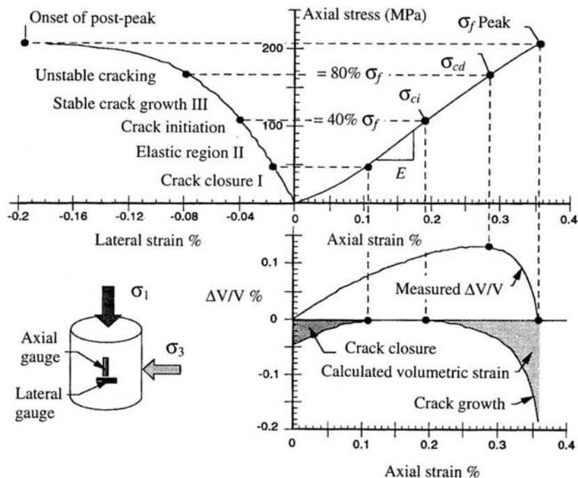
Figure 10.5: Typical stress/strain curves for Lac du Bonnet granite showing points defining peak strength, the onset of unstable crack growth and the onset of stable crack growth. After Martin (1993).
