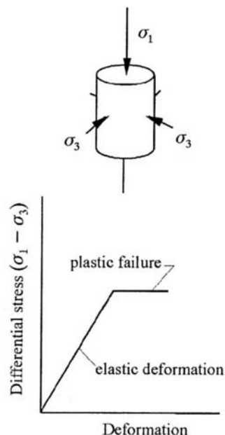
Stress-deformation curve for a constant confining pressure
