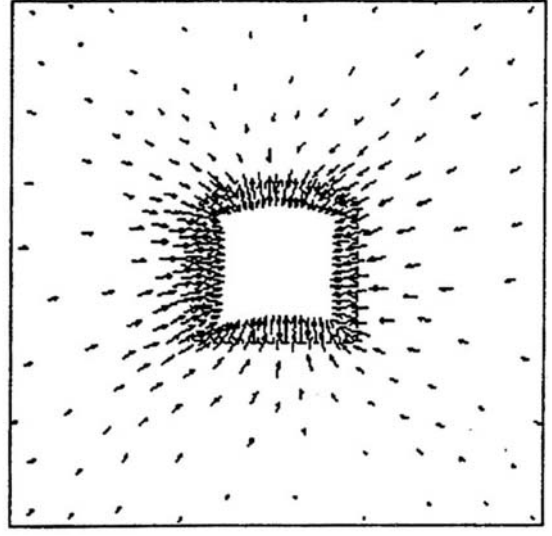
c) Displacements in the rock mass surrounding the unsupported tunnel. The maximum displacement in the roof is about 16 mm while the maximum floor heave is approximately 20 mm.
