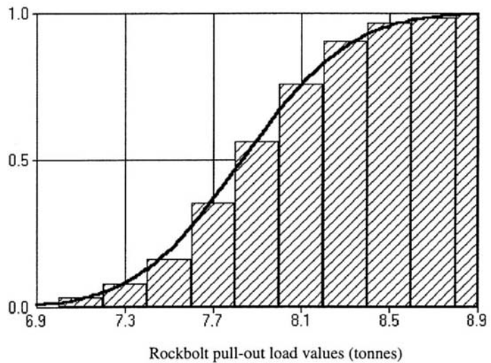
Figure 2.3: Hypothetical results from 62 pull-out tests on 17 mm diameter mechanically anchored rockbolts. The test results are plotted as histograms while fitted normal probability distributions are shown as continuous lines for a) a probability density function and b) a cumulative distribution function.
