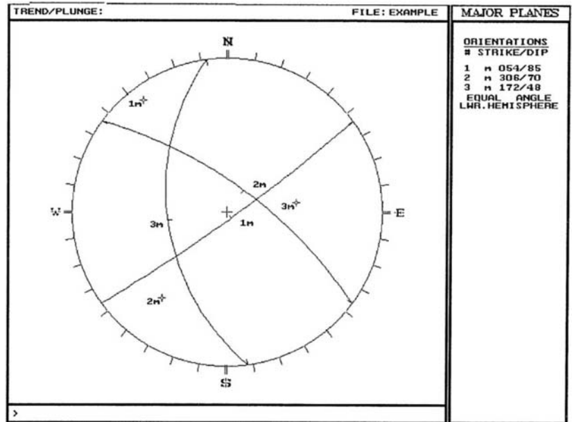
Figure 3.5: Poles and corresponding great circles for the average dip and dip direction of 3 discontinuity sets represented by the contour plot shown in Figure 3.4.
