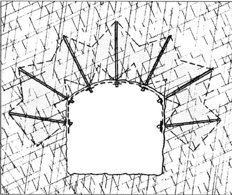
Figure 11.11: Pattern bolting for the support of heavily jointed rock which can fail by ravelling or squeezing. The shading represents a zone of compressive stress in which interlocking of individual rock pieces is retained and a self-supporting arch is created. Mesh or shotcrete should be applied to the excavation surface to retain small blocks and wedges in the stress-free zones between the rockbolts.
