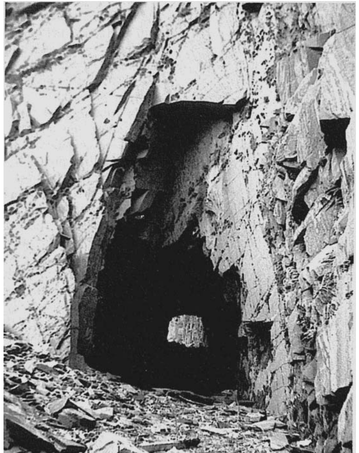
Figure 11.10: Structurally controlled failures in an old slate quarry in Wales. No support was installed in this tunnel and the final profile is defined by the wedges which have fallen from the surrounding rock mass.
