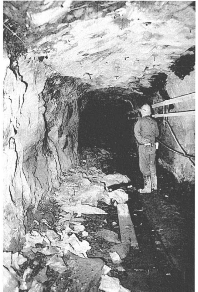
Figure 10.2: Spalling of one wall of a drive in quartzite at a depth of about 1,500 m in a uranium mine. In this case, an open stope on the left of the picture caused the stresses in the left-hand wall of the drift to be high enough to initiate spalling. This spalling is relatively minor and is parallel to the drift wall.
