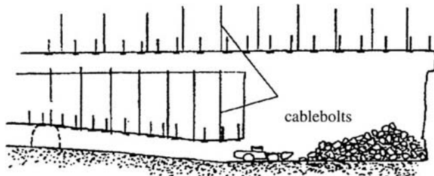
Figure 11.17: Use of cablebolts to control roof failure in bench cut and fill stope in the Kotalahti mine in Finland. After Lappalainen et al. (1984).
