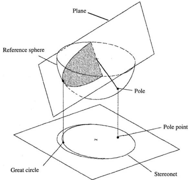
Figure 3.2: Definition of a great circle and pole.
