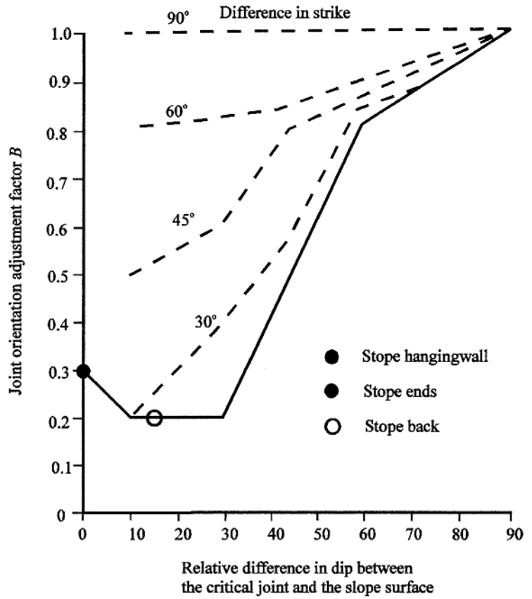
Figure 14.9: The correction factor B for the example mine.
