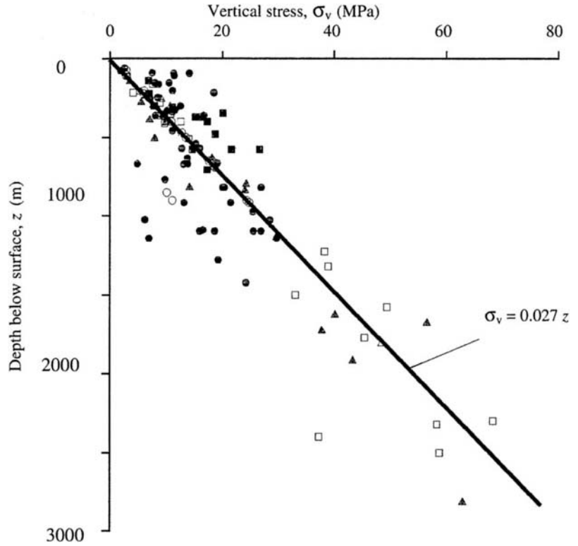
Figure 7.1: Vertical stress measurements from mining and civil engineering projects around the world (after Brown and Hoek, 1978).
