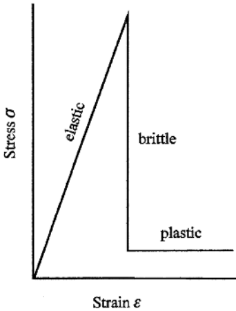
Elastic-brittle-plastic behaviour assumed for massive brittle rock
