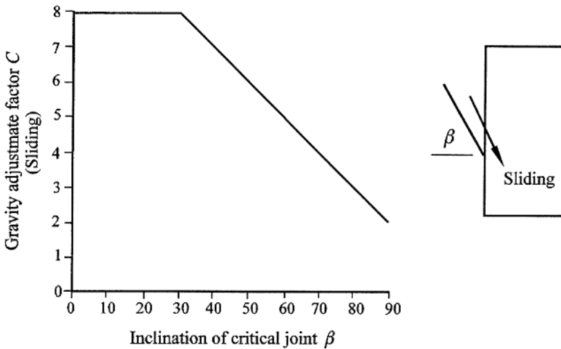
Figure 14.5: Gravity adjustment factor C for sliding failure modes. After Potvin (1988).
