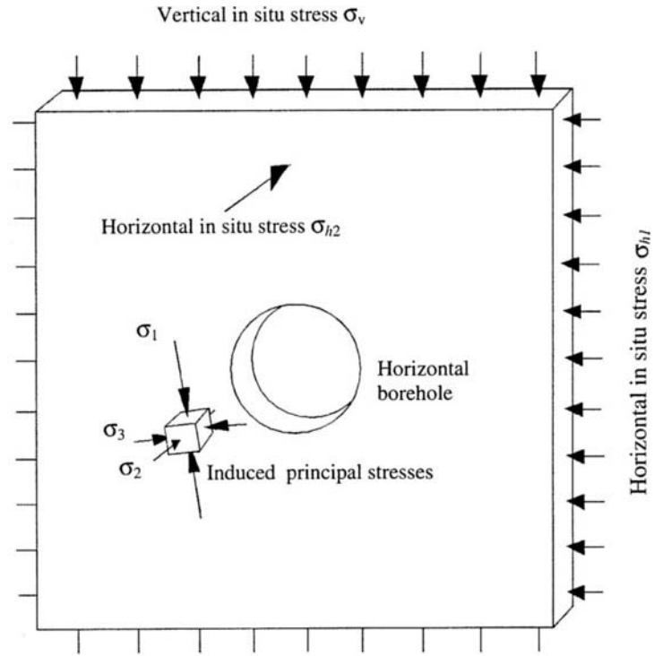
Figure 7.5: Illustration of principal stresses \sigma_1 , \sigma_2 and \sigma_3 induced in an element of rock close to a horizontal borehole subjected to a vertical in situ stress \sigma_v , a horizontal in situ stress \sigma_{h1} in a plane normal to the borehole axis and a horizontal in situ stress \sigma_{h2} parallel to the borehole axis.
