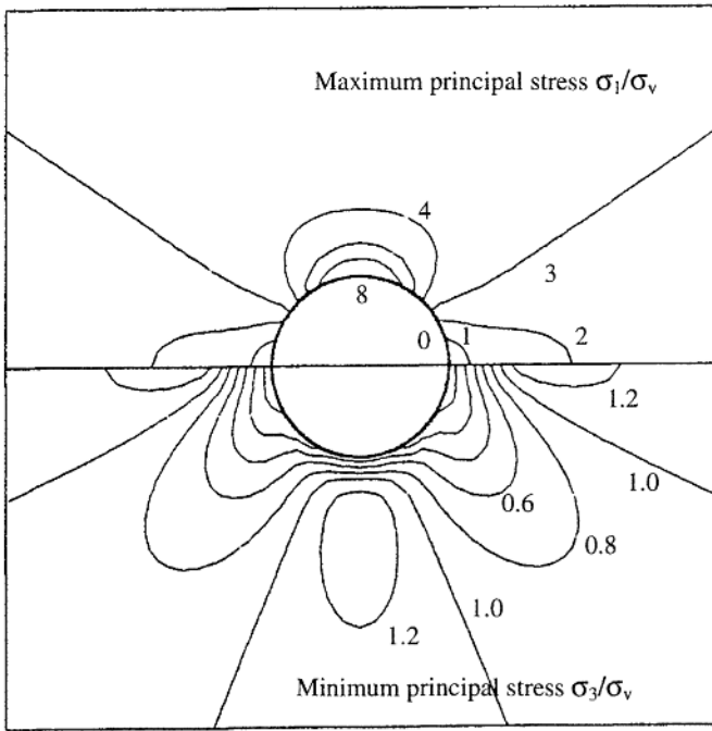
Figure 7.7: Contours of maximum and minimum principal stress magnitudes in the rock surrounding a horizontal borehole, subjected to a vertical in situ stress of \sigma_v and a horizontal in situ stress of 3\sigma_v .
