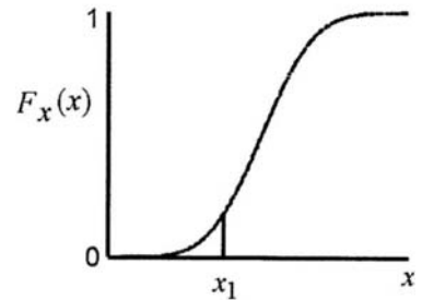
Cumulative distribution function (CDF)
