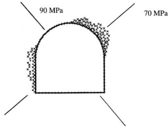
Figure 10.15: Failure zones predicted by PHASES for the second tunnel example.
