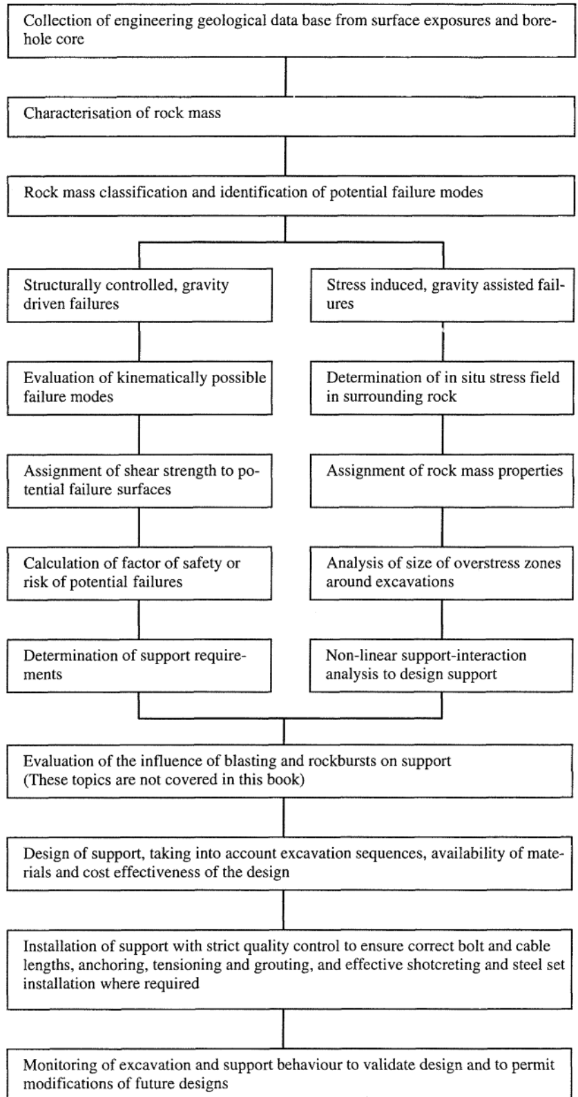
Figure 1.2: Steps involved in support design for underground excavations in hard rock.
