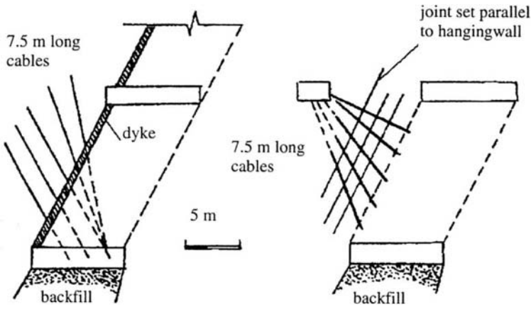
Figure 11.26: Hangingwall support for a longhole stope by means of cables placed from inside a stope and from a bypass drift at the Campbell mine. After Bouchier et al.(1992).
