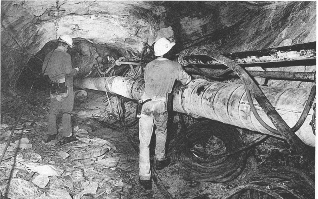
Figure 10.11: Overbreak resulting from spalling in a tunnel in massive quartzite at a depth of 3250 m below surface in the East Rand Proprietary Mine (ERPM) in South Africa. Photograph provided by Mr David Ortlepp.
