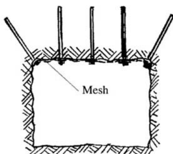
a) Conventional rectangular excavation
