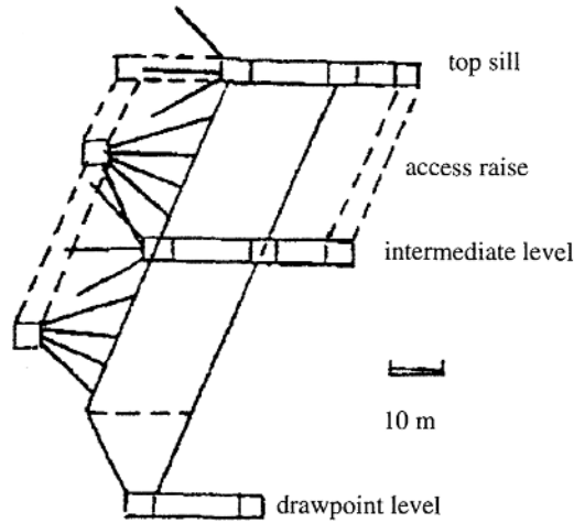
Figure 11.24: Cable patterns from specially driven access and from hangingwall drilling access. After Fuller (1984).
