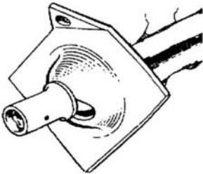
Domed faceplate used by Stillborg in test on EXL Swellex dowel.
