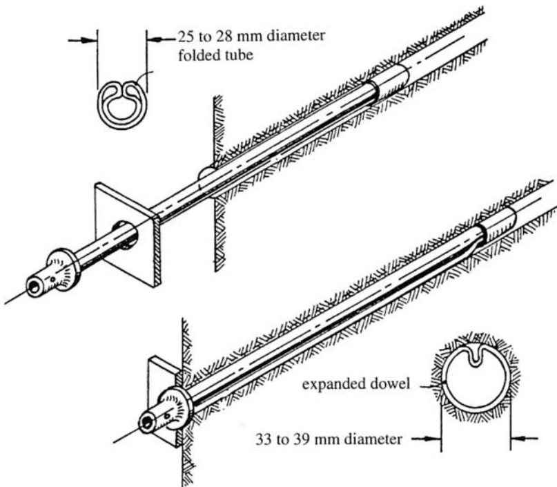
Figure 12.9: Atlas Copco Swellex dowel.
