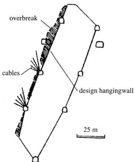
Figure 11.23: Hangingwall overbreak in the J704 stope at the Mount Isa mine. After Bywater and Fuller (1984).
