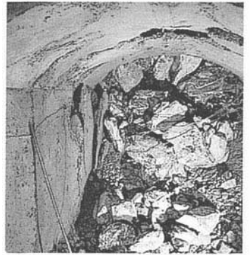
Attempting to reinforce a drawpoint with concrete or steel sets after failure has started is unlikely to be successful
