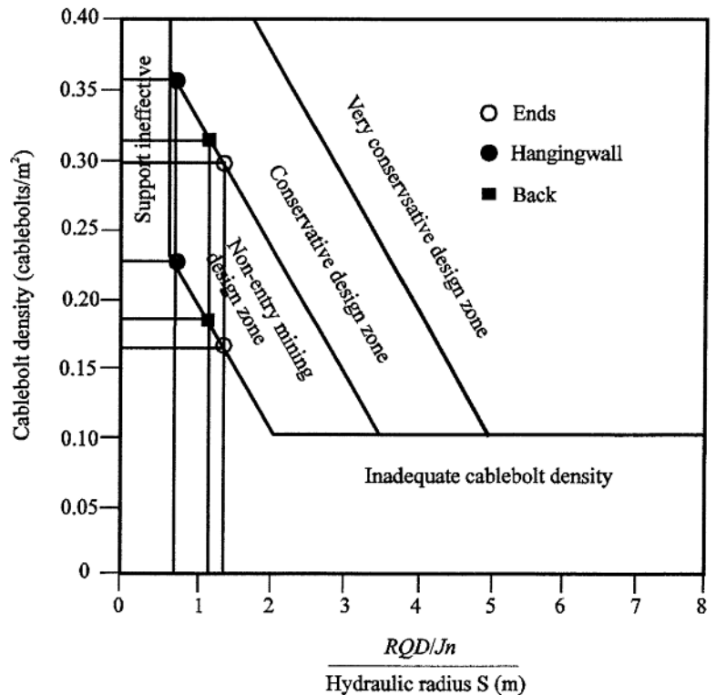
Figure 14.12: Cablebolt density for the preliminary design of the open stope at the example mine.
