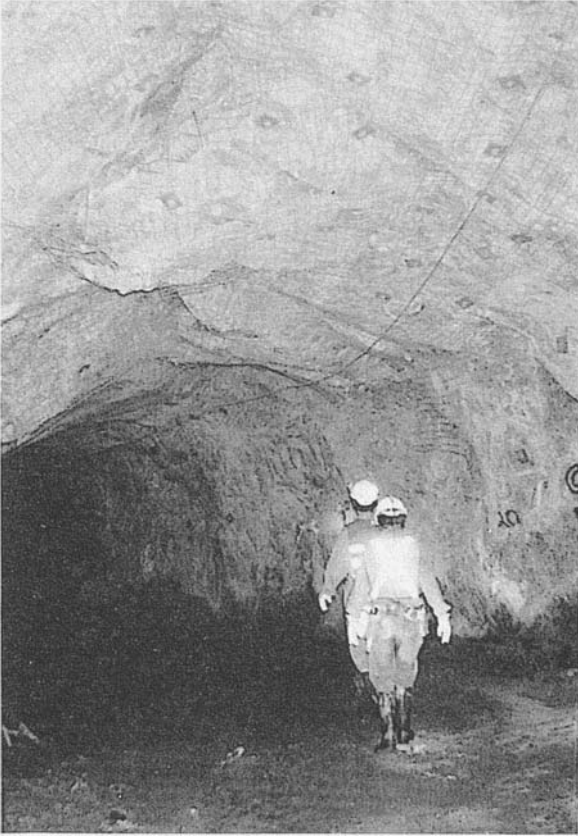
Figure 11.1: Rockbolts and welded wire mesh installed in the roof and upper sidewalls of a ramp excavation in an underground mine. This support has been installed to prevent injury to personnel and damage to equipment from small rockfalls.
