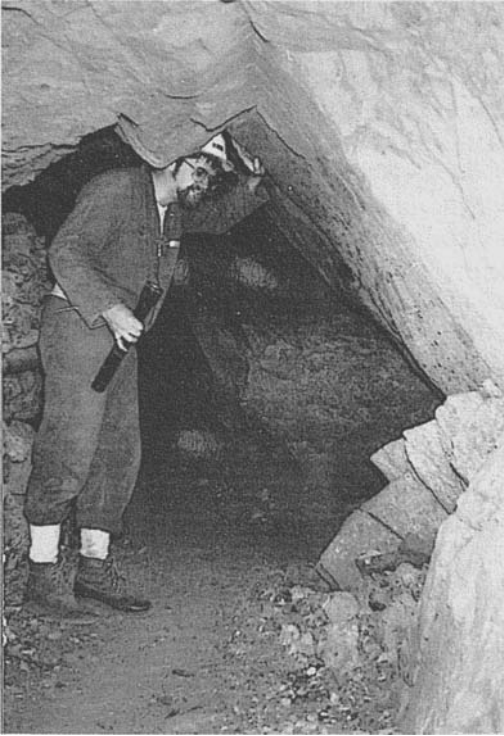
Figure 11.9: Profile of a small drive in massive blocky rock. The creation of a good excavation shape is sometimes difficult because blast fractures will tend to follow pre-existing weakness planes rather than break fresh rock.
