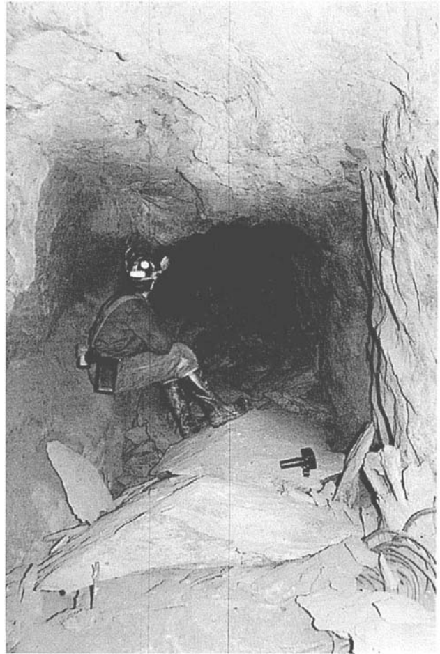
Figure 10.3: Spalling from the roof of an opening in highly stressed rock. The slabs on the floor have come from the left-hand side of the roof, just above the man's head. Spalling parallel to the right-hand sidewall is also visible.
