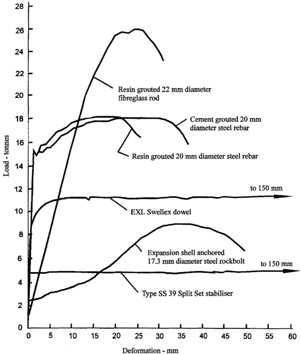
Figure 12.10: Load-deformation results obtained by Stillborg in tests carried out at Luleå University in Sweden. High strength reinforced concrete with a uniaxial compressive strength of 60 MPa was used for the test blocks and holes were drilled with a percussion rig to simulate in situ rock conditions.
