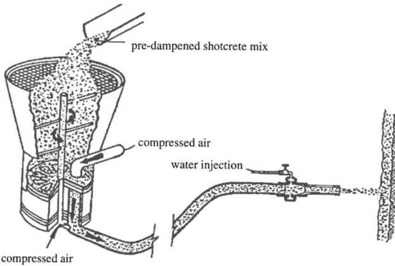
Figure 15.1: Simplified sketch of a typical dry mix shotcrete system. After Mahar et al. (1975).
