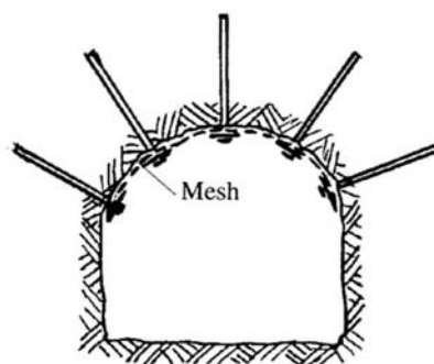
b) Arched roof excavation
