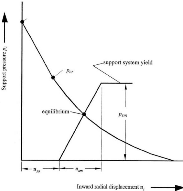
Figure 9.5: Response of support system to tunnel wall displacement resulting in establishment of equilibrium.
