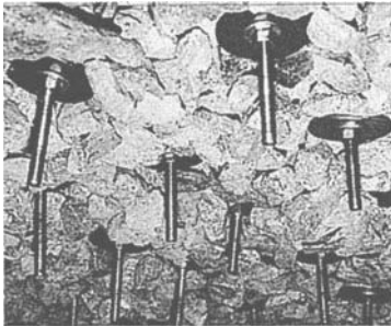
Photograph of the underside of Lang's bolted gravel plate model showing ravelling of rock pieces between face plates.
