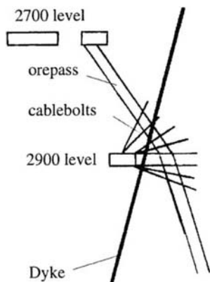
Pre-reinforcement of an orepass with cables installed from an external access. After Clegg and Hanson (1992).
