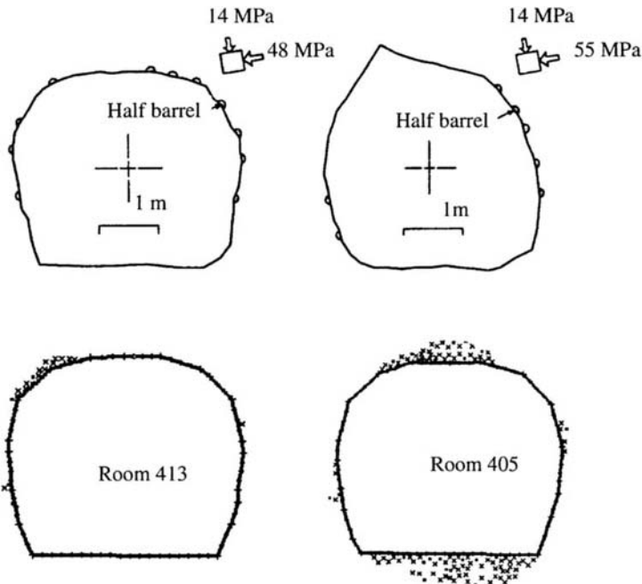
Figure 10.7: Comparison between observed and predicted failure in rooms 413 and 405 on the 410 level in the URL. The upper illustrations are observed conditions in room 413 and 405 respectively. The lower drawings show failure zones predicted by the program PHASES, applying the in situ stress conditions shown.
