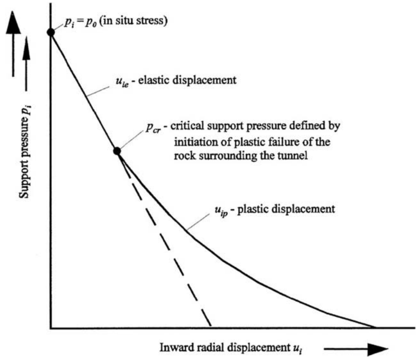
Figure 9.2: Graphical representation of relationships between support pressure and radial displacement of tunnel walls defined by Equations 9.5 and 9.7.
