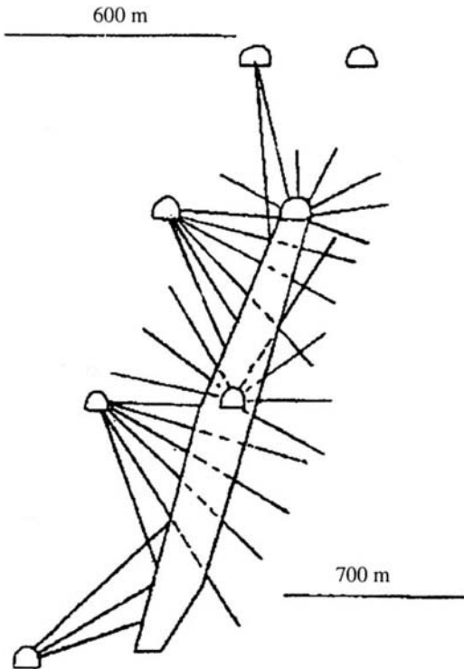
Figure 11.27: Cable bolt placing for sublevel stopping in the Kotalahti mine in Finland. Orebody sections are left without cables. After Lappalainen et al. (1984).
