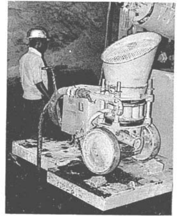
Typical dry mix shotcrete machine.
