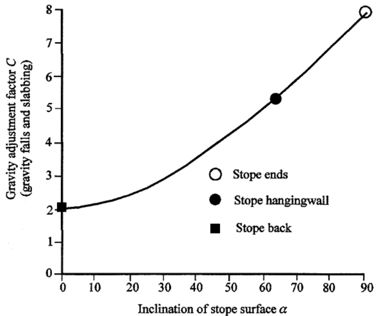
Figure 14.10: Gravity adjustment factors for example mine.
