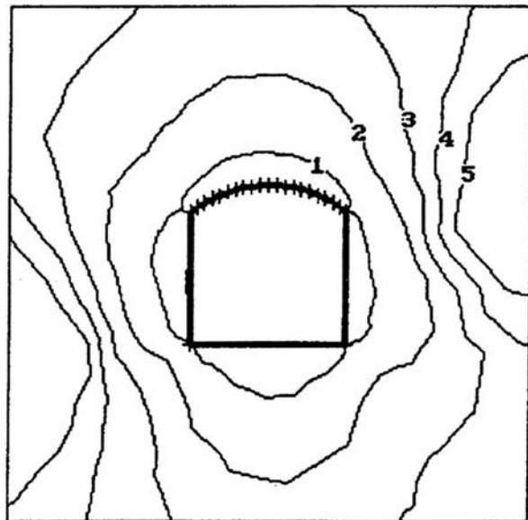
Figure 11.13: Contours of available strength to induced stress in the elastic rock surrounding a tunnel.
