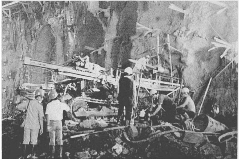
Figure 11.21: Installation of cables in the sidewall of the power cavern of the Mingtan project in Taiwan.
