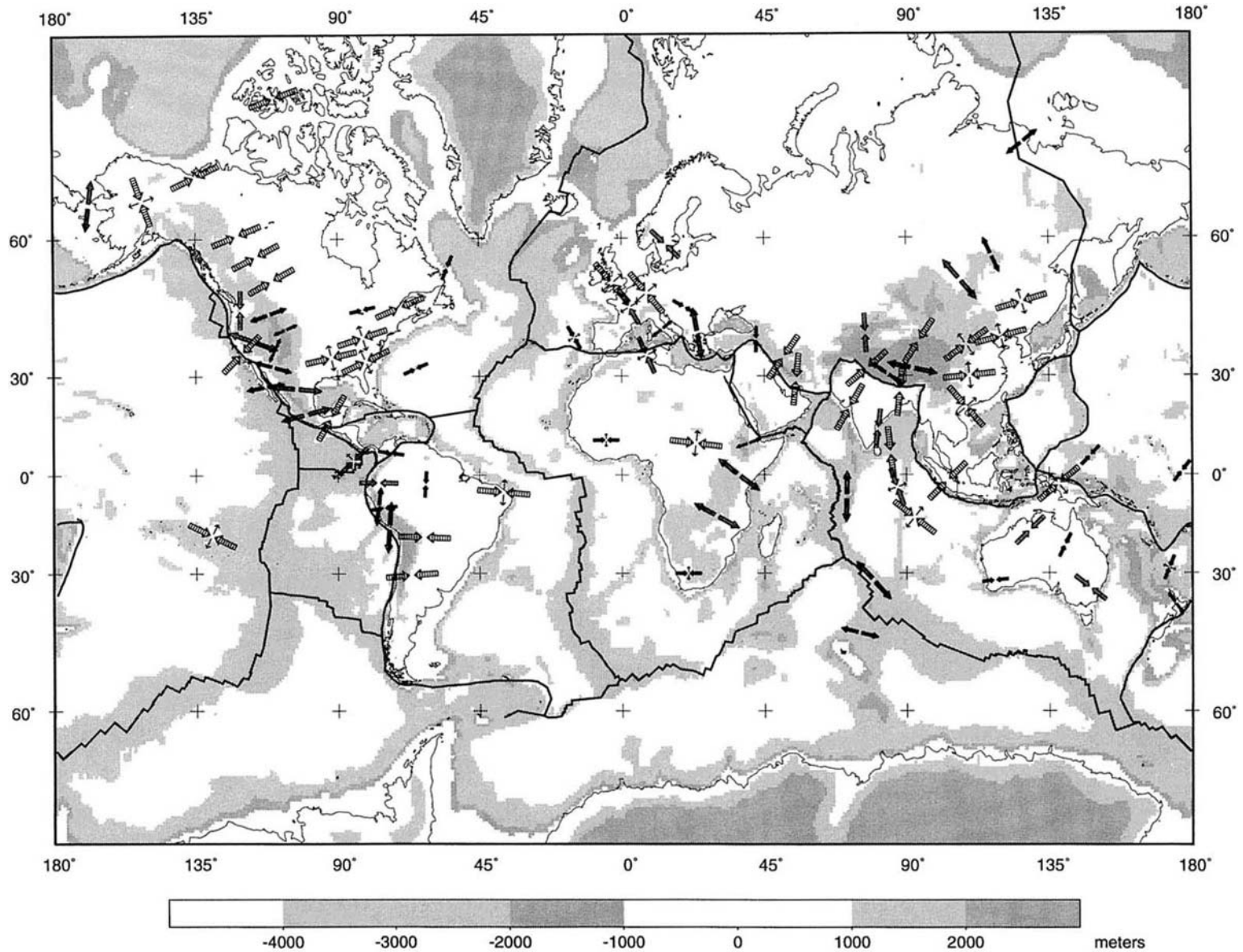
Figure 7.4: Generalised stress map showing mean directions based on average clusters of data shown in Figure 7.3. The meaning of the symbols is described in the text. Map provided by Dr M.L. Zoback from a paper by Zoback (1992).
