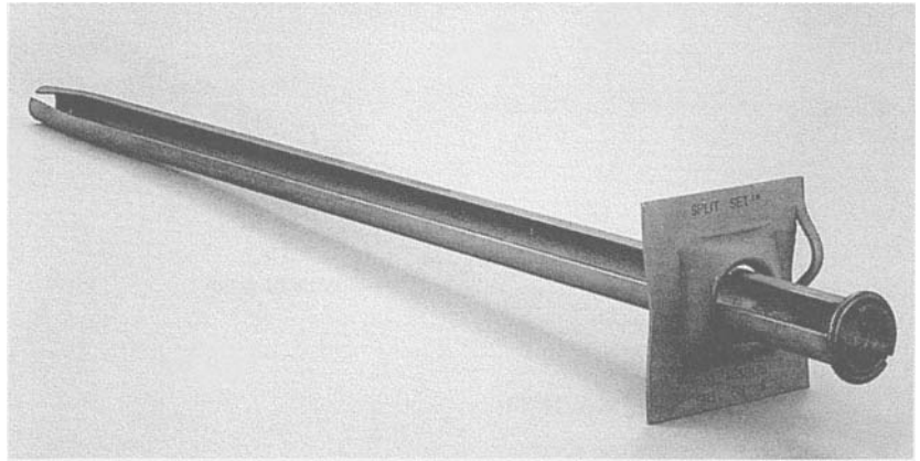
Figure 12.8: Split Set stabiliser. Ingersoll-Rand photograph.
