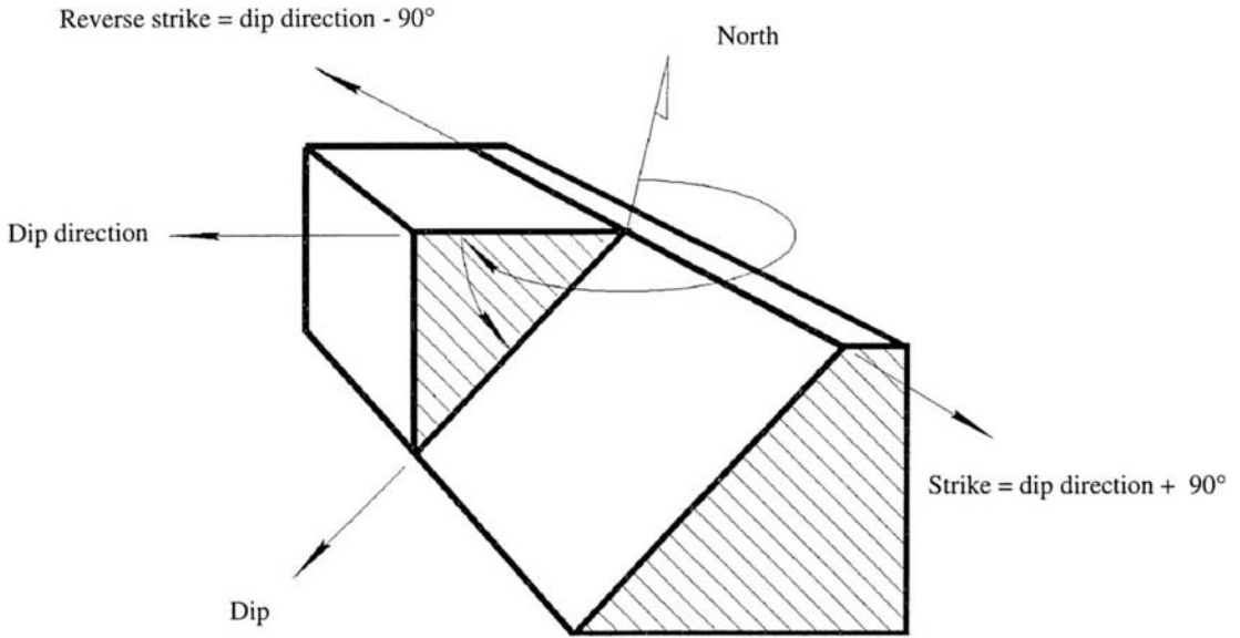
Figure 3.1: Definition of strike, dip and dip direction.
