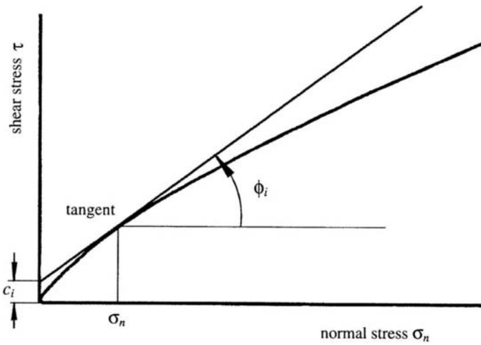
Figure 5.4: Definition of instantaneous cohesion c_i and instantaneous friction angle \phi_i for a non-linear failure criterion.
