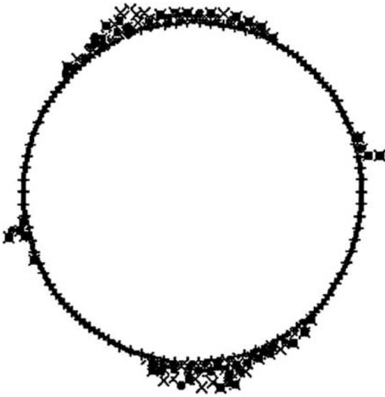
Figure 10.9: PHASES model showing the predicted shape of the failure zone for the Test Tunnel.
