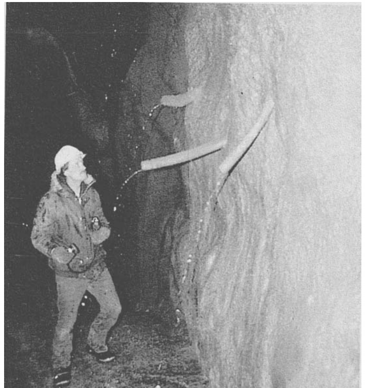
Figure 15.9: Plastic pipes used to provide drainage for a shotcrete layer applied to a rock mass with water-bearing joints.
