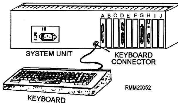
Figure 1-29.—Cable connection from keyboard to system unit.
