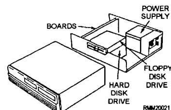
Figure 1-8.—A microcomputer system unit with the cover removed.
