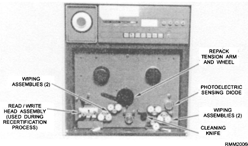
Figure 2-12.—Tape cleaner/certifier.
