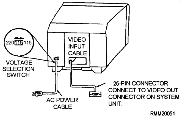
Figure 1-28.—Back of monitor.
