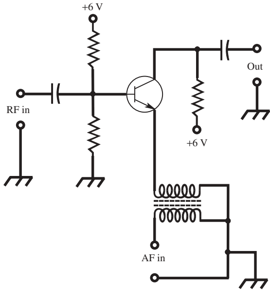
modulated amplifier
