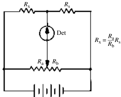
ratio-arm bridge
