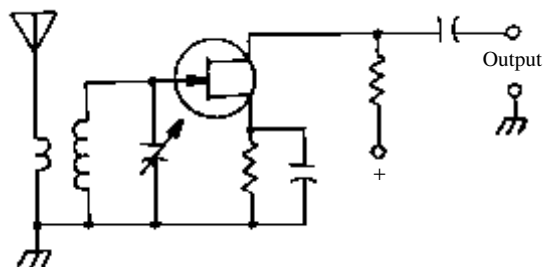
preamplifier
