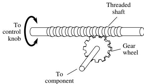
worm drive
