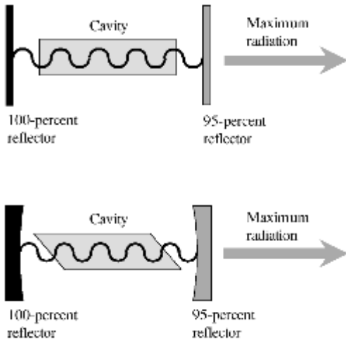
cavity laser
