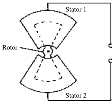
butterfly capacitor
