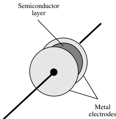
thermistor
