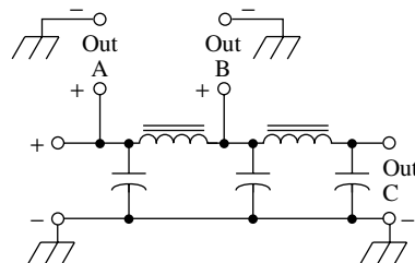
graded filter
