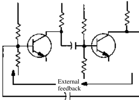
external feedback
