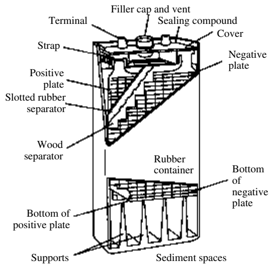
lead-acid cell
