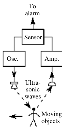
ultrasonic intrusion alarm
