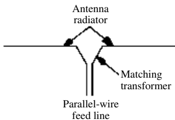
delta-matching transformer
