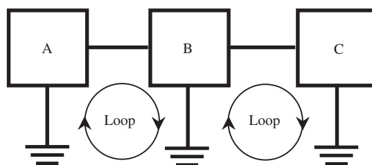
ground loop
