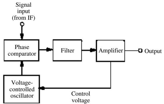
phase-locked loop
