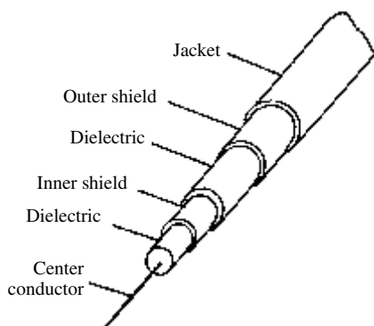
double shield
