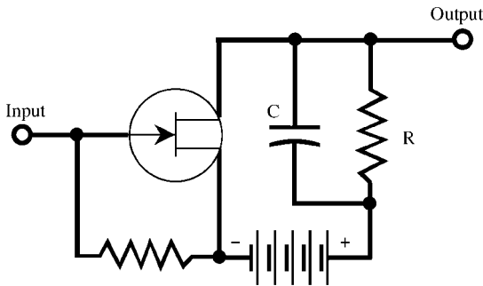
active RC network
