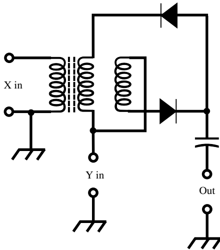
passive mixer
