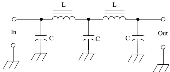
low-pass filter
