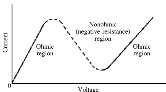
ohmic region
