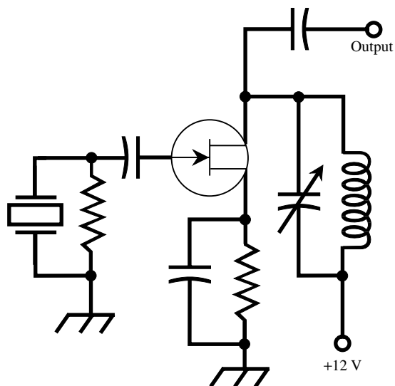
Miller oscillator
