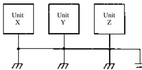
safety ground
