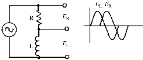
resistance-inductance phase shifter
