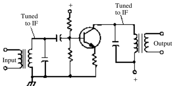
intermediate-frequency amplifier
