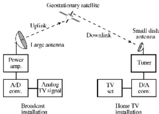
satellite television
