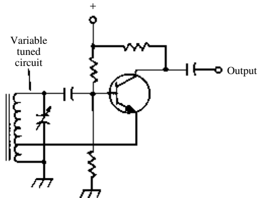
oscillator tuning
