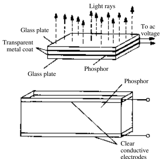
electroluminescent cell
