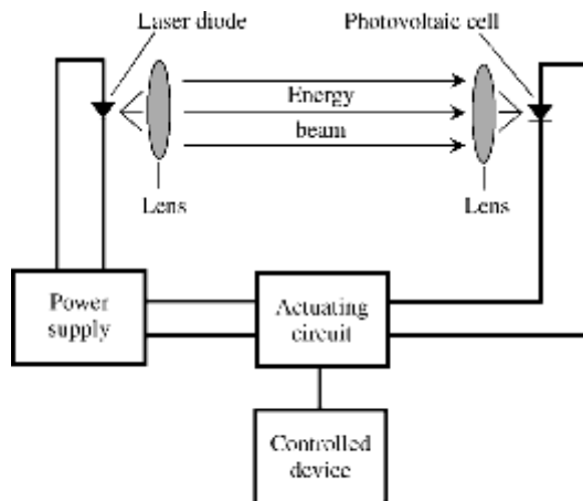
electric eye
