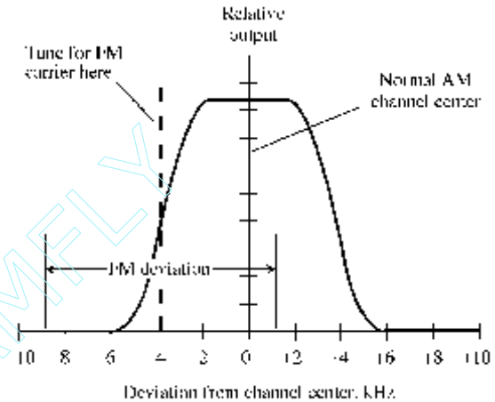
slope detector
