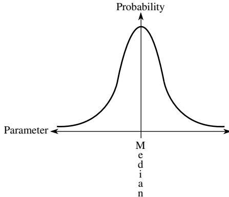
Gaussian distribution
