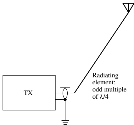
Fuchs antenna
