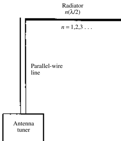
zeppelin antenna
