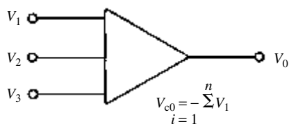
summing amplifier
