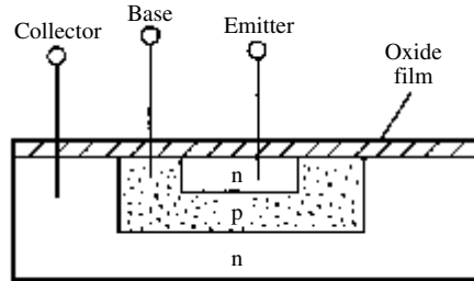
planar transistor
