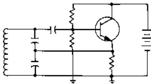
Colpitts oscillator
