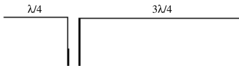
off-center feed
