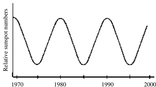
sunspot cycle
