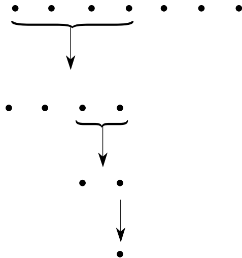
binary search
