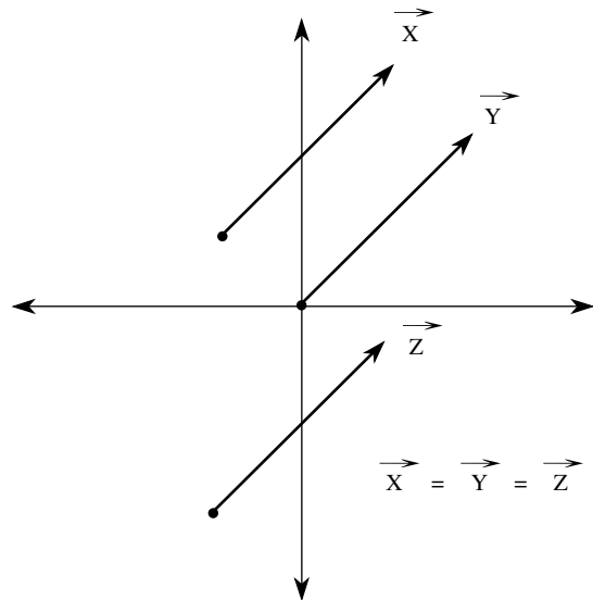
equal vectors
