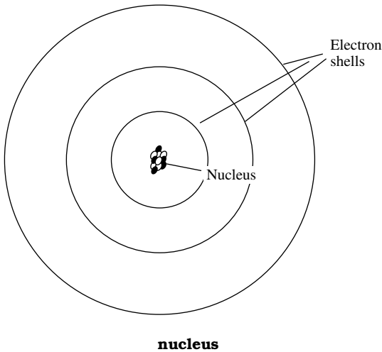
nucleus
