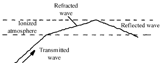
atmospheric refraction
