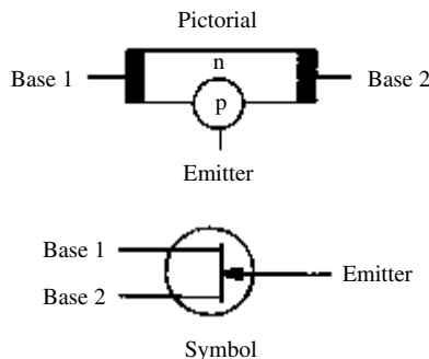
unijunction transistor
