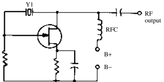
Pierce oscillator
