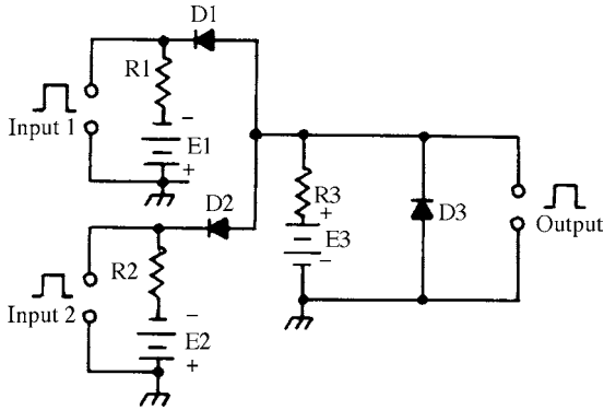
AND circuit
