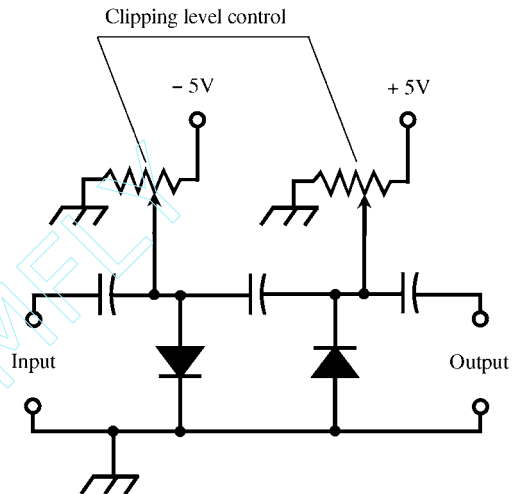
audio clipping
