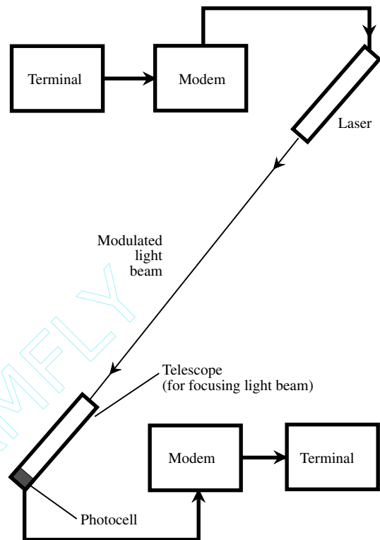
light-beam communication
