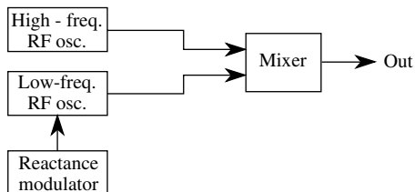
subcarrier frequency modulation
