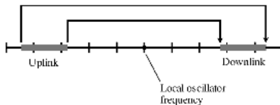
inverting transponder
