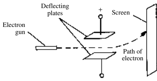
deflecting plate
