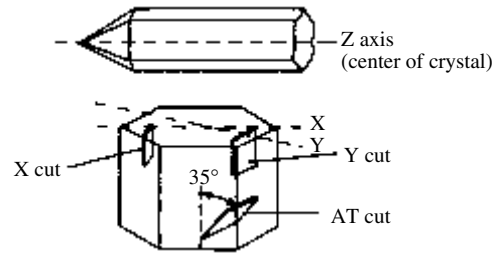
crystal cuts
