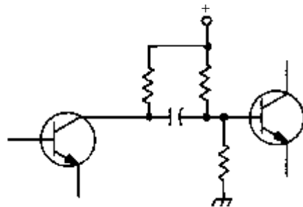
capacitive coupling
