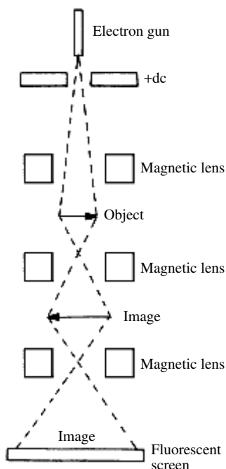
electron microscope
