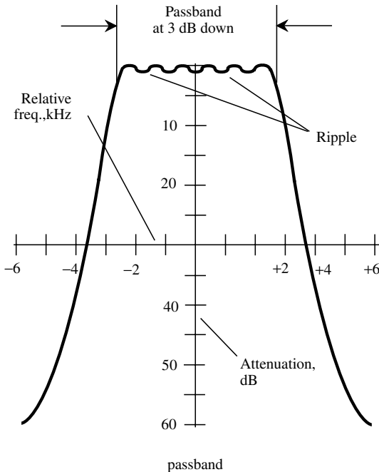
passband ripple
