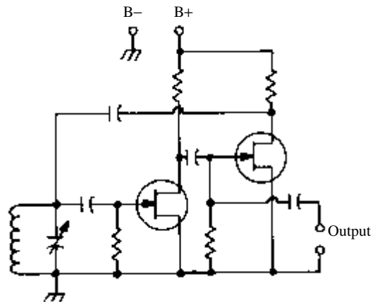
Franklin oscillator
