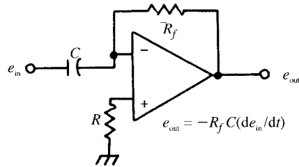
analog differentiator
