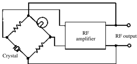
Meacham oscillator
