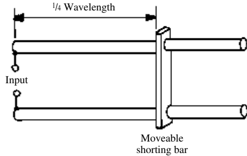
parallel-rod tuning
