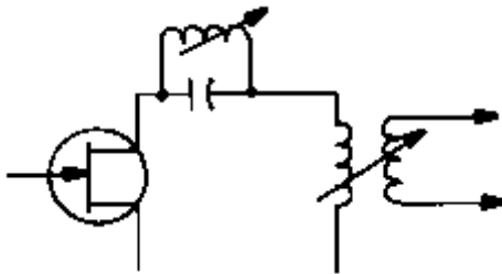
parallel-resonant trap
