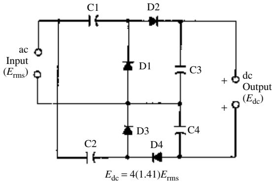
voltage quadrupler
