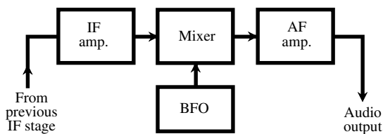
beat-frequency oscillator
