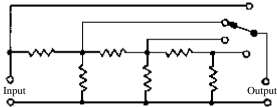
ladder-type attenuator
