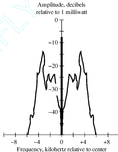
amplitude modulation
