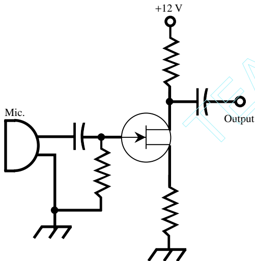
microphone amplifier
