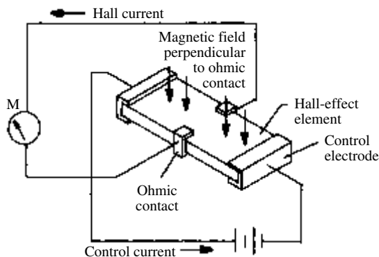
Hall generator
