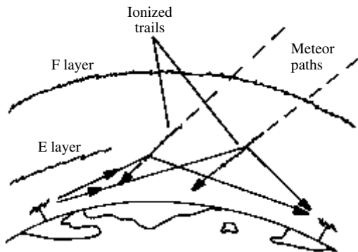
meteor-trail reflections
