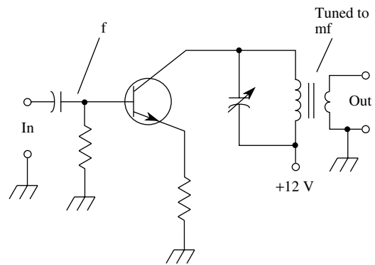
multiplier amplifier
