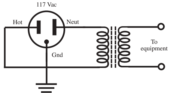
isolating transformer
