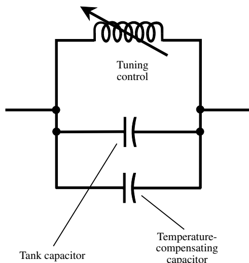
temperature-compensating component
