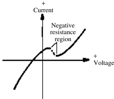
negative resistance
