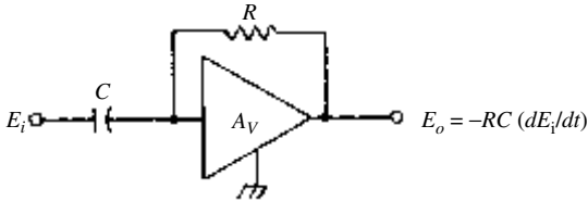
differentiator, 2
