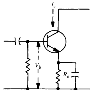
automatic bias
