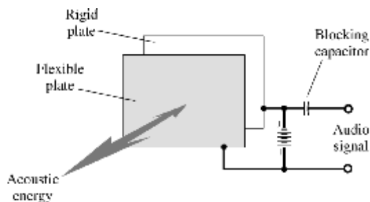
electrostatic speaker
