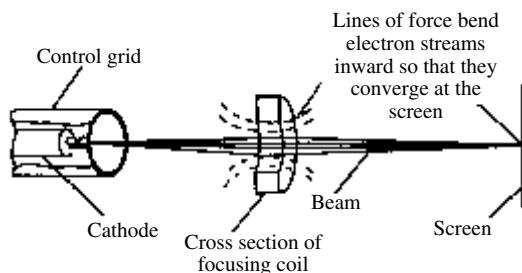
electromagnetic focusing
