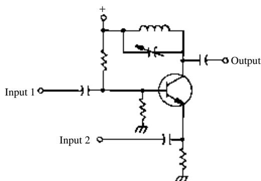
mixer
