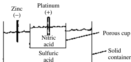
Grove cell
