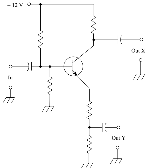
paraphase inverter
