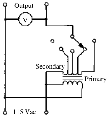
tapped transformer
