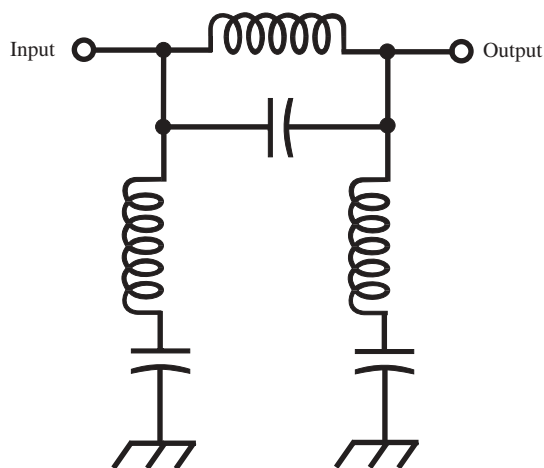
rejection filter
