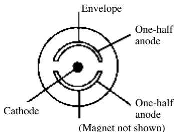
split-anode magnetron
