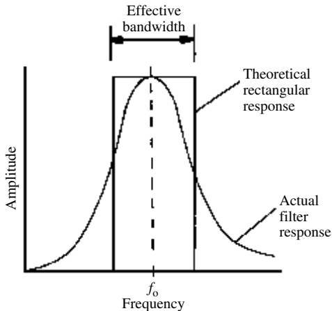
effective bandwidth
