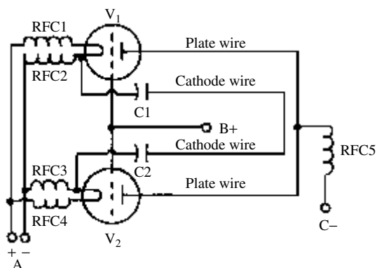
Kozanowski oscillator
