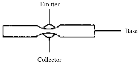
surface-barrier transistor
