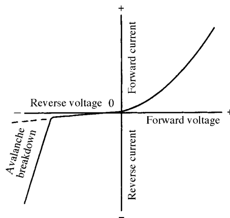
avalanche breakdown
