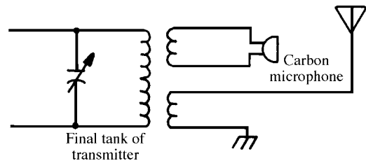
absorption modulation
