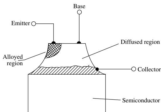
mesa transistor
