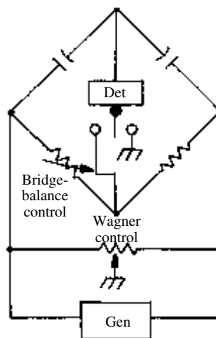
Wagner ground (with capacitance bridge)
