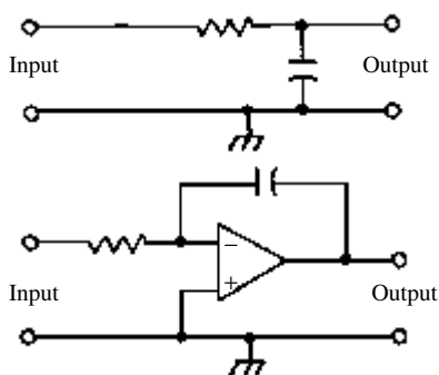
integrating networks
