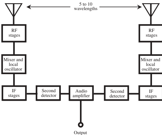
diversity reception
