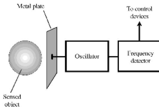
capacitive proximity sensor
