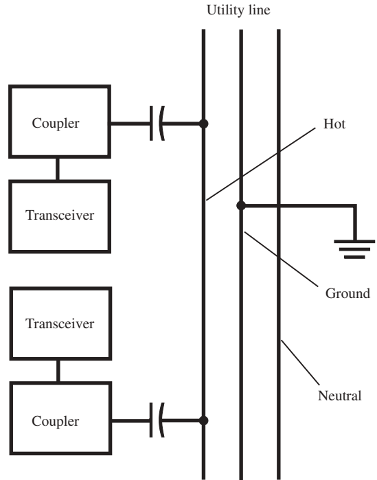
wired radio
