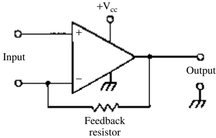
negative feedback
