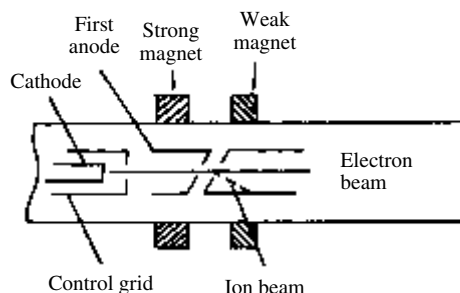
slashed-field-gun CRT
