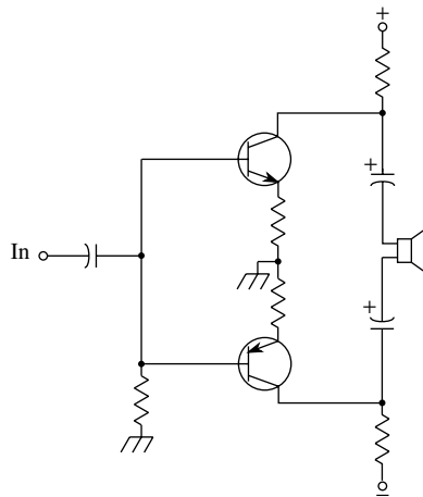
complementary-symmetry circuit
