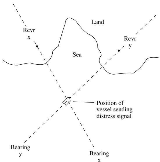
direction finding
