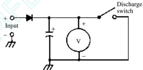
positive-peak voltmeter
