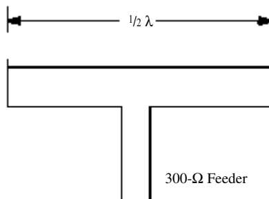
folded dipole
