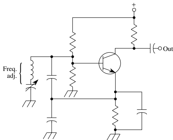
Clapp oscillator
