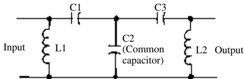
common-capacitor coupling
