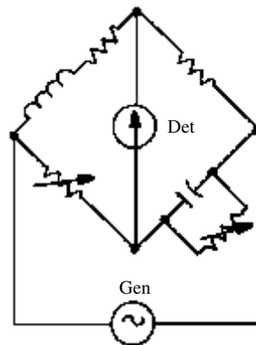
Maxwell bridge
