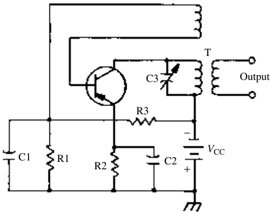
tuned-collector oscillator
