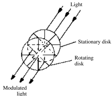
episcotister
