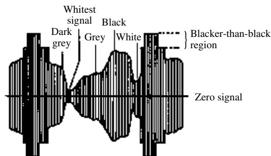
video signal
