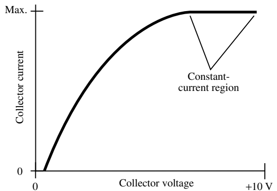
constant-current curve
