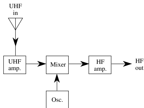
UHF converter, 1
