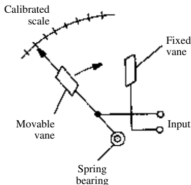
electrostatic voltmeter
