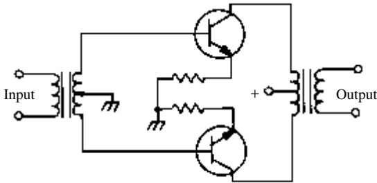
power amplifier
