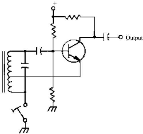
oscillator keying
