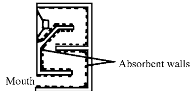
acoustic labyrinth
