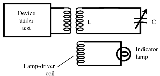
absorption wavemeter
