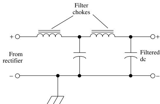
power-supply filter
