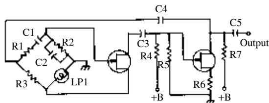
Wien-bridge oscillator
