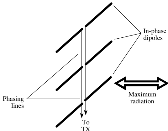
broadside array
