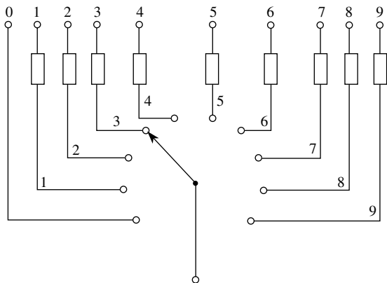
decade box
