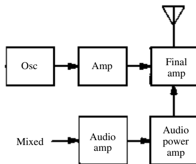
high-level modulation
