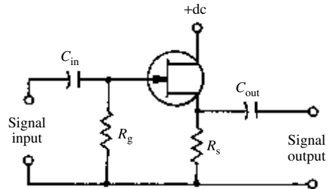
source follower
