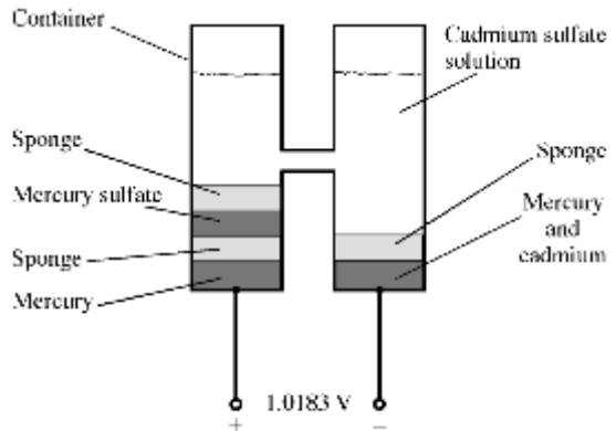
standard cell
