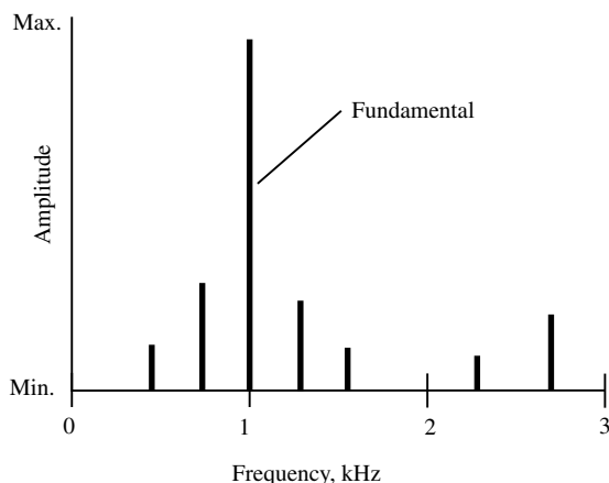
inharmonic distortion
