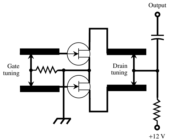
Meissner circuit
