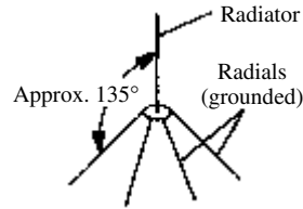
drooping radials
