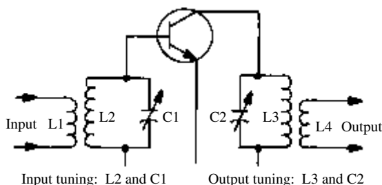
double-tuned circuit
