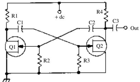
drain-coupled multivibrator
