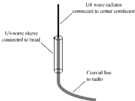
coaxial antenna
