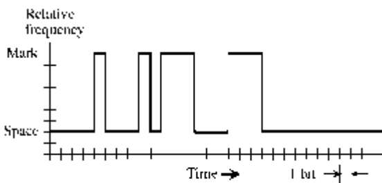
frequency-shift keying
