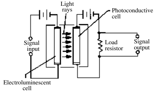
lumistor
