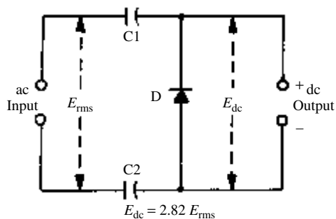
Villard circuit, 1
