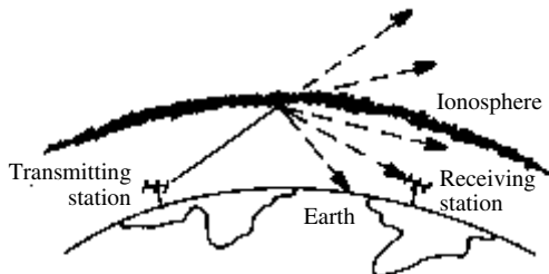
scattering
