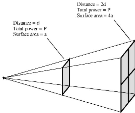
inverse-square law
