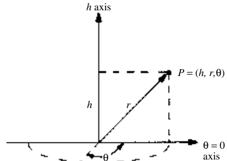
cylindrical coordinates
