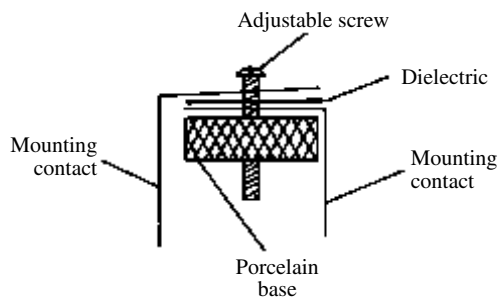
trimmer capacitor
