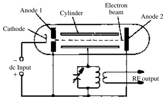
Heil oscillator
