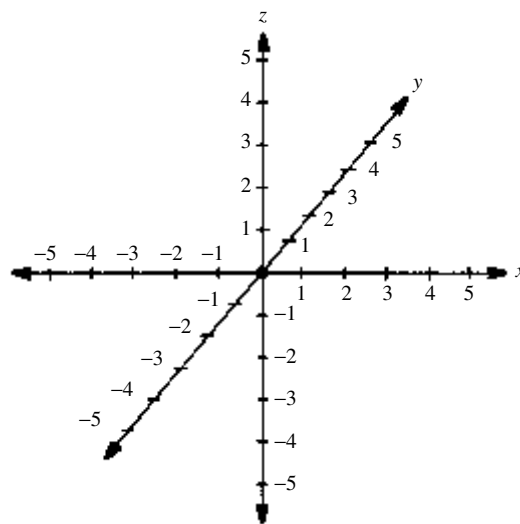
Cartesian three-space
