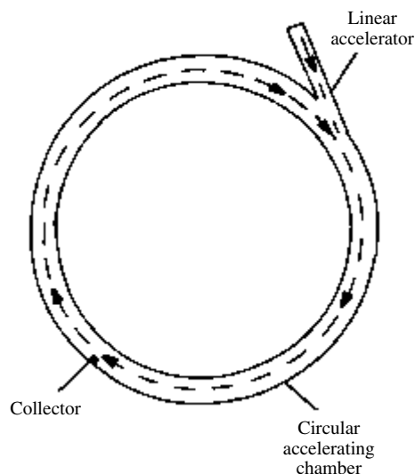
synchrotron
