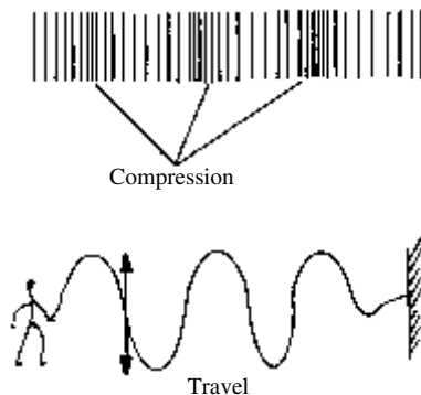
elastic waves
