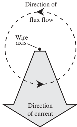
Ampere's Law
