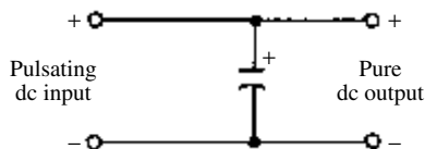
capacitor filter
