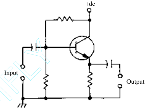
emitter follower
