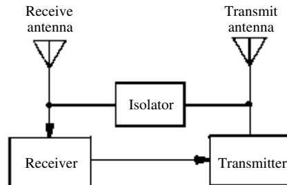
repeater
