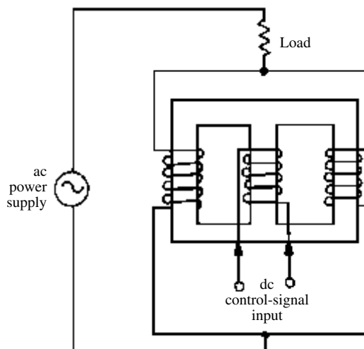
magnetic amplifier
