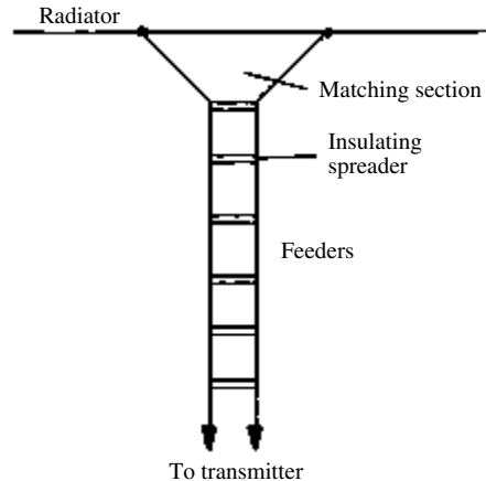
wye-matched-impedance antenna
