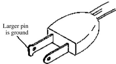
polarized plug
