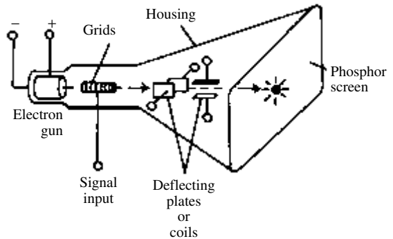
picture tube
