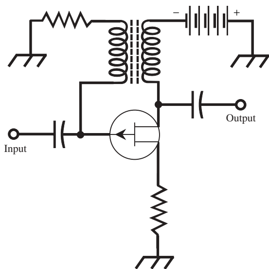
magnetic feedback
