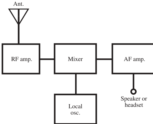
direct-conversion receiver
