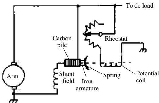
carbon-pile regulator
