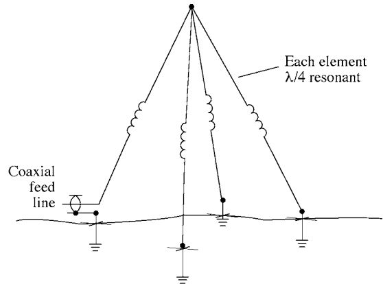
Alexanderson antenna
