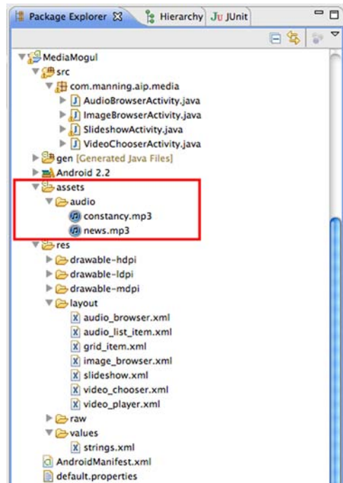
Figure 11.3 Storing multimedia files as assets
