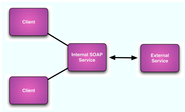
Figure 7.2: SOAP architecture
