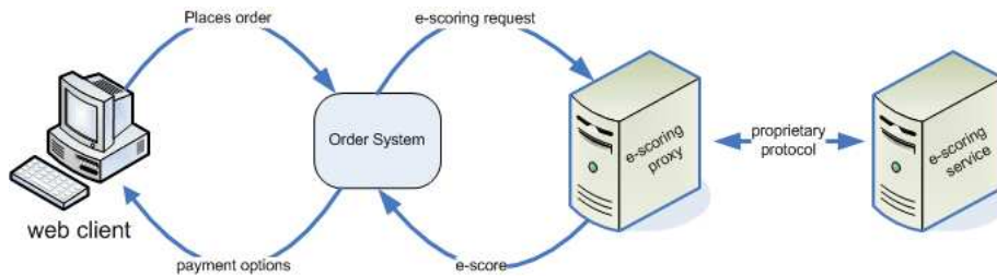
Figure 3.2: e-score architecture
