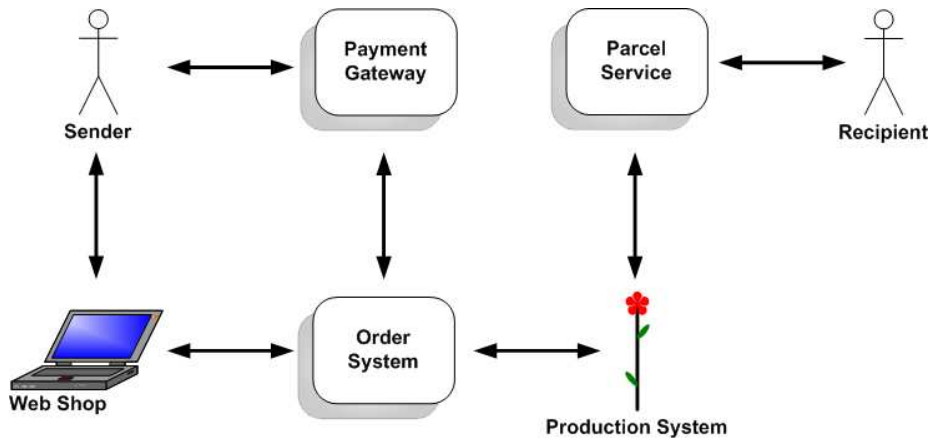
Figure 1.1: PragBouquet Infrastructure
