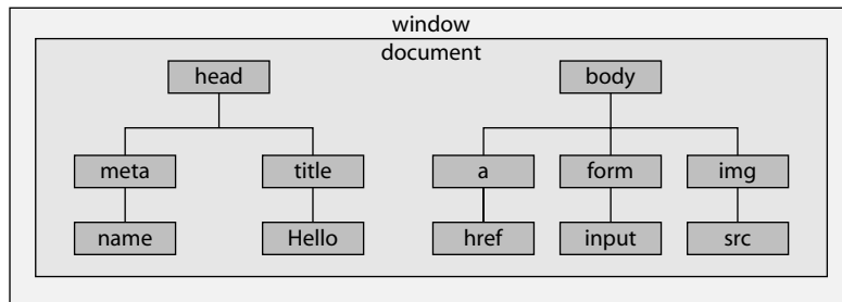
FIGURE 2-1 Example of a DOM showing head and body sections
