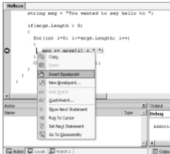
Figure 2.6 Inserting a Breakpoint
