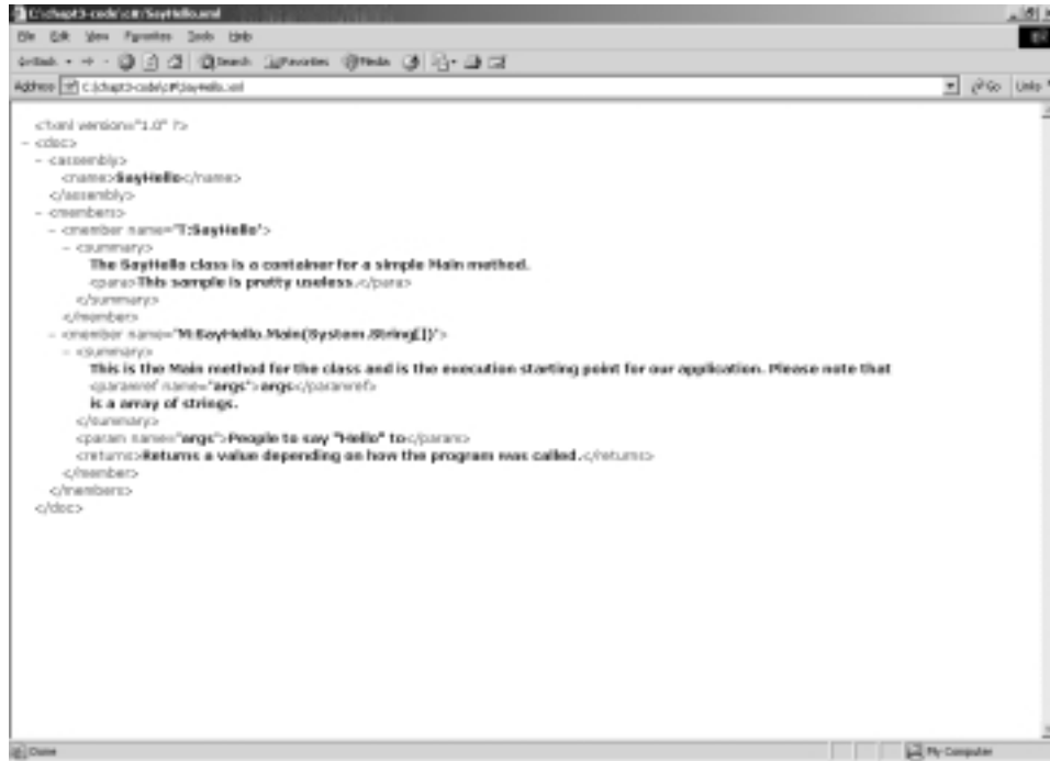
Figure 3.1 XML Documentation—Standard Format
