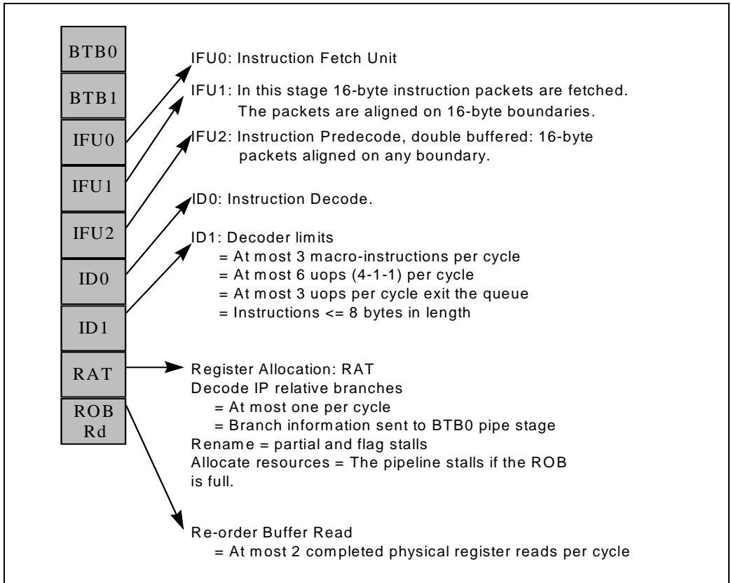
Figure 2-4. In-Order Issue Front-End
