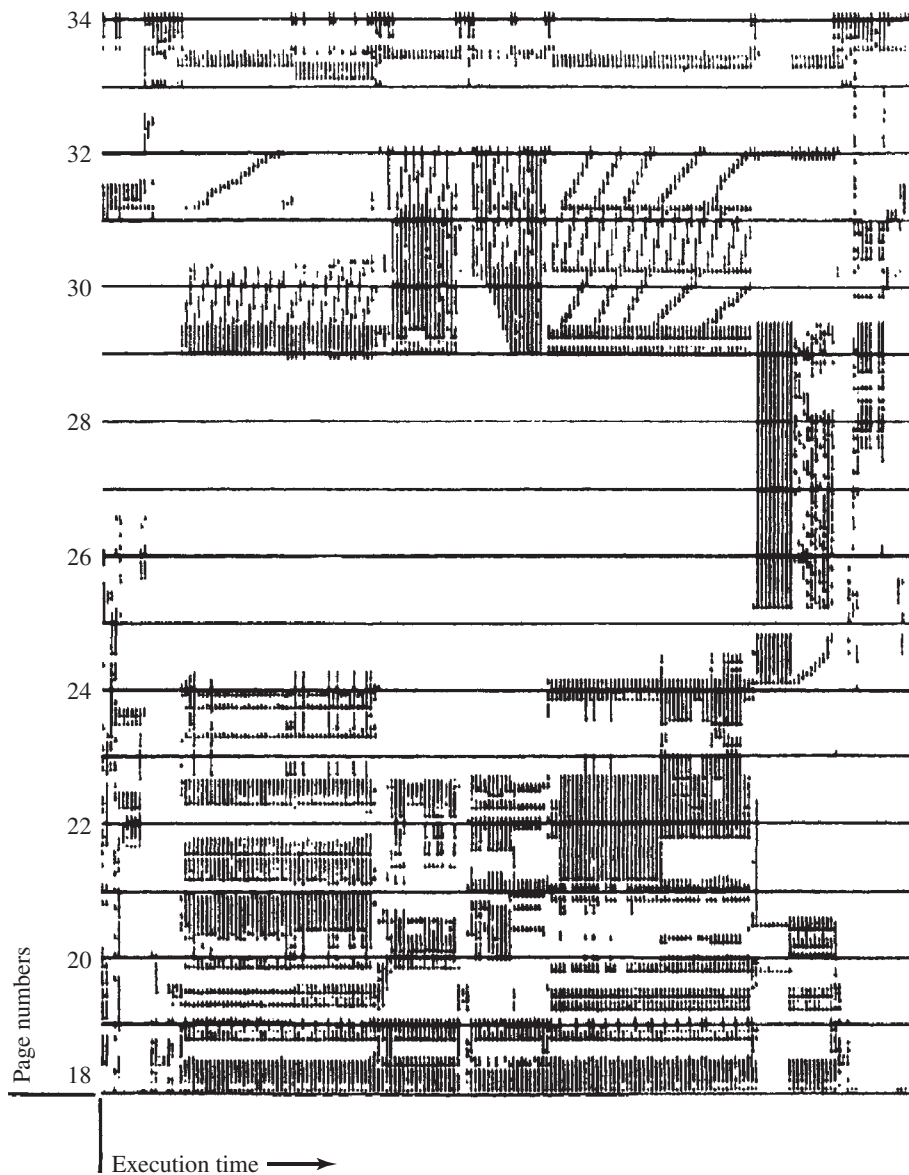
Figure 8.1 Paging Behavior
