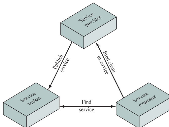
Figure 16.10 SOA Model
