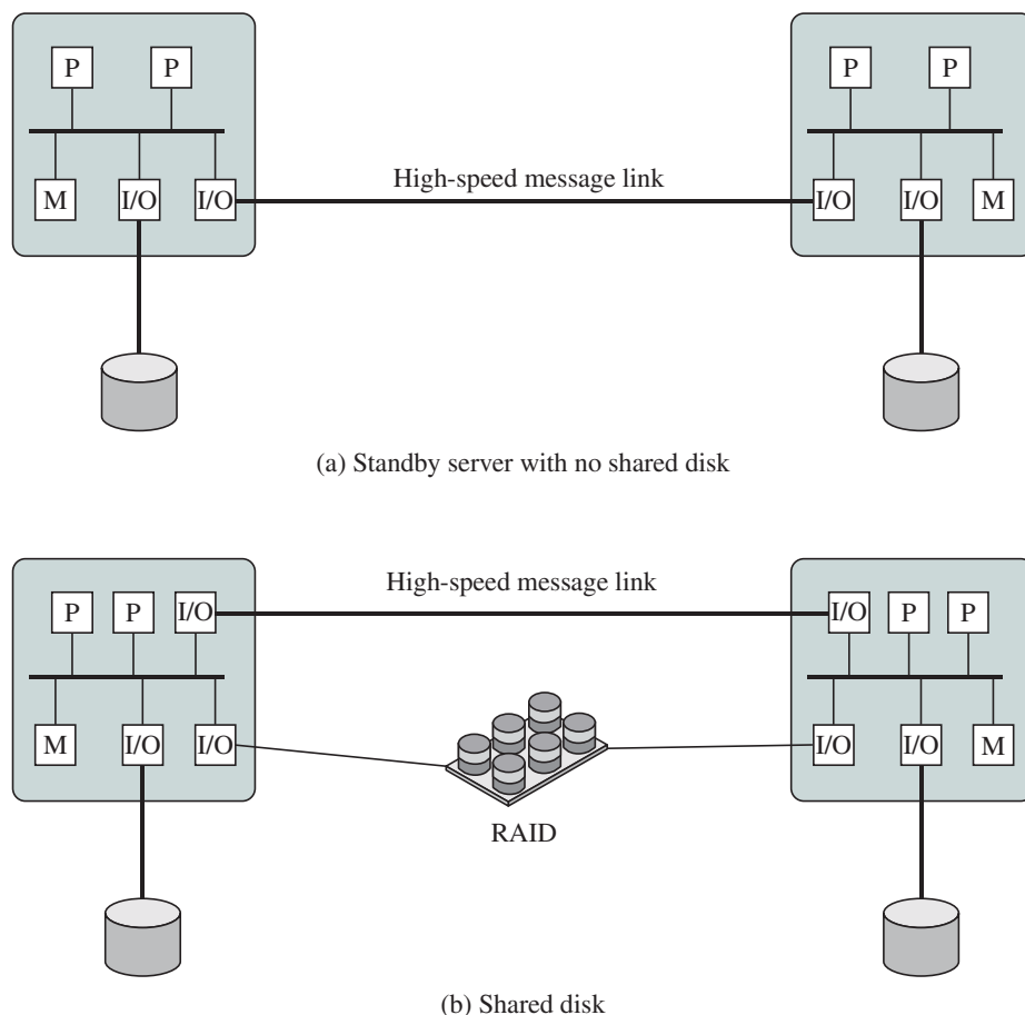
Figure 16.15 Cluster Configurations
