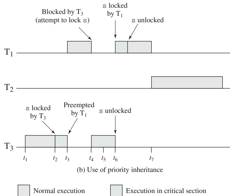
Figure 10.9 Priority Inversion
