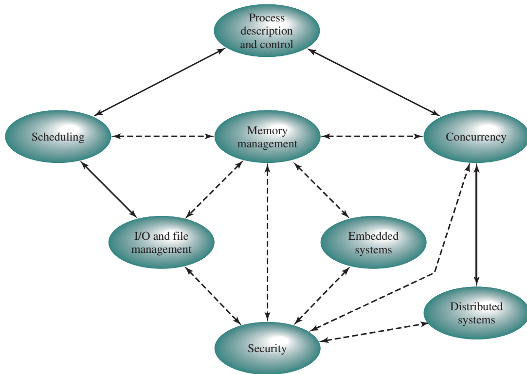
Figure 0.1 OS Topics
