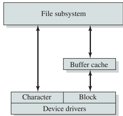
Figure 11.12 UNIX I/O Structure
