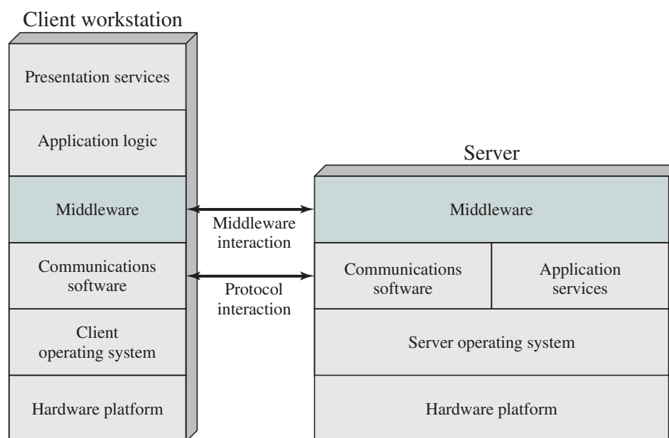
Figure 16.8 The Role of Middleware in Client/Server Architecture
