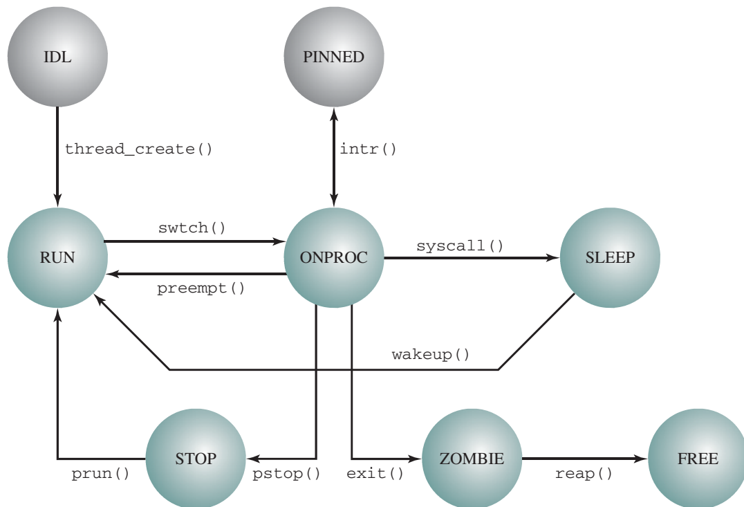
Figure 4.15 Solaris Thread States
