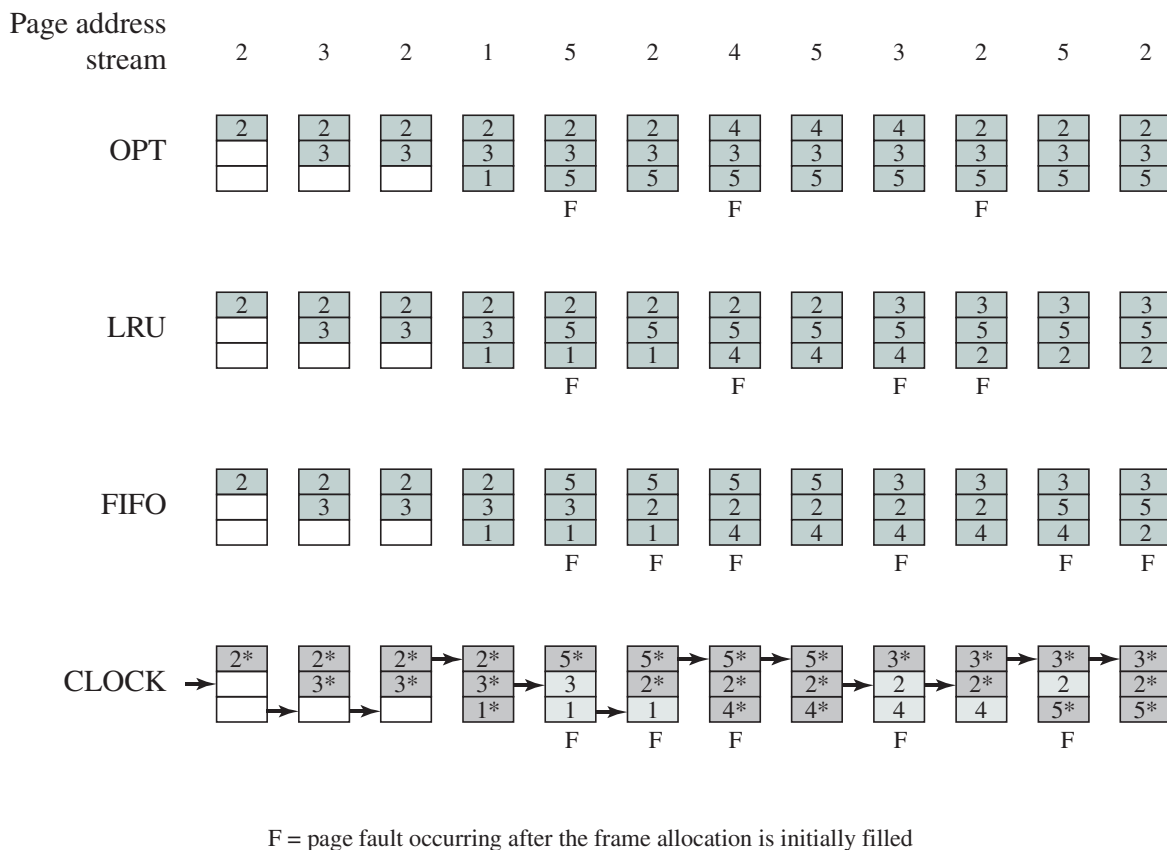
Figure 8.15 Behavior of Four Page Replacement Algorithms
