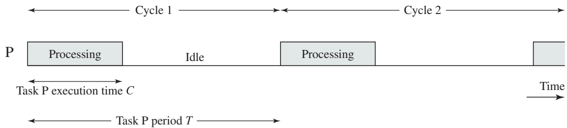
Figure 10.8 Periodic Task Timing Diagram
