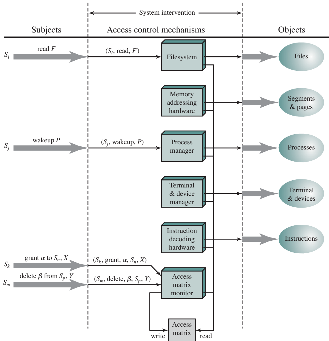
Figure 15.5 An Organization of the Access Control Function
