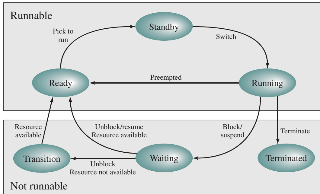
Figure 4.12 Windows Thread States
