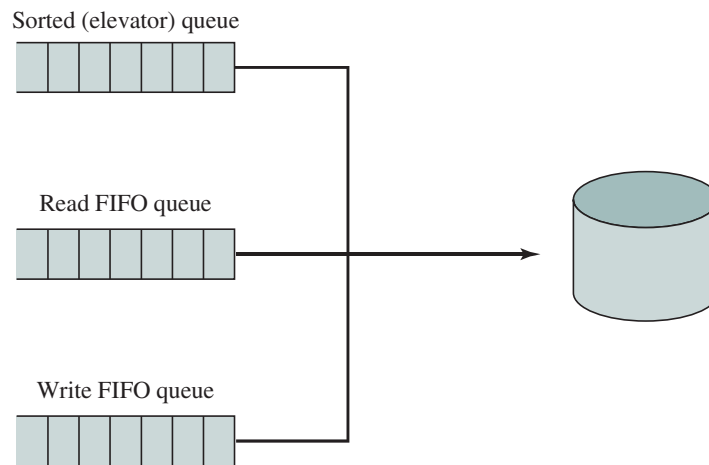
Figure 11.14 The Linux Deadline I/O Scheduler
