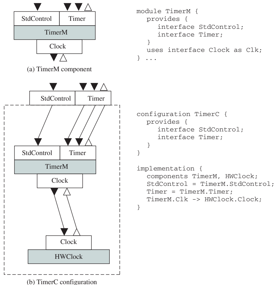
Figure 13.11 Example Component and Configuration
