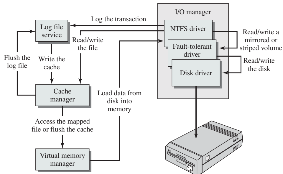
Figure 12.22 Windows NTFS Components
