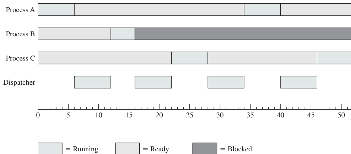
Figure 3.7 Process States for the Trace of Figure 3.4
