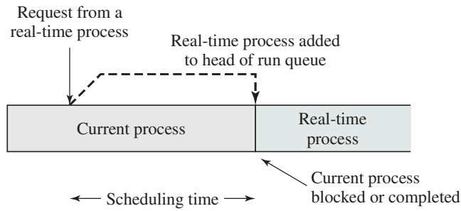
(b) Priority-driven nonpreemptive scheduler
