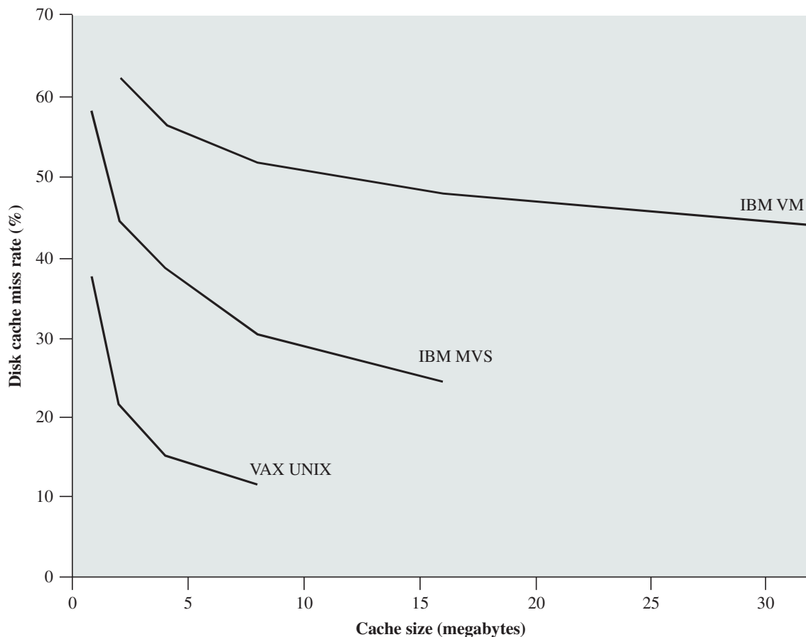
Figure 11.11 Disk Cache Performance Using Frequency-Based Replacement
