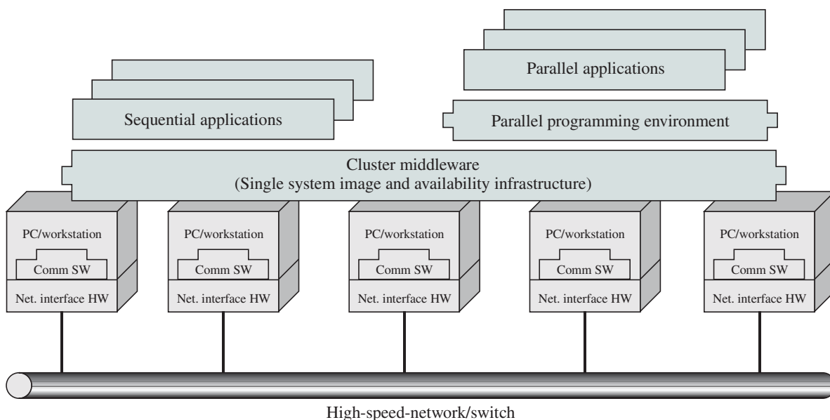
Figure 16.16 Cluster Computer Architecture
