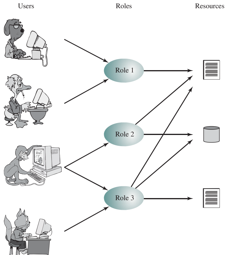
Figure 15.6 Users, Roles, and Resources
