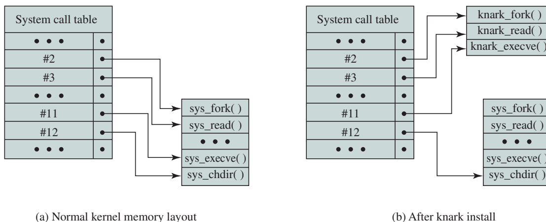
Figure 14.6 System Call Table Modification by Rootkit
