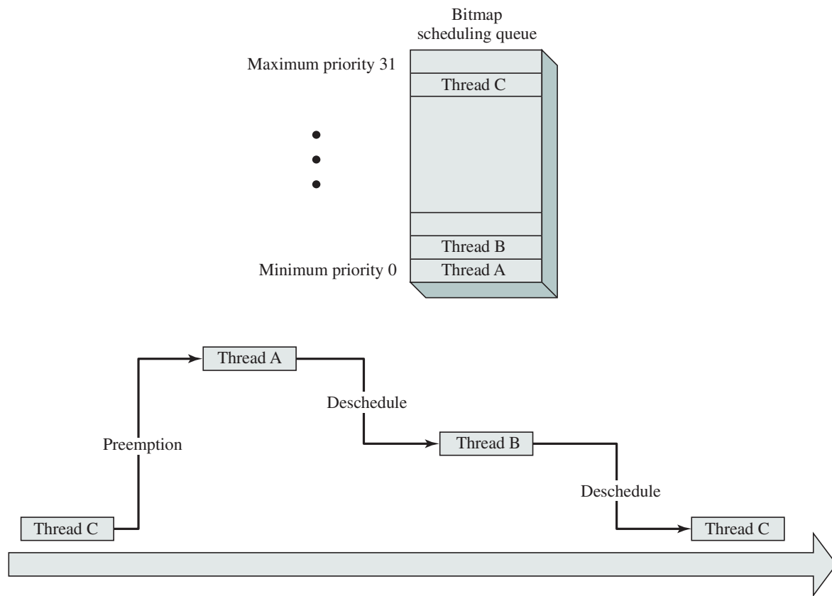
(a) Bitmap scheduler thread operation
