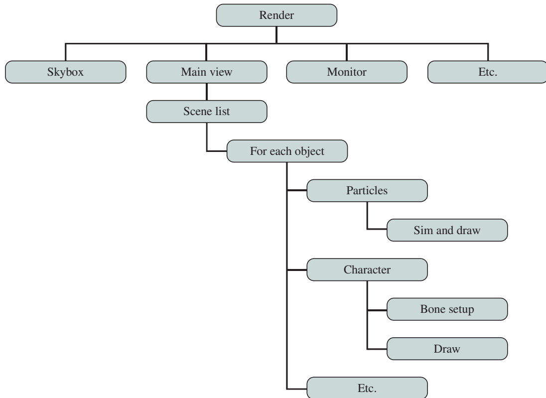
Figure 4.9 Hybrid Threading for Rendering Module
