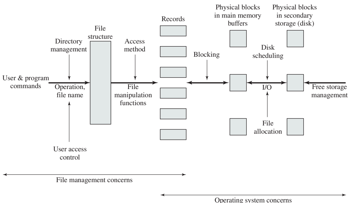
Figure 12.2 Elements of File Management
