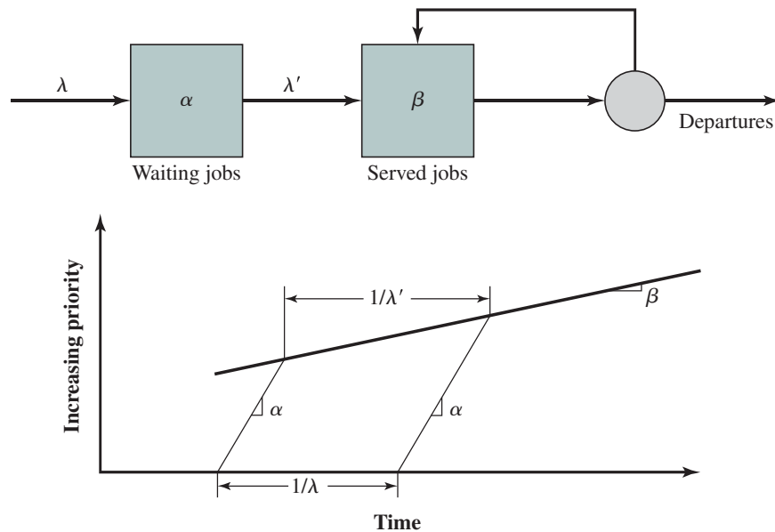
Figure 9.19 Selfish Round Robin
