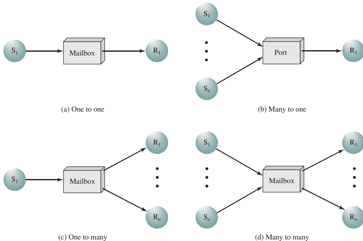
Figure 5.18 Indirect Process Communication
