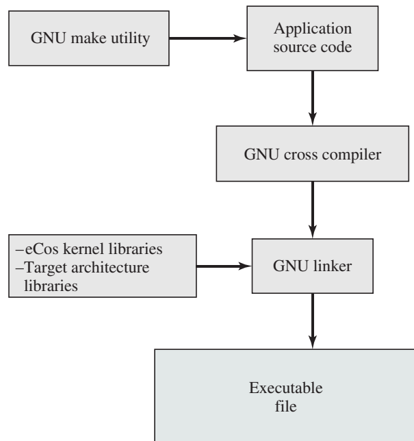
Figure 13.4 Loading an eCos Configuration
