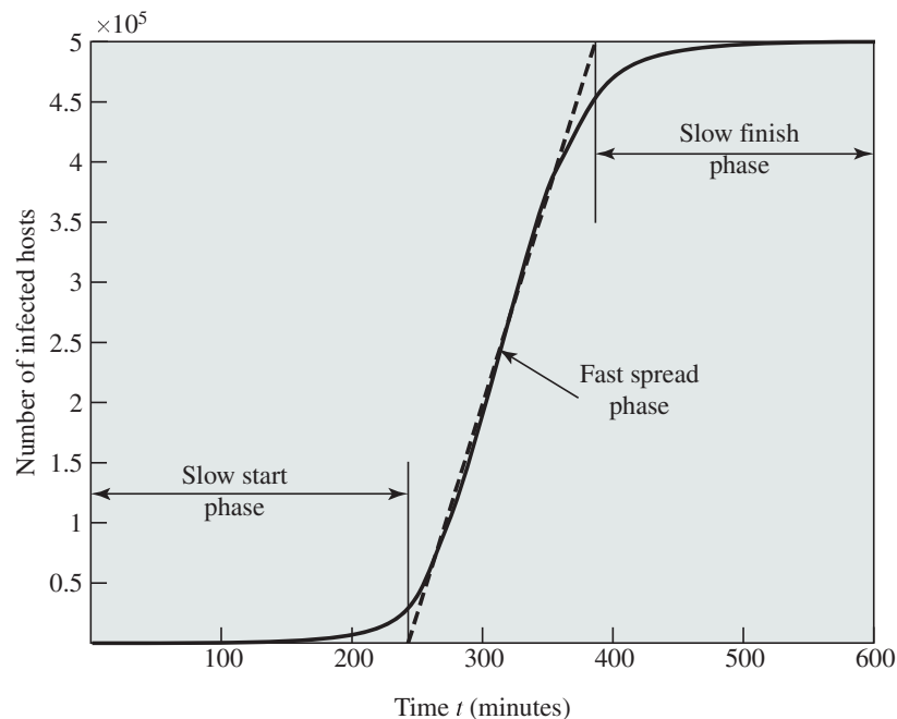
Figure 14.5 Worm Propagation Model
