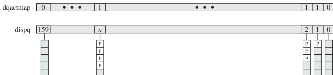
Figure 10.13 SVR4 Dispatch Queues
