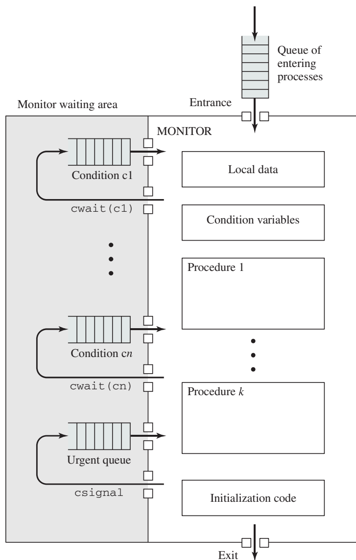
Figure 5.15 Structure of a Monitor
