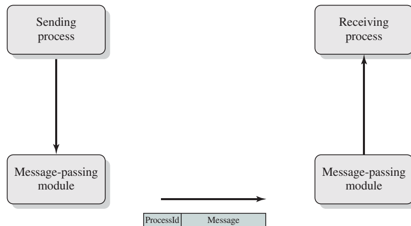
Figure 16.13 Basic Message-Passing Primitives
