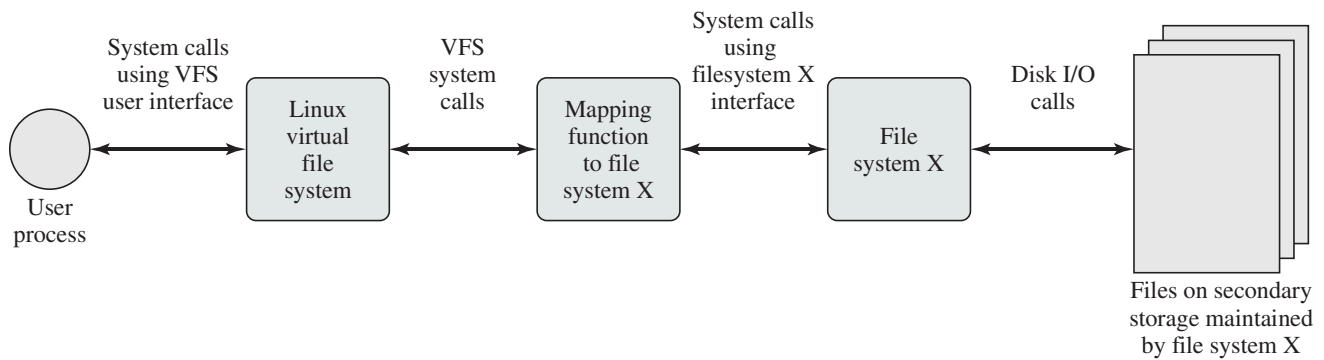
Figure 12.20 Linux Virtual File System Concept
