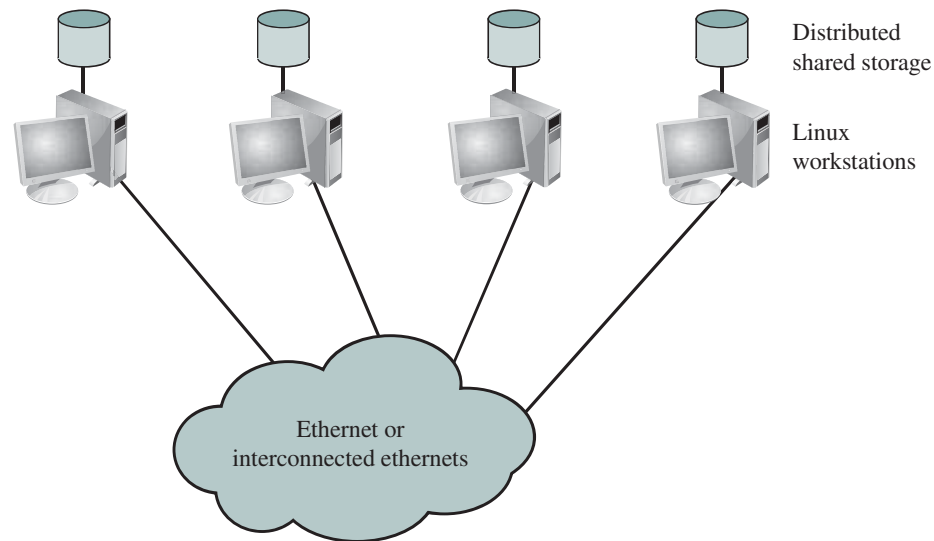
Figure 16.18 Generic Beowulf Configuration
