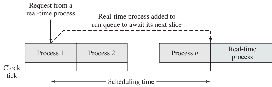
(a) Round-robin preemptive scheduler
