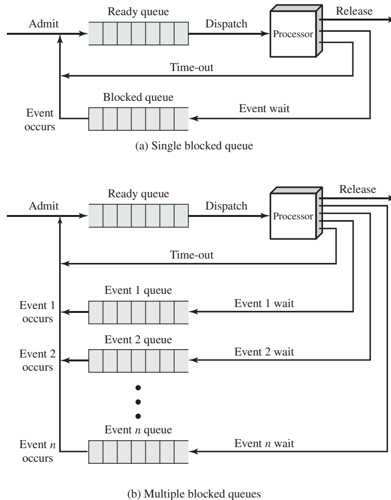
Figure 3.8 Queuing Model for Figure 3.6
