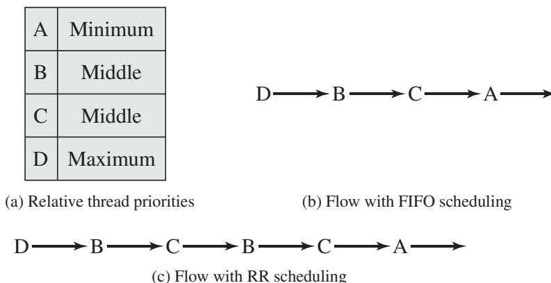
Figure 10.10 Example of Linux Real-Time Scheduling
