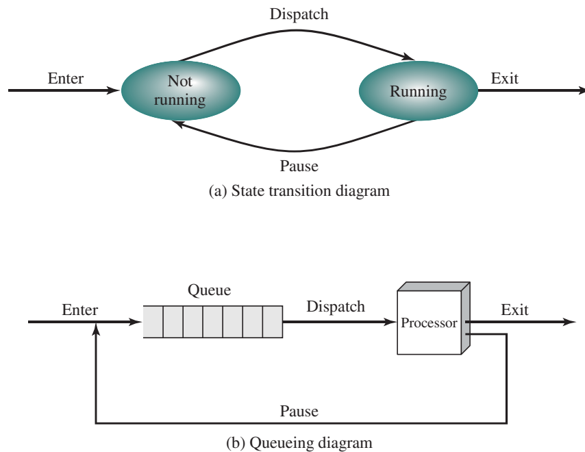
Figure 3.5 Two-State Process Model
