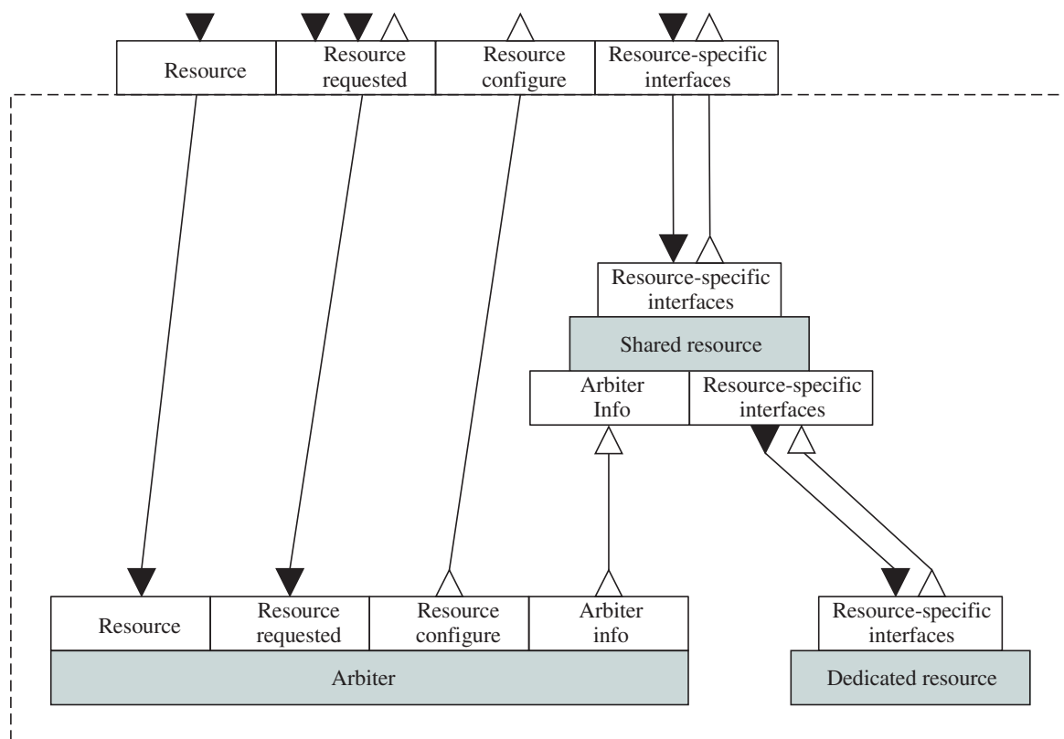
Figure 13.13 Shared Resource Configuration
