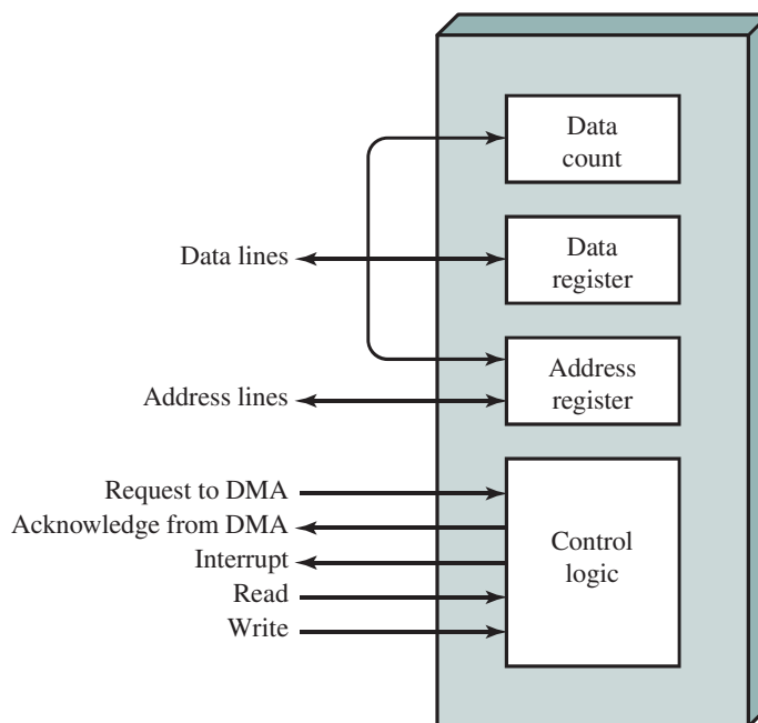
Figure 11.2 Typical DMA Block Diagram
