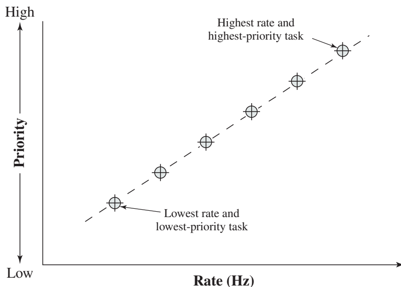
Figure 10.7 A Task Set with RMS [WARR91]
