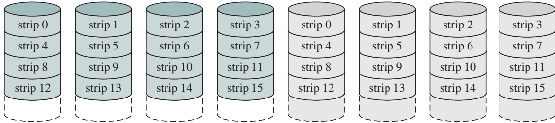
(b) RAID 1 (mirrored)
