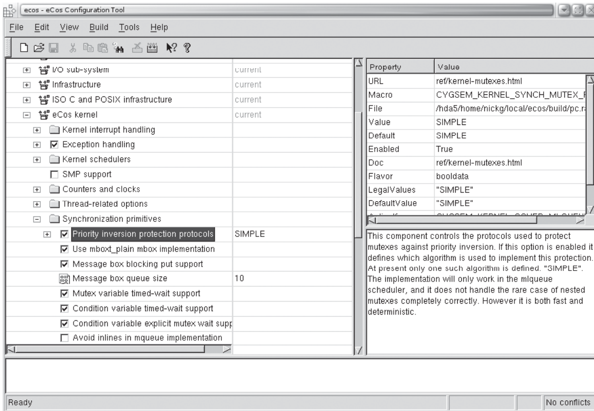
Figure 13.3 eCos Configuration Tool—Kernel Details
