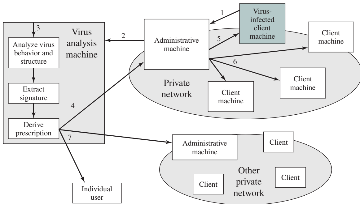
Figure 15.9 Digital Immune System
