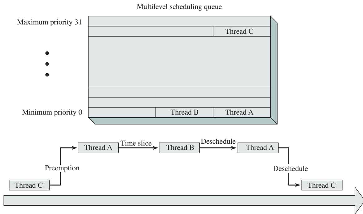
(b) Multilevel queue scheduler thread operation
