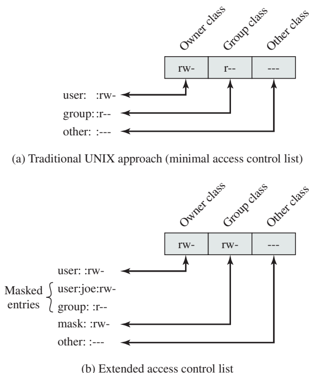
Figure 12.18 UNIX File Access Control
