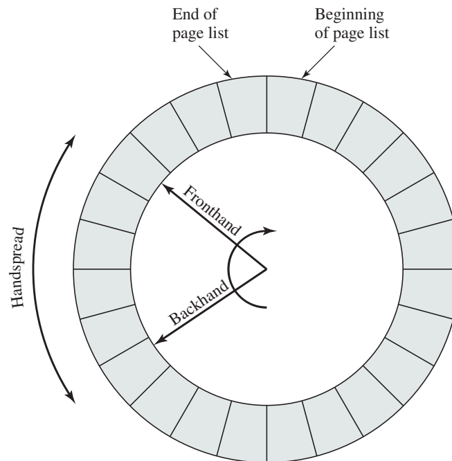
Figure 8.23 Two-Handed Clock Page Replacement Algorithm
