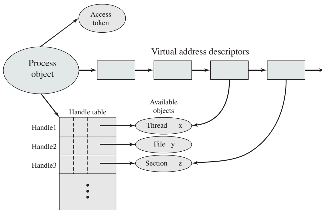
Figure 4.10 A Windows Process and Its Resources
