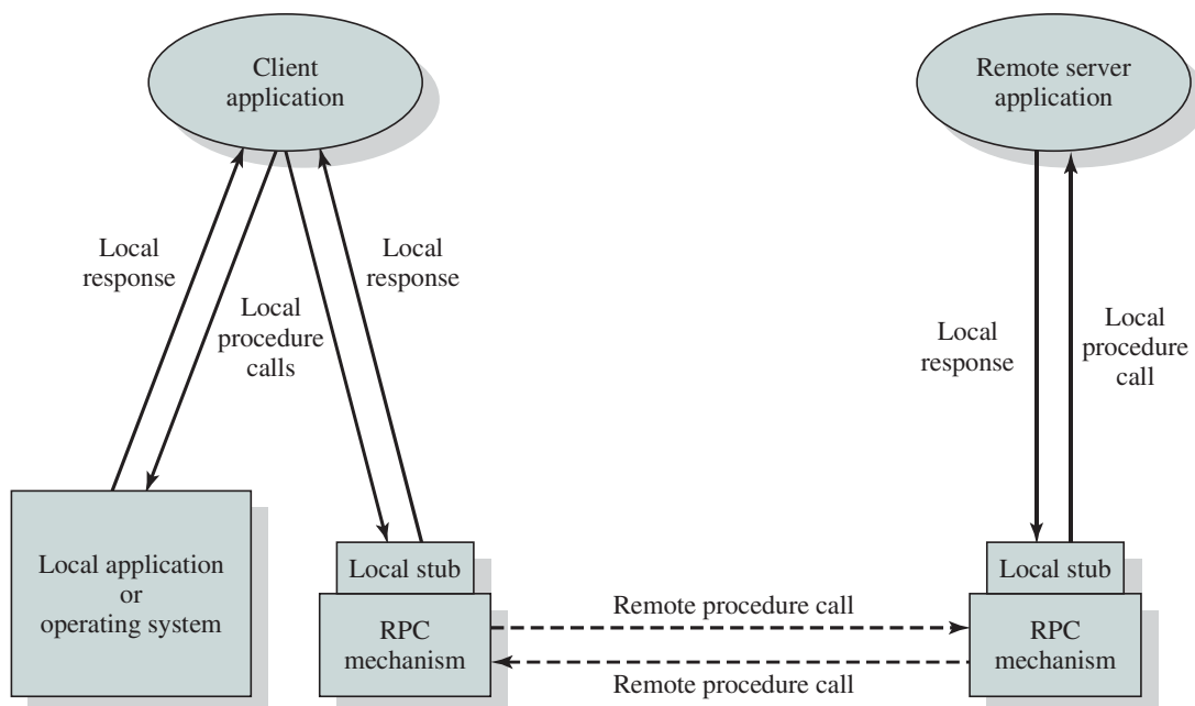
Figure 16.14 Remote Procedure Call Mechanism
