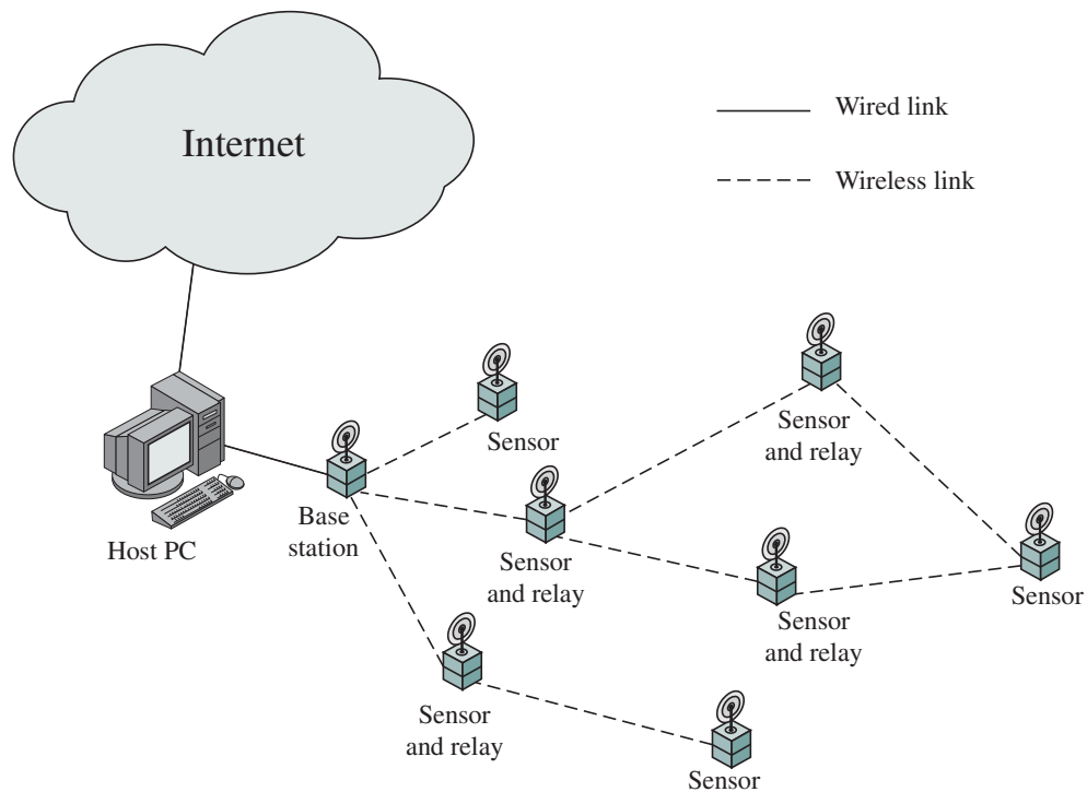
Figure 13.10 Typical Wireless Sensor Network Topology
