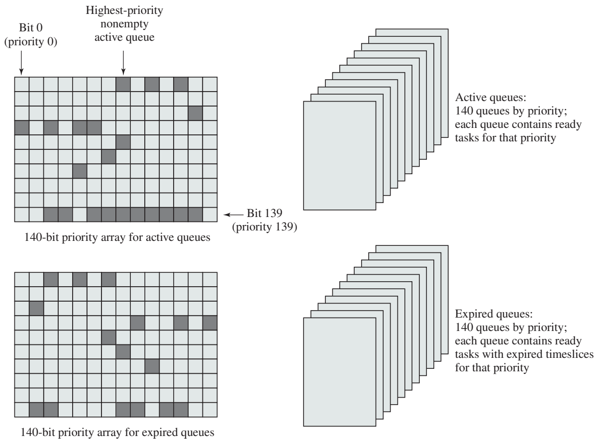
Figure 10.11 Linux Scheduling Data Structures for Each Processor
