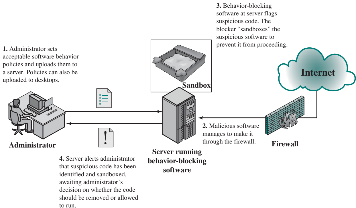
Figure 15.10 Behavior-Blocking Software Operation
