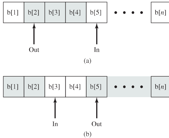
Figure 5.12 Finite Circular Buffer for the Producer/Consumer Problem
