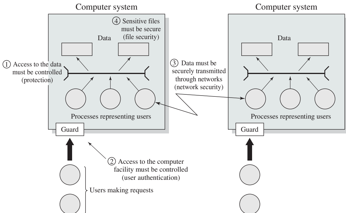
Figure 14.2 Scope of System Security
