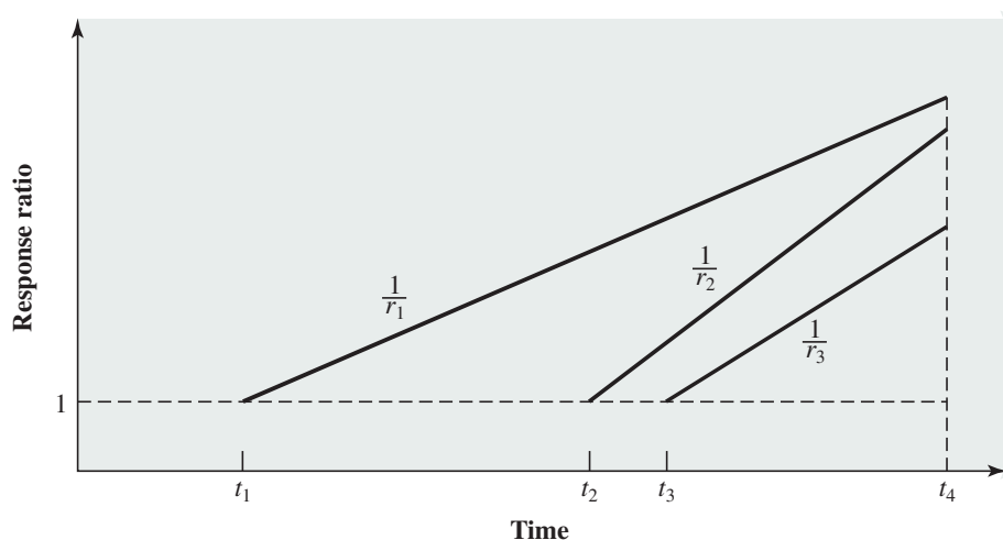
Figure 9.18 Response Ratio as a Function of Time
