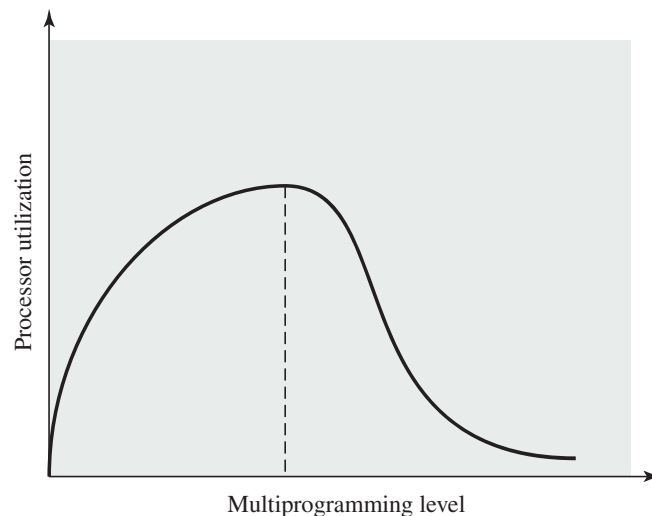
Figure 8.21 Multiprogramming Effects
