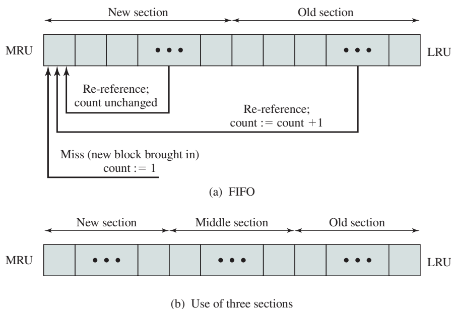
Figure 11.9 Frequency-Based Replacement
