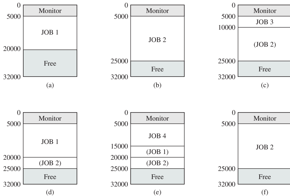
Figure 2.7 CTSS Operation
