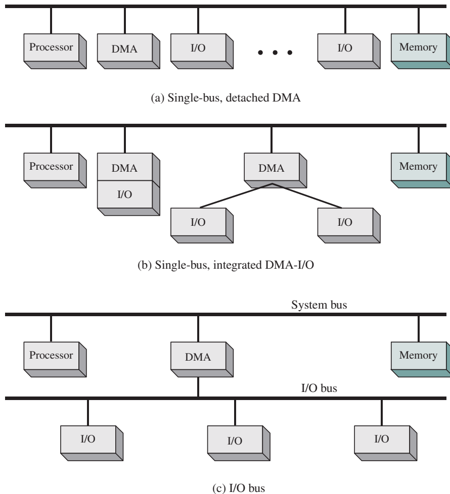
Figure 11.3 Alternative DMA Configurations
