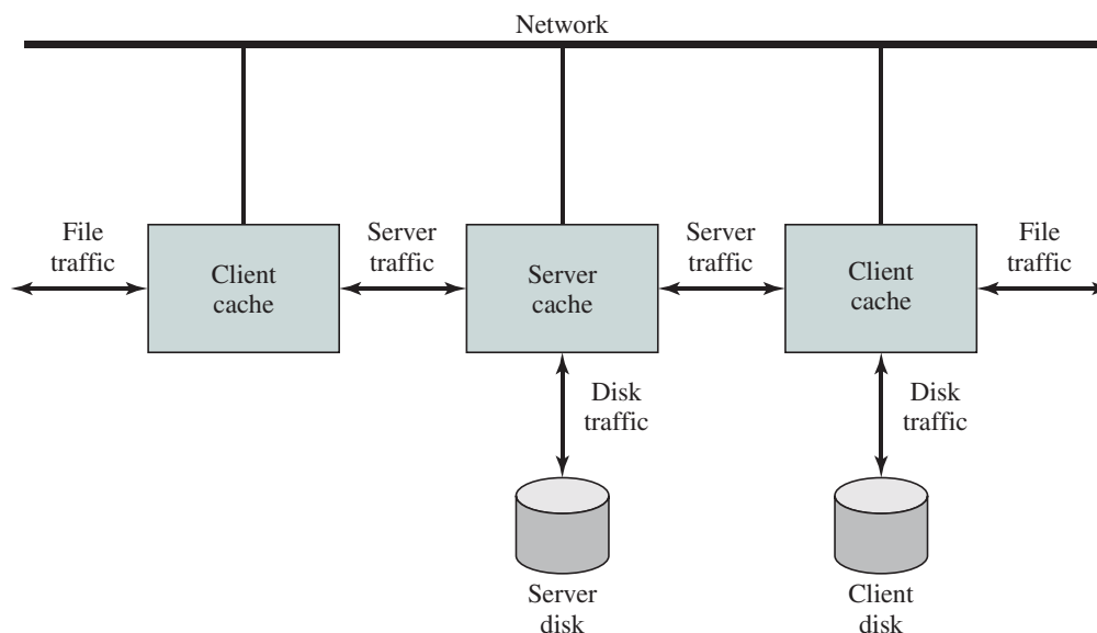
Figure 16.7 Distributed File Caching in Sprite
