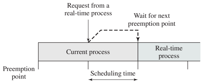
(c) Priority-driven preemptive scheduler on preemption points
