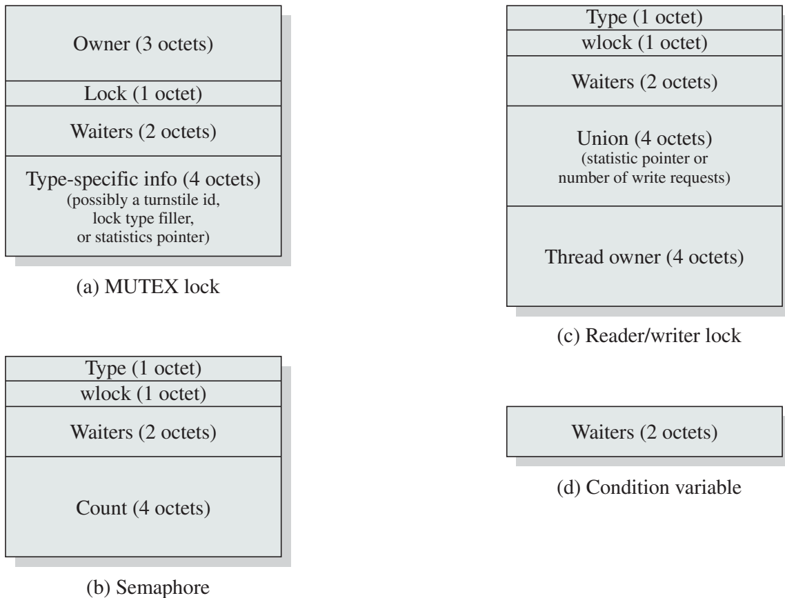
Figure 6.15 Solaris Synchronization Data Structures
