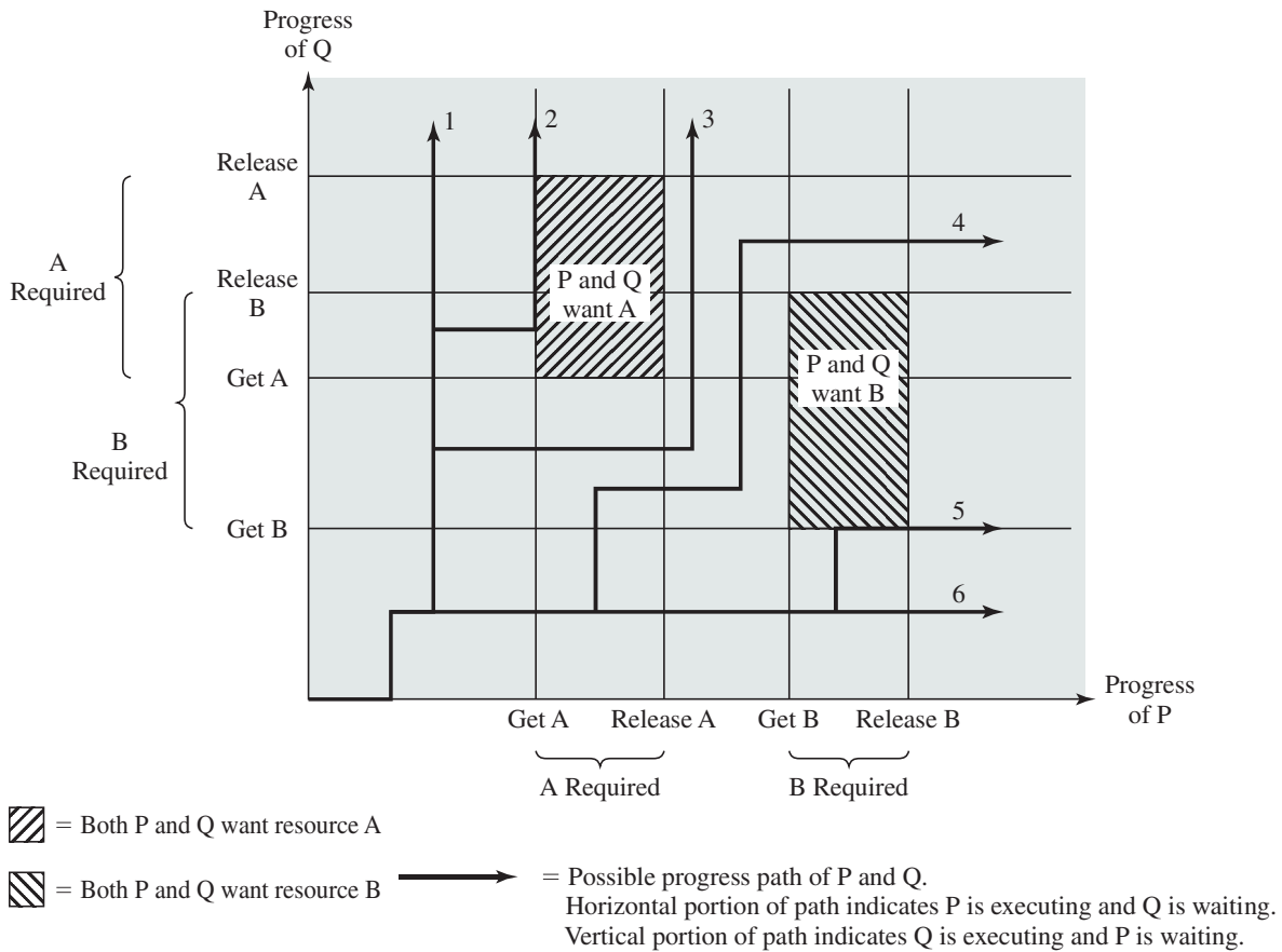
Figure 6.3 Example of No Deadlock [BACO03]
