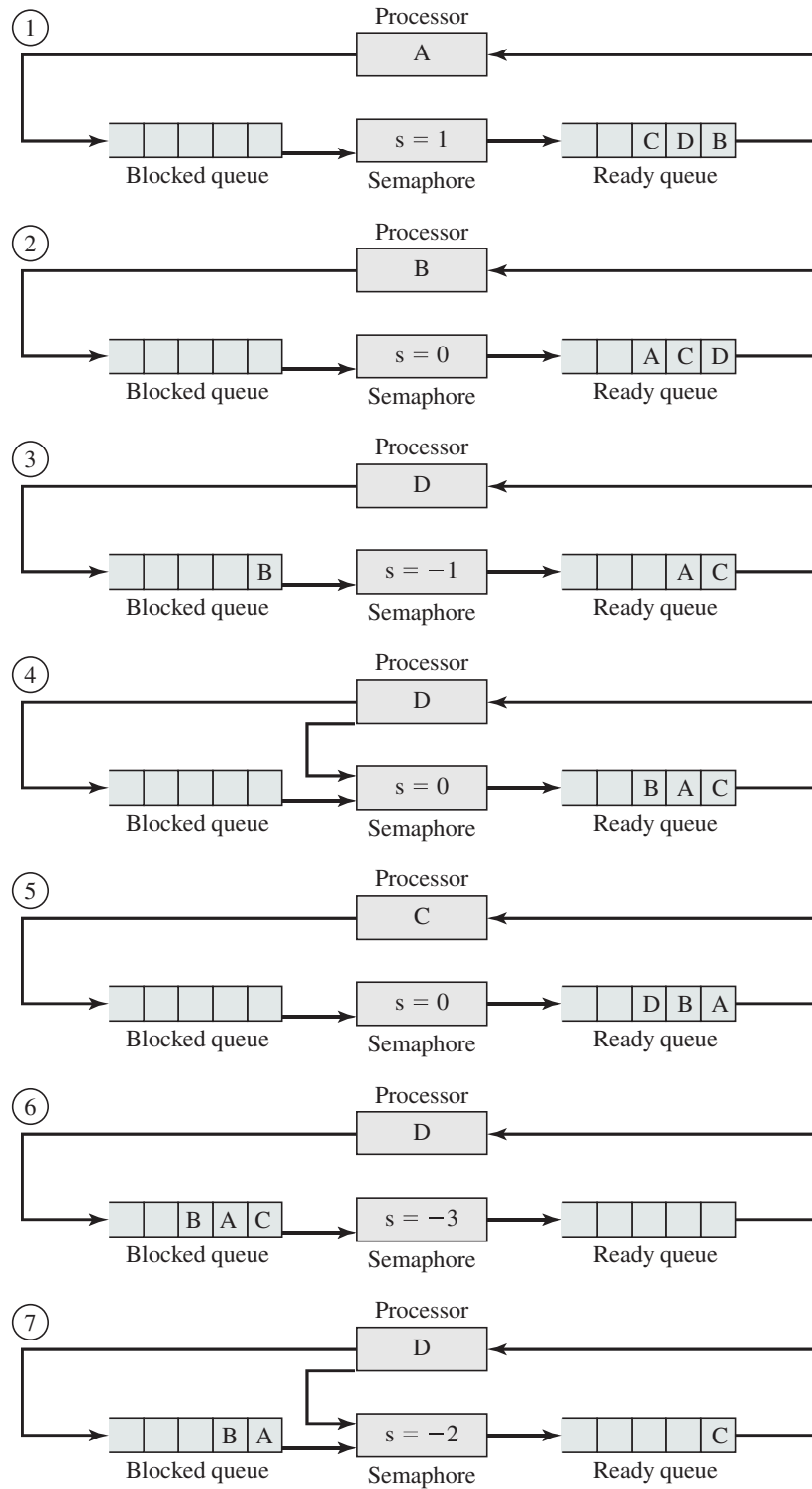
Figure 5.5 Example of Semaphore Mechanism
