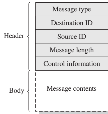
Figure 5.19 General Message Format
