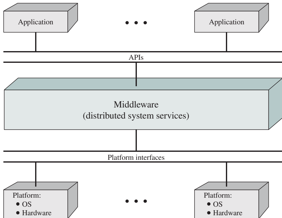
Figure 16.9 Logical View of Middleware
