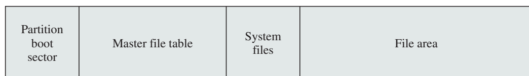
Figure 12.21 NTFS Volume Layout
