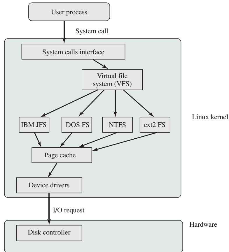
Figure 12.19 Linux Virtual File System Context
