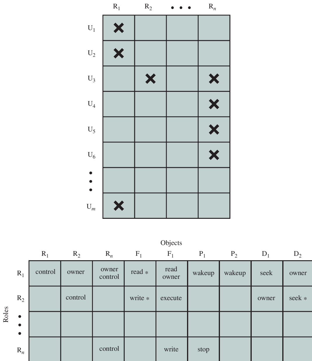
Figure 15.7 Access Control Matrix Representation of RBAC
