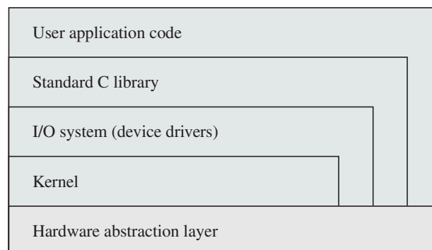
Figure 13.5 eCos Layered Structure
