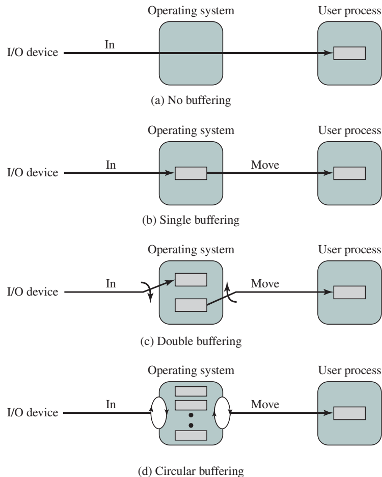
Figure 11.5 I/O Buffering Schemes (Input)
