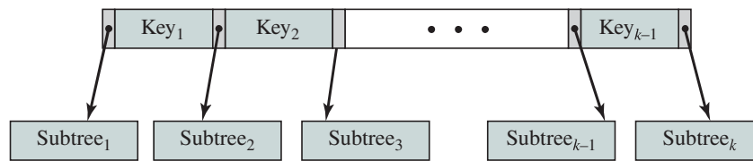
Figure 12.4 A B-tree Node with k Children
