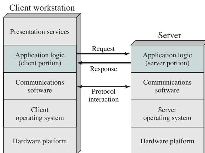
Figure 16.2 Generic Client/Server Architecture
