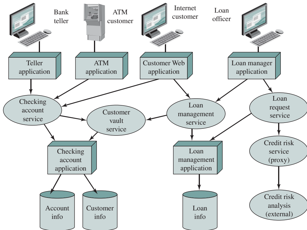
(b) An architecture reflecting SOA principles
