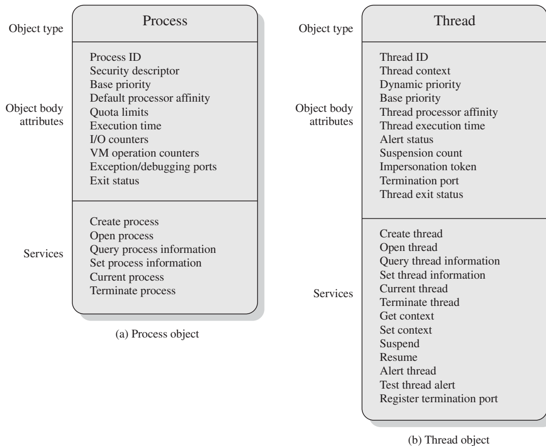
Figure 4.11 Windows Process and Thread Objects
