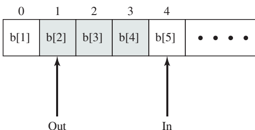
Figure 5.8 Infinite Buffer for the Producer/Consumer Problem
