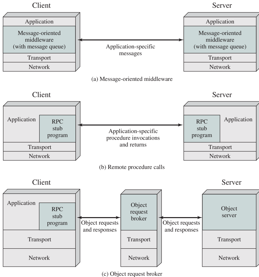
Figure 16.12 Middleware Mechanisms
