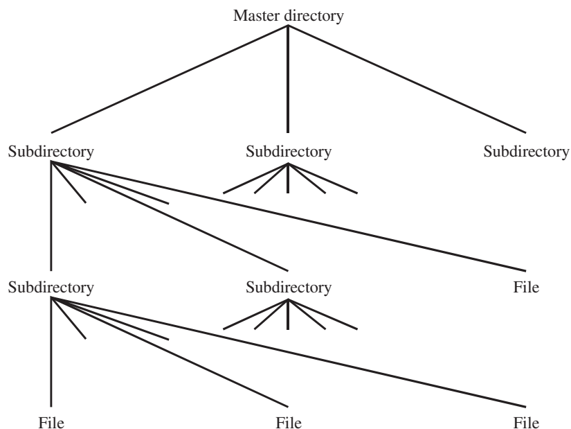
Figure 12.6 Tree-Structured Directory
