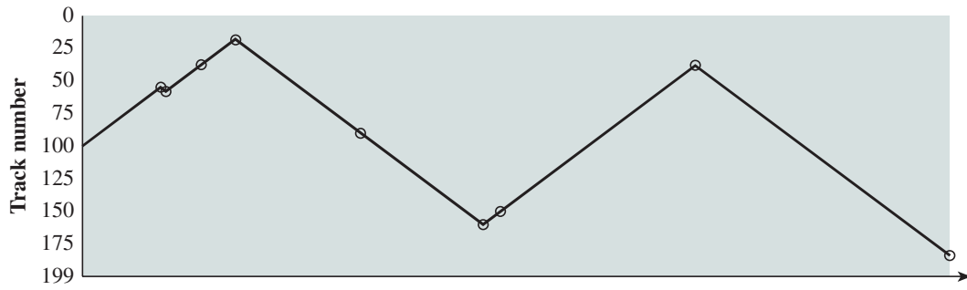
(a) FIFO
