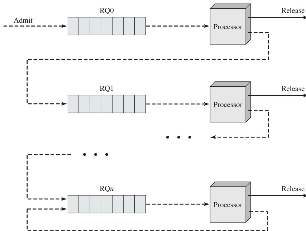
Figure 9.10 Feedback Scheduling
