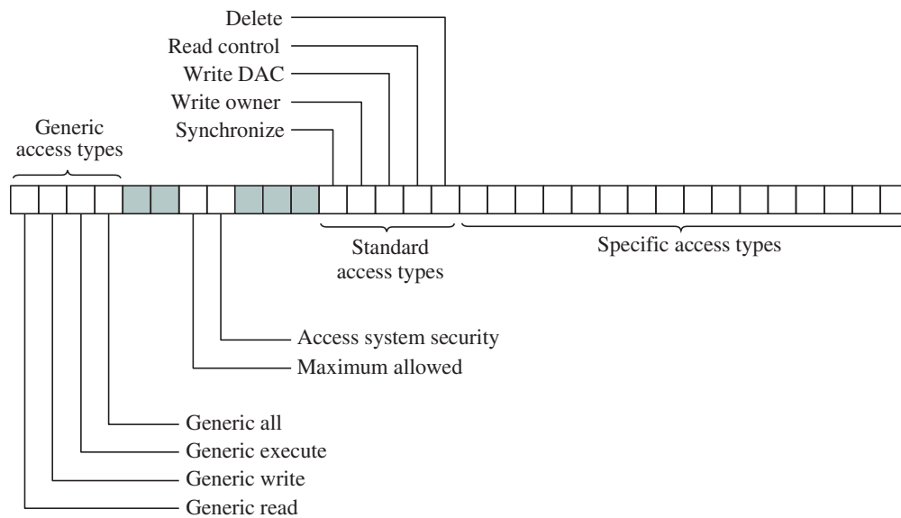
Figure 15.12 Access Mask
