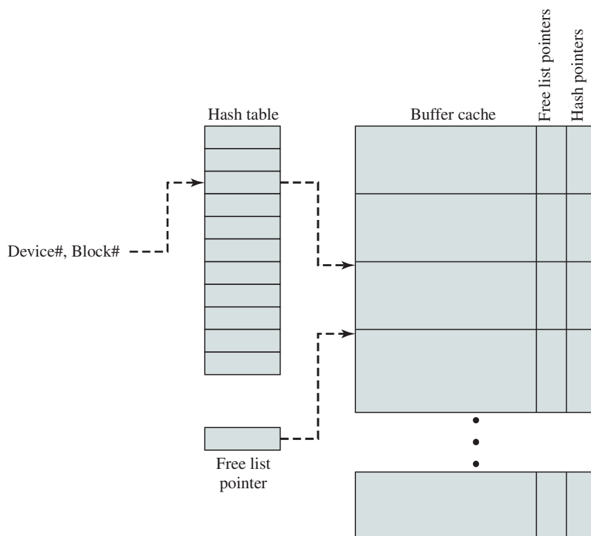
Figure 11.13 UNIX Buffer Cache Organization
