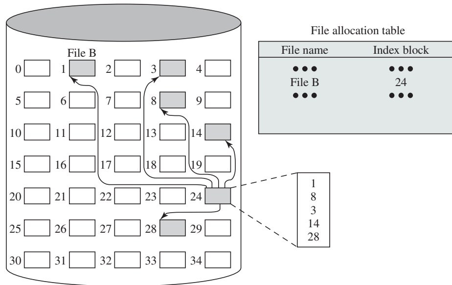
Figure 12.13 Indexed Allocation with Block Portions
