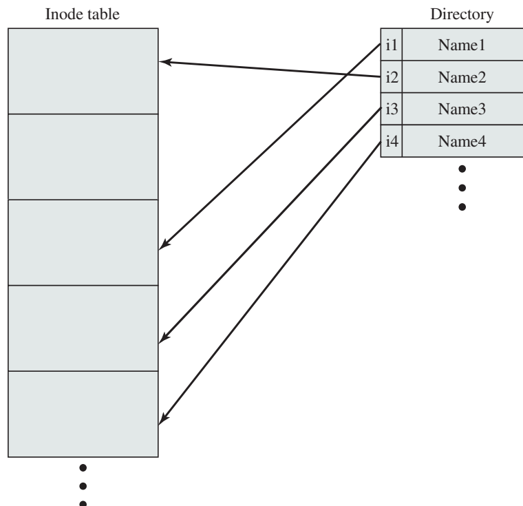
Figure 12.17 UNIX Directories and Inodes
