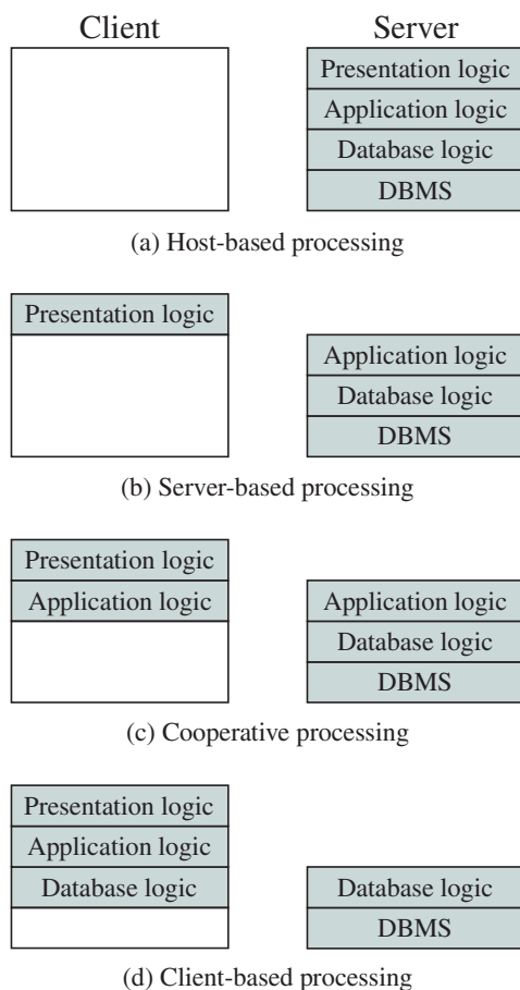
Figure 16.5 Classes of Client/Server Applications
