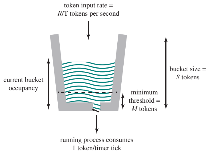
Figure 10.16 Linux VServer Token Bucket Scheme
