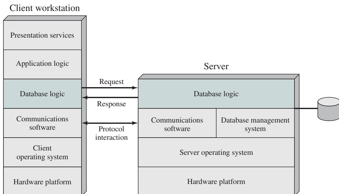
Figure 16.3 Client/Server Architecture for Database Applications
