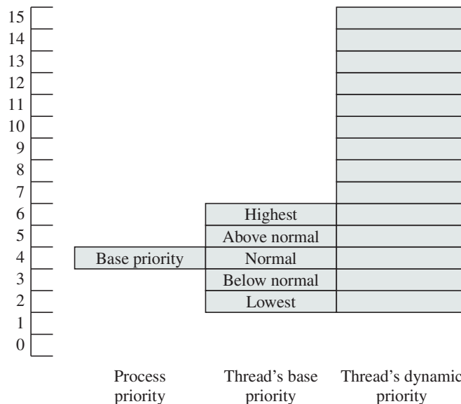
Figure 10.15 Example of Windows Priority Relationship
