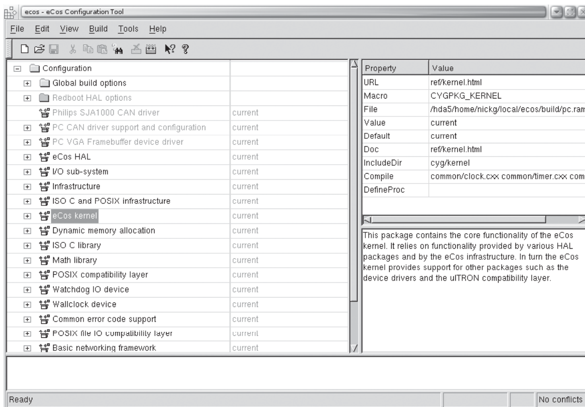
Figure 13.2 eCos Configuration Tool—Top Level
