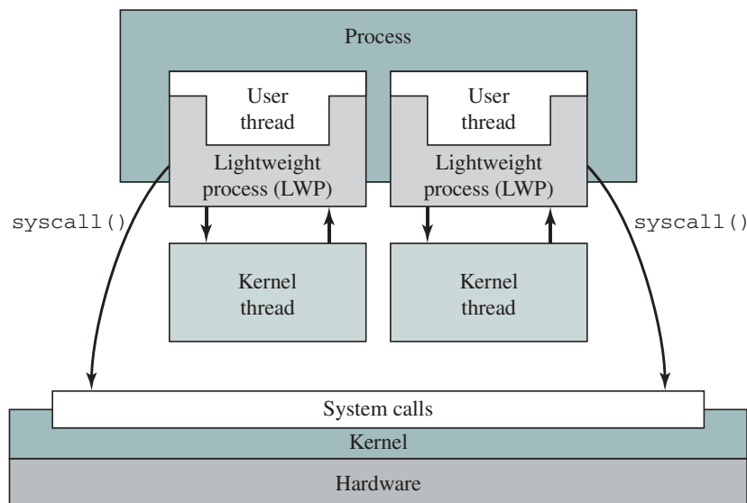
Figure 4.13 Processes and Threads in Solaris [MCDO07]
