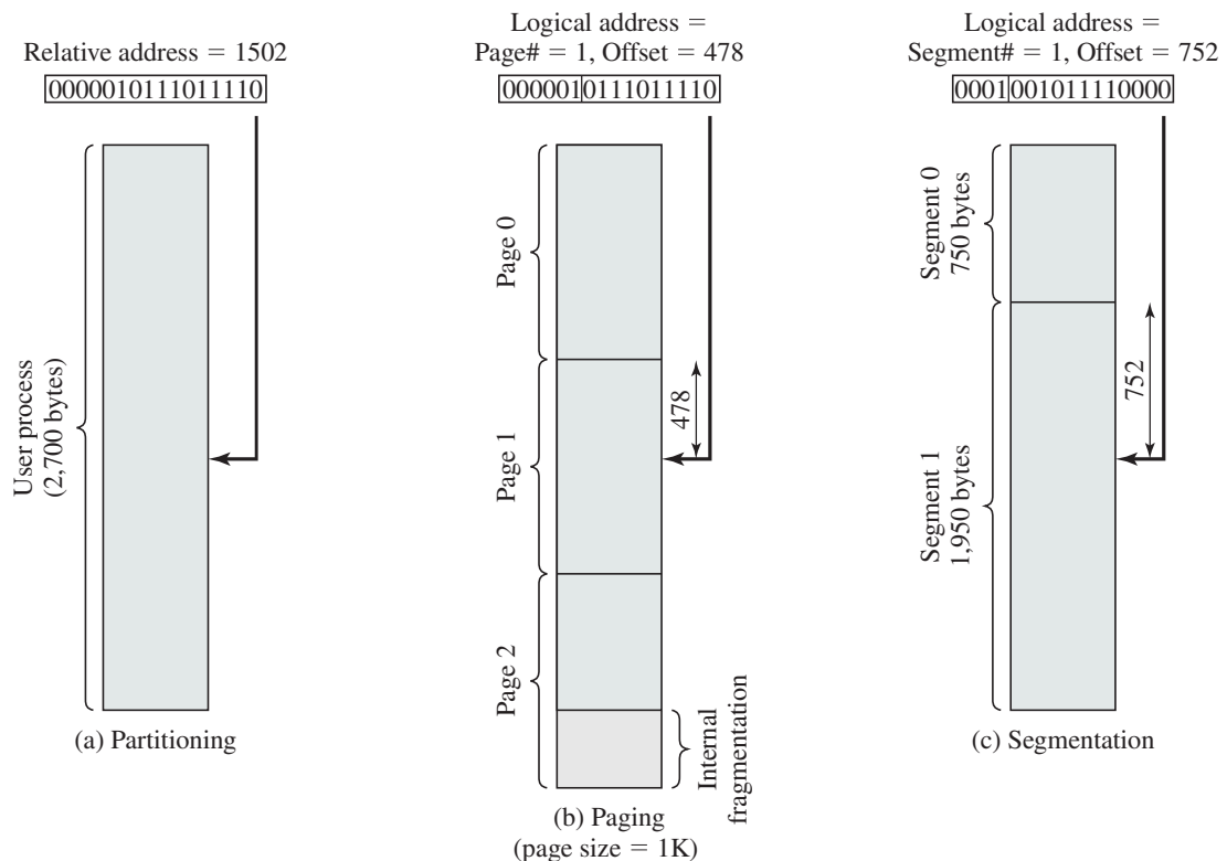
Figure 7.11 Logical Addresses
