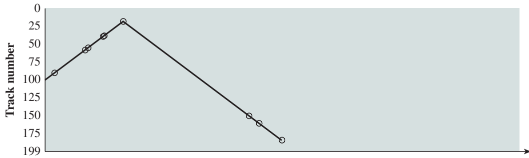
(b) SSTF
