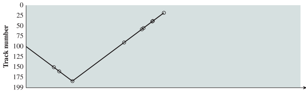
(c) SCAN
