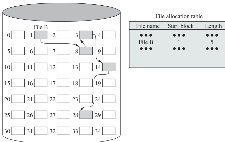
Figure 12.11 Chained Allocation
