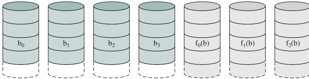
(c) RAID 2 (redundancy through Hamming code)
