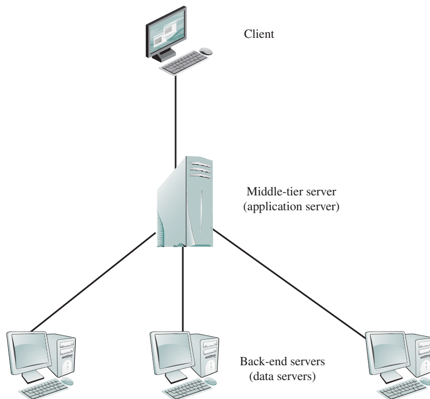
Figure 16.6 Three-Tier Client/Server Architecture
