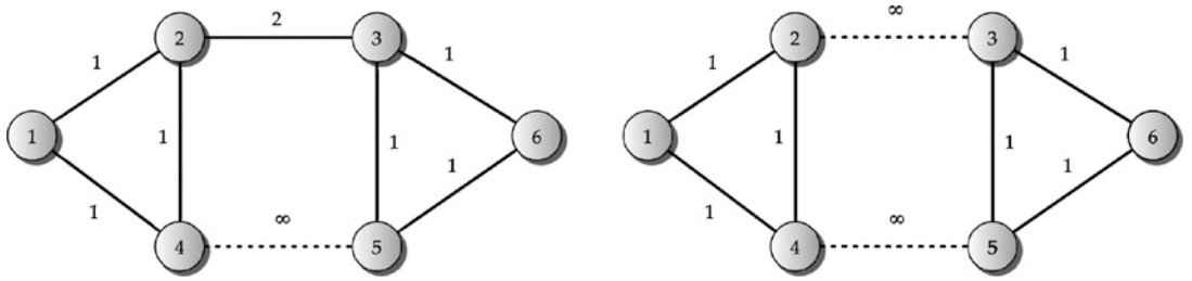
FIGURE 3.12 Six-node network: before and after failure of link 2-3 (assuming link 4-5 has already failed).
