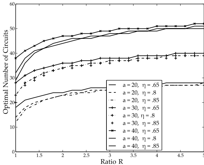
FIGURE 11.4 Determination of the optimal number of circuits using the ECCS method.
