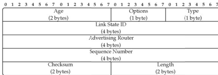
FIGURE 6.10 OSPF link state advertisement header.
