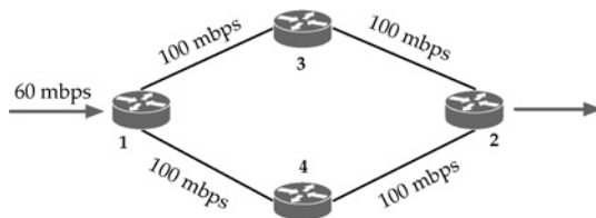
FIGURE 7.5 A four-node network example with the same link capacity.
