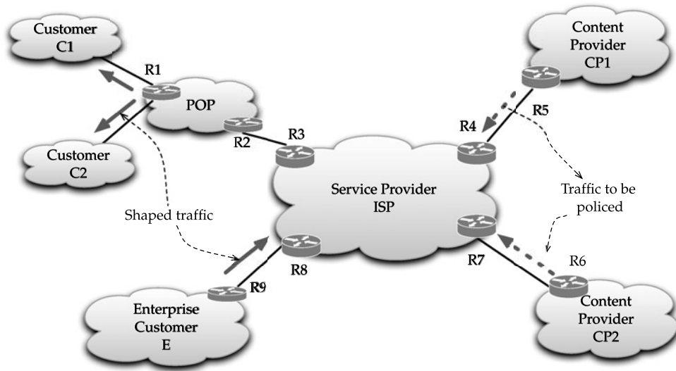
FIGURE 23.3 An ISP network.
