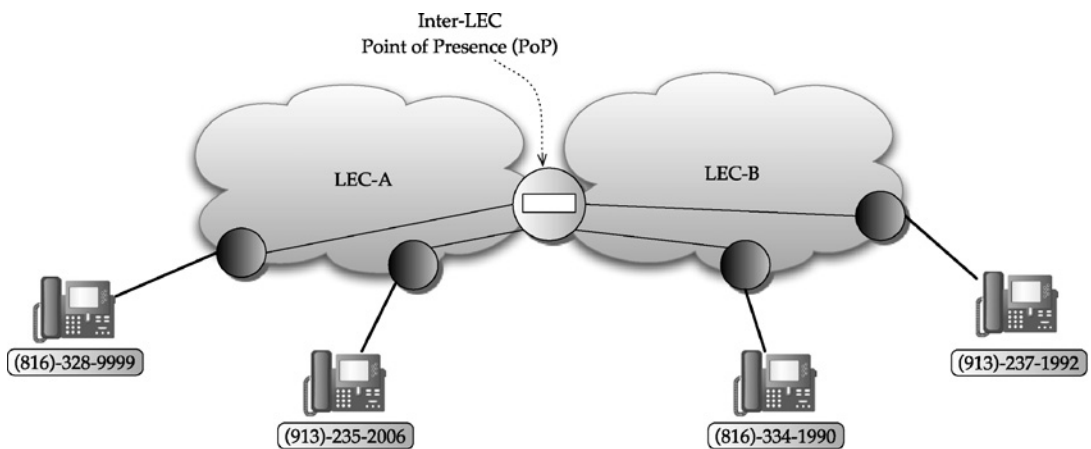
FIGURE 13.11 Inter-LEC connectivity through a PoP tandem switch.
