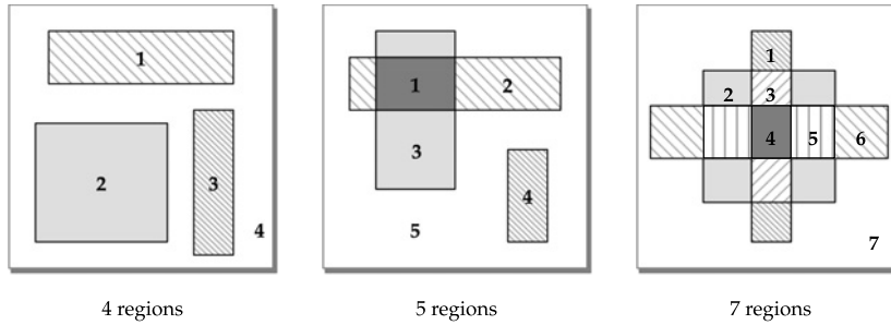
FIGURE 16.9 Possible arrangements of 3 rules in two dimensions (adapted from [273]).
