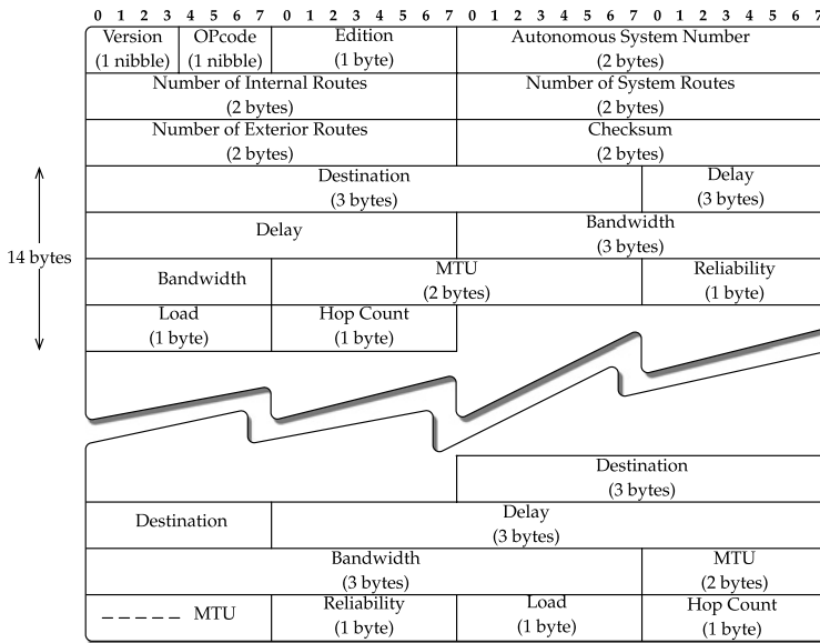
FIGURE 5.6 IGRP packet format.
