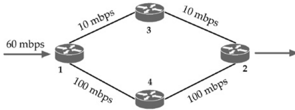
FIGURE 7.6 A four-node network example with different link capacity.
