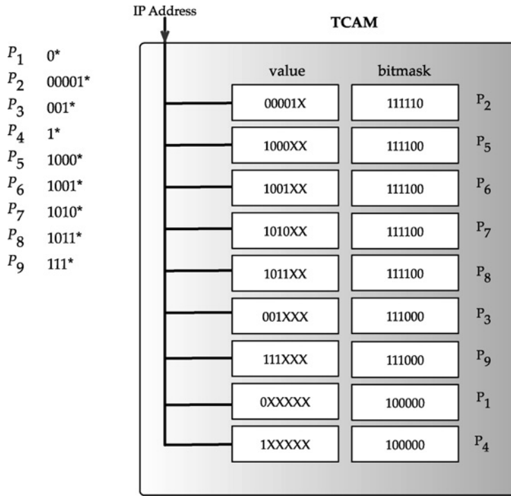
FIGURE 15.26 Storing the prefixes of Table 15.2 in TCAM.
