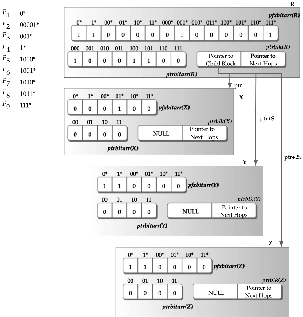
FIGURE 15.19 Tree bitmap data structure for the prefixes in Table 15.2.
