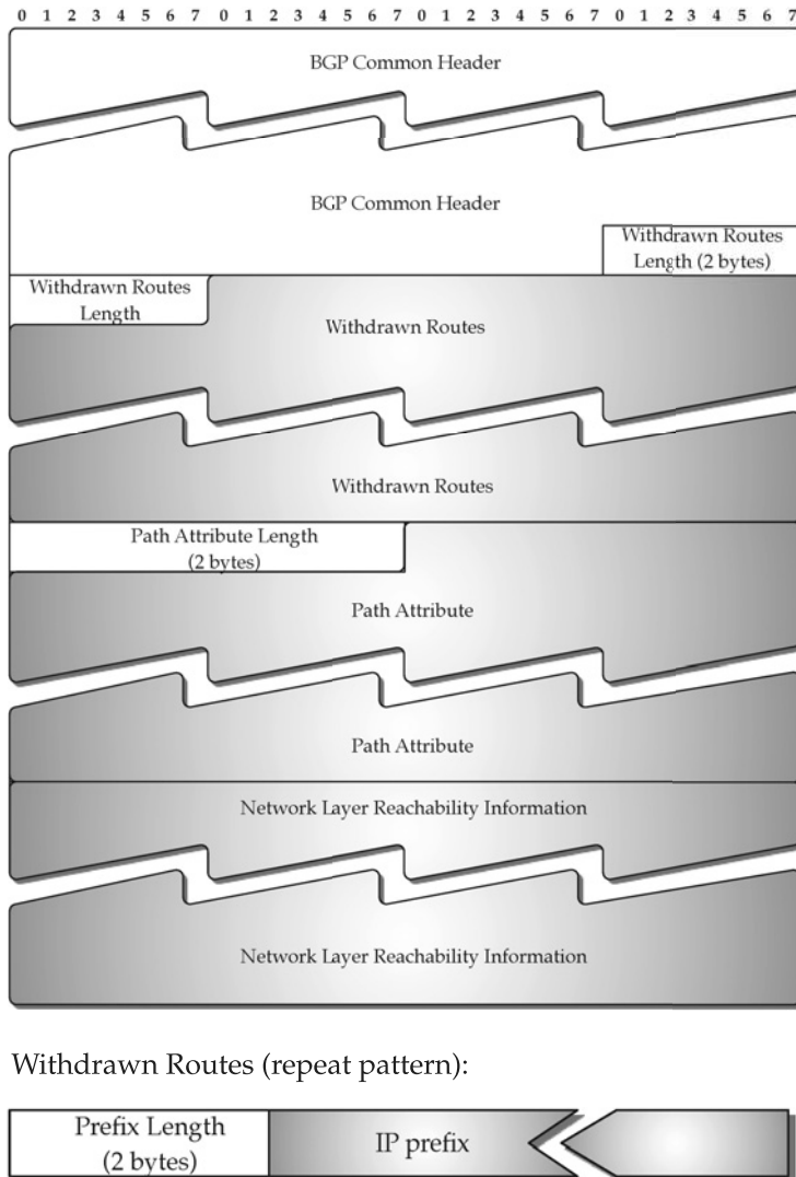
FIGURE 8.18 BGP4 UPDATE message.
