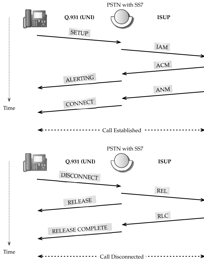
FIGURE 20.1 Call flow: setup and tear-down with Q.931 and SS7 ISUP.
