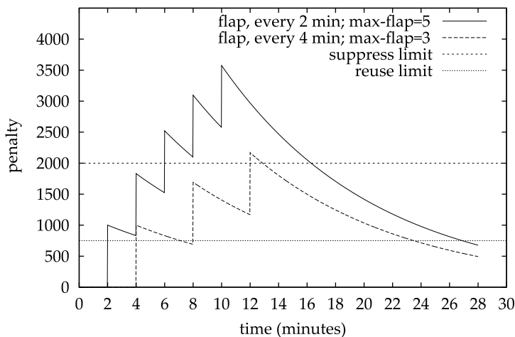
FIGURE 8.14 Route dampening figure-of-merit penalty.
