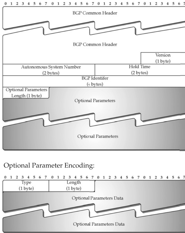
FIGURE 8.17 BGP4 OPEN message.
