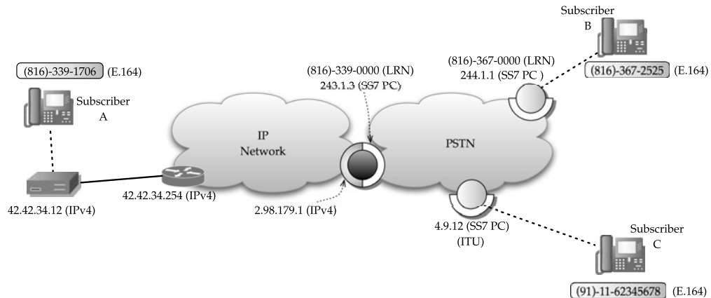
FIGURE 20.3 Addressing and call routing example.
