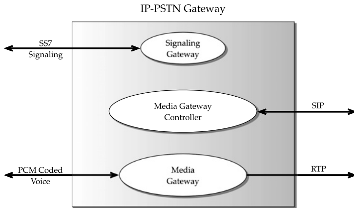
FIGURE 20.6 Gateway interfacing between PSTN and IP.
