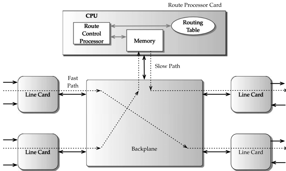
FIGURE 14.5 Router components.
