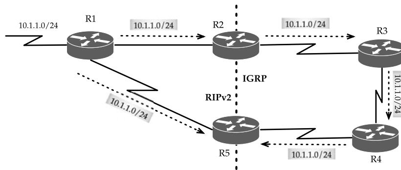
FIGURE 5.11 Route redistribution example with two routing protocols: RIPv2 and IGRP.
