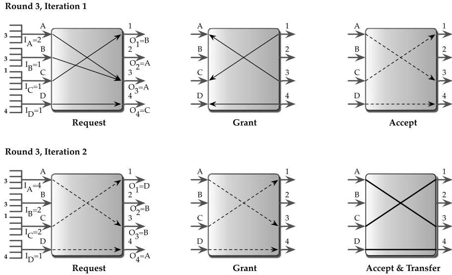
FIGURE 21.21 Two-iteration iSLIP scheduling in operation — round 3.
