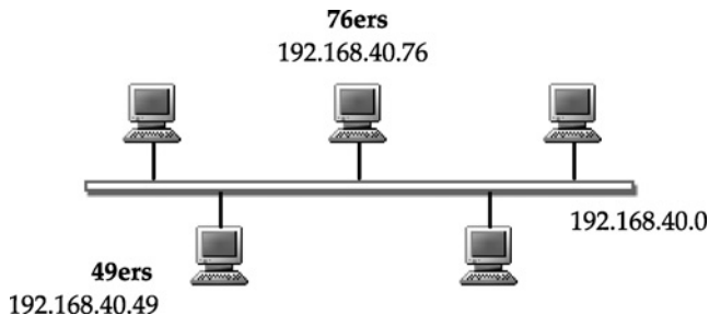
FIGURE 9.2 Host “49ers” (192.168.40.49) and Host “76ers” (192.168.40.76) on an Ethernet subnet with mask 255.255.255.0.
