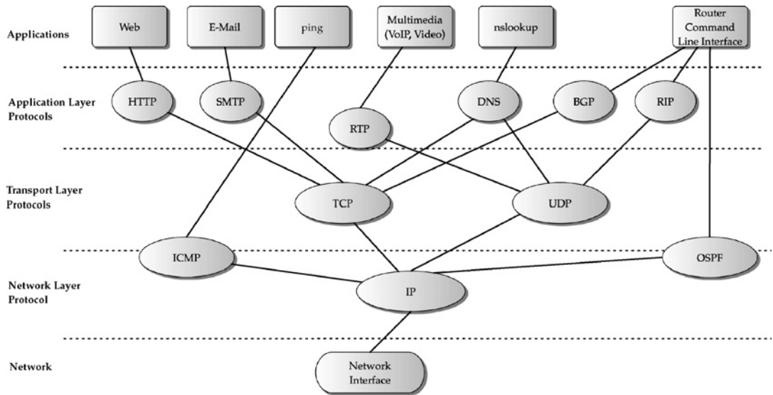
FIGURE 1.5 Protocol layering in IP architecture.
