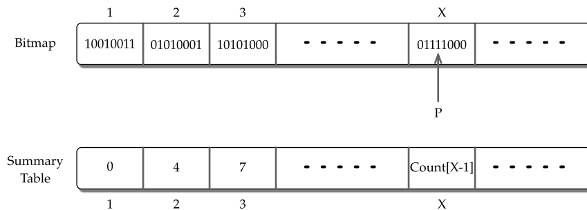
FIGURE 15.17 Counting the number of 1 bits up to position P .
