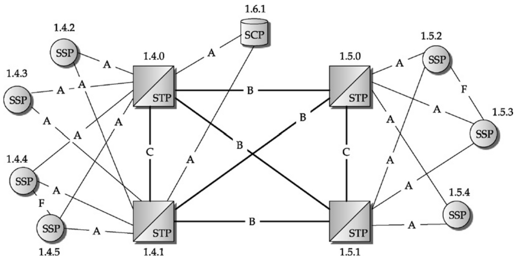
FIGURE 12.2 An SS7 network example with point codes identified.
