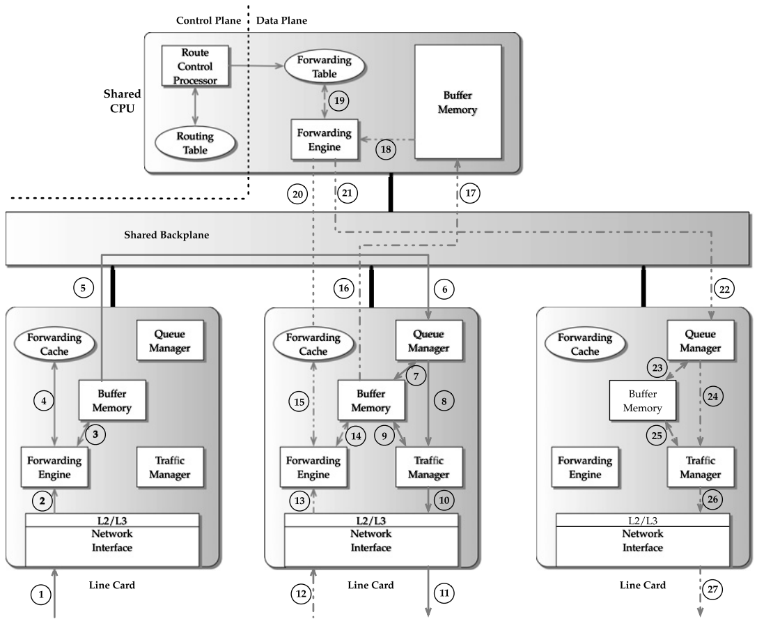
FIGURE 14.7 Shared CPU architecture with route caches.
