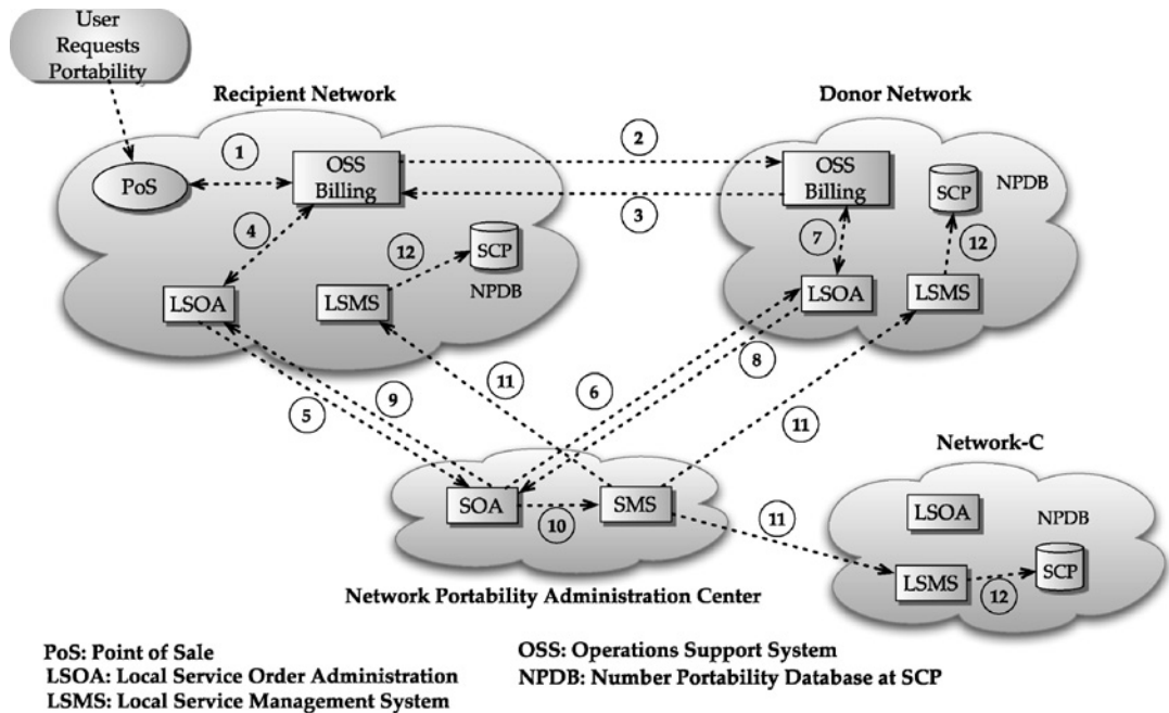
FIGURE 13.15 Number portability architecture: initial porting from a donor network to a recipient network.
