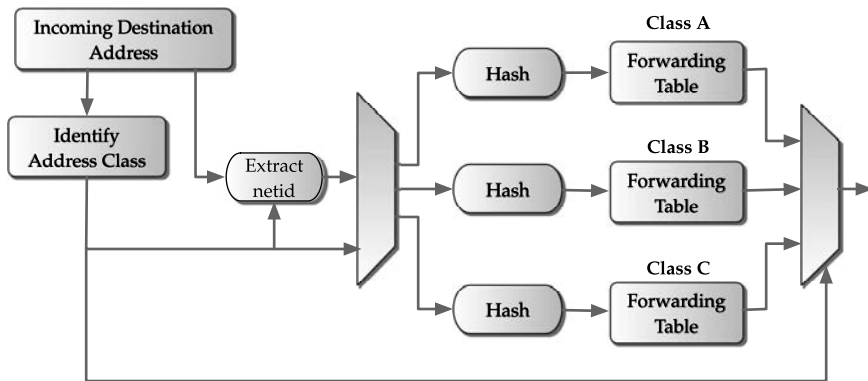
FIGURE 15.1 Lookup operation in a classful IP addressing scheme (adapted from [273]).
