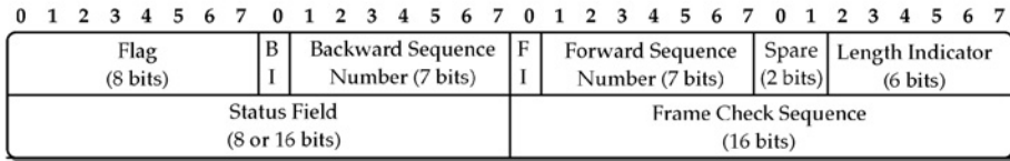
(b) Link Status Signaling Unit (LSSU)
