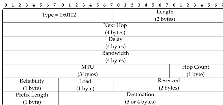
FIGURE 5.10 EIGRP: TLV type for communicating distance vector of an internal route.
