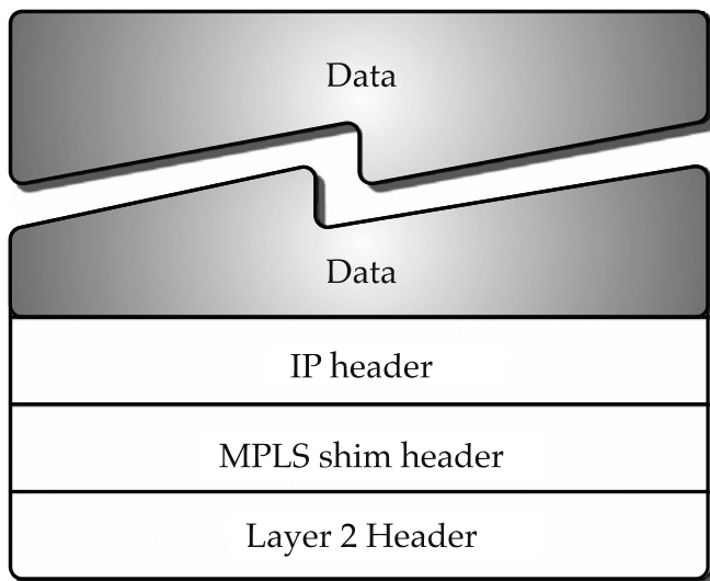
FIGURE 18.2 MPLS header as layer 2.5.
