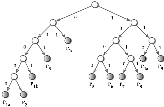
FIGURE 15.7 Disjoint prefix (leaf pushed) binary trie.
