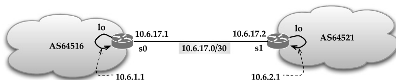
FIGURE 8.4 BGP session setup: use loopback interface between two ASes.
