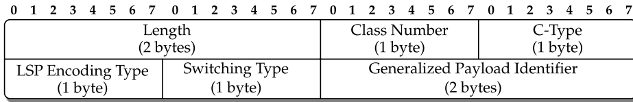
FIGURE 18.14 RSVP-TE generalized label request object for GMPLS.
