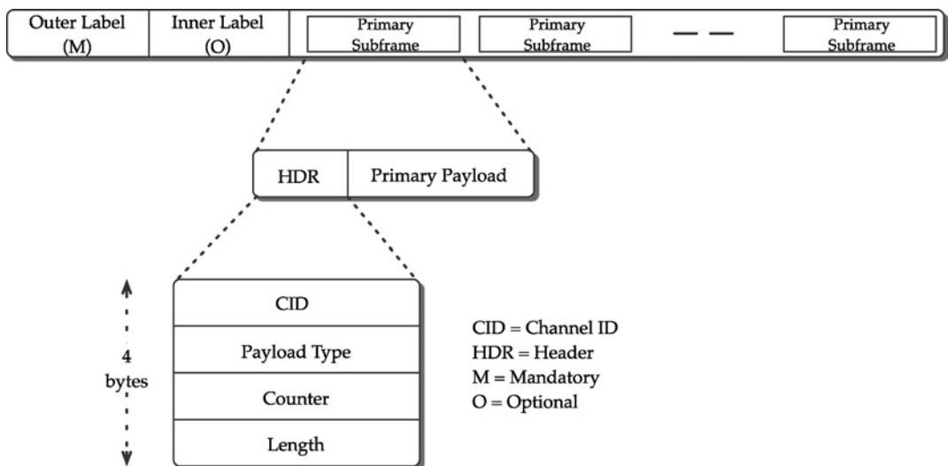
FIGURE 19.3 LSP Structure in VoMPLS (adapted from [487]).
