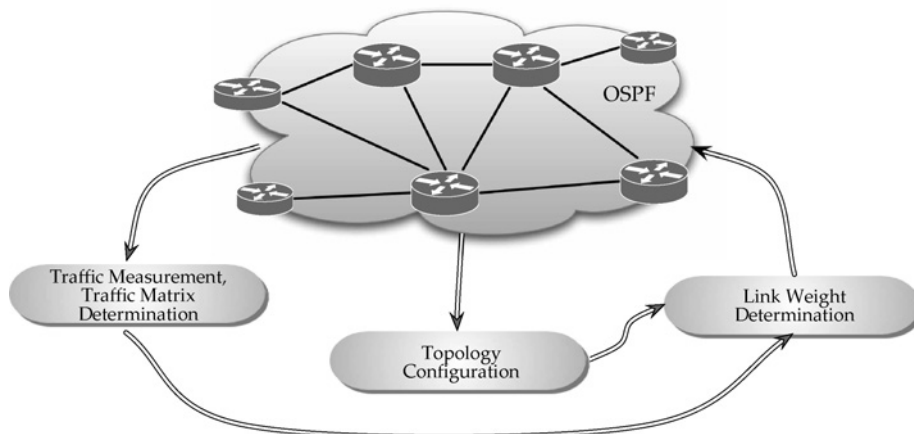
FIGURE 7.3 IP traffic engineering: an architectural framework.
