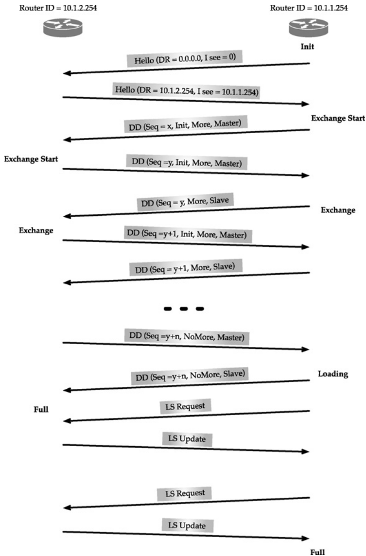
FIGURE 6.2 OSPF link state database synchronization process (based on [505]).
