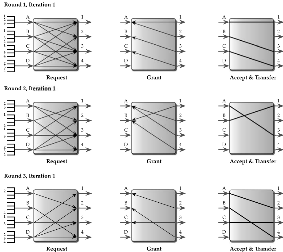
FIGURE 21.15 Single-iteration PIM in operation.
