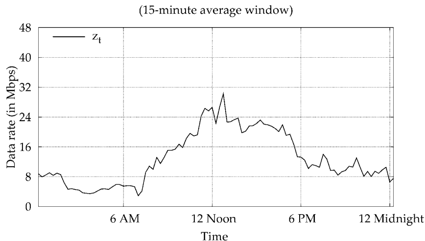
FIGURE 7.2 Traffic data rate over a 24-hour period.
