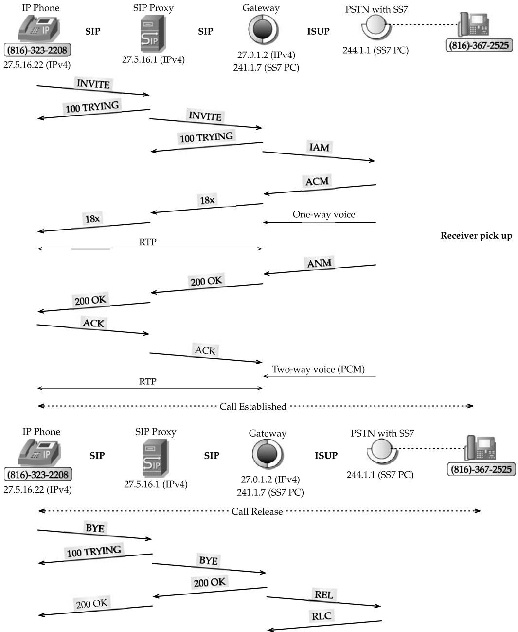
FIGURE 20.7 Call flow example from SIP phone to PSTN.
