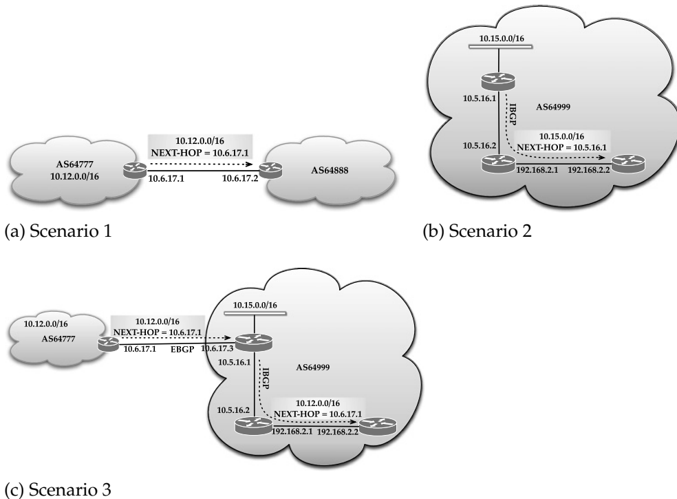
FIGURE 8.7 BGP path attribute: NEXT-HOP examples.
