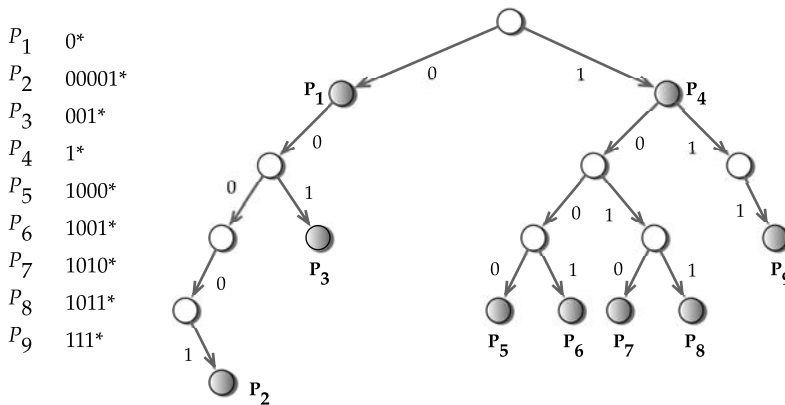
FIGURE 15.3 Binary trie data structure for the prefixes of Table 15.2.
