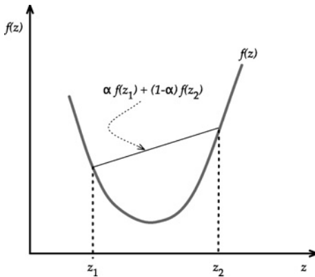
FIGURE 4.7 Convex function.
