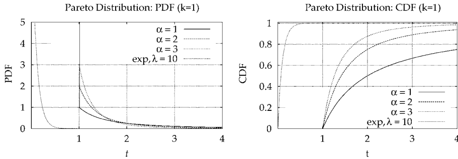
FIGURE B.4 PDF and CDF of Pareto distribution (including exponential with \lambda = 10 ).
