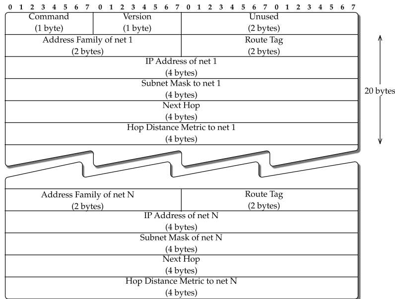
FIGURE 5.4 IPv2 packet format.
