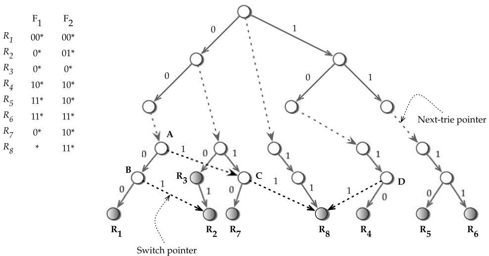
FIGURE 16.6 Using switch pointers to speed up search in grid-of-tries data structure.
