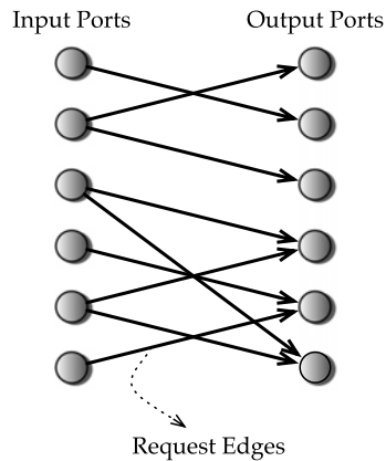
FIGURE 21.12 Equivalence of scheduling and bipartite matching.
