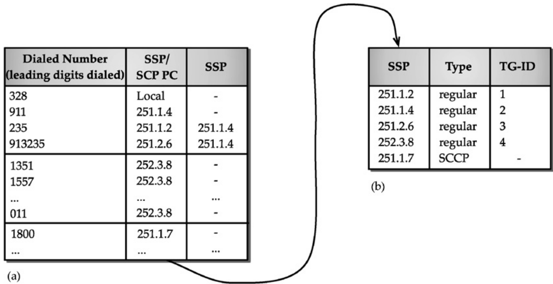
FIGURE 13.3 Call routing decision: conceptual view through table lookup.
