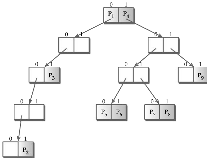
FIGURE 15.5 Implementation of the binary trie shown in Figure 15.3.
