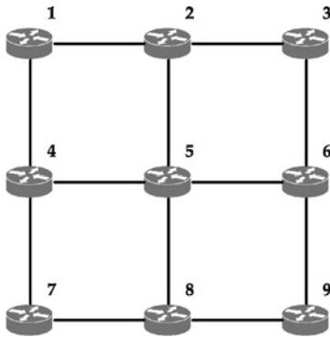
FIGURE 4.9 A nine-node Manhattan street network.
