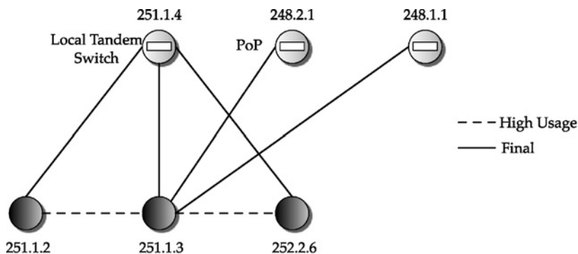
FIGURE 13.6 Hierarchical routing view at the TDM switch level in a LEC/IXC environment.
