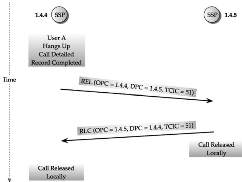
FIGURE 12.8 ISUP call tear-down message exchanges.
