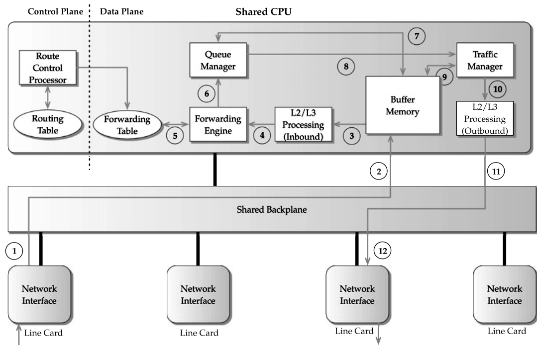
FIGURE 14.6 Shared CPU architecture.
