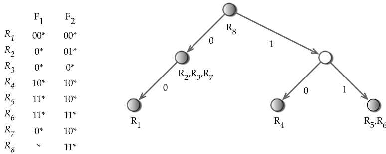
FIGURE 16.2 Constructing the F_1 trie needed for a hierarchical trie.
