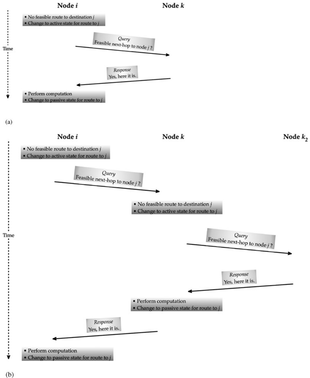
FIGURE 3.7 Request/response handling in a loop-free distance vector protocol.
