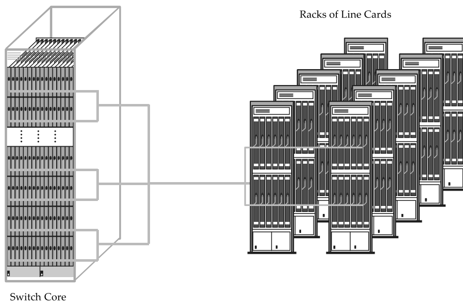
FIGURE 14.11 Clustered router architecture with a central switch core (adapted from [569]).
