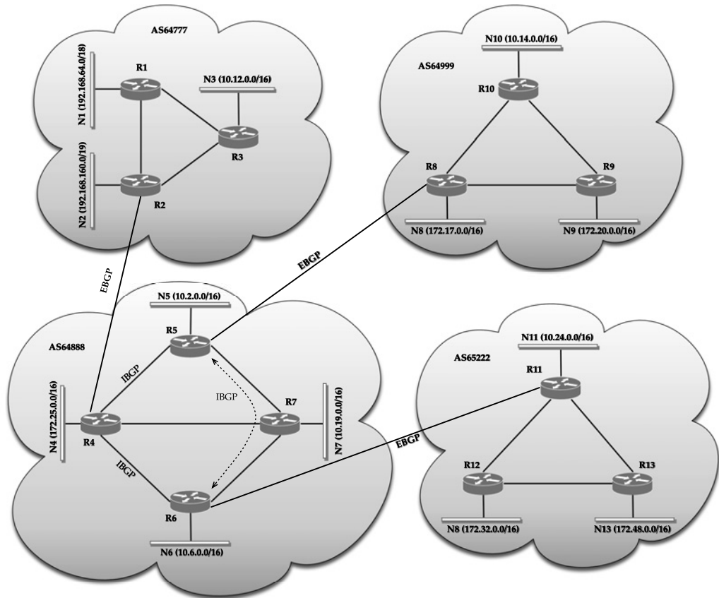
FIGURE 8.5 External BGP and internal BGP example.
