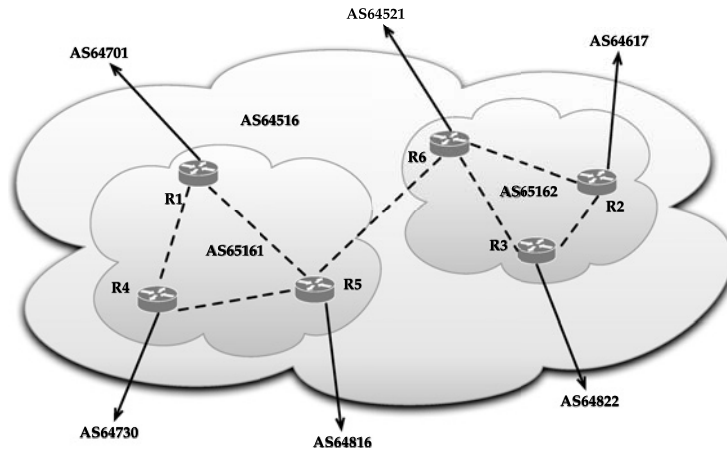
FIGURE 8.13 IBGP confederation example.
