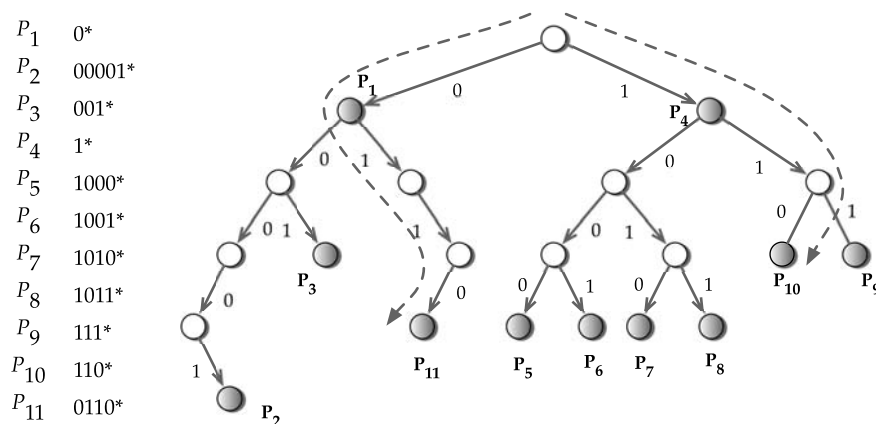
FIGURE 15.4 Inserting new prefixes in a binary trie.
