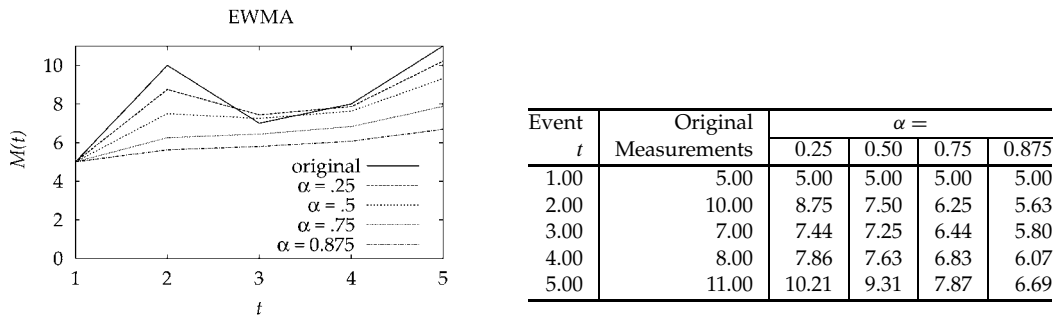
FIGURE B.2 Exponential weighted moving average.
