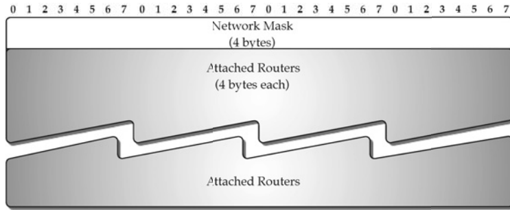
FIGURE 6.12 OSPF Network LSA content (LSA type = 2).
