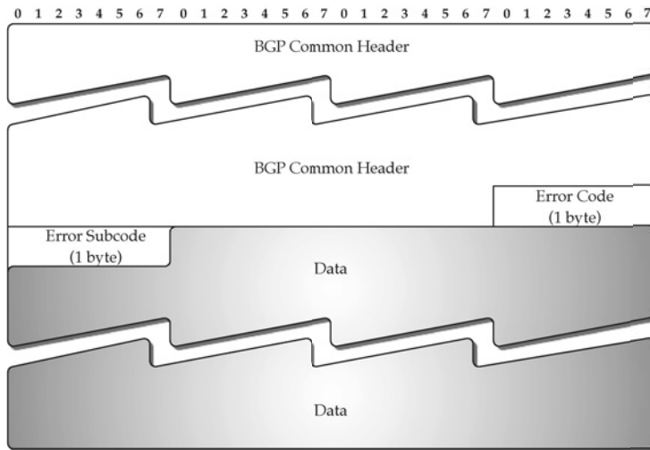
FIGURE 8.19 BGP4 NOTIFICATION message.
