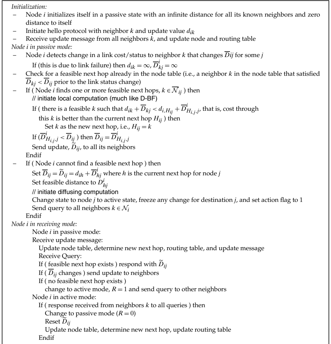
FIGURE 3.8 Loop-free distance vector protocol based on diffusing computation with coordinated update (node i 's view).
