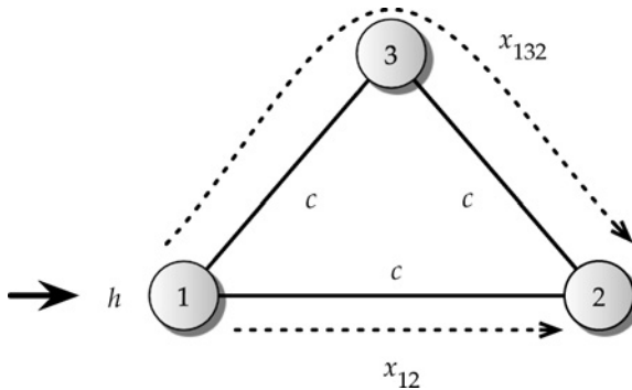
FIGURE 4.2 Single-commodity network flow modeling: three-node network.
