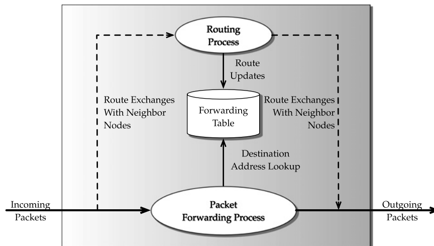
FIGURE 14.1 Routing and packet forwarding process.
