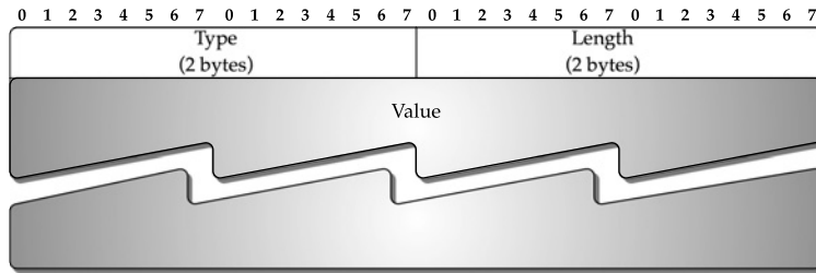
FIGURE 5.8 Data encoding in EIGRP packet: Generic TLV format.
