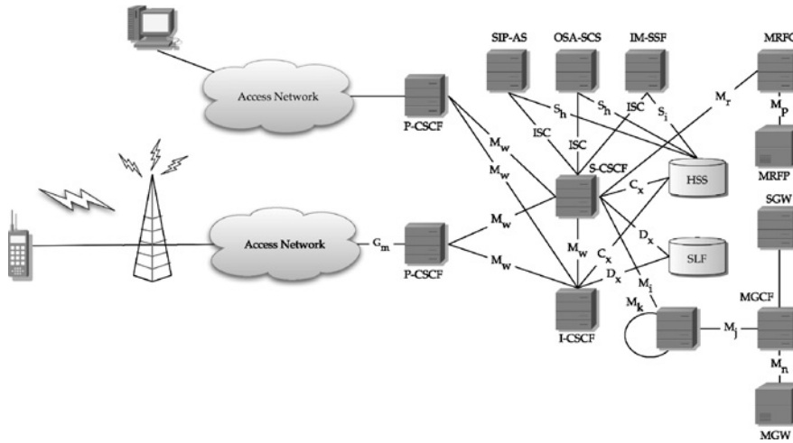
FIGURE 20.10 IMS architecture.
