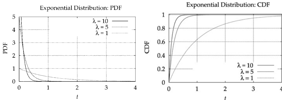
FIGURE B.3 PDF and CDF of the exponential distribution.
