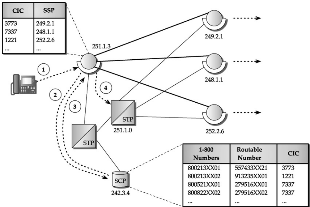
FIGURE 13.9 Lookup up for 1-800 number routing.
