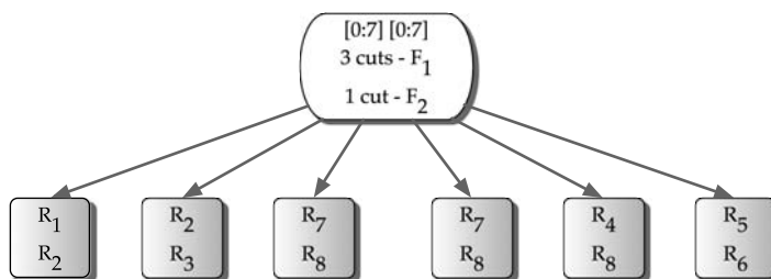
FIGURE 16.26 HyperCuts decision tree for rules in Table 16.2.
