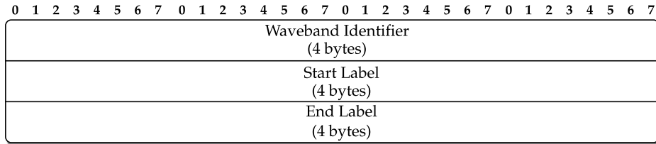
FIGURE 18.12 GMPLS label for wavelength switching.
