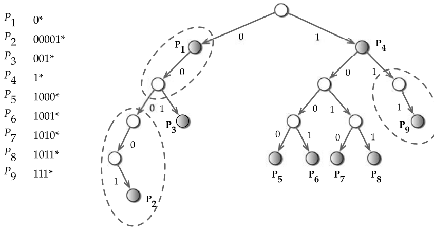
FIGURE 15.12 Identifying the paths to be compressed in the binary trie shown in Figure 15.3.
