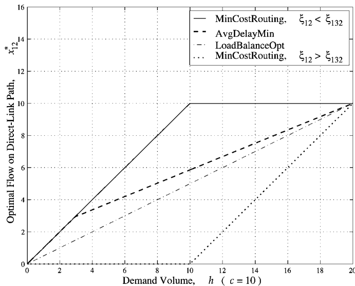
FIGURE 4.3 Optimal flow on the direct link path with different objectives.
