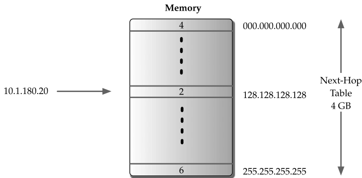
FIGURE 15.25 RAM based lookup.
