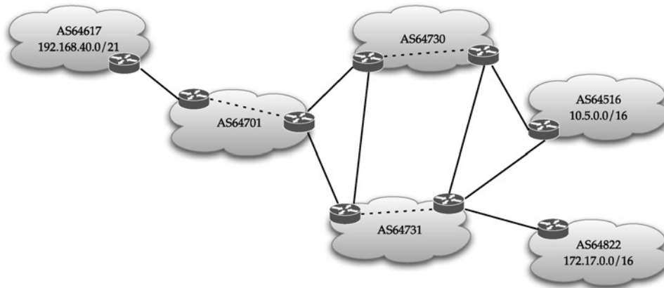
FIGURE 9.5 AS routing path of a packet from 192.168.40.0/21 to 10.5.0.0/16 through intermediate ASes.
