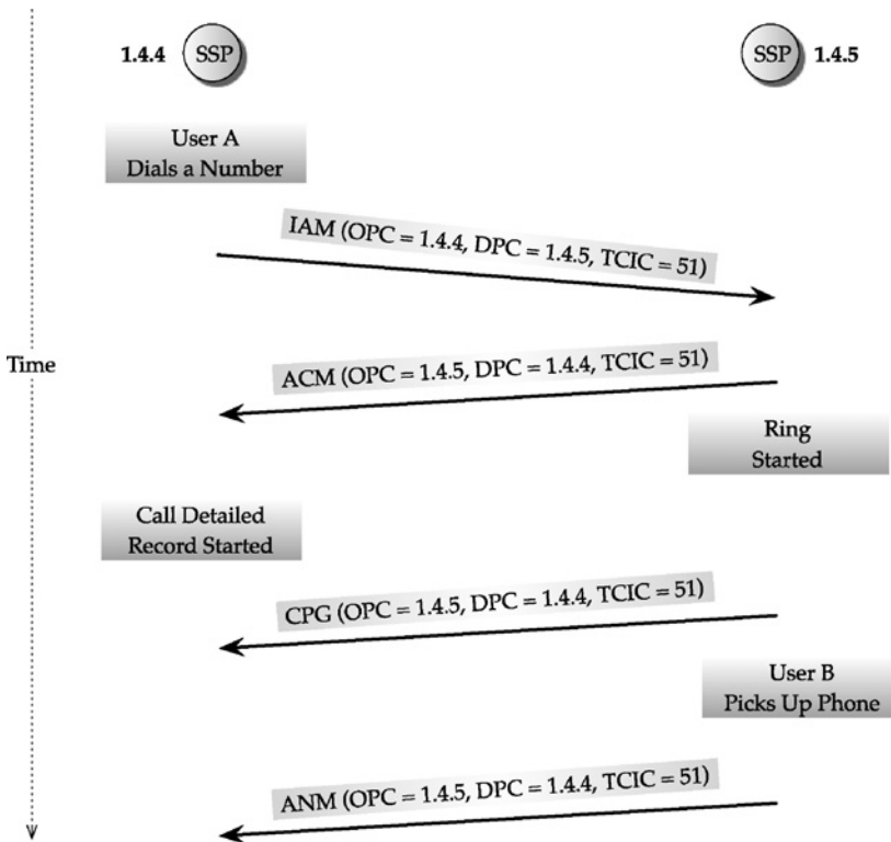
FIGURE 12.7 ISUP call setup message exchanges.
