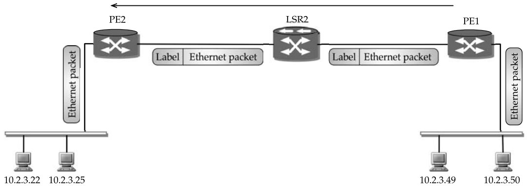
FIGURE 18.19 Layer 2 VPN over MPLS.
