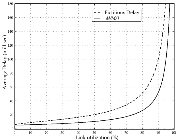
FIGURE 7.1 The M/M/1 average delay curve along with a fictitious delay curve.
