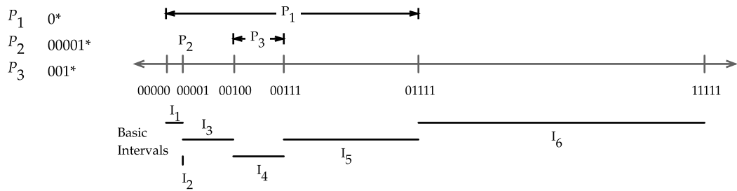
FIGURE 15.23 Prefix intervals identified by three prefixes 0^* , 00001^* and 001^* .
