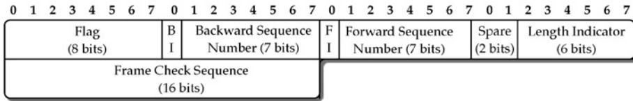
(a) Fill-In Signaling Unit (FISU)
