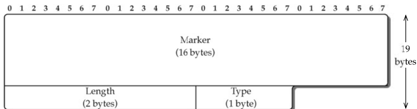
FIGURE 8.16 BGP4 common header.
