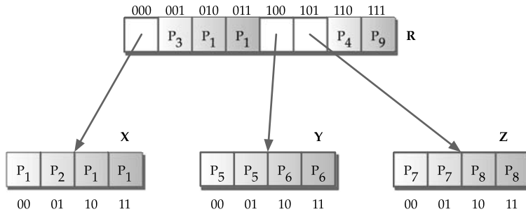
FIGURE 15.15 Implementation of leaf pushed fixed stride multibit trie for the trie in Figure 15.8.
