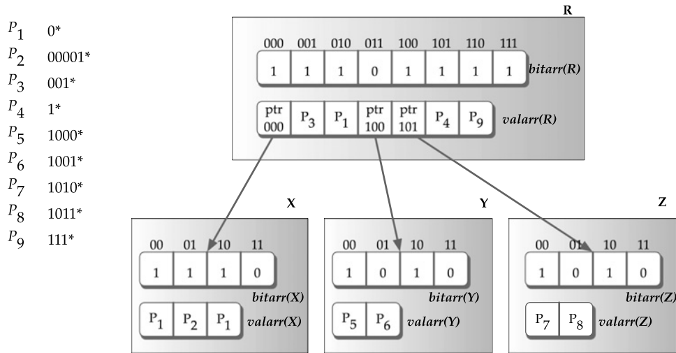
FIGURE 15.16 Lulea compressed trie data structure for the prefixes in Table 15.2.
