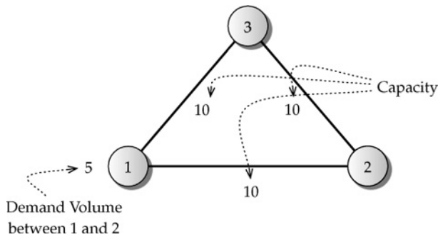
FIGURE 4.1 Three-node network with single demand between node 1 and node 2.
