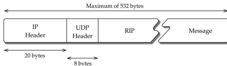
FIGURE 5.2 RIPv1 message structure, with IP and UDP header.
