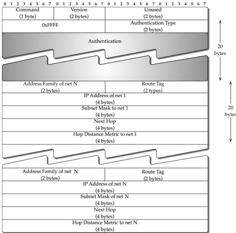
FIGURE 5.5 RIPv2 packet format with authentication.
