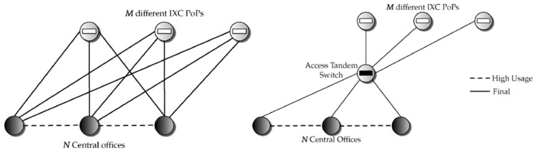
FIGURE 13.10 LEC/IXC access topology scenarios: (a) full connectivity requires N \times M trunkgroups, (b) access-tandem based connectivity requiring N + M trunkgroups (“hub-and-spoke topology”).
