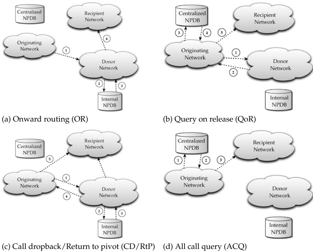
FIGURE 13.16 Call routing schemes, with number portability.
