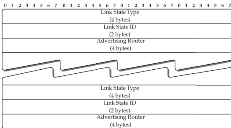
FIGURE 6.8 OSPF link state request packet (OSPF packet type = 3).
