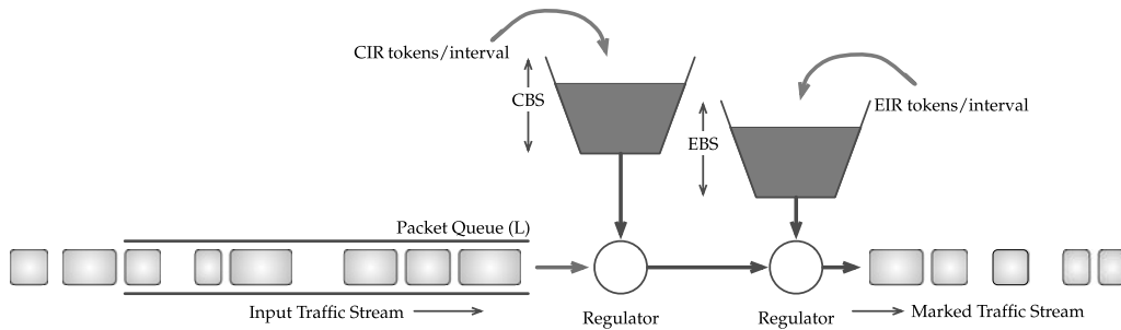
FIGURE 23.12 Two-rate three-color marking.
