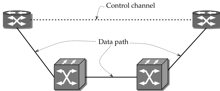
FIGURE 18.15 Control and data path separation in GMPLS.
