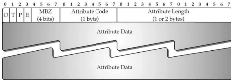
FIGURE 8.21 Path Attribute in UPDATE message.
