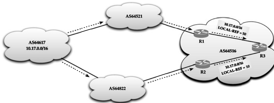
FIGURE 8.9 BGP path attribute: LOCAL-PREF example.
