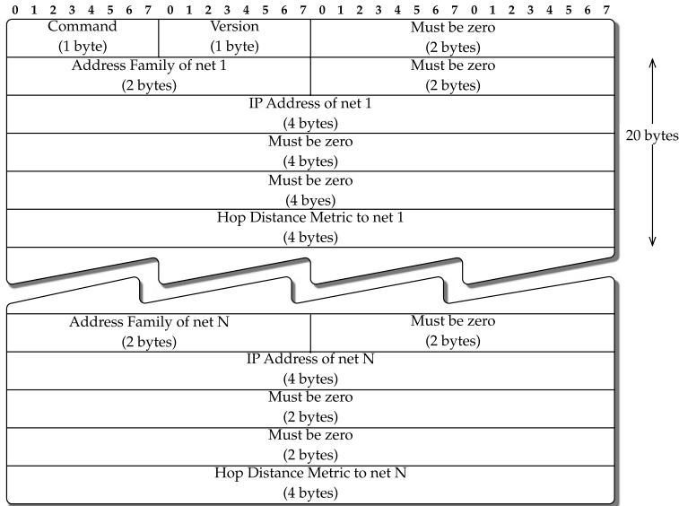
FIGURE 5.3 RIPv1 packet format.
