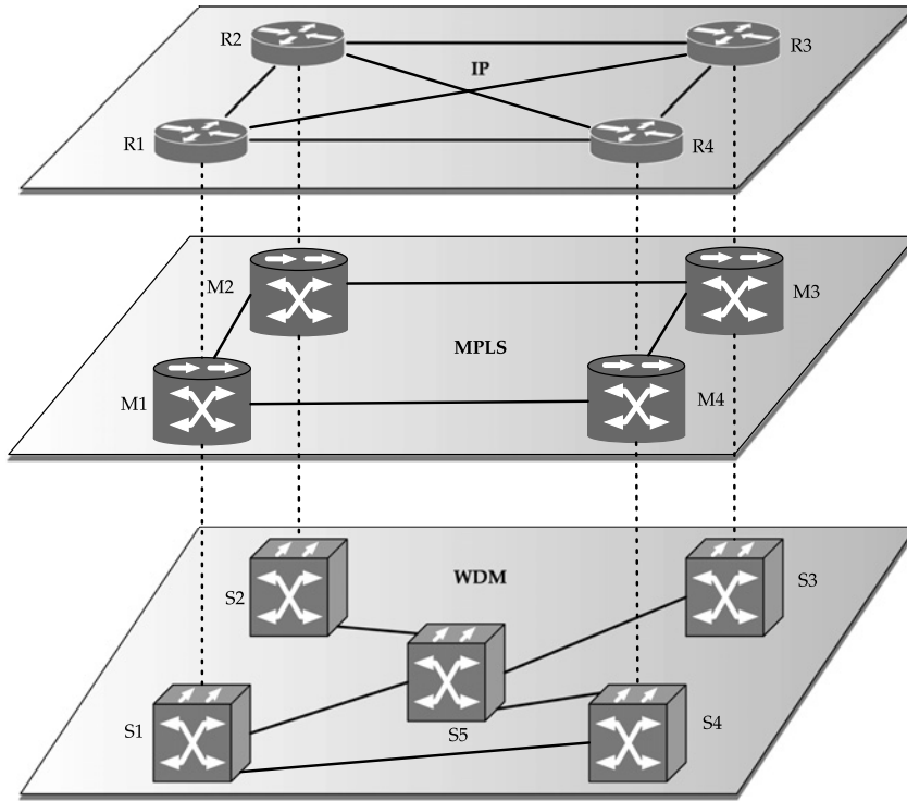
FIGURE 25.8 IP over MPLS over WDM: a three-layer architectural view.
