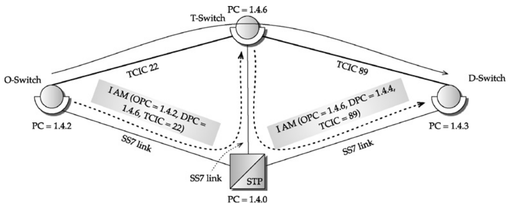
FIGURE 12.9 Call routing and SS7 message routing illustration.
