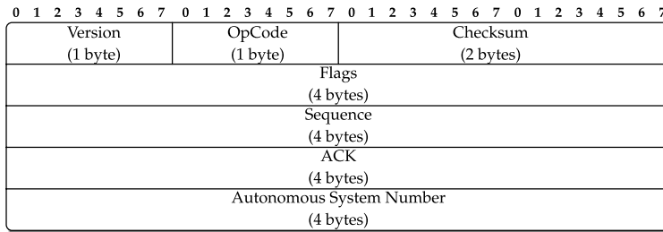
FIGURE 5.7 EIGRP packet header.
