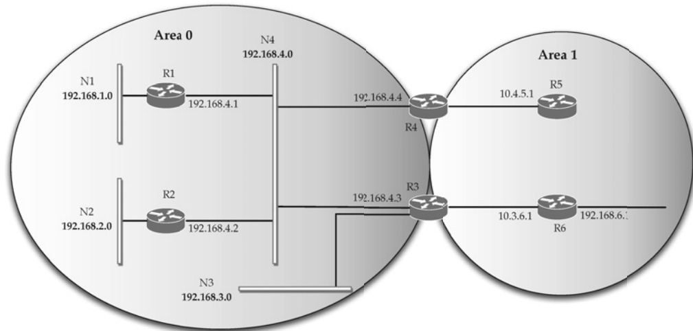
FIGURE 6.13 OSPF network example.
