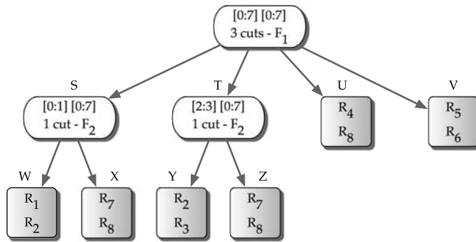
FIGURE 16.25 HiCuts decision tree for rules in Table 16.2.
