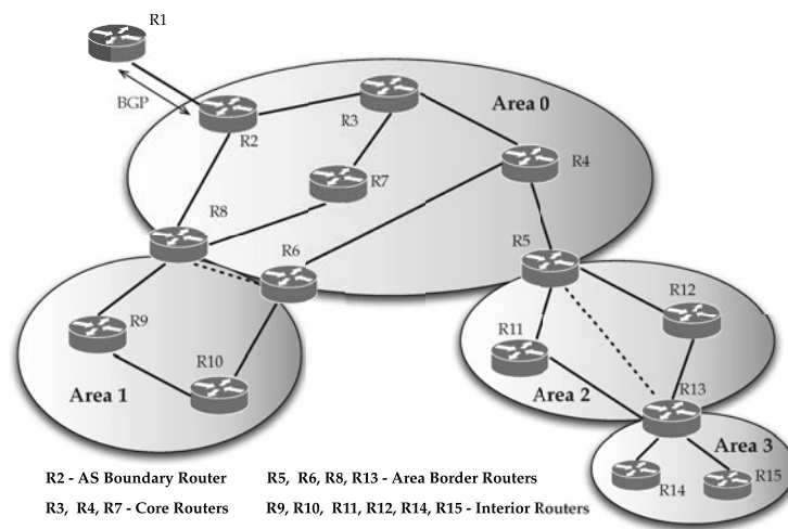
FIGURE 6.1 OSPF backbone and low-level areas.
