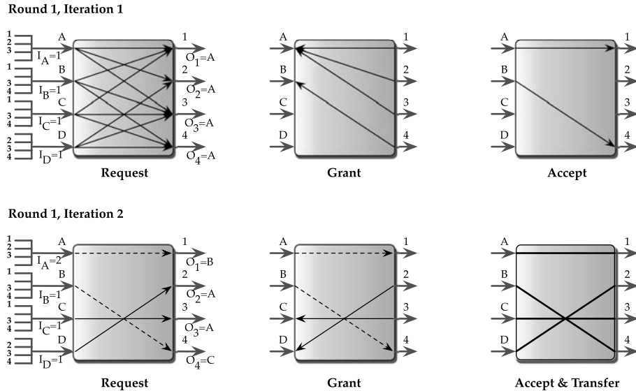
FIGURE 21.19 Two-iteration iSLIP scheduling in operation—round 1.
