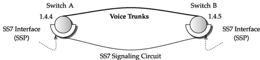
FIGURE 12.3 Switch-SS7 interface.
