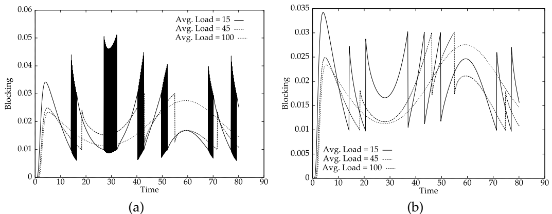
FIGURE 19.4 Transient performance due to an LSP bandwidth allocation/deallocation scheme: (a) instability; (b) corrected through control.
