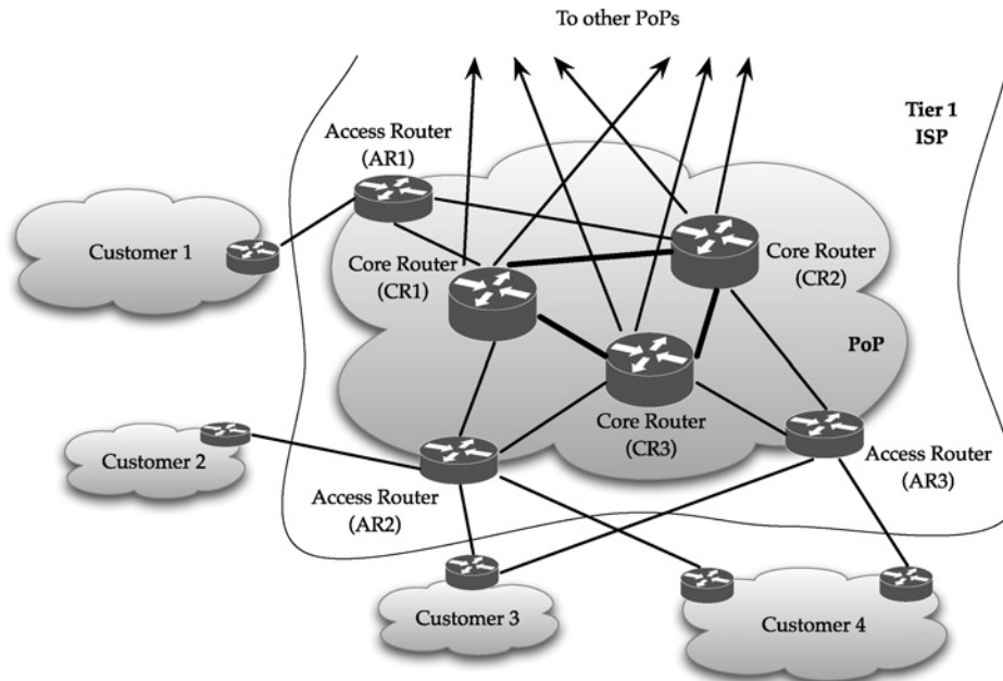
FIGURE 9.14 Tier 1 ISP's Point of Presence (PoP) connectivity architecture.
