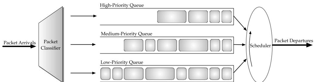
FIGURE 22.1 Priority queuing.
