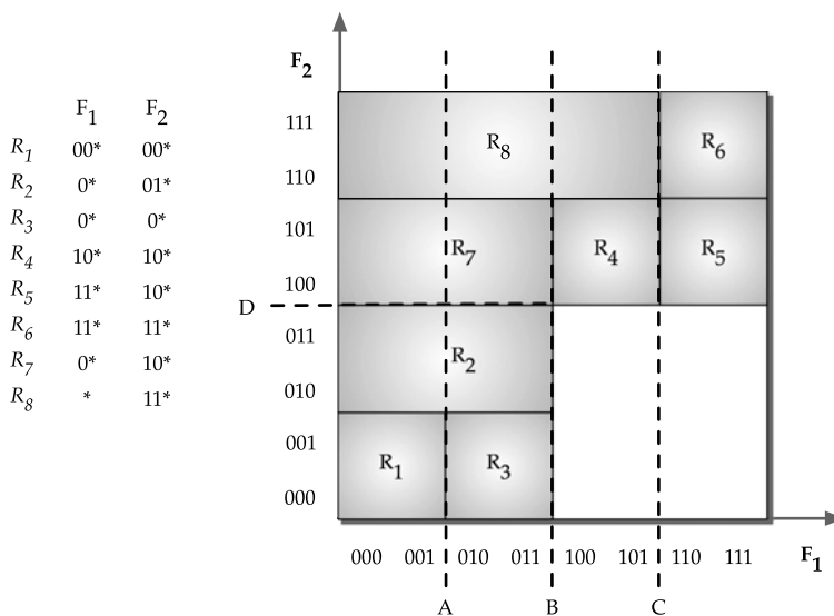
FIGURE 16.24 Geometric representation of HiCuts .
