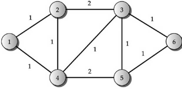
FIGURE 3.13 Network topology for illustration of the path vector protocol.
