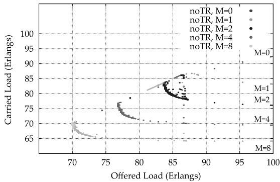
FIGURE 11.8 Symmetric network, no trunk reservation.
