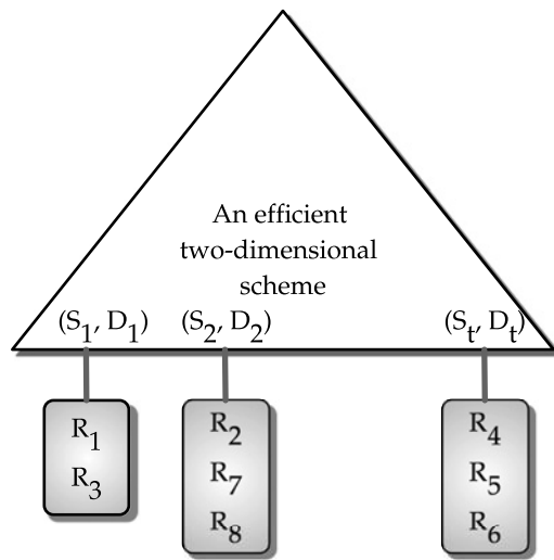
FIGURE 16.10 Extending a two-dimensional scheme for classification on arbitrary number of fields (adapted from [47]).
