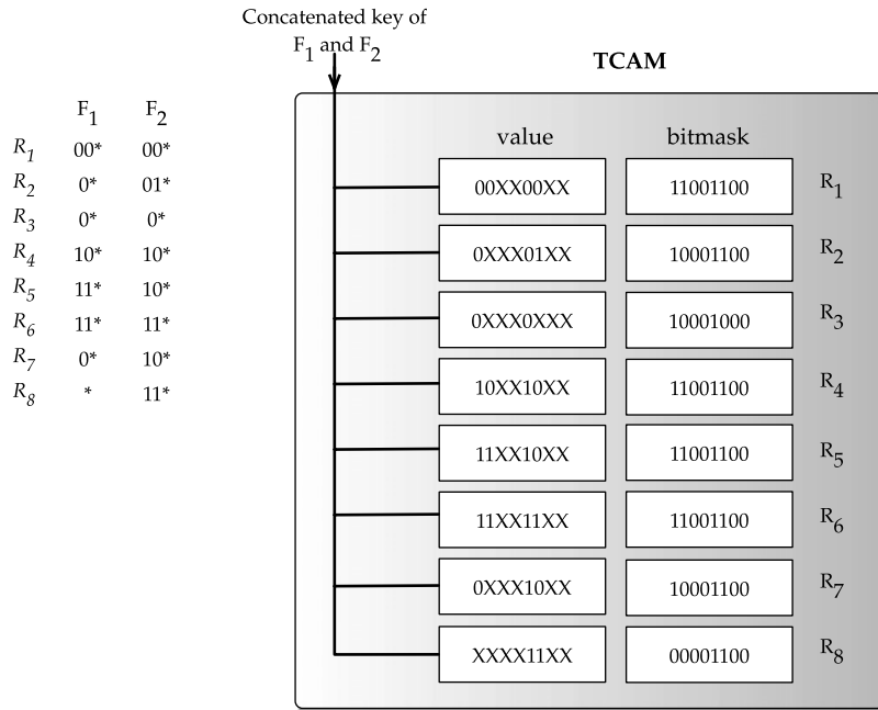
FIGURE 16.27 Representing the rules of Table 16.2 in TCAM.
