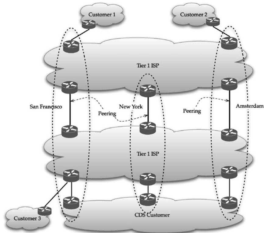
FIGURE 9.9 Customer traffic routing from a geographic perspective.
