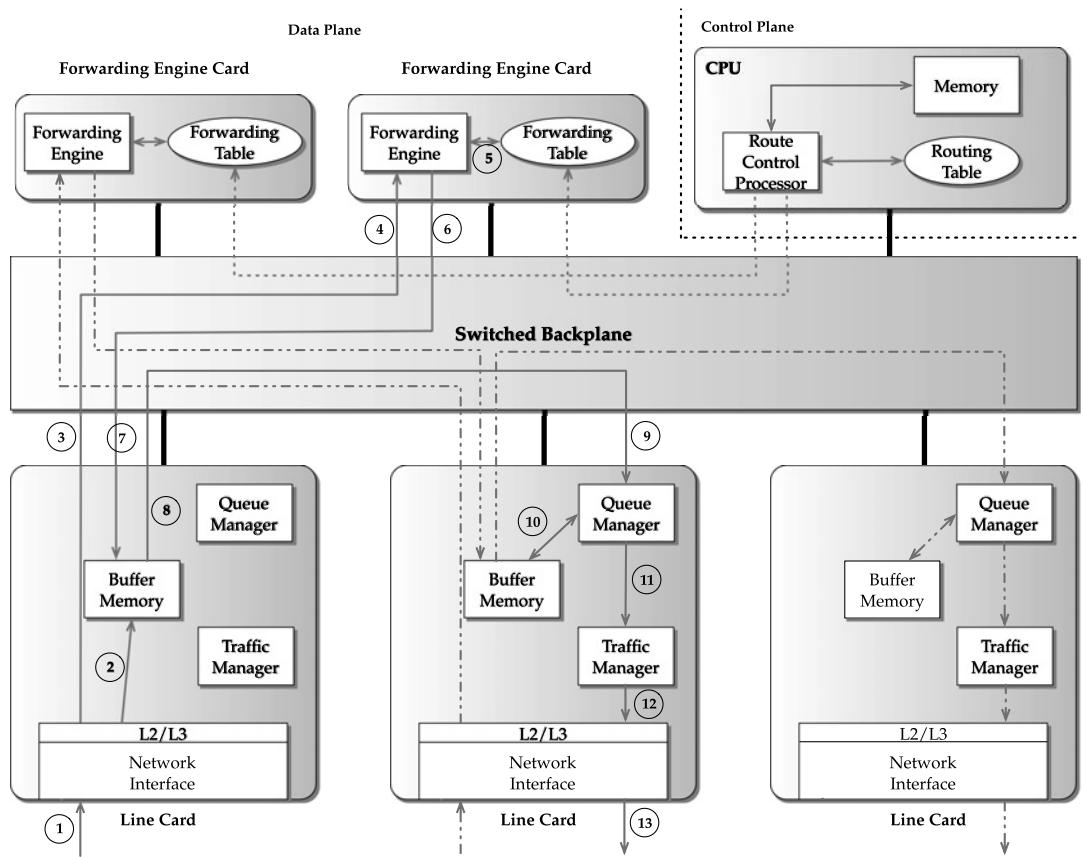
FIGURE 14.9 Shared forwarding engine architecture using a switched backplane.
