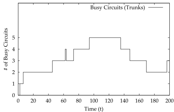
FIGURE 11.1 Number of busy circuits (trunks) as calls arrive and leave over time (shown up to 200 sec) for calls listed in Table 11.1.
