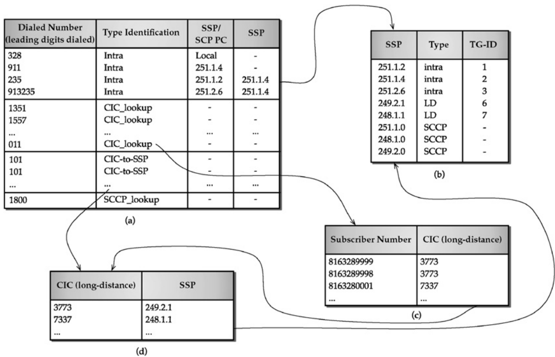
FIGURE 13.8 Table lookup phases in a LEC/IXC environment.
