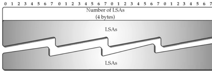
FIGURE 6.9 OSPF link state update packet (OSPF packet type = 4).
