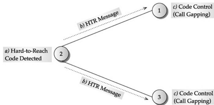
FIGURE 11.6 Code control and hard-to-reach (HTR) capability, from detection to action.
