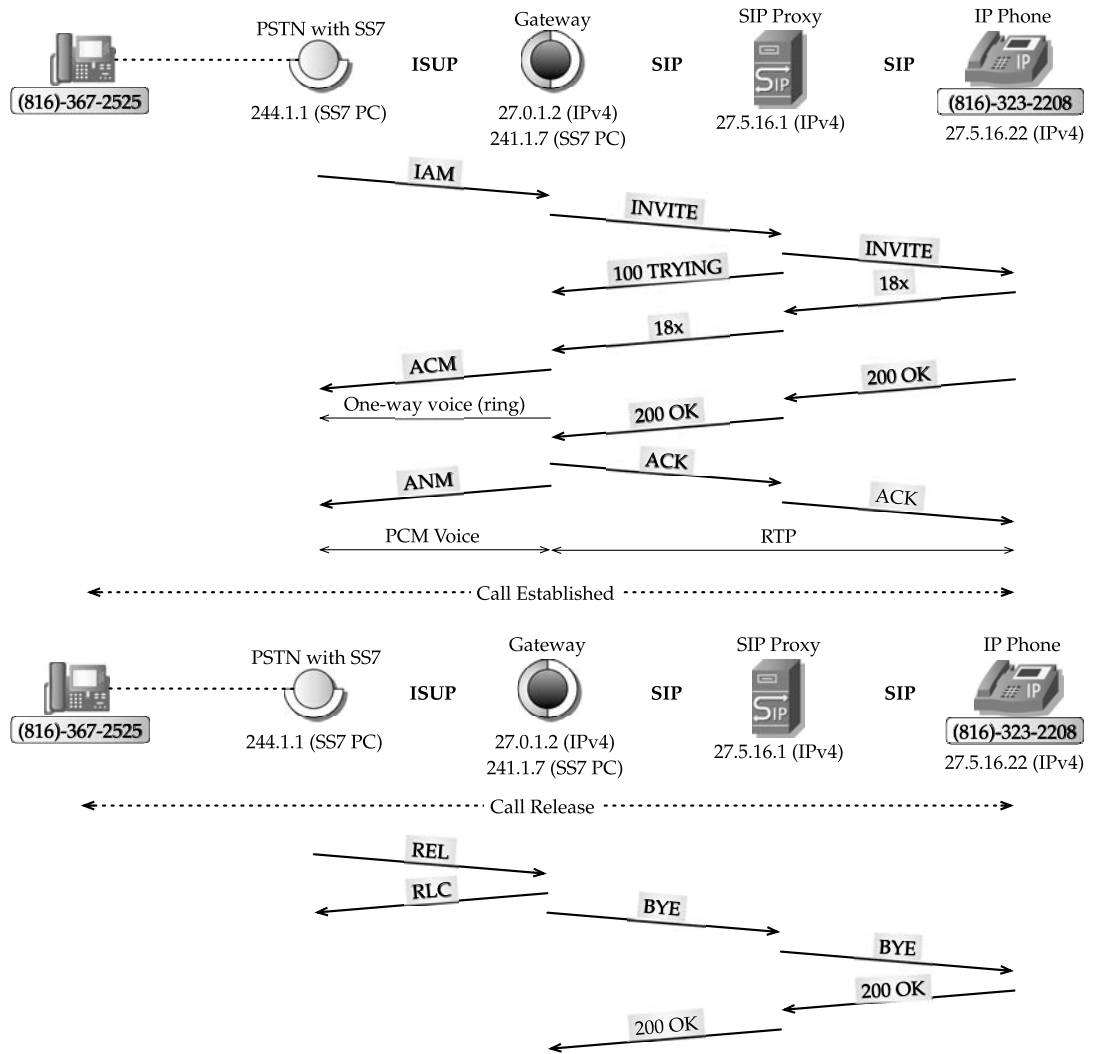
FIGURE 20.8 Call flow example from PSTN to SIP.
