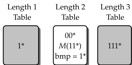
FIGURE 15.22 Prefix length tables with markers and precomputed best matching prefix.
