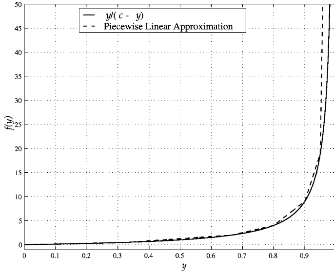
FIGURE 4.8 Piecewise linear approximation function (4.3.16) of y/(c - y) (when c = 1 ).
