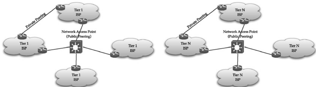
FIGURE 9.6 ISP connectivity through public peering at an exchange point and through private peering (left: used to be more common among tier 1 ISPs; right: now seen more commonly at other tiering (“tier-N”) levels).
