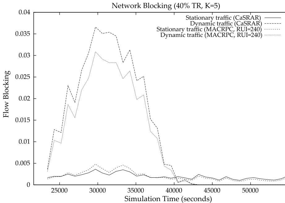
FIGURE 17.7 Performance of dynamic and stationary traffic (with trunk reservation).
