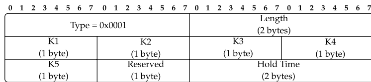
FIGURE 5.9 EIGRP: TLV type for EIGRP parameters.
