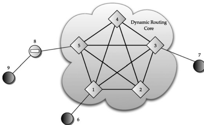
FIGURE 10.7 Dynamic call routing in conjunction with hierarchical routing.
