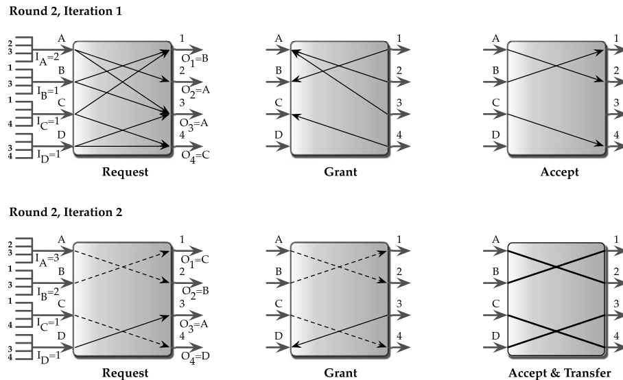
FIGURE 21.20 Two-iteration iSLIP scheduling in operation—round 2.
