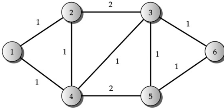
FIGURE 3.5 Six-node, nine-link network example.
