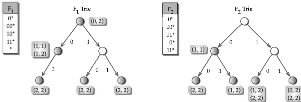
FIGURE 16.23 The F_1 and F_2 tries with tuples for rules in Table 16.2.
