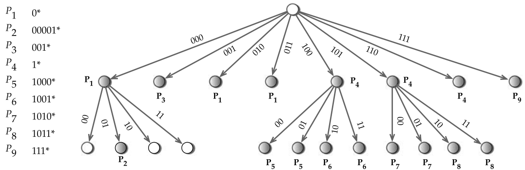
FIGURE 15.8 Fixed stride multibit trie data structure for the prefixes of Table 15.2.
