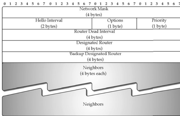
FIGURE 6.6 OSPF hello packet (OSPF packet type = 1).
