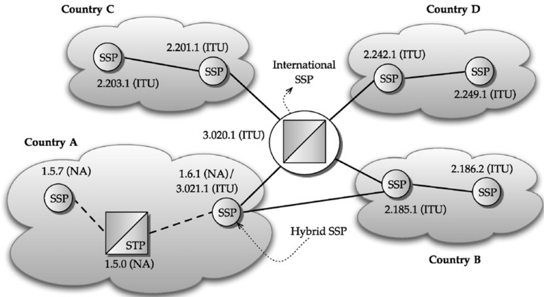
FIGURE 12.4 Interworking of SS7 networks with different point code systems.
