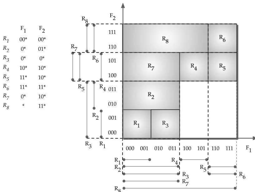
FIGURE 16.16 Geometric representation for identifying equivalence classes.
