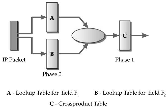
FIGURE 16.20 Packet flow in recursive flow classification.
