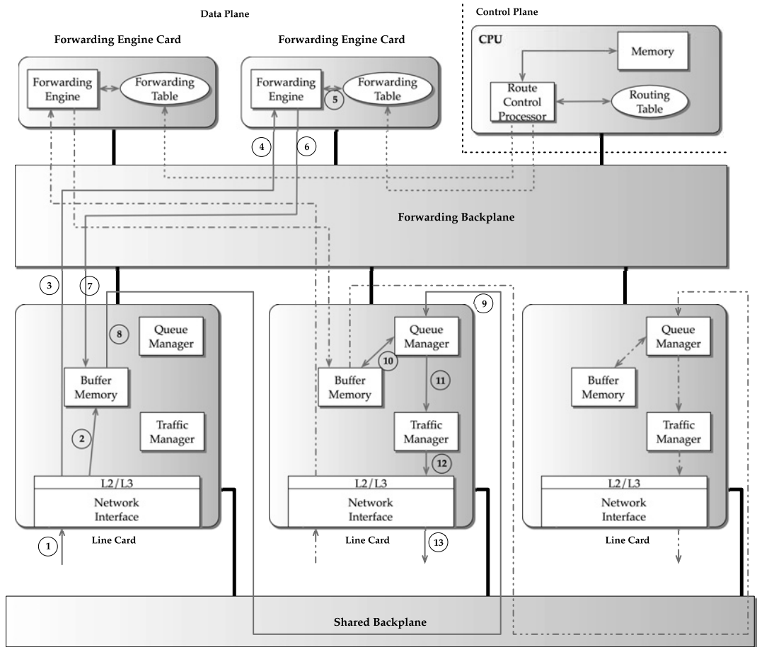
FIGURE 14.8 Shared forwarding engine architecture using two shared backplanes.
