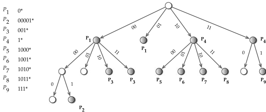
FIGURE 15.11 Variable stride multibit trie.
