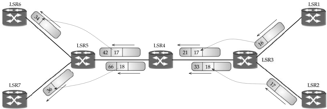
FIGURE 18.5 Label-switched paths using an LSP tunnel (“tunnel within a tunnel”).
