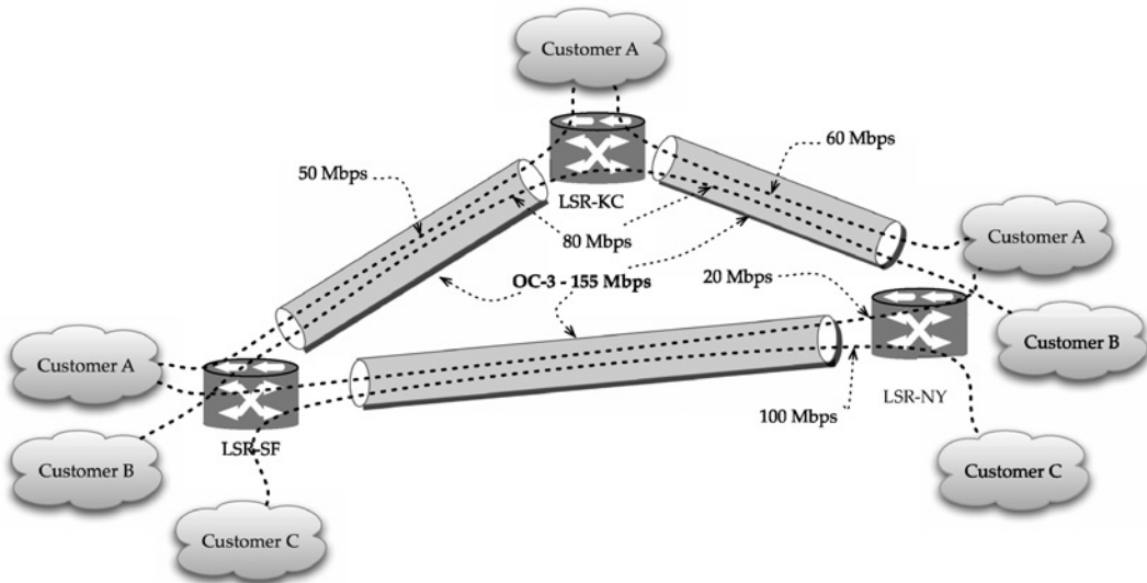
(c) Routing view to MPLS-VPN provider
