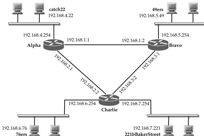
FIGURE 5.1 IP network illustration.
