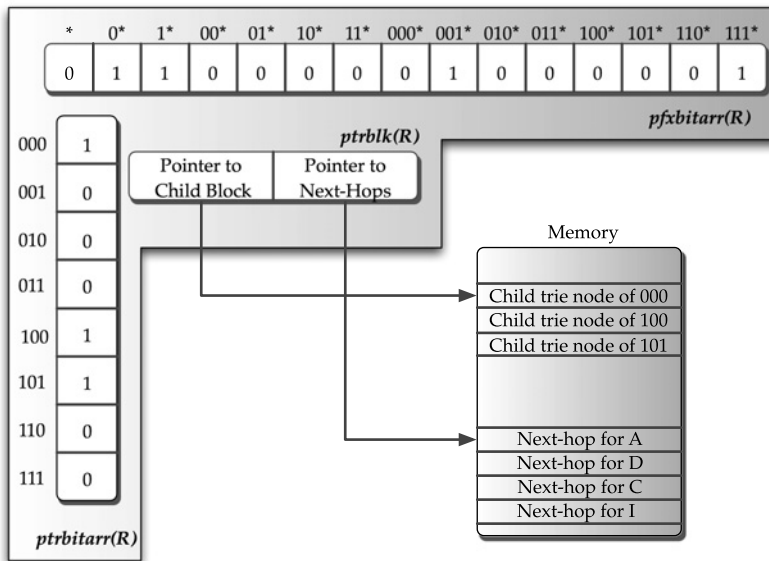
FIGURE 15.18 Structure of tree bitmap node corresponding to root node of trie in Figure 15.10.
