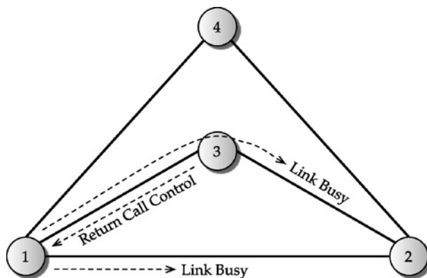
FIGURE 10.6 Illustration of crankback.
