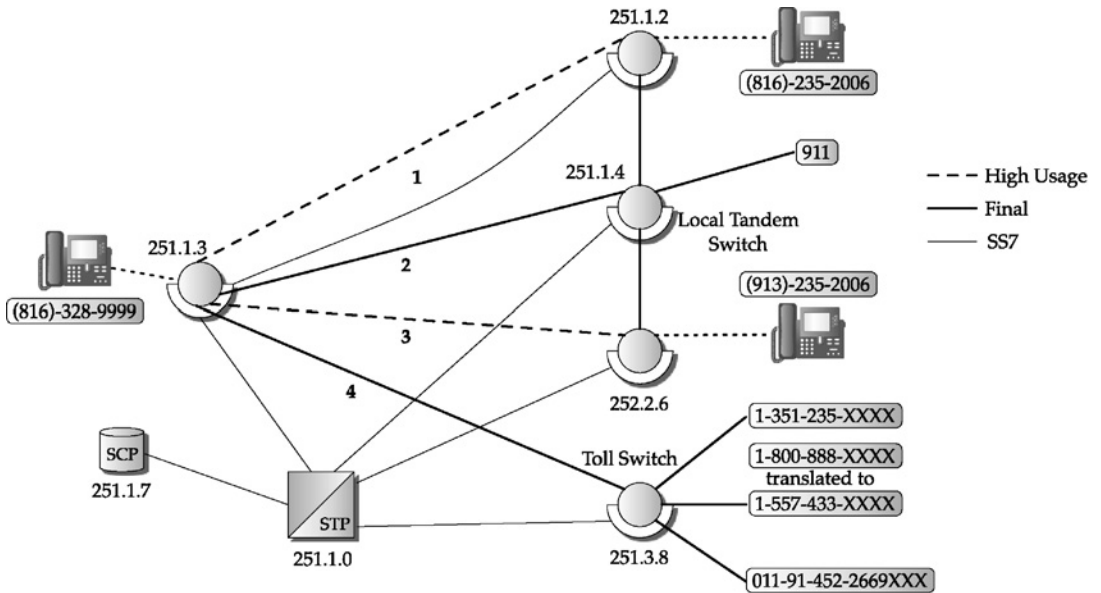
FIGURE 13.2 Call and message routing for calls dialed from 816-328-9999.
