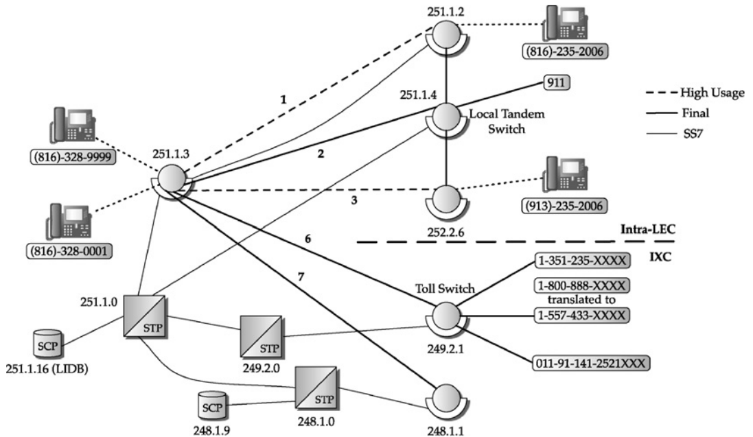
FIGURE 13.7 Call and message routing for calls dialed from SSP 251.1.3 in a LEC/IXC environment.
