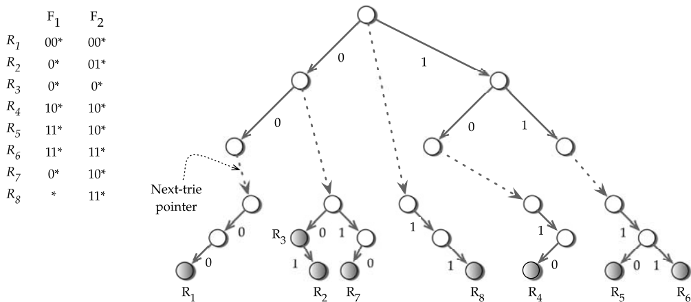
FIGURE 16.4 Combining the F_1 and F_2 tries for building a hierarchical trie.
