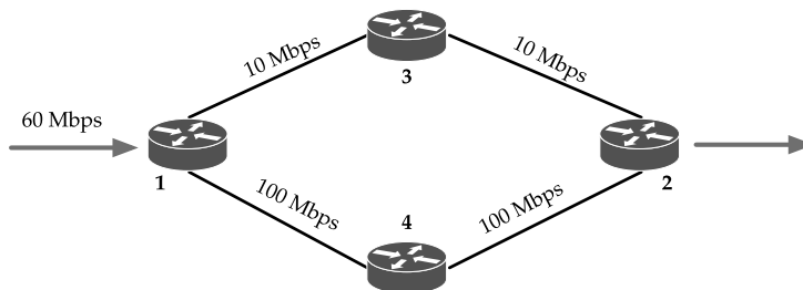
FIGURE 19.1 Four-node example with different link capacity.
