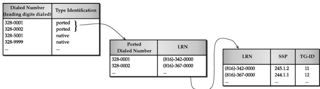
FIGURE 13.17 Lookup for ported local numbers for ISUP message and call routing.
