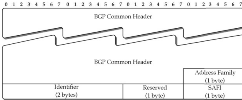
FIGURE 8.20 BGP4 ROUTE-REFRESH message.
