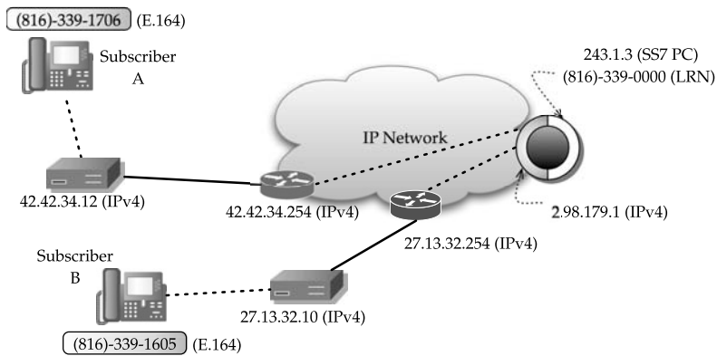
FIGURE 20.4 Call between two subscribers who are homed to Provider X's switch.
