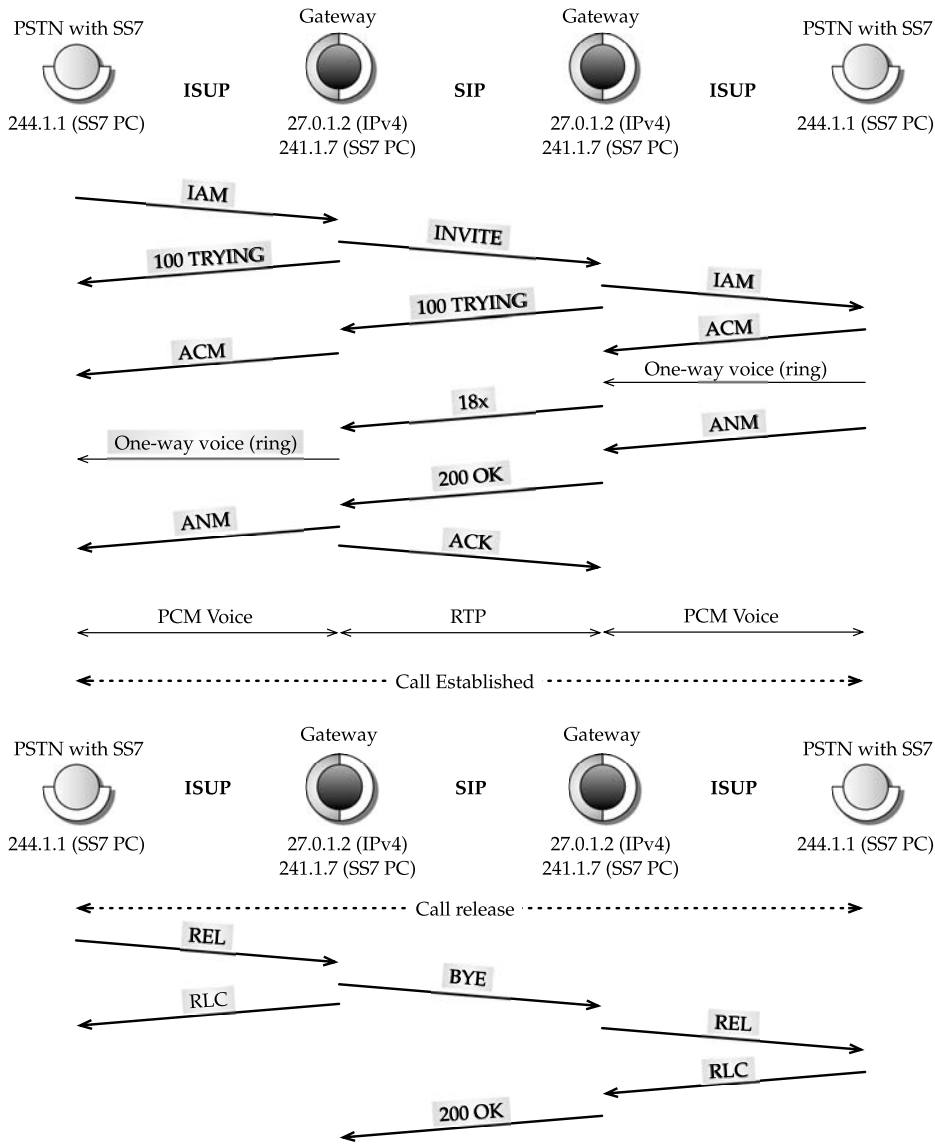
FIGURE 20.9 PSTN to IP to PSTN.
