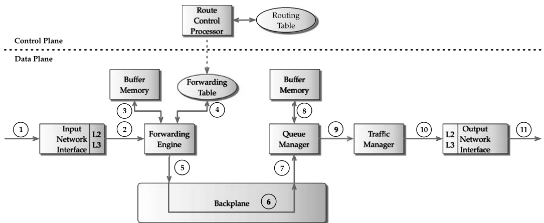
FIGURE 14.3 Packet flow in a router.
