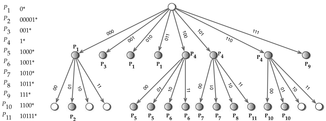
FIGURE 15.9 Inserting new prefixes in fixed stride multibit trie.
