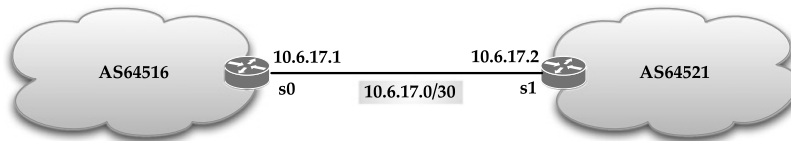
FIGURE 8.2 BGP session setup: direct interface between two ASes.
