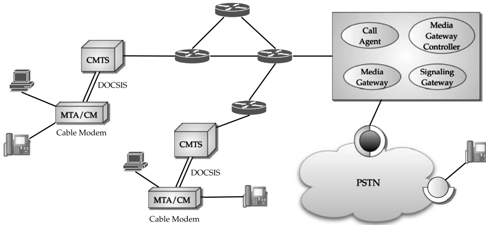
FIGURE 20.5 Cable IP networking for telephony services.
