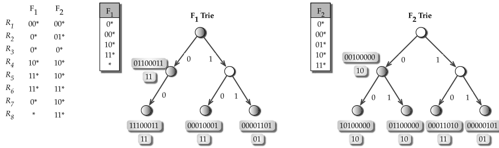
FIGURE 16.14 The F_1 and F_2 tries with original and aggregated bit vectors.
