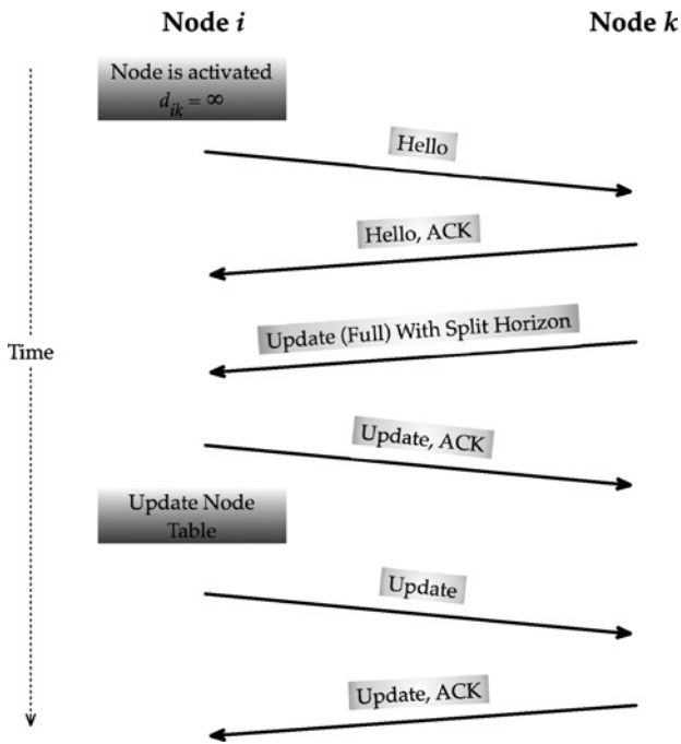
FIGURE 3.6 Protocol message exchanges when a node is activated.
