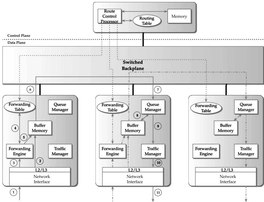
FIGURE 14.10 Shared nothing architecture.
