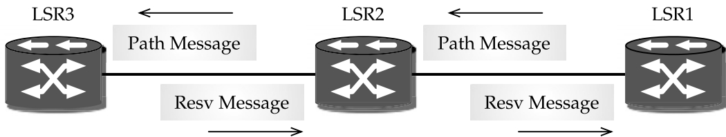
FIGURE 18.10 Example: label distribution using RSVP-TE.
