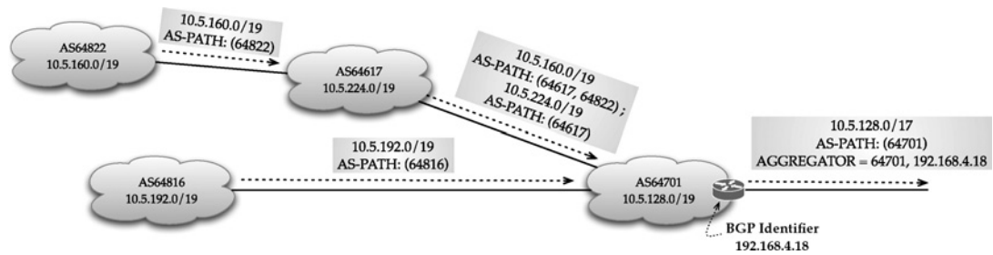
FIGURE 8.10 Route aggregation example using ATOMIC-AGGREGATE and AGGREGATOR.
