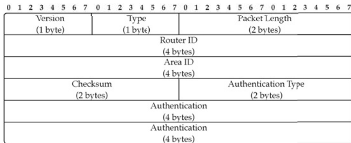
FIGURE 6.4 OSPF packet common header.
