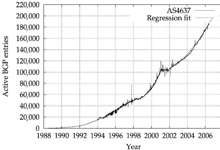
FIGURE 9.10 BGP routing table growth at AS4637 and regression fit.
