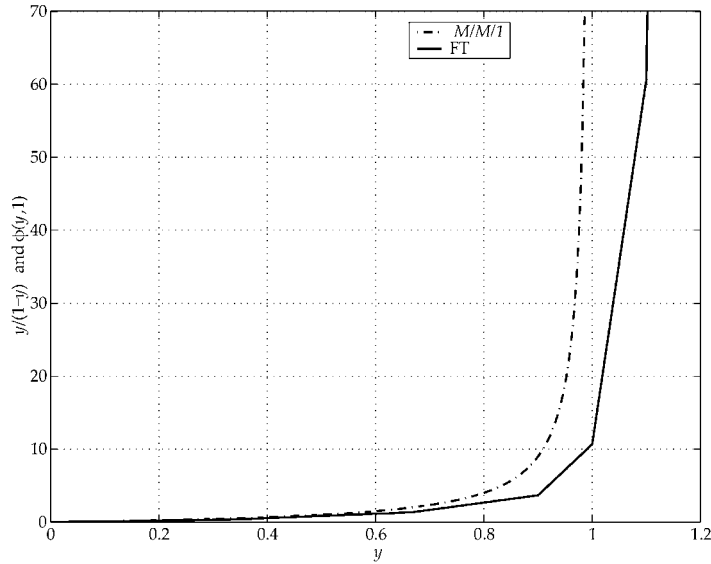
FIGURE 7.9 The Fortz–Thorup function and the load latency function (when c = 1 ).
