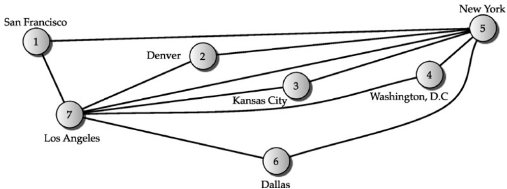
FIGURE 10.8 Engineered and real-time paths in DNHR between New York (switch 5) and Los Angeles (switch 7). Engineered and real-time paths are partitioned using a vertical line, whereas real-time paths are listed in italics in the routing table; note: switch 7 in the routing table indicates a direct link path. (Adapted from [27].)
