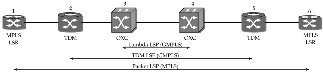
FIGURE 18.13 Label stacking and hierarchical LSPs: MPLS/GMPLS.
