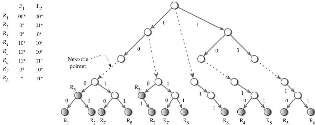
FIGURE 16.5 Set pruning trie data structure containing replicated rules.
