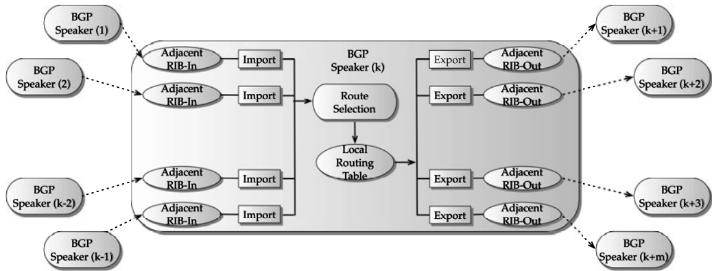
FIGURE 8.11 BGP decision process.
