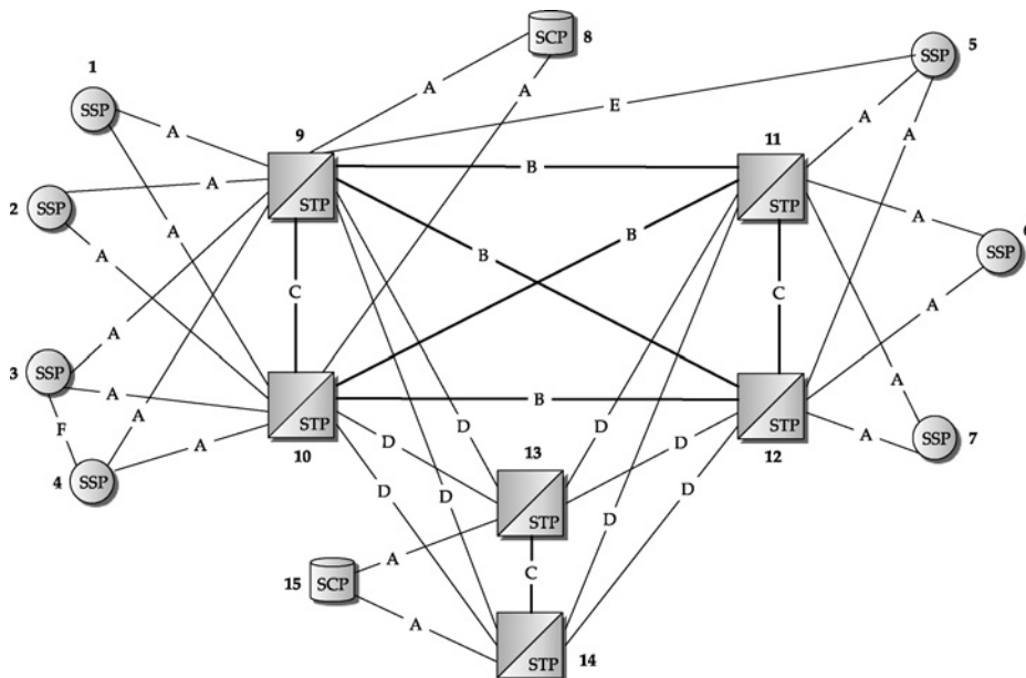
FIGURE 12.1 A sample SS7 network topology where all link and node types are shown.
