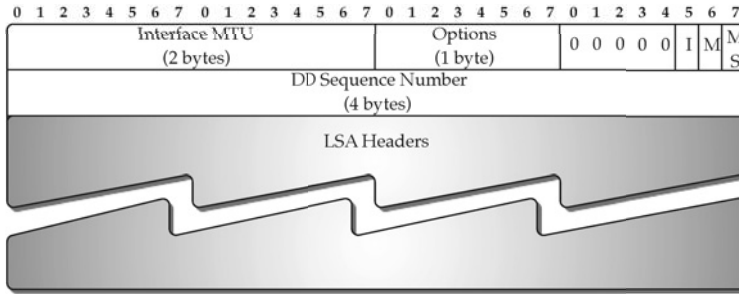
FIGURE 6.7 OSPF database description packet (OSPF packet type = 2).
