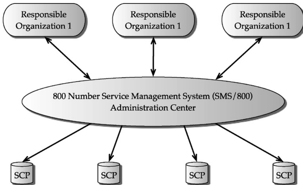
FIGURE 13.13 Service Management System/800-number architecture: process and communication to SCPs.
