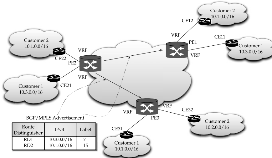
FIGURE 18.18 BGP/MPLS example with multiple customers.
