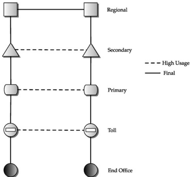
FIGURE 10.2 Switching hierarchy in hierarchical routing.
