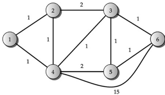
FIGURE 3.2 Six-node, ten-link network example (the entry shown next to a link is the cost of the link).
