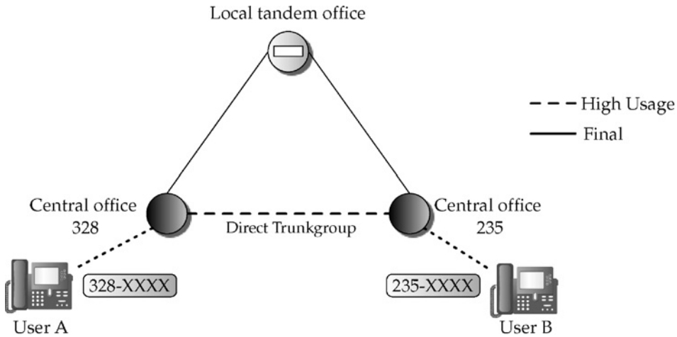
FIGURE 13.1 A local call from (816) 328-9999 to (816) 235-2006.
