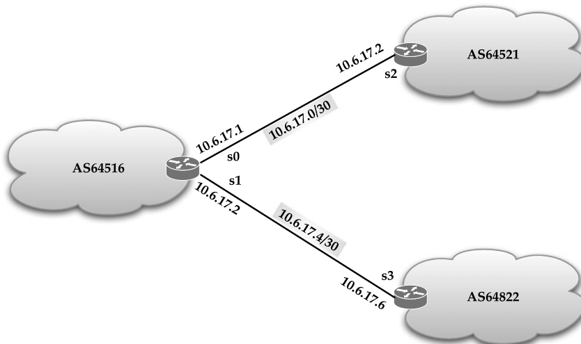
FIGURE 8.3 BGP session setup: direct interface between an autonomous system (AS) and its two neighbors.
