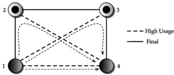
FIGURE 10.5 Limitation due to hierarchical routing.
