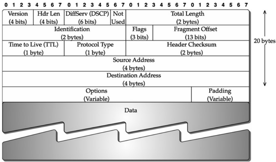
(a) IPv4 packet
