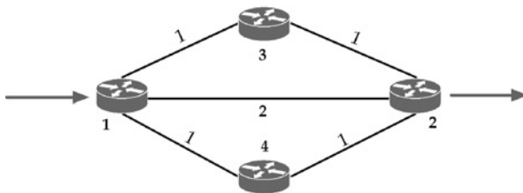
FIGURE 7.8 A four-node network example with link weights.
