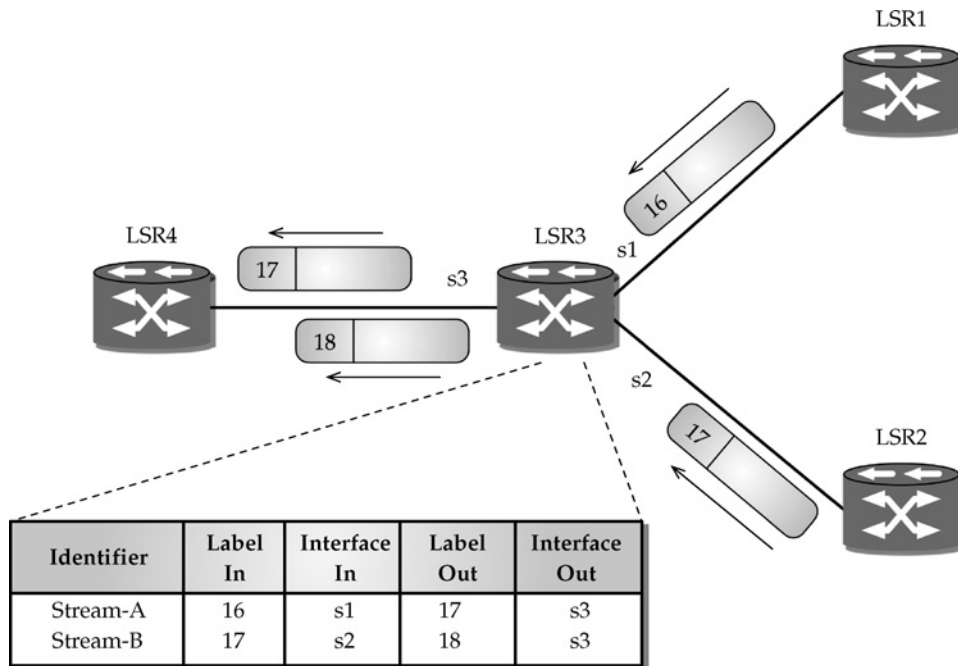
FIGURE 18.4 Label swapping and label switched paths.
