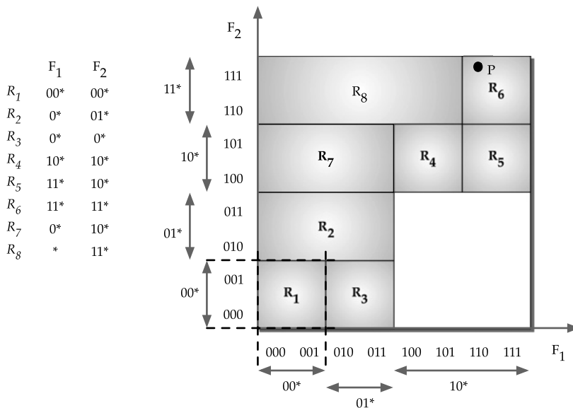
FIGURE 16.8 Geometric representation of rules. Each rule is shown as a shaded region.
