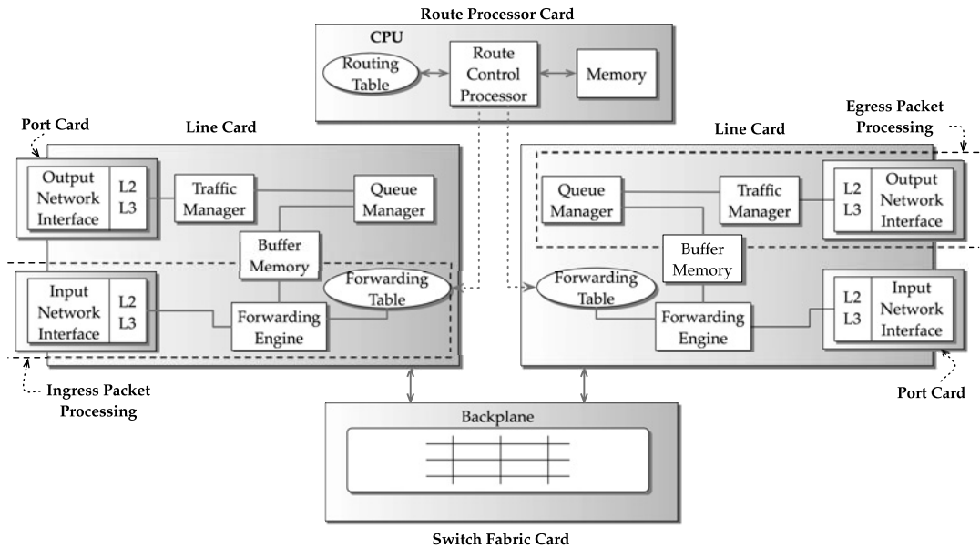
FIGURE 14.2 Components of a router.
