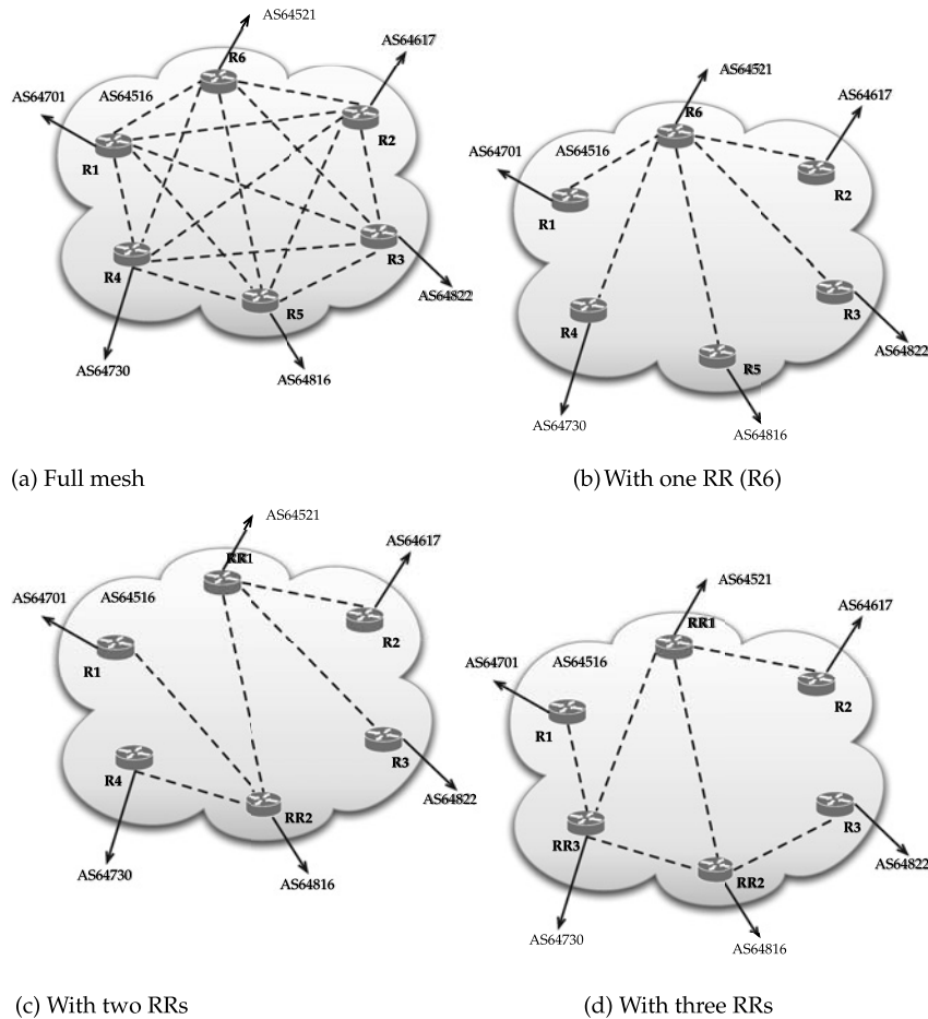
FIGURE 8.12 IBGP route reflector example showing IBGP sessions (route reflectors are identified by RR).
