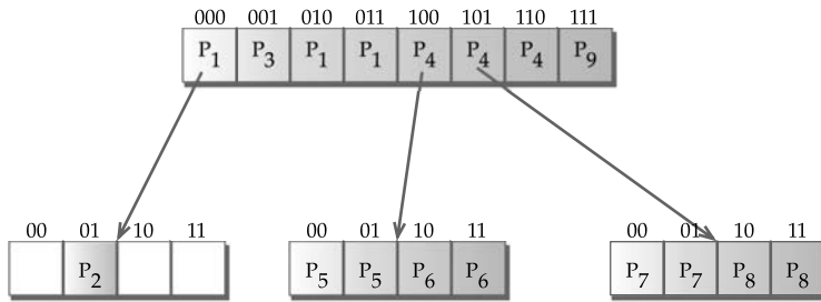
FIGURE 15.10 Implementation of the fixed stride multibit trie shown in Figure 15.8.
