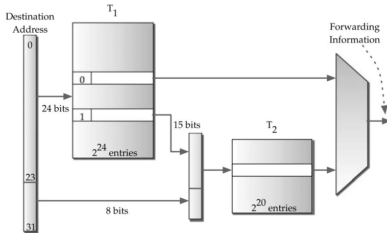
FIGURE 15.28 Implementation of multibit tries in hardware.
