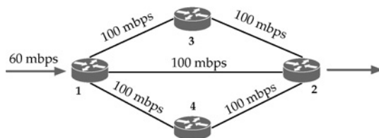
FIGURE 7.7 A four-node network example with five links.
