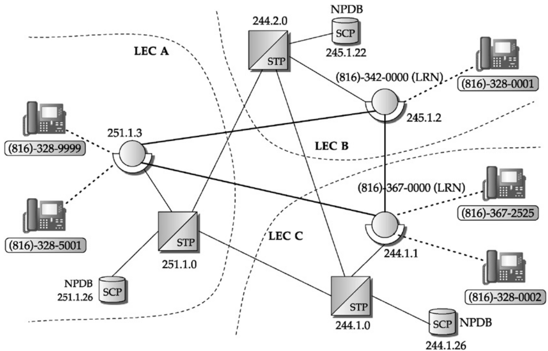
FIGURE 13.18 Multiple LECs in a geographic region: architecture and call routing for ported numbers.
