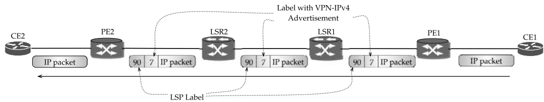
FIGURE 18.17 Prepending of two labels in BGP/MPLS packet forwarding.
