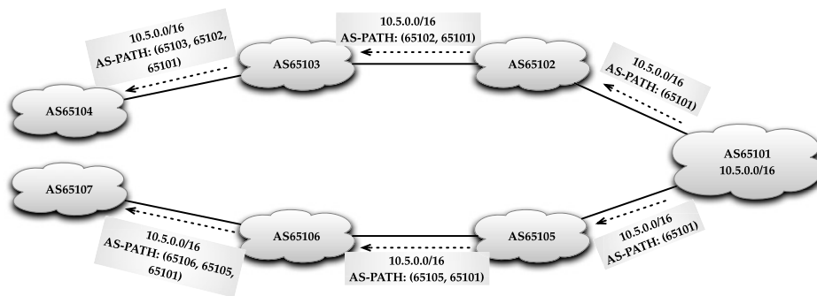
FIGURE 8.6 BGP path Attribute: AS-PATH example.
