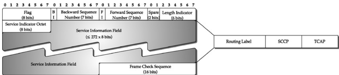
FIGURE 12.11 SCCP and TCAP in Service Information Field of MSU.
