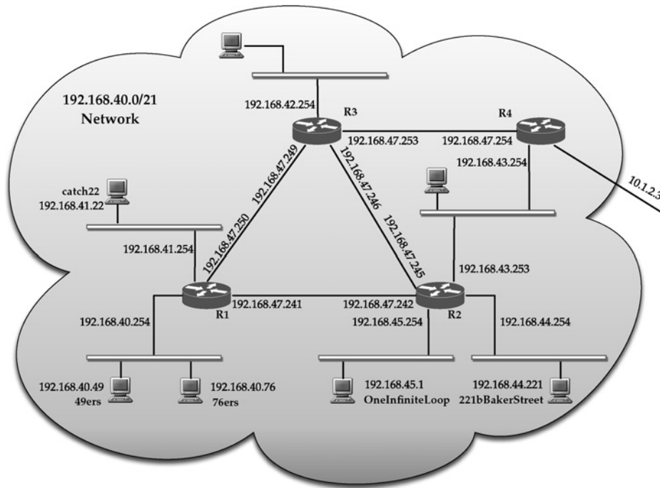
FIGURE 9.3 Network 192.168.40.0/21 with subnets and routers.
