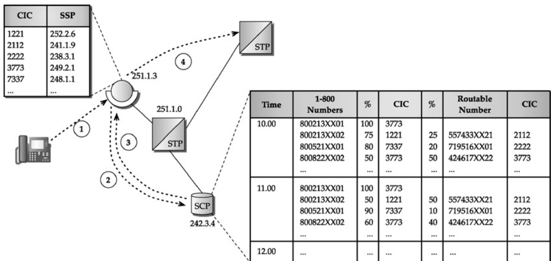
FIGURE 13.14 800-number portability, lookup, and ISUP message routing: 1—call initiated by user; 2, 3—TCAP messages; 4—IAM message.
