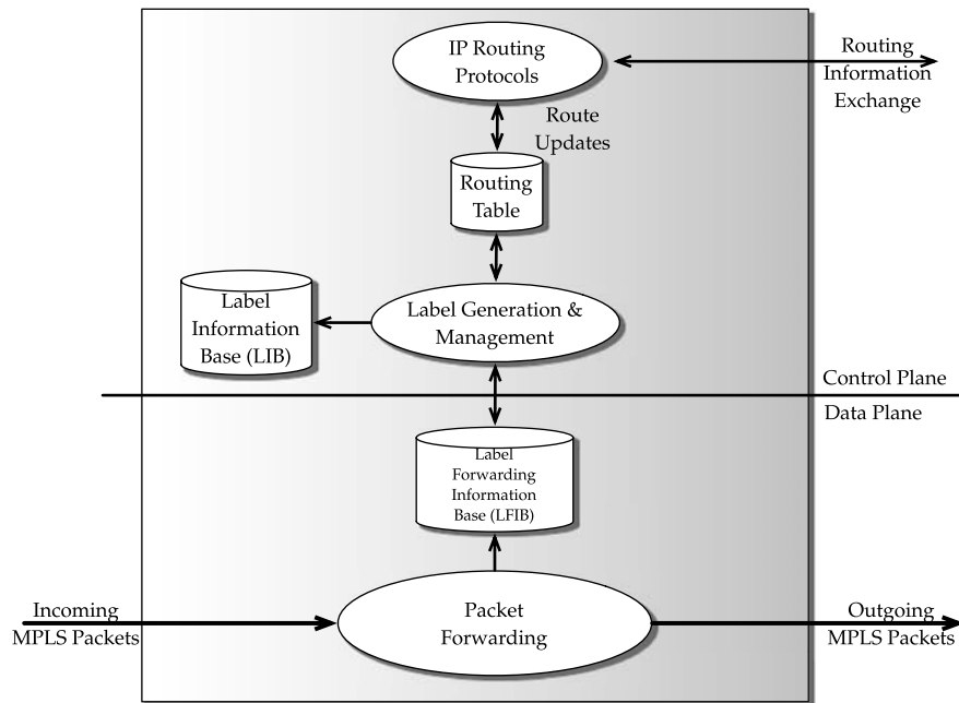
FIGURE 18.1 Conceptual architecture of an MPLS label-switched router.
