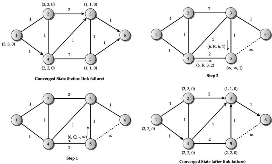
FIGURE 3.9 Coordination activities in the loop-free distance vector protocol.
