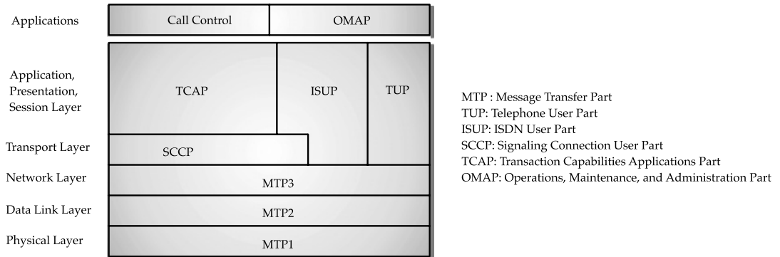
FIGURE 12.5 SS7 protocol stack.
