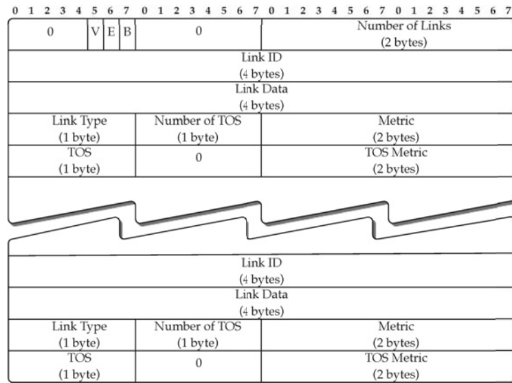
FIGURE 6.11 OSPF Router LSA content (LSA type = 1).
