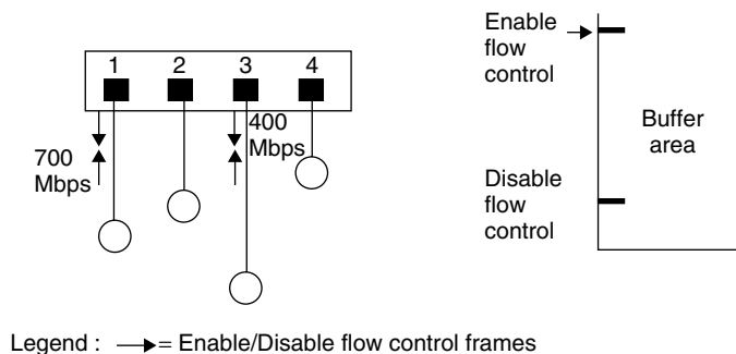
Figure 3.52 A buffered distributor uses IEEE 802.3z flow control whenever the offered traffic exceeds the bandwidth of its shared bus.
