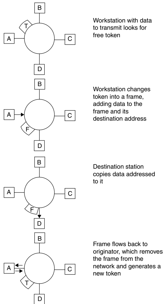
Figure 1.12 Token-Ring operation.
