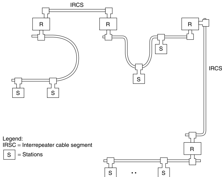
Figure 3.11 Expanding a 10BASE-2 network. Up to five cable segments connected through the use of four repeaters can be used to expand a 10BASE-2 network.
