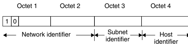
Figure 5.40 Class B subnetting.
