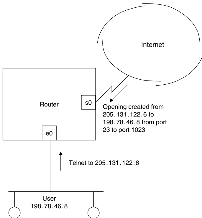
Figure 9.5 Examining the operation of a reflexive access list.
