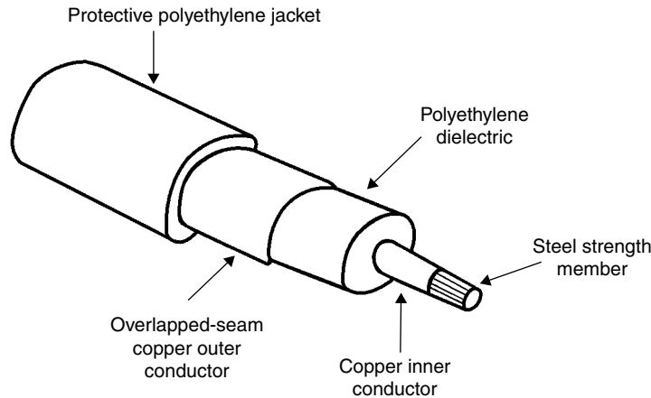
Figure 1.8 Coaxial cable.
