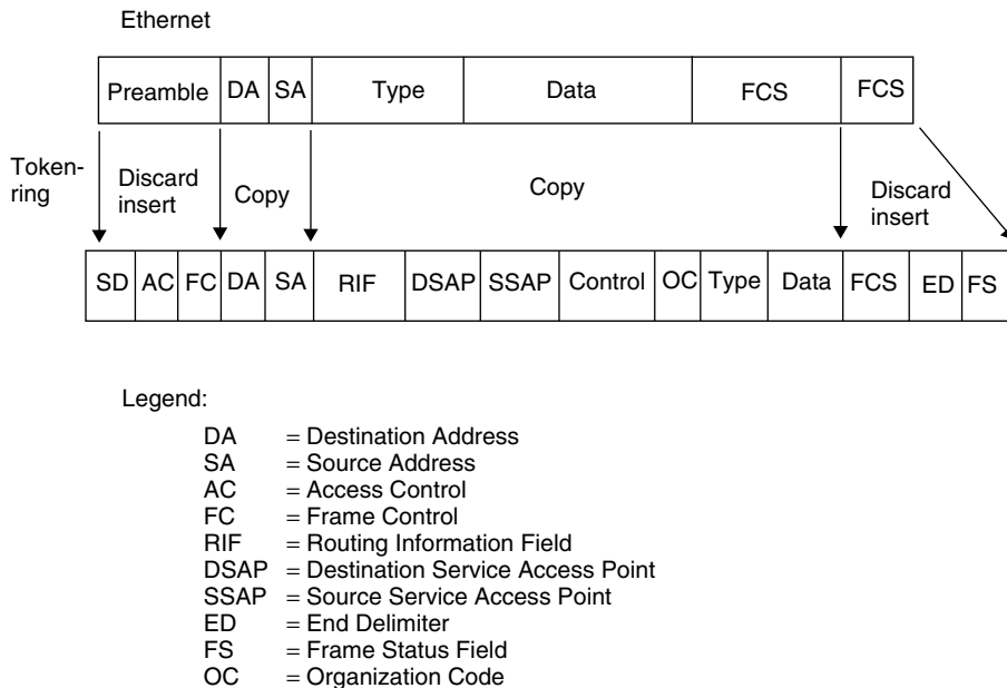
Figure 6.10 Ethernet to Token-Ring frame conversion.
