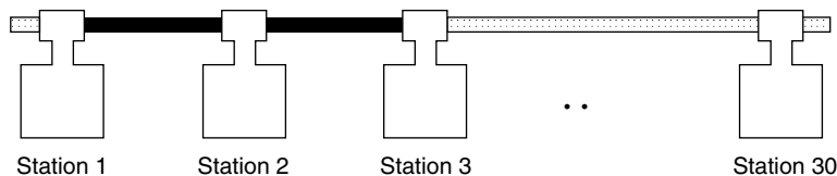
Figure 3.8 Cabling a 10BASE-2 network. A 10BASE-2 cable segment cannot exceed 185 meters and is limited to supporting up to 30 nodes or stations.
