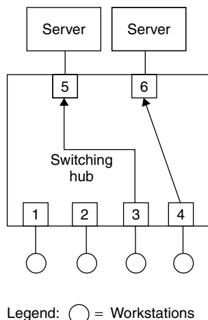
Figure 5.17 A switching hub supports multiple simultaneous cross-connection operations, which enhance available network bandwidth.
