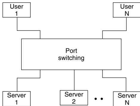
Figure 6.21 Port-based switching. In port-based switching only a single address per port is supported, restricting switching to one device per port.
