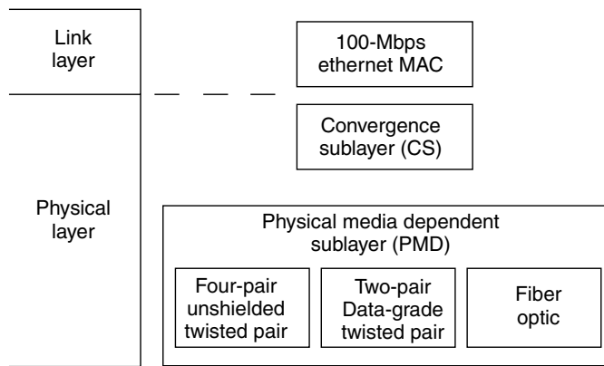
Figure 3.27 Fast Ethernet physical layering subdivision overview.
