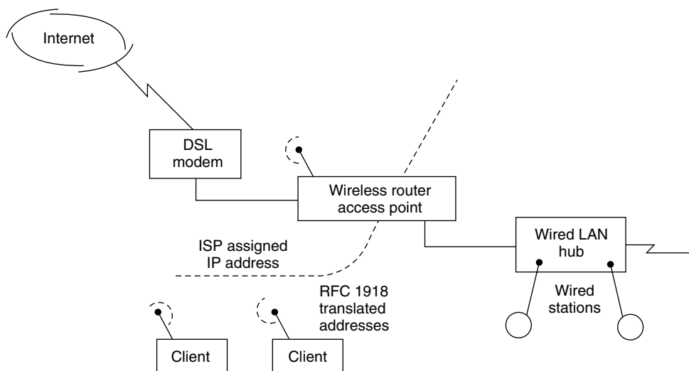
Figure 8.18 Using a wireless router/access point.
