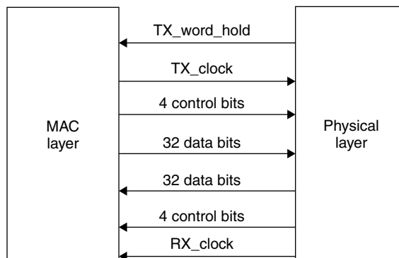
Figure 3.54 The 10 GMII.
