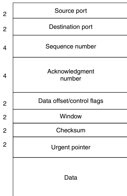
Figure 5.35 TCP protocol header.
