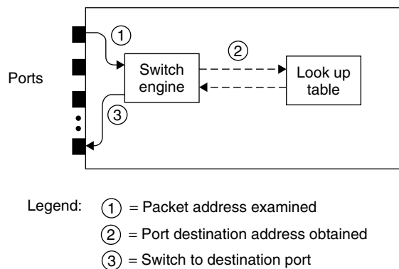
Figure 6.19 Cross-point/cut-through switching.
