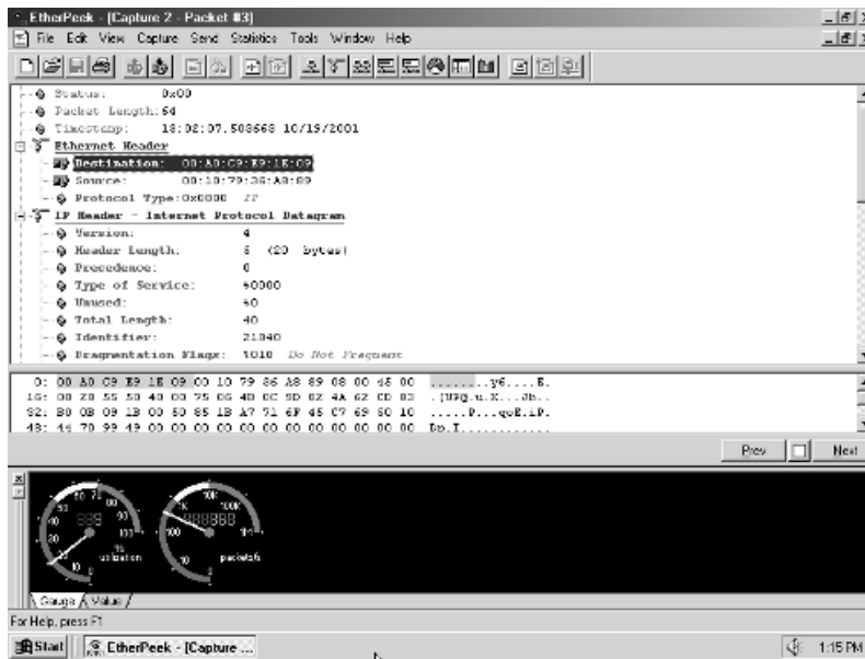
Figure 10.23 Using EtherPeek to decode a packet transported in an Ethernet frame.
