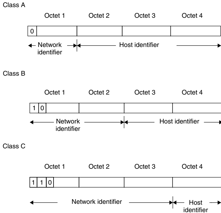
Figure 5.39 IP Classfull address formats.
