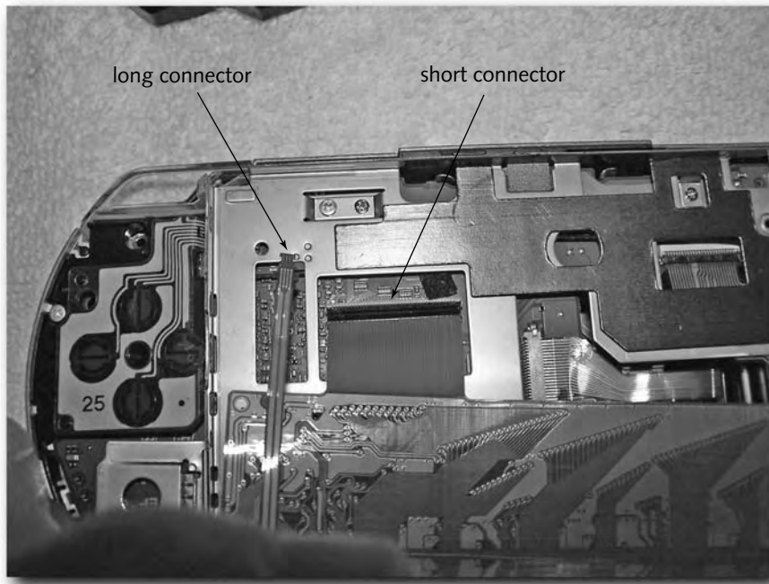
FIGURE 4-10: The display circuit strips connected to the mainboard
