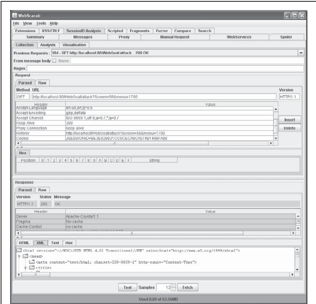
Figure 11-5 WebScarab, after intercepting several requests
