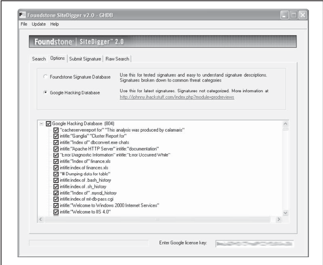
Figure 1-7 Foundstone’s SiteDigger searches Google’s cache using the Google Hacking Database (GHDB) to look for vulnerable systems.
