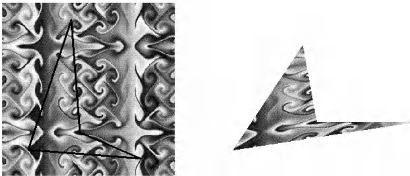
Figure 9-1 Texture-Mapping Process
