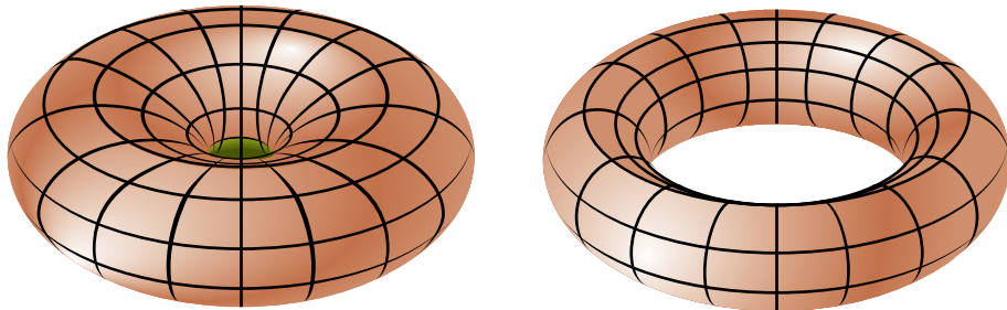
Figure 9-9 Texture-Map Distortion
