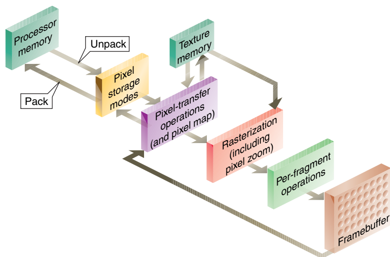
Figure 8-5 Imaging Pipeline
