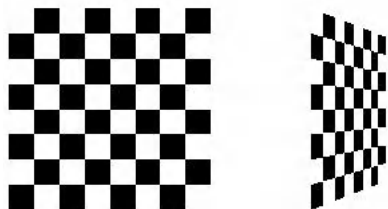
Figure 9-2 Texture-Mapped Squares
