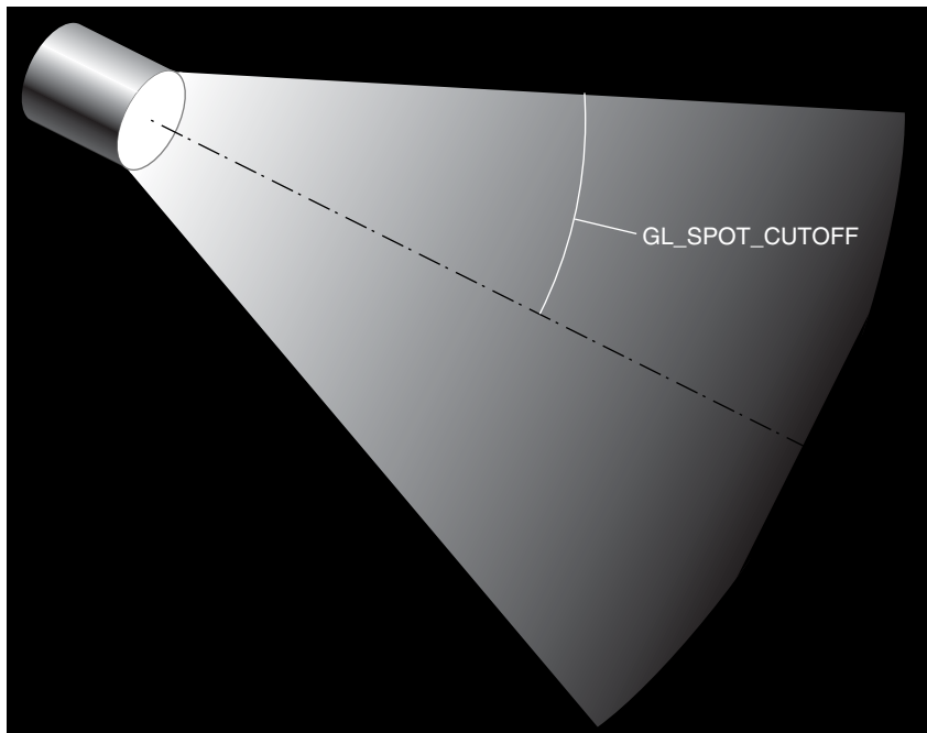
Figure 5-2 GL_SPOT_CUTOFF Parameter
