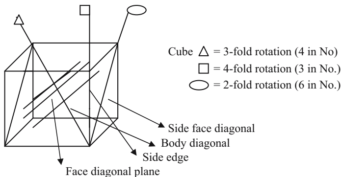
Fig. 4.1. Different planes and rotation axes in cube. \Delta = threefold rotation (4 in number); \square = fourfold rotation (3 in numbers); \circ = twofold rotation (6 in numbers)
