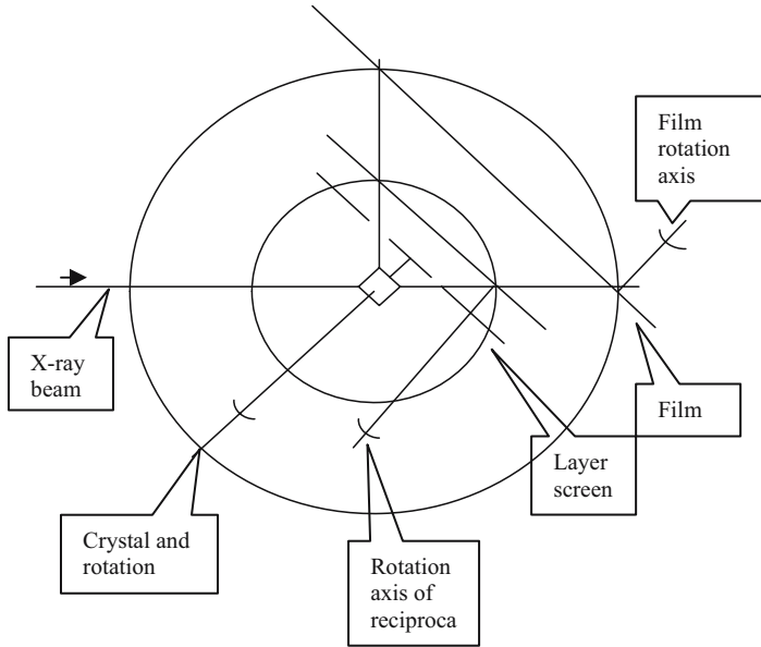
Fig. 7.12. de Jong–Boumann camera setup for recording the zero layer. (a) The crystal is mounted with its principal axis perpendicular to the film and rotated along its axis. The diffracted beam makes 90^\circ with the incident beam. (b) The zero layer rotates about the parallel axis. (c) The flat film parallel to the set of reciprocal lattice layers is also rotated about the axis. (d) The rotation of film and reciprocal lattice is synchronized, so that the diffracted spot reaches the same point on the film
