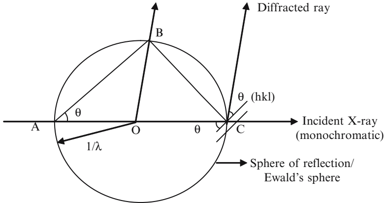
Fig. 6.9. Ewald's sphere of radius 1/\lambda , crystal may be stationed either at the center O or at C . The reciprocal lattice origin is also at C , \theta is the Bragg angle of reflection from the Miller plane (hkl) in the crystal, CB is drawn normal on the hkl plane
