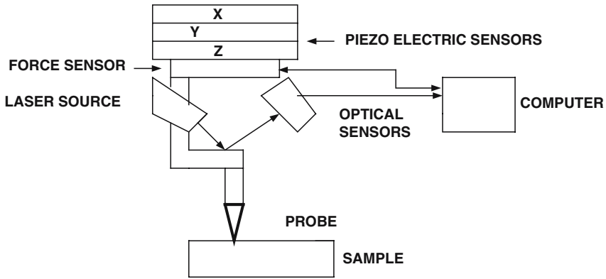
Fig. 10.20. The atomic force microscope. X,Y,Z are the piezoelectric sensors to control the motion of the probe over the sample in XYZ directions. Force sensor is to measure the force between the probe and the sample. (CPU) Computer – The computer is used for setting the scanning parameters such as scan size, scan speed, feedback control response, and visualizing images captured with the microscope
