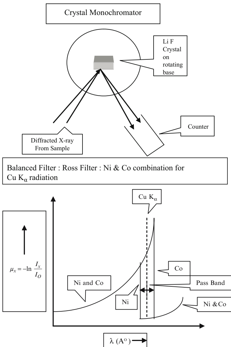
Fig. 6.4. (a) Crystal monochromator. LiF single crystals can diffract like other crystals, K_{\alpha} and K_{\beta} radiations from any target at specific angles and the counter placed at such angles will only record the diffraction pattern due to that wavelength and that without reducing the intensity of the radiation and reducing considerably the background. This is the major advantage of crystal monochromator now attached invariably with diffractometer. (b) Ross filter. As mass absorption coefficient is dependent on \lambda^3 , the two absorbers differing in Z by one will give same absorption coefficient for any wavelength except for the narrow region called pass band . This is the narrow region between K absorption edges of these two absorbers and when this pass band is chosen to include the K_{\alpha} , the result is a strong monochromatic beam
