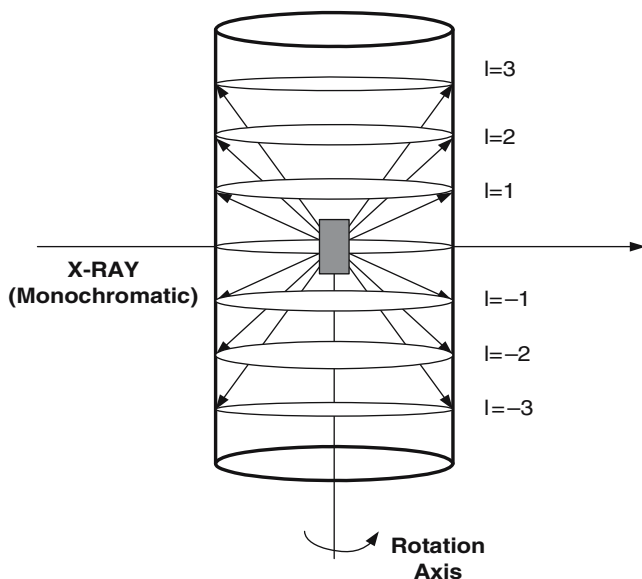
Fig. 7.4. The rotation-oscillation (cylindrical) camera. Monochromatic K_{\alpha} is used. The crystal shown at the center is rotated or oscillated. The layer lines formed by the intersection of diffraction cones and the cylindrical film are shown for different l values
