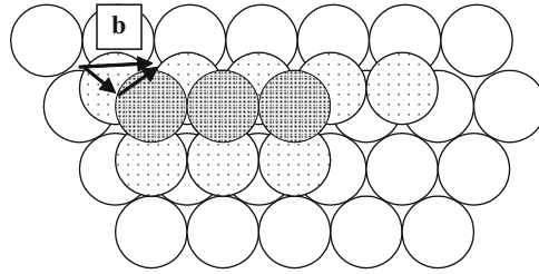
Fig. 10.2. Stacking sequence of close-packed plane \{111\} . The slip occurs in \langle 110 \rangle directions, which involves the sliding of one plane over other. A to B to C by the burger vector b = \frac{1}{2}[\bar{1}01] . Open circles , A Site; light-shaded circles , B Site; dark-shaded circles , C Site
