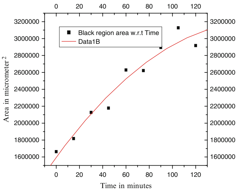
Fig. 10.15. 1-( trans -4-Hexylcyclohexyl)-4-isothiocyanatobenzene (nematic). The variation of black area with time at constant voltage of 12 V
