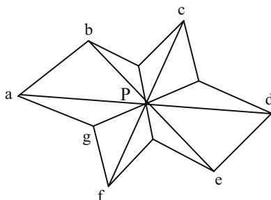
Fig. 3.5. One diagonal mirror plane in the pattern
