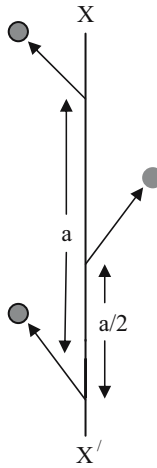
Fig. 5.5. A twofold rotation and half translation a/2 along the rotation axis XX' ; Symbol: 2_1
