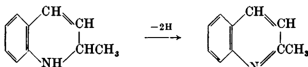
1:2-Dihydroquinaldine
