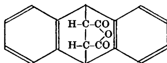
9 : 10-Dihydroanthracene-9 : 10-endo- \alpha\beta -succinic anhydride
