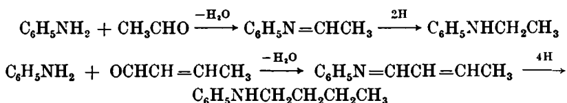
1:2-Dihydroquinaldine
