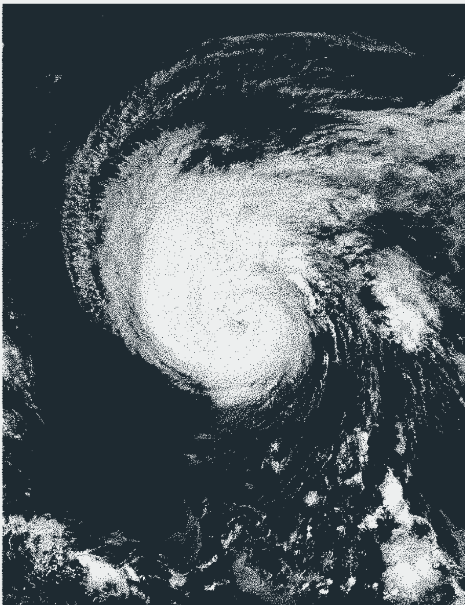
PLATE 2 Hurricane Isabel as it approached landfall on the outer banks of North Carolina on September 18, 2003. The image is a true-color (red-green-blue) NASA image taken by the Moderate-resolution Imaging Spectroradiometer (MODIS)—the research equivalent of the Visible and Infrared Imager/Radiometer Suite (VIIRS) to be flown on NPP and operationally by NPOESS in three orbit planes (with global coverage every 4 hours) beginning in 2009. SOURCE: Courtesy of NASA Goddard Space Flight Center.
