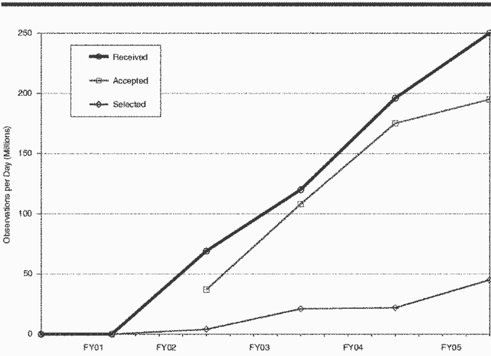
FIGURE 5.1 Use of operational satellite data over the past several years. SOURCE: "The Role of Satellite Data in Environmental Modeling," Louis Uccellini, director, NCEP, presentation to the National Research Council Committee on Environmental Satellite Data Utilization, September 11, 2003.
