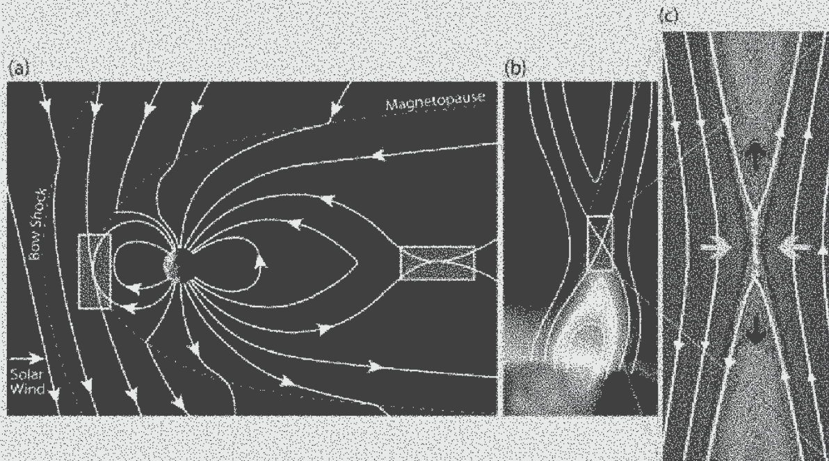
FIGURE 1.4.1 Regions of reconnection (boxed areas) occur in many locations in astrophysical systems, including (a) Earth's magnetosphere and (b) the solar corona. Panel (c) shows a computer simulation of reconnection showing magnetic field lines (white) and strong electrical currents. Oppositely directed magnetic field lines, together with the plasma, flow toward the center of the picture from the sides (light arrows). The field lines reconnect at the center and accelerate strongly outward (up and down) in a slingshot action. The resulting release of magnetic energy produces high-speed plasma flows (dark arrows) and large numbers of energetic particles. Electrons that are accelerated by electric fields to velocities close to the speed of light power the aurora and drive radio bursts from the Sun. SOURCES: (a) Committee on the Assessment of the Role of Solar and Space Physics in NASA's Space Exploration Initiative, (b) Yohkoh SXT science team, and (c) M. Shay, University of Maryland.
