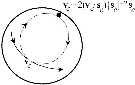
Figure 3.7. Reconnection on the Kibble–Turok sphere.
