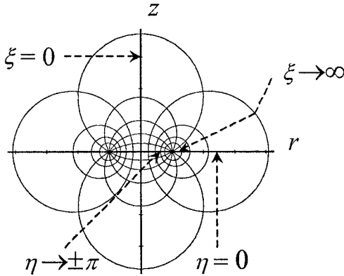
Figure 10.1. The toroidal coordinate system.
