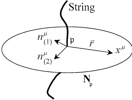
Figure 1.5. The normal plane \mathbf{N}_p .
