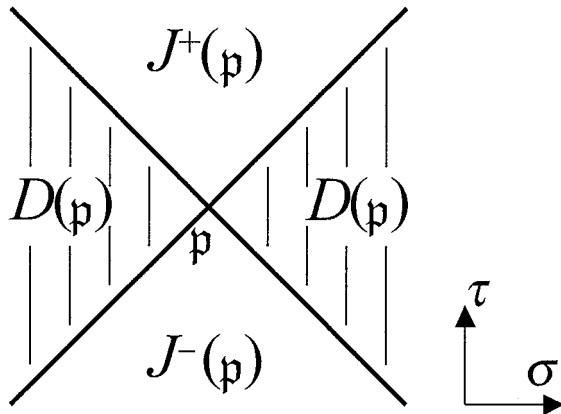
Figure 2.1. Causal structure of an infinite string.
