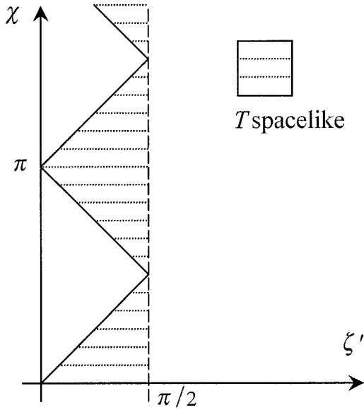
Figure 8.2. The metrized parameter space for an arbitrary system of parallel cosmic strings.
