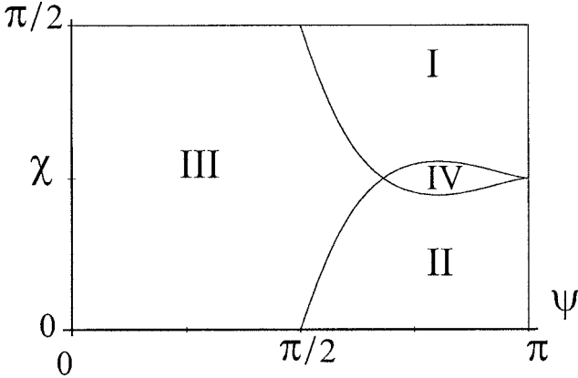
Figure 6.7. Orientations of the divergent contributions to the self-acceleration near a cusp.
