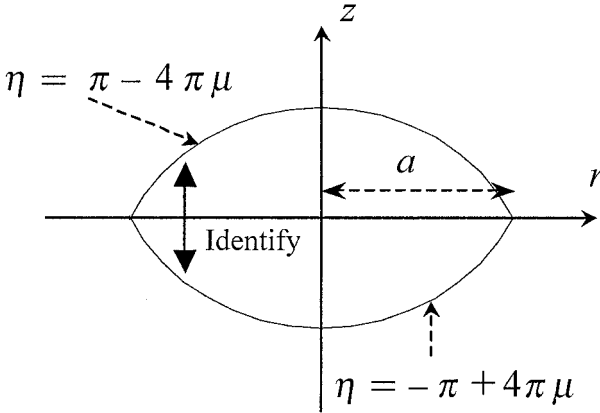
Figure 10.2. Excising the wedge -\pi + 4\pi\mu < \eta < \pi - 4\pi\mu .
