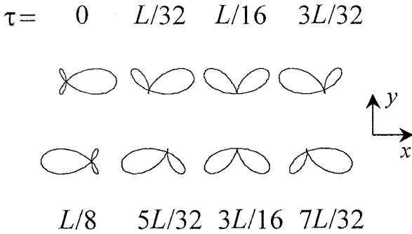
Figure 4.20. The 2/1 harmonic string with \psi = \frac{1}{2}\pi in the x - y projection.
