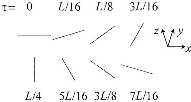
Figure 4.17. The same string projected onto the plane spanned by \hat{x} and \hat{y} + \hat{z} .
