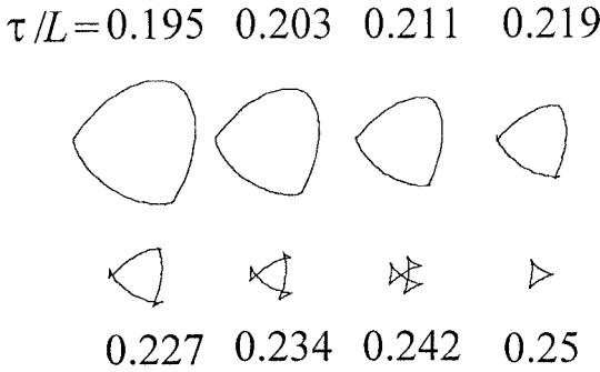
Figure 4.32. The teardrop string for 0.195 \leq \tau/L \leq 0.25 .
