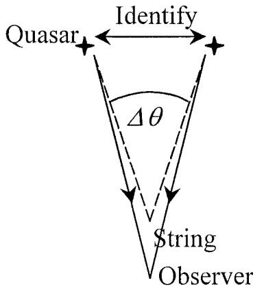
Figure 7.2. Gravitational lensing of the light from a distant quasar by an intervening string.
