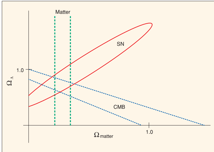
FIGURE 5.2 Concordance of the three independent measurements of the mass/energy density of the universe, as indicated by their intersection. The two axes are the dark energy (vertical) and matter (horizontal). The ellipse denotes the supernova measurements, which indicate that the expansion of the universe is speeding up. The vertical lines correspond to measurements of the dark matter density and the sloping triangle represents the CMB measurements that indicate a flat, critical universe (here, matter plus dark energy sum to one).
