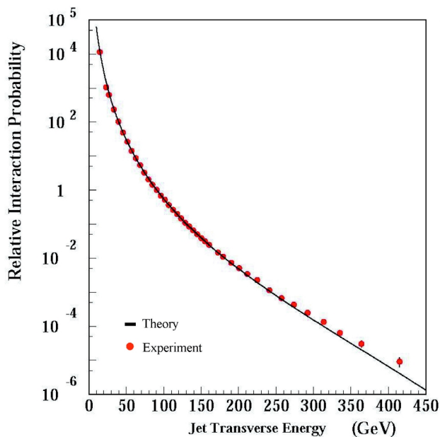
FIGURE 2.2 An example of one of the many successes of the quantum chromodynamics (QCD) sector of the Standard Model. Shown are theoretical predictions (black solid curve), which agree well with experimental data (red points) over 11 orders of magnitude. The data come from high-energy proton-antiproton collisions at Fermilab’s Tevatron. The plot shows the relative rate of quark and gluon jet production carrying energy of the amount shown on the horizontal axis, in a direction transverse to the incoming proton and antiproton directions. Adapted from an image courtesy of the D0 Collaboration.
