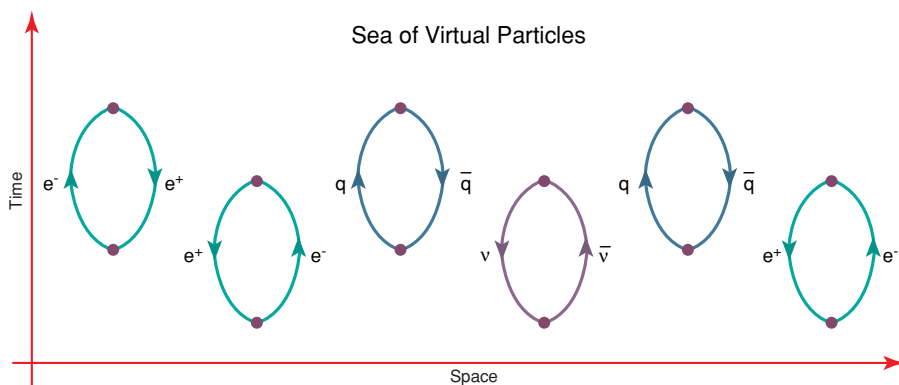
FIGURE 2.2.1 According to the rules of quantum field theory, the vacuum is not empty but it is actively populated by particle-antiparticle pairs that appear, annihilate, and disappear, existing for only brief instants.
