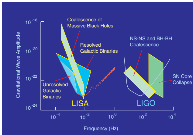
FIGURE 6.4.3 A comparison of the sensitivities of the two laser interferometer projects (LIGO and LISA) to gravitational waves of different frequencies. Different sources of gravity waves are expected to produce waves of different kinds; the LIGO and LISA project are expected to complement each other to cover a broader range of the gravity wave spectrum. Figure courtesy of the Jet Propulsion Laboratory, California Institute of Technology, Pasadena, California.
