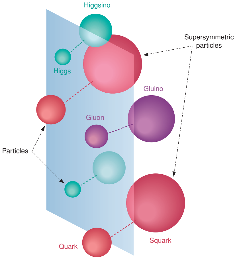
FIGURE 2.4.1 Depiction of the one-to-one correspondence of supersymmetric partner particles for every type of ordinary particle. Because the superpartners are expected to be very massive, they have not yet been directly observed.
