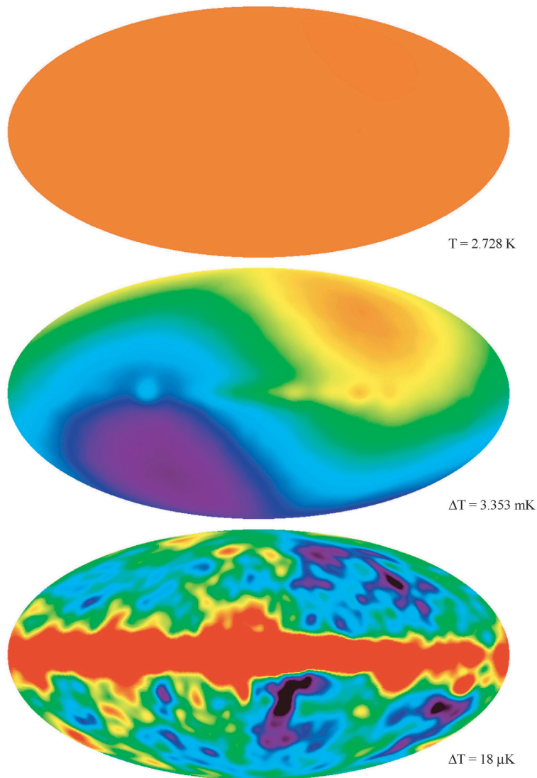
FIGURE 4.4 False color maps of the temperature of the CMB measured by the Differential Microwave Radiometer (DMR) on COBE from the 4-year dataset. The top image shows the remarkable uniformity of the CMB, which testifies to the large-scale homogeneity of the universe. The middle image shows the dipole anisotropy due to the motion of the solar system at 370 km/sec. The bottom image shows the 30-microkelvin fluctuations discovered by COBE that rose from the small (0.001 percent) variations in primeval matter density (the bright band across the middle is the microwave emission from our own galaxy). Image courtesy of NASA.
