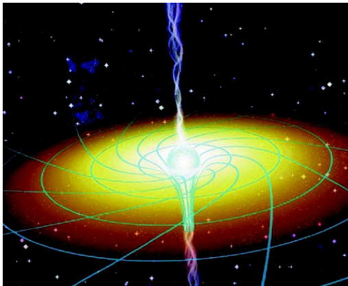
FIGURE 6.1 Frame dragging near a massive, rotating black hole. All matter must follow the black hole's spin when it gets very close to the event horizon. Image courtesy of Joe Bergeron ©2001, < www.joebergeron.com >.
