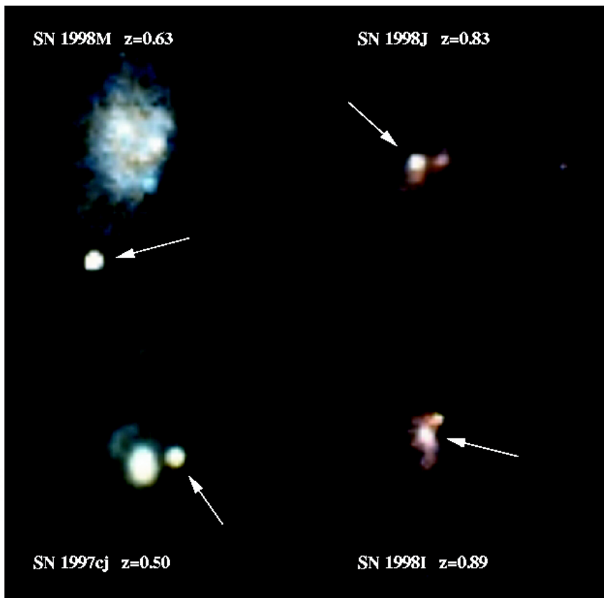
FIGURE 5.7 Images of distant Type Ia supernovae. For about a month, these thermonuclear stellar explosions produce about as much light as the rest of the stars in the galaxy combined. Image courtesy of NASA.
