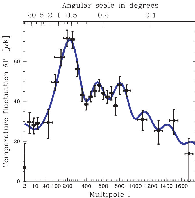
FIGURE 5.3 Power spectrum of cosmic microwave background (CMB) fluctuations measured by the BOOMERanG, MAXIMA, and DASI experiments. The height of the curve is a measure of temperature differences, while the horizontal axis is a measure of the angular separation, with larger values of l corresponding to smaller angles. The position of the first peak indicates that we live in a flat universe; the ratio of the amplitudes of the first and second peaks indicates a baryon density of around 4 percent, consistent with the big bang nucleosynthesis determination. The solid curve is the theoretical prediction for a flat universe whose composition is 4 percent ordinary matter, 29 percent cold dark matter, and 67 percent dark energy. Image courtesy of M. Tegmark and M. Zaldarriaga, 2002.
