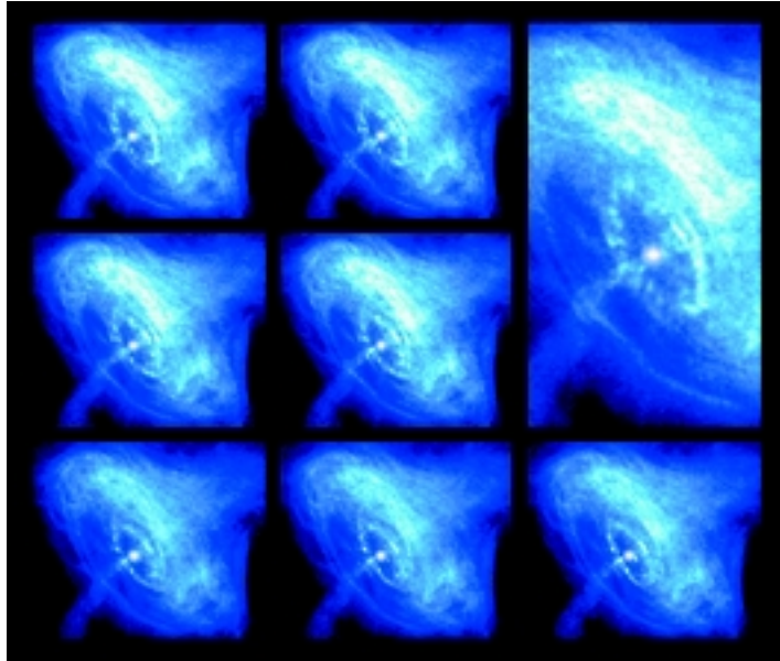
FIGURE 6.3 Time-lapse, false-color x-ray images of the hot spinning disk of gas surrounding the neutron star with the Crab Nebula taken by the Chandra X-ray Observatory over the course of several months. Image courtesy of NASA/CXC/ASU/J. Hester et al.
