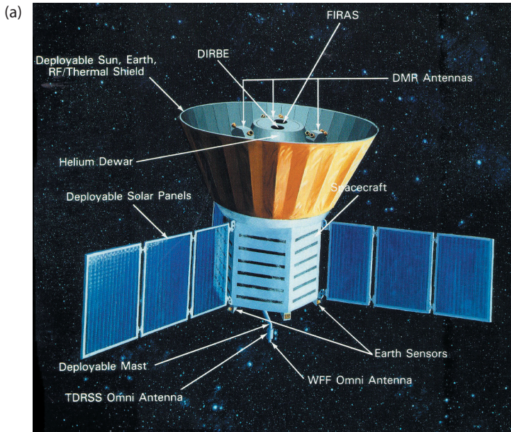
FIGURE 4.1 (a) NASA’s COsmic Background Explorer (COBE) satellite as depicted orbiting Earth. COBE was launched in 1989 and made precision measurements of the CMB radiation and discovered the 30 microkelvin variation in its intensity across the sky; image courtesy of NASA. (b) Measurements made by the Balloon Observation of Millimetric Extragalactic Radiation and Geophysics (BOOMERanG) balloon experiment launched in 1998 helped to establish that the universe is flat; image courtesy of the BOOMERanG Collaboration. (c) The Degree Angular Scale Interferometer (DASI) telescope in Antarctica. Measurements by DASI showed that the density of ordinary matter is small (about 4 percent) and revealed the first evidence of CMB polarization; image courtesy of the DASI Collaboration.
