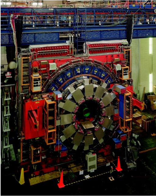
FIGURE 2.3 The Tevatron at the Fermi National Accelerator Laboratory collides protons and antiprotons with high enough energy to bring the constituent quarks very close together, allowing them to interact. Occasionally, a pair of top quarks is produced, each of which has about the mass of a gold atom. The top quarks quickly decay further into lighter particles. The Collider Detector Facility (above) and the D0 detector (right) are two experiments located at different points where the particles are brought into collision. Images courtesy of Fermilab.
