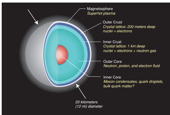
FIGURE 6.2.1 Schematic of the interior of a neutron star showing the layers of packed and compressed matter. Condensed matter physics can tell us many things about the forms that matter takes, except at the very center of the neutron star, where densities exceed those of nuclear matter.
