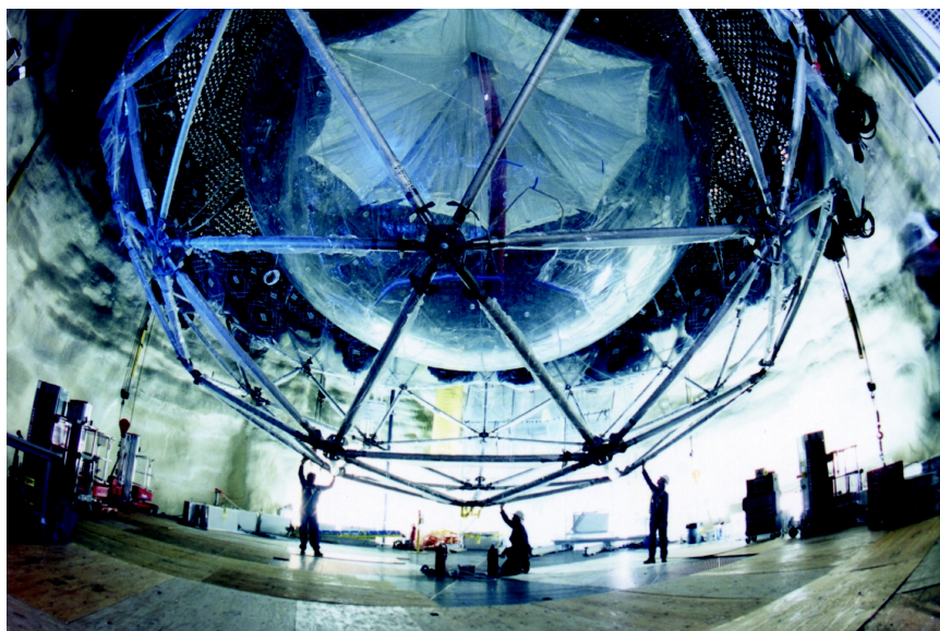
FIGURE 3.3 The Sudbury Neutrino Observatory (SNO). SNO consists of 1,000 tons of heavy water (made of deuterium and oxygen rather than hydrogen and oxygen) contained in an acrylic vessel (viewed here with a fisheye lens) and surrounded by 9,500 photomultiplier tubes. Neutrino interactions with heavy water reveal separately the number of electron neutrinos and other types. Image courtesy of Lawrence Berkeley National Laboratory.
