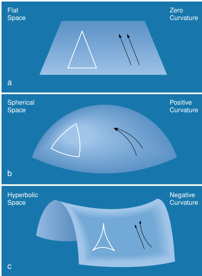
FIGURE 5.2.1 Three-dimensional curved space is not possible to visualize, but curvature in two dimensions can be illustrated. A positively curved universe is like the surface of a sphere; a negatively curved universe, like a saddle. A universe with zero curvature is like a plane. The geometry of curved space, two- or three-dimensional, is different: parallel lines may intersect (positively curved space) or may diverge (negatively curved space) and the sum of angles in a triangle may be more than 180 degrees (positively curved space) or less than 180 degrees (negatively curved space). The CMB determination of the curvature of space relied upon these facts.
