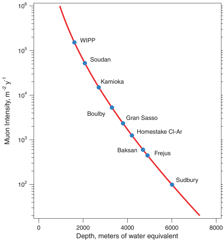
FIGURE 7.1 The number of penetrating cosmic-ray muons vs. overburden of earth (measured in mwe—meters of water equivalent; 1 mwe is approximately 1 foot of material). Existing underground labs are WIPP, Homestake, and Soudan in the United States; Kamioka in Japan; Boulby, Gran Sasso, Baksan, and Frejus in Europe; and Sudbury in Canada. There is a deeper option in the Homestake mine at about the same depth as Sudbury. Figure courtesy of R.G.H. Robertson.
