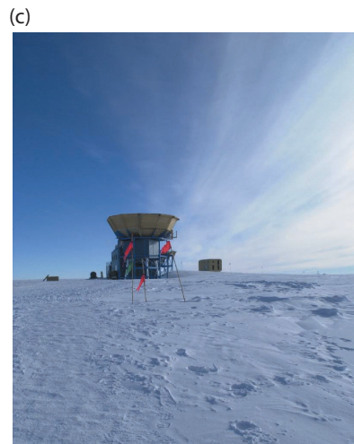
FIGURE 4.1 (a) NASA’s COsmic Background Explorer (COBE) satellite as depicted orbiting Earth. COBE was launched in 1989 and made precision measurements of the CMB radiation and discovered the 30 microkelvin variation in its intensity across the sky; image courtesy of NASA. (b) Measurements made by the Balloon Observation of Millimetric Extragalactic Radiation and Geophysics (BOOMERanG) balloon experiment launched in 1998 helped to establish that the universe is flat; image courtesy of the BOOMERanG Collaboration. (c) The Degree Angular Scale Interferometer (DASI) telescope in Antarctica. Measurements by DASI showed that the density of ordinary matter is small (about 4 percent) and revealed the first evidence of CMB polarization; image courtesy of the DASI Collaboration.
