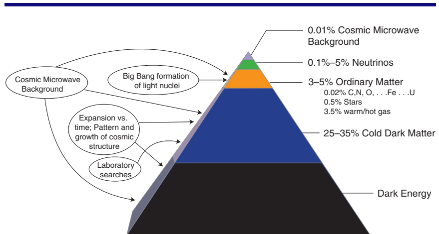
FIGURE 5.4 Pyramid diagram of the composition of the universe and the different techniques that can be used to measure the various components. For instance, evidence for dark matter comes from cosmic microwave background radiation and the pattern of cosmic structure. Laboratory searches have the potential to identify dark matter by detecting halo dark matter particles or producing it in accelerators.
