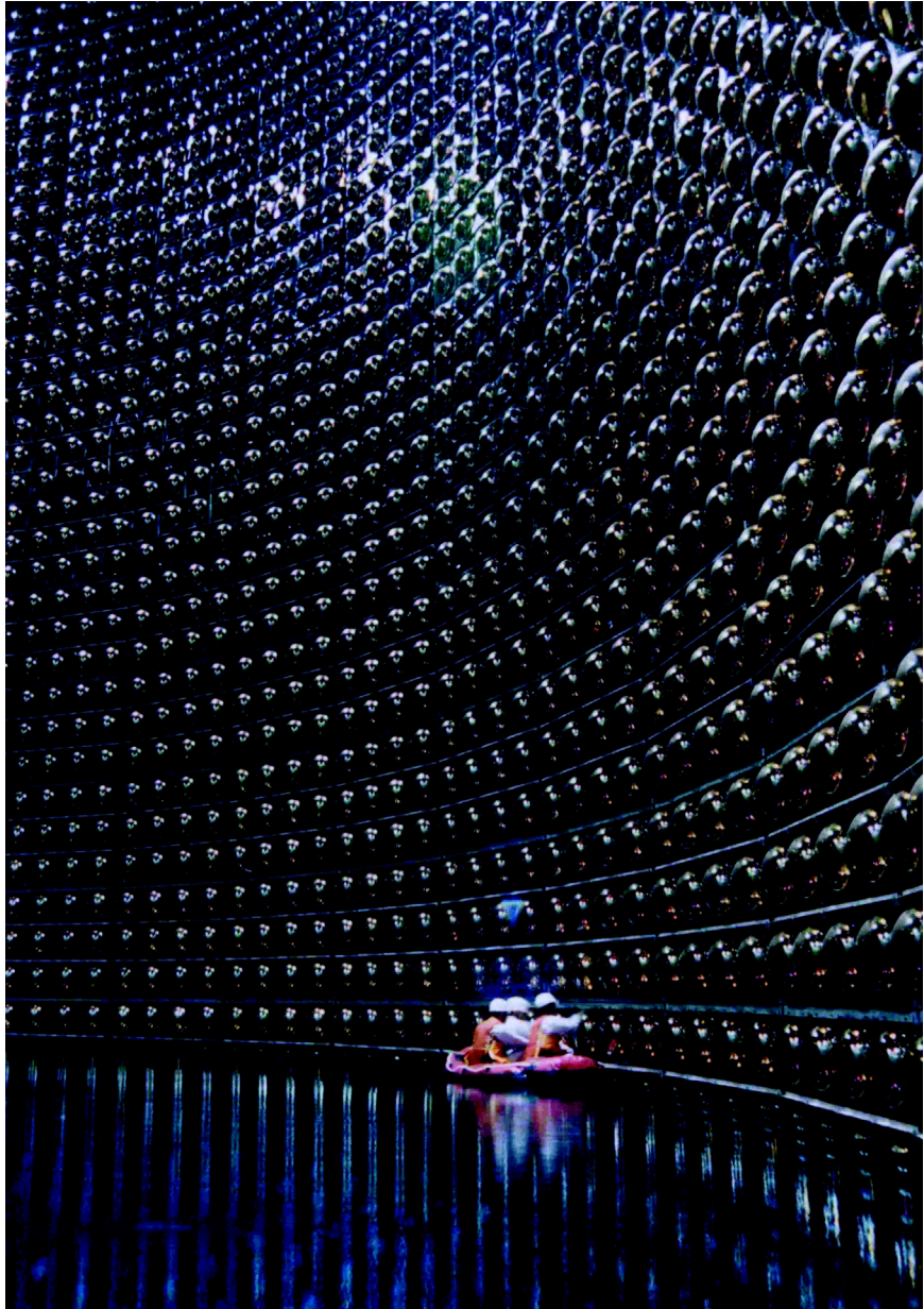
FIGURE 3.2 The Super-Kamiokande detector. Here, scientists (in a rubber raft) inspect the large photomultiplier tubes as the enormous tank is filled with water. Image courtesy of the Institute for Cosmic Ray Research, University of Tokyo.
