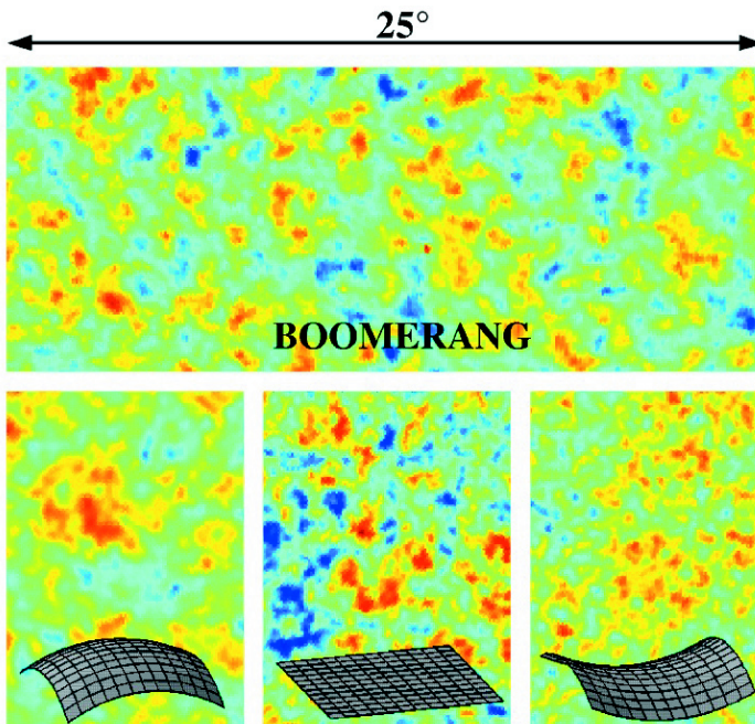
FIGURE 5.1 The pattern of hot and cold spots on the cosmic microwave background (CMB) sky expected in a high-density, closed universe; in a critical-density, flat universe; and in a low-density, open universe (bottom, from left to right) and the real map of the CMB sky made by the BOOMERanG experiment (top). The tiny temperature variations map the distribution of matter 400,000 years after the big bang; their angular size is determined by the shape of the universe. The BOOMERanG results indicate that we live in a spatially flat universe. Image courtesy of the BOOMERanG Collaboration.
