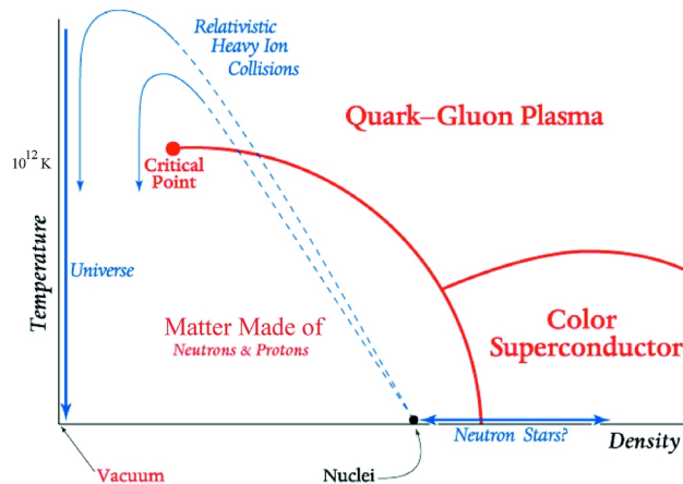
FIGURE 6.4 The phase diagram for quark-based, ordinary matter. At high temperatures or density, a transition from nuclear matter to a plasma of quarks and gluons takes place. Quark-gluon plasmas can be produced at high temperature and low density (early universe), at low temperature and high density (neutron stars), or at moderate temperature and density (at the RHIC facility). The three different methods of producing quark-gluon plasma probe different aspects of the transition. Image courtesy of K. Rajagopal and M. Stock.
