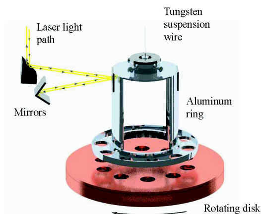
FIGURE 3.4 Extra dimensions that are open to gravitational interactions may explain gravity’s apparent weakness in our four dimensions. If those dimensions are “curled up” on the scale of fractions of a millimeter, it may be possible to observe a strengthening of the gravitational force at very short distances. The highly sensitive short-range torsion balance shown here is used to detect this effect. An aluminum ring was suspended by a fine tungsten wire above a disk that rotated once every 2 hours. The ring and disk both had 10^{3/8} -inch-diameter holes bored into them. The gravitational force between the “missing mass” in the two sets of 10 holes produced a twist on the ring that varied back and forth 10 times for each revolution of the disk. The disk’s twist was measured by bouncing a laser beam off one of two mirrors mounted above the ring. So far, extra dimensions of extent greater than 0.2 mm have been ruled out by experiments such as this one. Image courtesy of E. Adelberger, B. Heckel, and E. Swanson, University of Washington.
