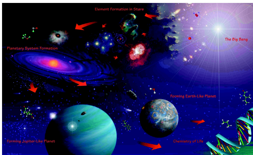
FIGURE 1.1.1 The universe today is the product of a long, long chain of events, as shown in this artist's conception of cosmological evolution beginning with the big bang. Scientists are exploring not only the chronological relationships between these events but also the causal connections. Image courtesy of NASA.
