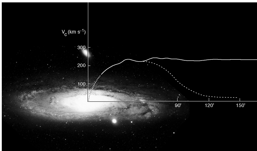
FIGURE 5.5 An image of the Andromeda galaxy with its rotation curve (velocity of gas clouds and stars orbiting the center of the galaxy vs. distance from the center). The constancy (flatness) of the rotation curve beyond the point where the light ends indicates the presence of dark matter that holds the galaxy together. The dashed line fading back to zero shows what the rotation curve would look like in the absence of dark matter. Image courtesy of M. Roberts.
