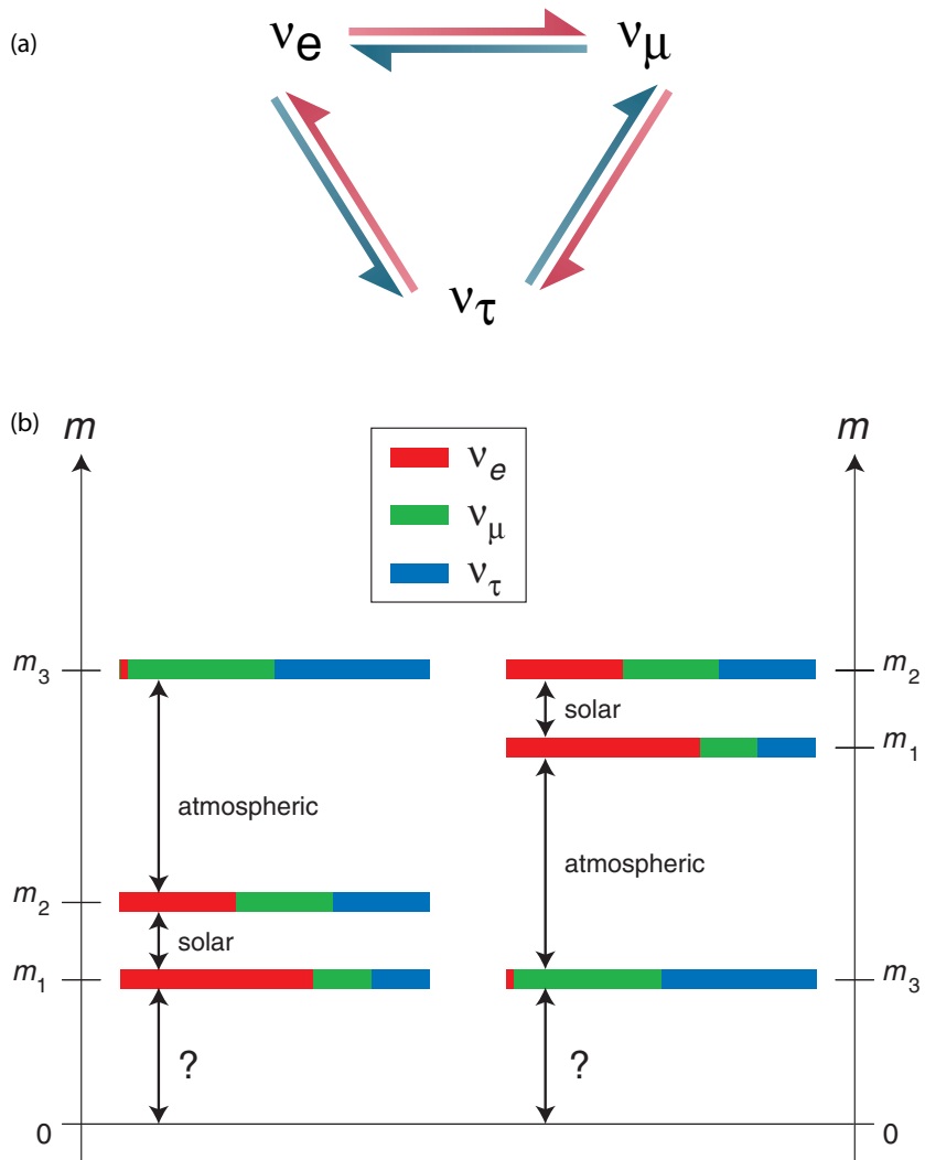
FIGURE 3.1 (a) If neutrinos have mass, the different types mix with one another, as indicated in the first diagram. The so-called neutrino mixing parameters correspond to the arrows in each direction. It is because of this mixing that one flavor of neutrino can “disappear” (and reappear as a another flavor that has different detailed interactions) and be noted as a deficit in the detector. (b) Two mass schemes for neutrinos are consistent with measurements of atmospheric and solar neutrinos. The three “mass states” are mixtures of the different neutrino types, as illustrated in the second figure. Note, too, that the solar and atmospheric neutrino experiments determine mass differences and do not set the absolute scale of neutrino masses. Image courtesy of H. Murayama, University of California at Berkeley.
