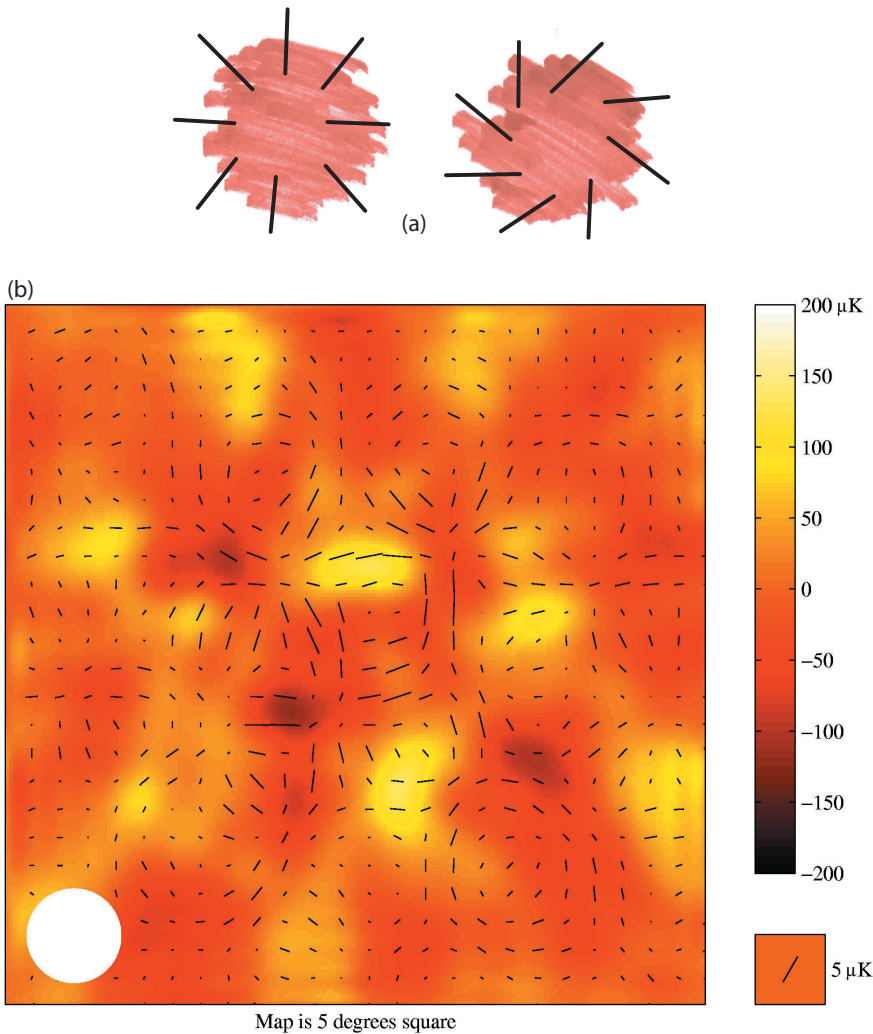
FIGURE 4.6 (a) A cartoon sketch showing polarization measurements of the CMB. The small temperature variations in the CMB are shown in false color, with yellow hot and red cold. The polarization of each spot is shown by a black line segment. The length of the line segment shows the strength of the polarization, and the orientation shows the direction in which the radiation is polarized. E-mode polarization (left) is characterized by a radial pattern and B-mode (right) polarization is indicated by a circulation pattern. (b) An image of the intensity and polarization of the CMB radiation made from DASI at the South Pole. The white spot in the corner shows the approximate angular resolution of DASI's polarimeter. This measurement, the first of its kind, is the type necessary to detect gravity waves through CMB polarization maps. Image courtesy of the DASI Collaboration.
