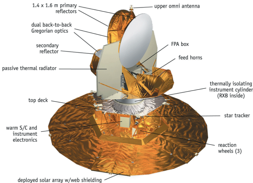
FIGURE 4.5 The MAP satellite as designed and launched in June 2001. To address its key scientific questions, MAP measures small variations in the temperature of the cosmic microwave background radiation with 30 times the angular resolution of the decade-earlier COBE satellite. The first significant results are expected in early 2003. Image courtesy of NASA.
