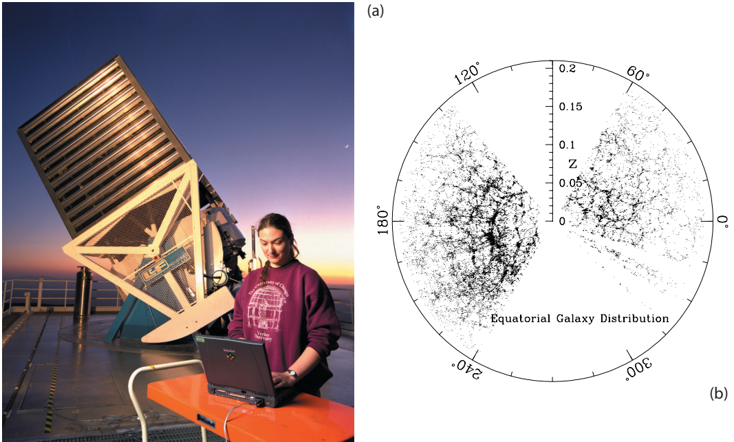
FIGURE 4.3 The Sloan Digital Sky Survey (SDSS) project uses a telescope in New Mexico to make a detailed map of the night sky. (a) Constance Rockosi, a graduate student at the University of Chicago and a member of the multi-institutional team that built the digital scanning camera for the Sloan Digital Sky Survey, checks the status of the instrument during its first on-the-sky trial runs in May 1998. (b) Based on the data collected through April 2002, the team released this map of one sector of the visible universe. The filaments, walls, and voids within the structure defined by the positions of about 65,000 galaxies define the “large-scale structure” of the universe. Images courtesy of Fermilab Visual Media Services.
