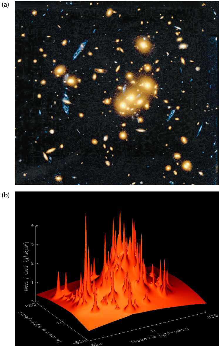
FIGURE 5.6 (a) Hubble Space Telescope image of the gravitational lensing of light from distant galaxies (distorted and multiple blue images) by a more nearby cluster (orange galaxies). (b) Derived map of the mass that must be between the distant galaxies and our observation point to cause the gravitational lensing. The height of the surface is proportional to the projected mass density. Images courtesy of NASA, W.N. Colley, E. Turner, and J.A. Tyson.
