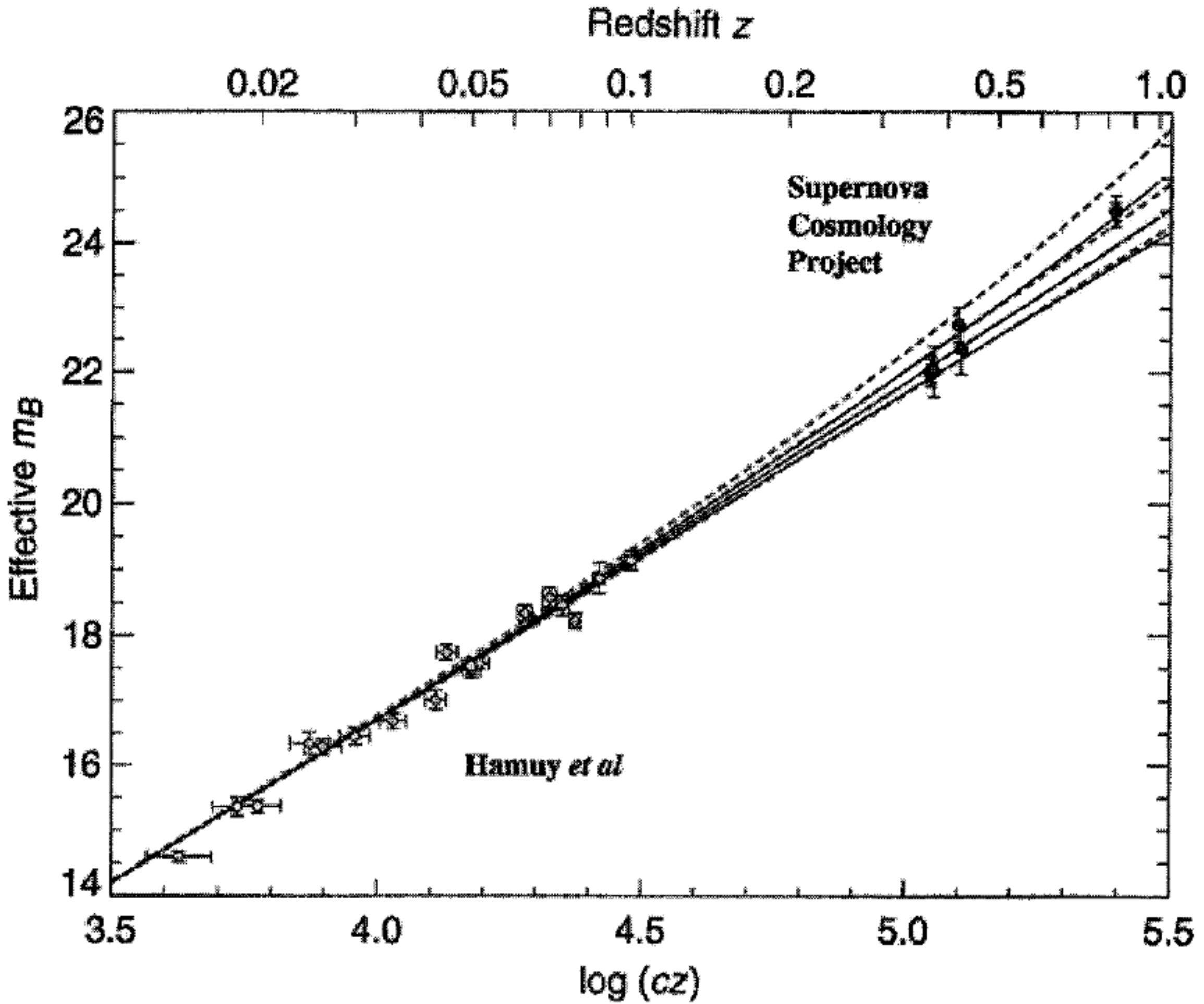
Figure 6.3. Hubble plot of effective magnitude against \log cz . The full curves are computed from models for various values of \Omega_M and \Omega_\Lambda with, from the top down, (\Omega_M, \Omega_\Lambda) = (0, 0), (1, 0), (2, 0) and similarly for the dotted curves (\Omega_M, \Omega_\Lambda) = (0, 1), (0.5, 0.5), (1, 0), (1.5, -0.5) . The experimental points are from type 1a supernovae (Perlmutter et al 1998).
