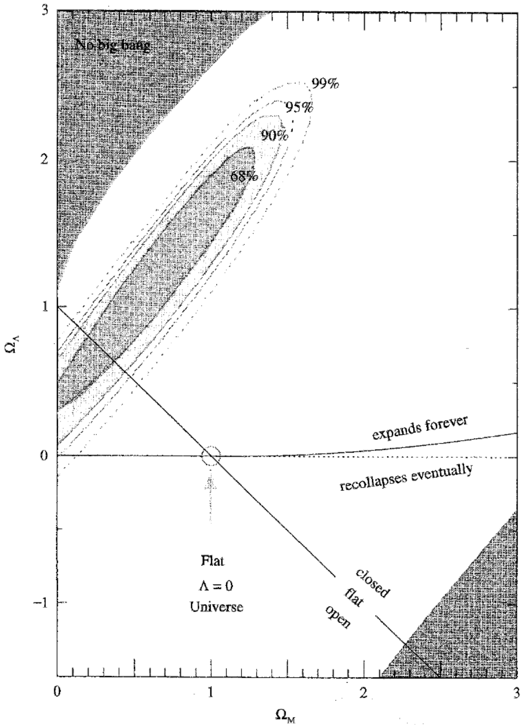
Figure 6.4. Allowed ranges of \Omega_M and \Omega_\Lambda showing the confidence regions obtained from observations of type 1a supernovae by the Supernova Cosmology Project (Goldhaber and Perlmutter 1998).
