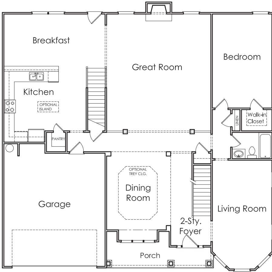
FIRST FLOOR
