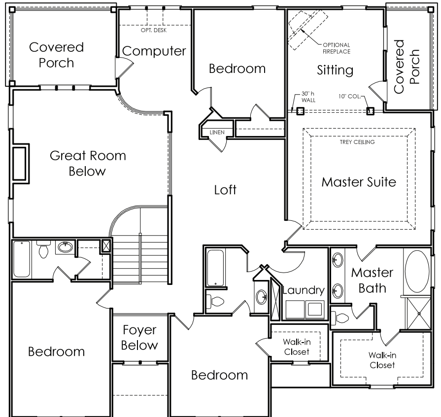
SECOND FLOOR
