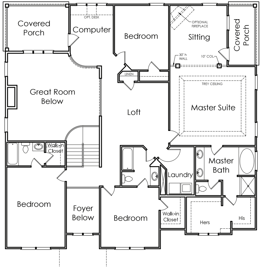
SECOND FLOOR
